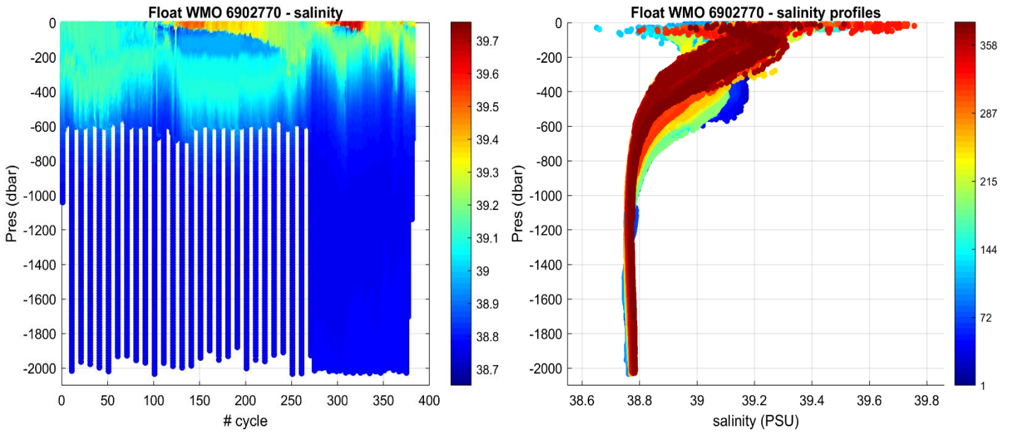
Figure 3: Float 6902770. Time series of Argo float potential salinity (PSS-78) on the left, and salinity profiles color-coded per cycle number on the right.
