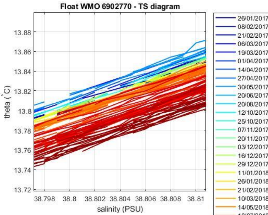
Figure 5: Float 6902770. Area of the \theta -S diagram (color-coded per cycle number) where the \theta -S relationship is more uniform.
