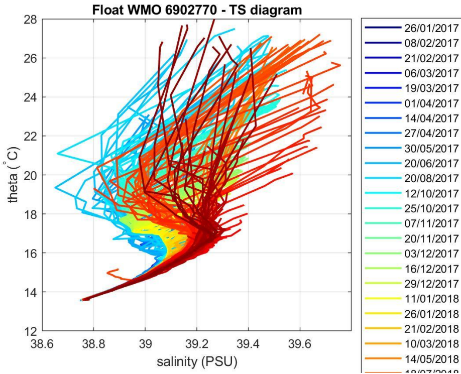
Figure 4: Float 6902770. \theta -S diagram color-coded per cycle number.
