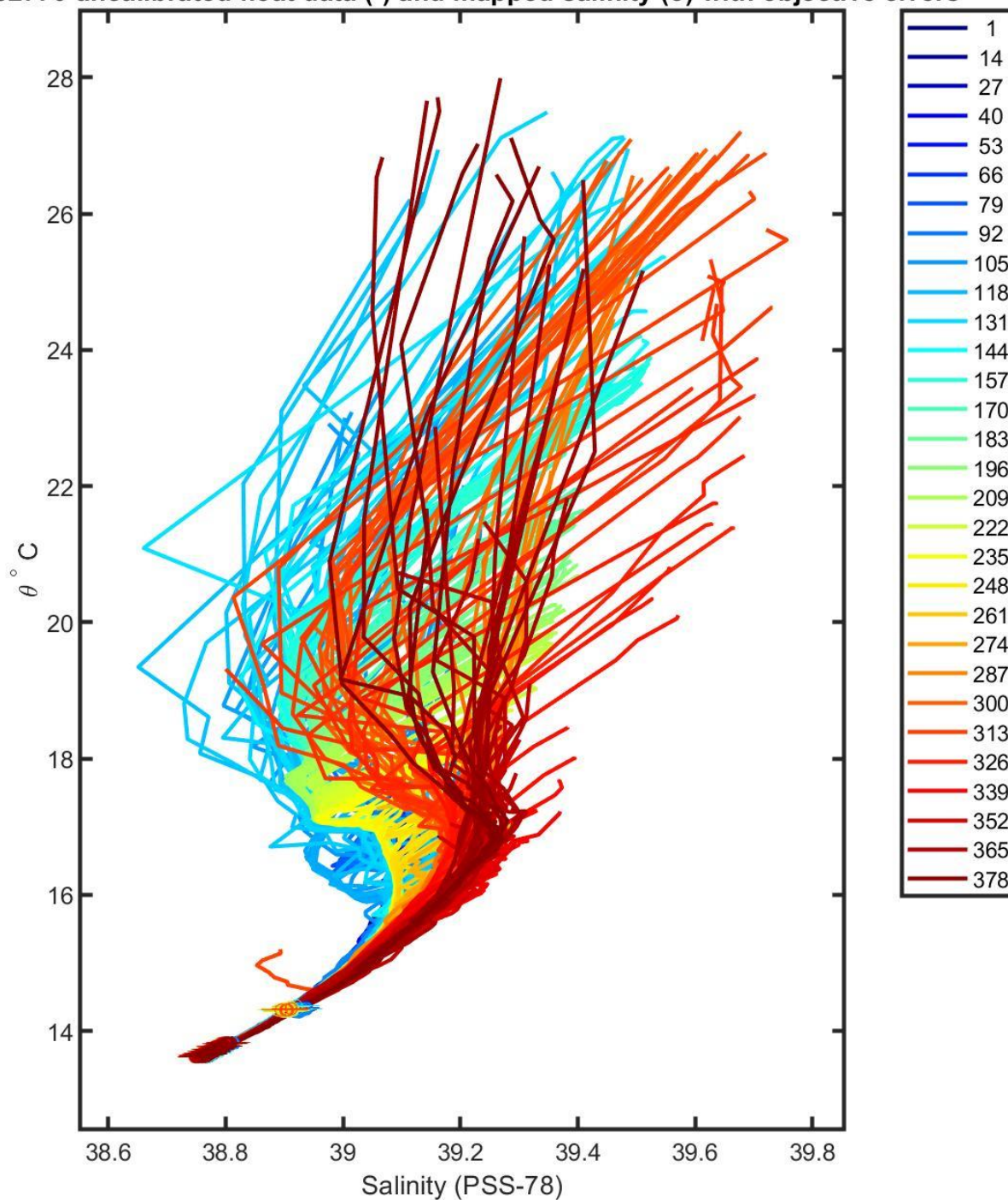
6902770 uncalibrated float data (-) and mapped salinity (o) with objective errors
