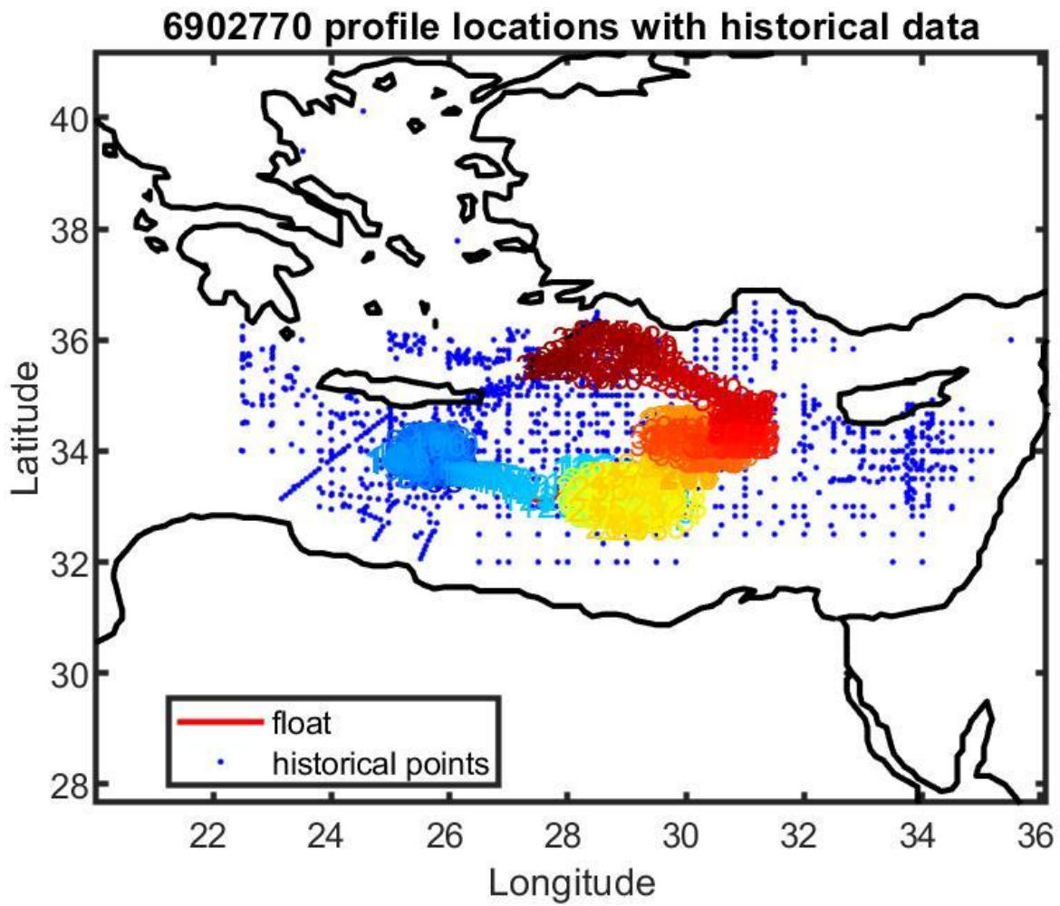
Figure 13: Float 6902770. Location of the float profiles (red line with colored numbers) and the reference data selected for mapping (blue dots).
