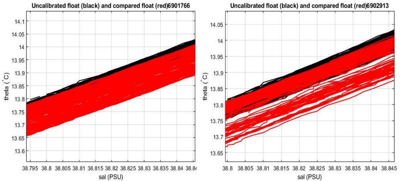
Figure 21: Float 6902770. Comparison between float 6902770 (black line) and other floats (red line), in the most uniform part of the \theta -S curve.
