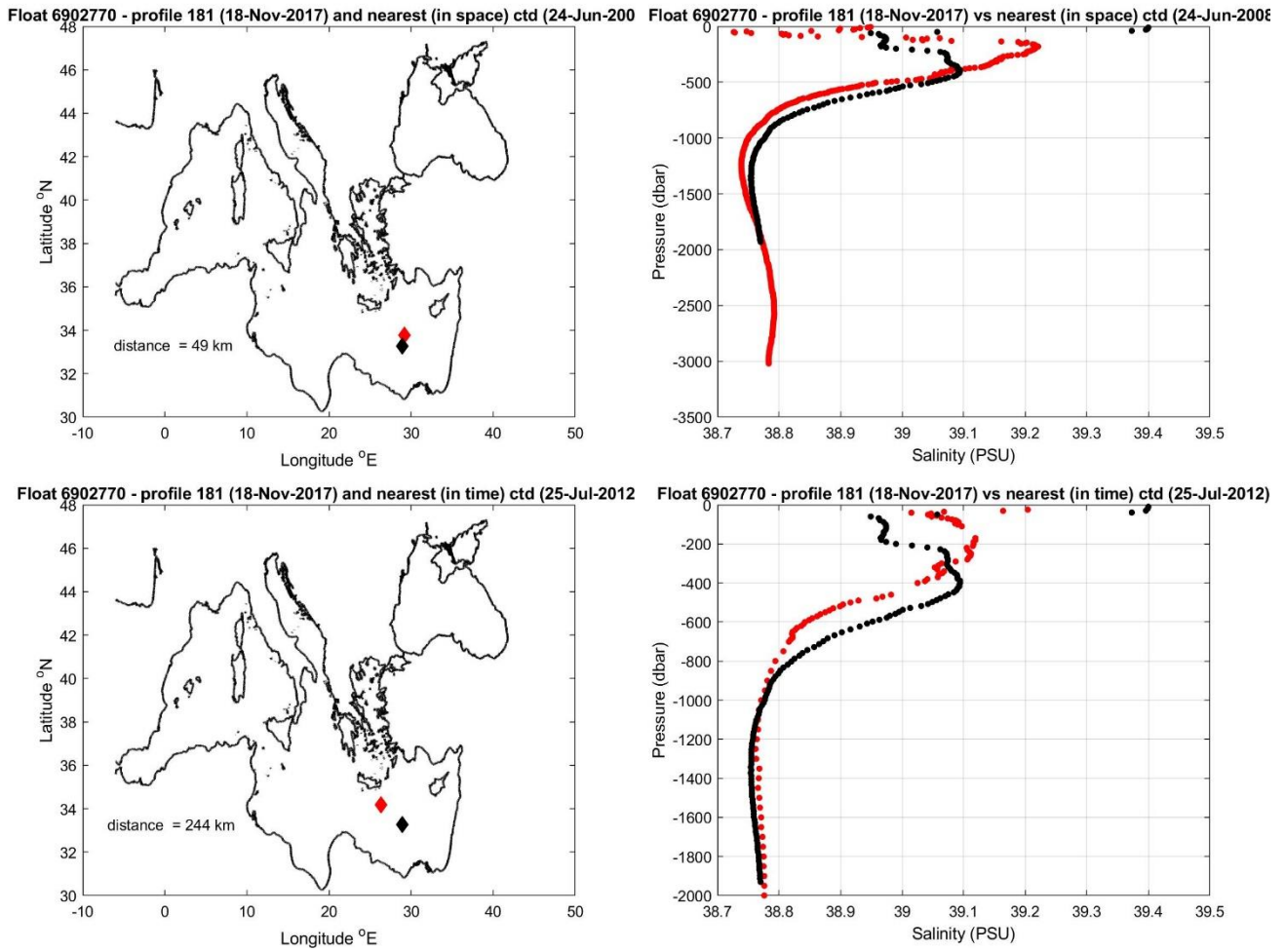
Figure 10: Float 6902770. The salinity float profile number 181 (black dots) are compared to the nearest in space (top) and in time (bottom) reference profile (red dots). The locations of the two profiles and their distance is given in the left panel.
