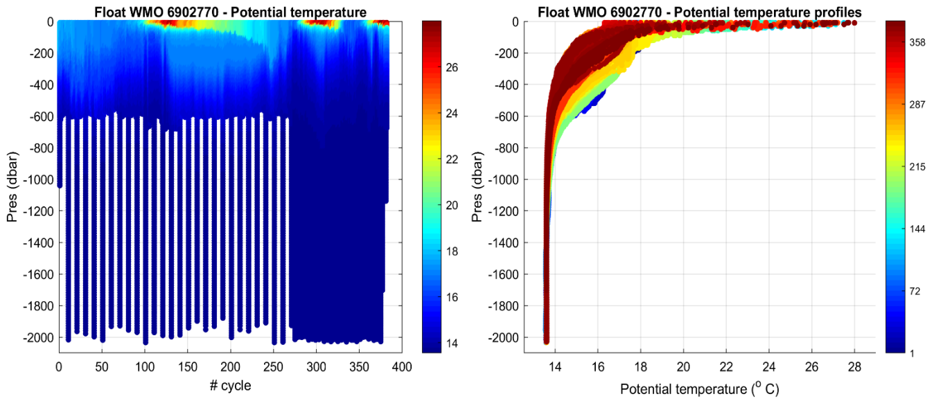
Figure 2: Float 6902770. Time series of Argo float potential temperature ( ^{\circ}\text{C} ) on the left, and potential temperature profiles color-coded per cycle number on the right.
