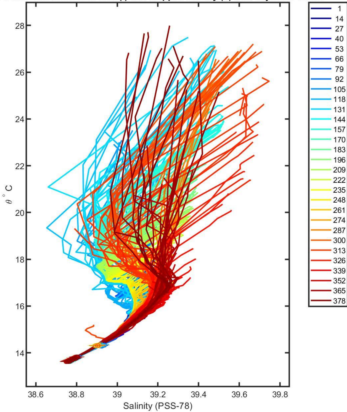
6902770 calibrated float data (-) and mapped salinity (o) with objective errors
