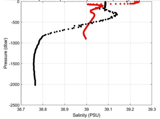
Float 6902770 - profile 51 (17-Mar-2017) vs nearest (in time) ctd (19-Dec-2013)
