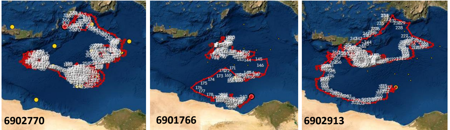
Figure 20: Float 6902770. Trajectory of the floats used for the comparison.
