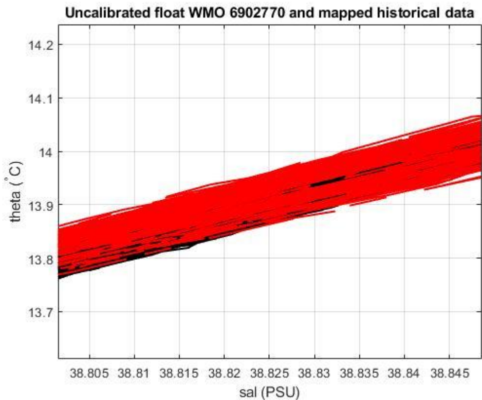
Figure 19: Float 6902770. Uncalibrated float salinity profile (black lines) and mapped historical data (red lines) in the most uniform part of the \theta -S curve.
