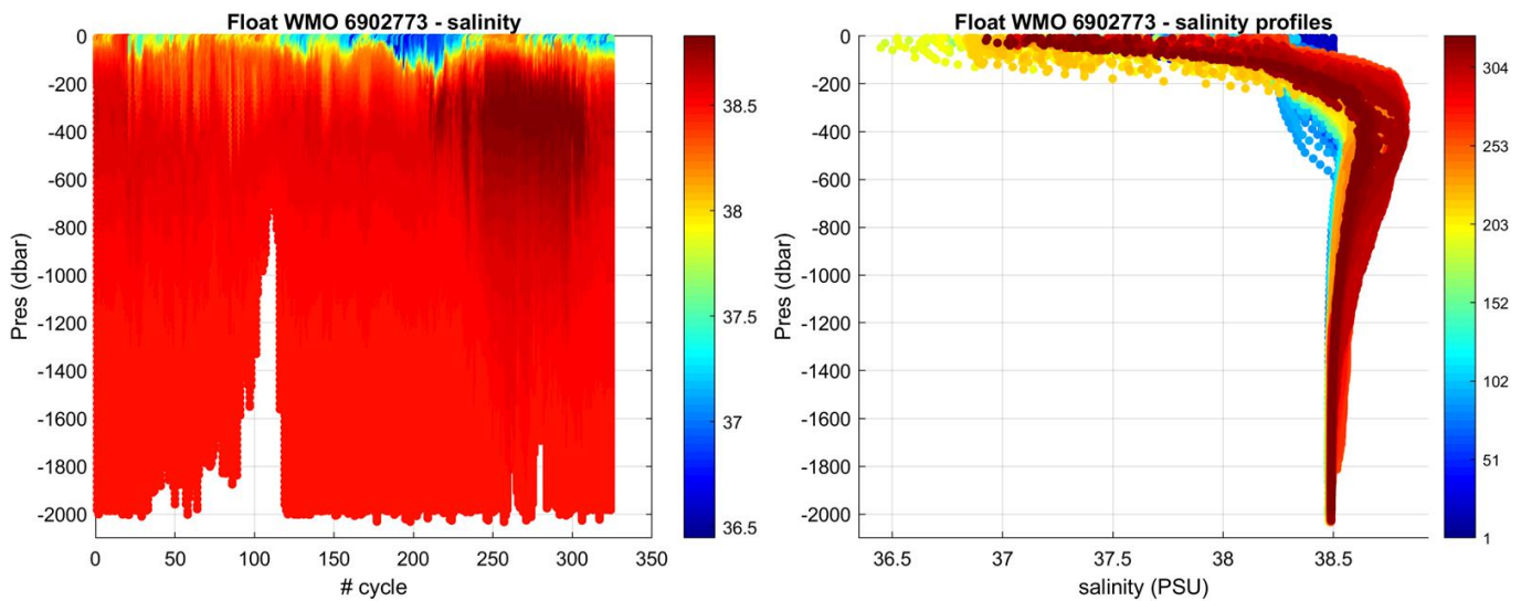
Figure 3: Float 6902773. Time series of Argo float potential salinity (PSS-78) on the left, and salinity profiles color-coded per cycle number on the right.
