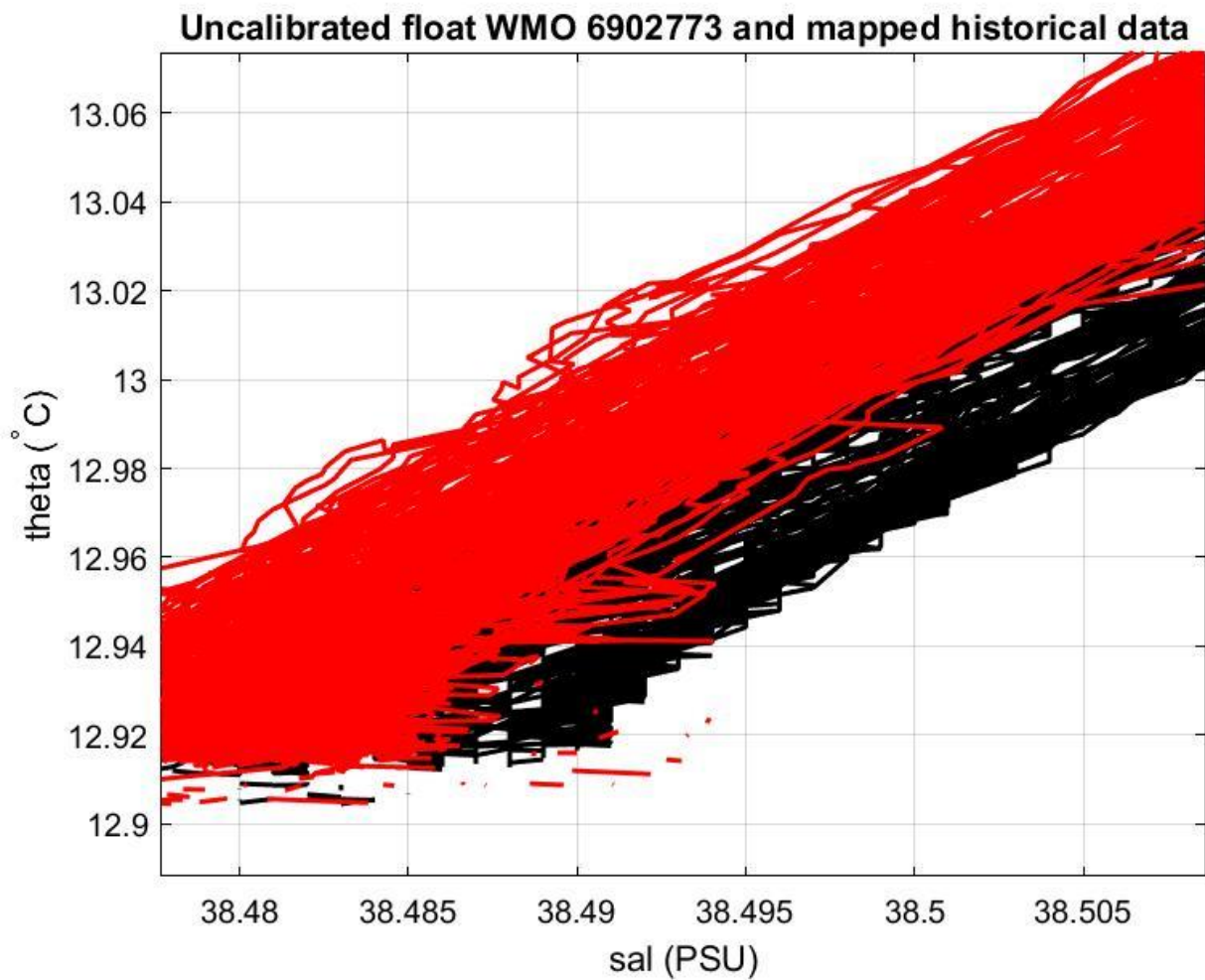
Figure 18: Float 6902773. Uncalibrated float salinity profile (black lines) and mapped historical data (red lines) in the most uniform part of the \theta -S curve.
