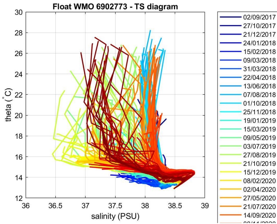
Figure 4: Float 6902773. \theta -S diagram color-coded per cycle number.
