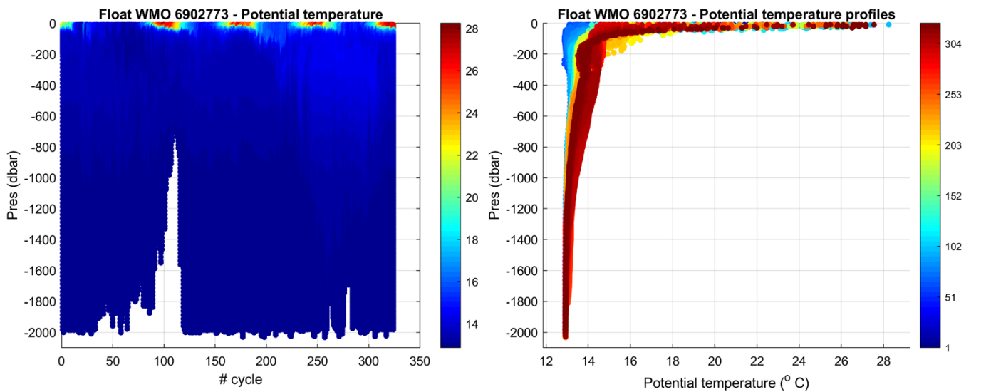
Figure 2: Float 6902773. Time series of Argo float potential temperature ( ^{\circ}\text{C} ) on the left, and potential temperature profiles color-coded per cycle number on the right.
