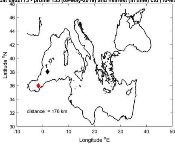
Figure 10: Float 6902773. The salinity float profile number 155 (black dots) are compared to the nearest in space (top) and in time (bottom) reference profile (red dots). The locations of the two profiles and their distance is given in the left panel.
