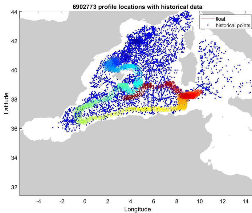
Figure 12: Float 6902773. Location of the float profiles (red line with colored numbers) and the reference data selected for mapping (blue dots).
