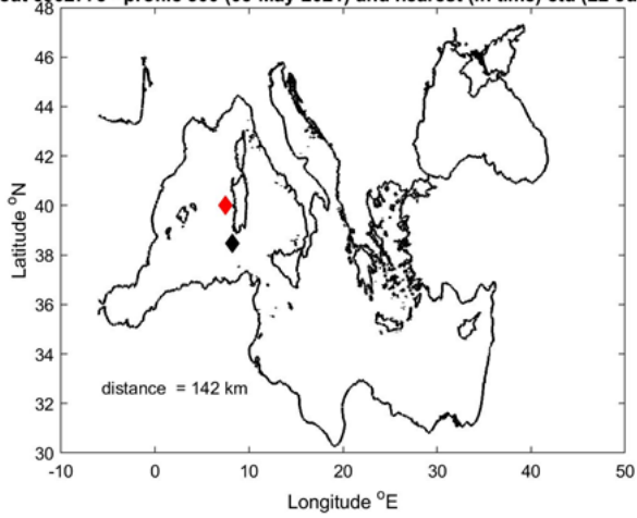
Float 6902773 - profile 300 (03-May-2021) and nearest (in time) ctd (22-Jun-2019)
