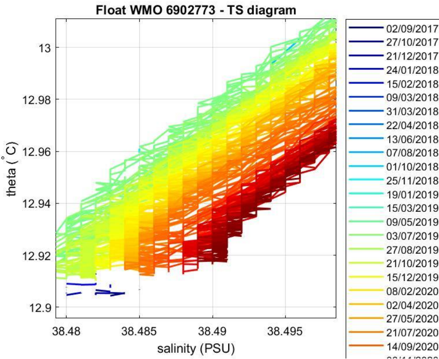
Figure 5: Float 6902773. Area of the \theta -S diagram (color-coded per cycle number) where the \theta -S relationship is more uniform.
