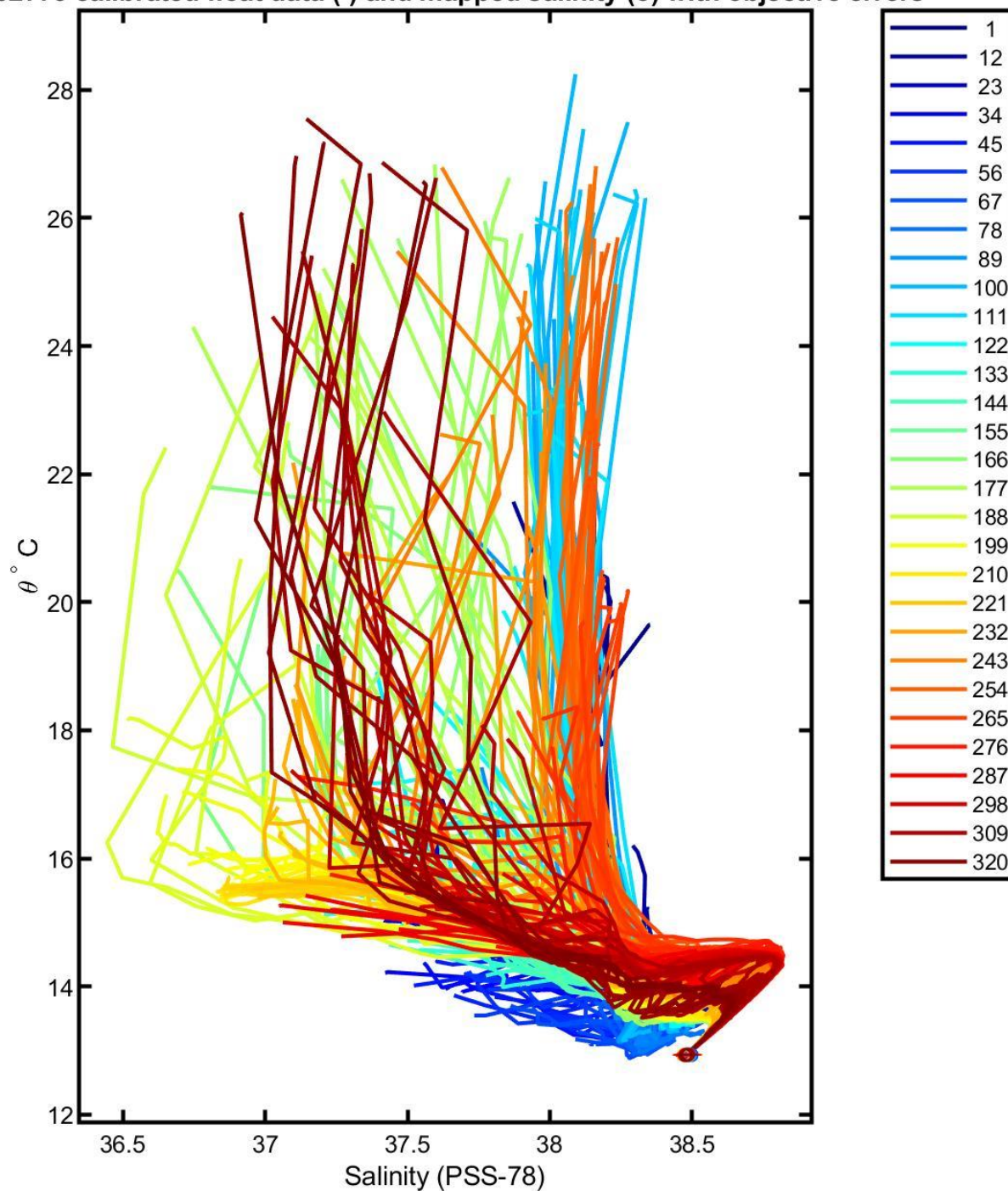
6902773 calibrated float data (-) and mapped salinity (o) with objective errors
