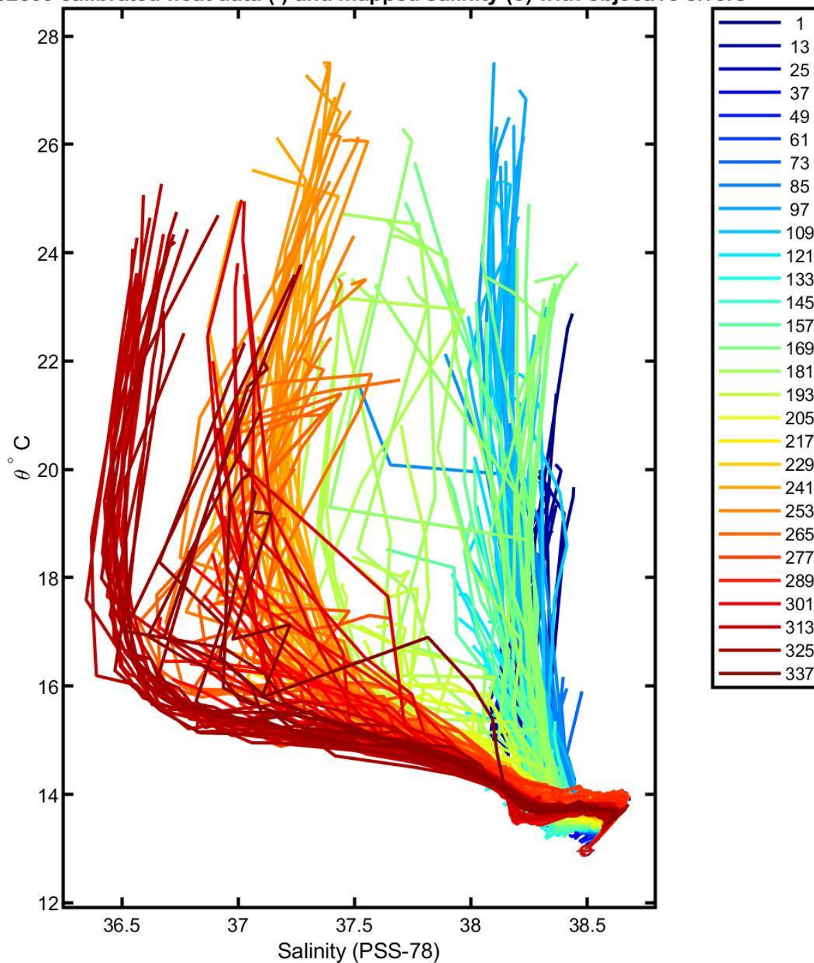
6902803 calibrated float data (-) and mapped salinity (o) with objective errors
