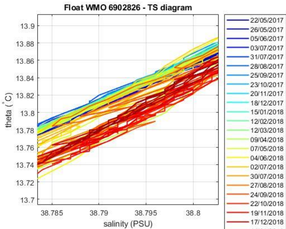
Figure 5: Float 6902826. Area of the \theta -S diagram (color-coded per cycle number) where the \theta -S relationship is more uniform.
