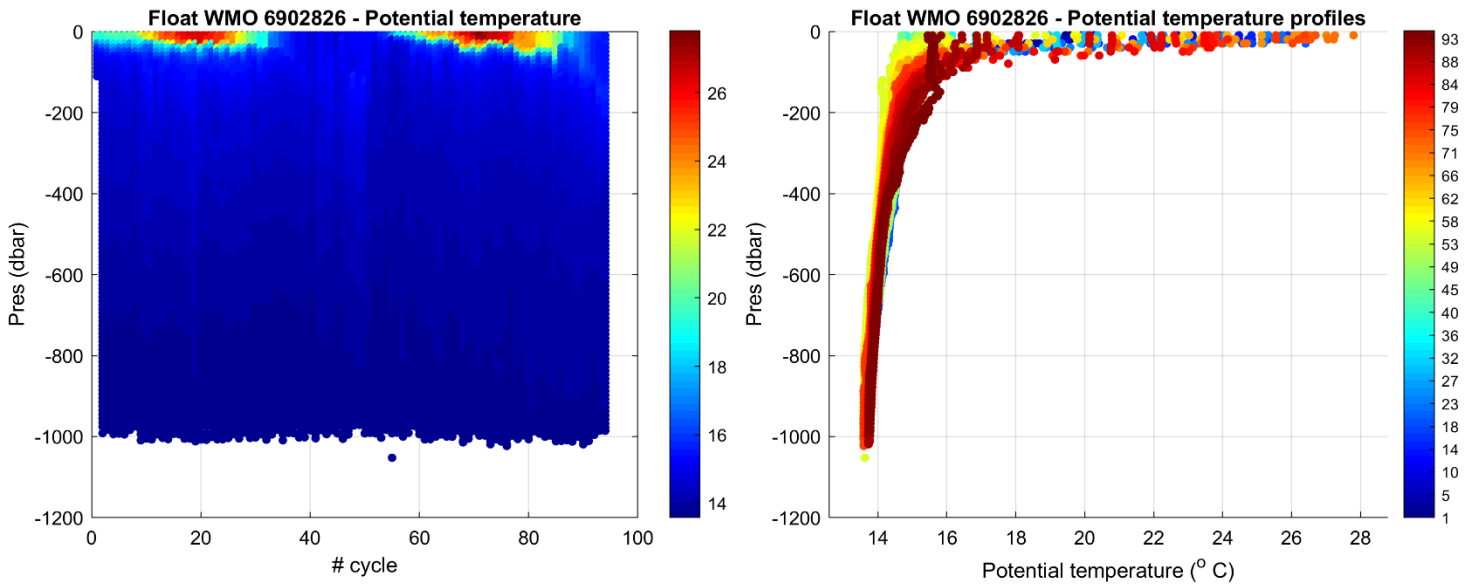
Figure 2: Float 6902826. Time series of Argo float potential temperature ( ^{\circ}\text{C} ) on the left, and potential temperature profiles color-coded per cycle number on the right.
