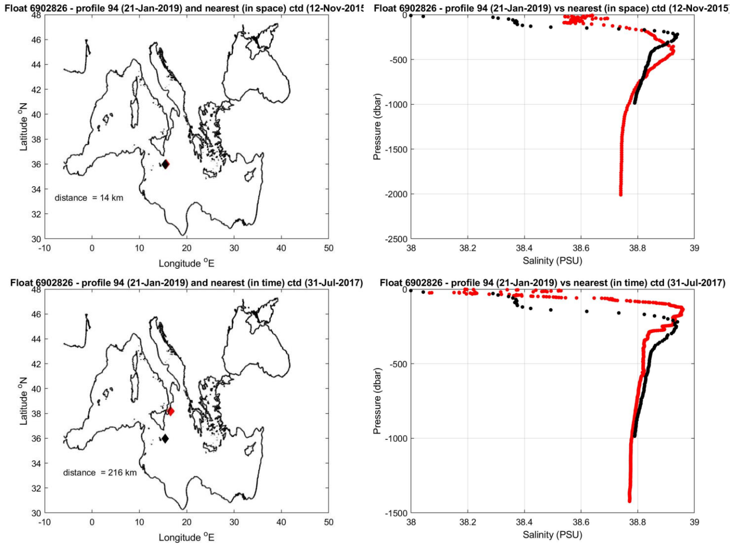
Figure 11: Float 6902826. The salinity float profile number 94 (black dots) are compared to the nearest in space (top) and in time (bottom) reference profile (red dots). The locations of the two profiles and their distance is given in the left panel.
