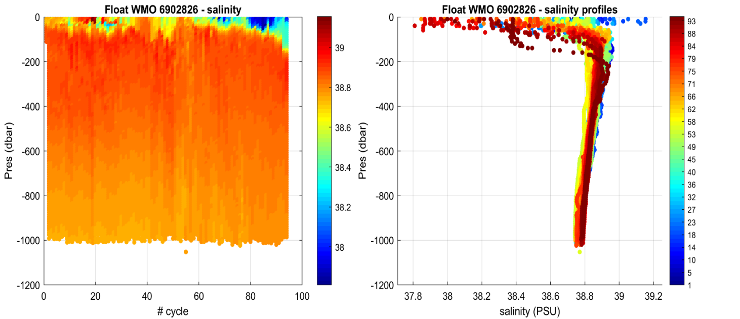
Figure 3: Float 6902826. Time series of Argo float potential salinity (PSS-78) on the left, and salinity profiles color-coded per cycle number on the right.
