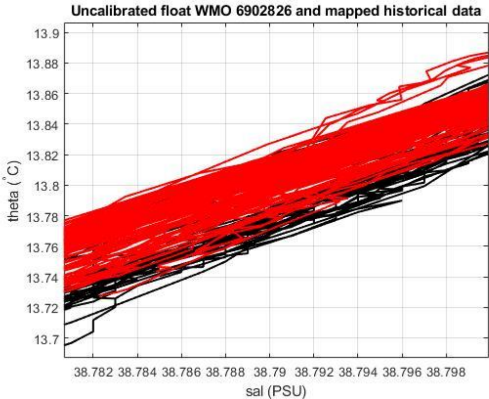
Figure 19: Float 6902826. Uncalibrated float salinity profile (black lines) and mapped historical data (red lines) in the most uniform part of the \theta -S curve.
