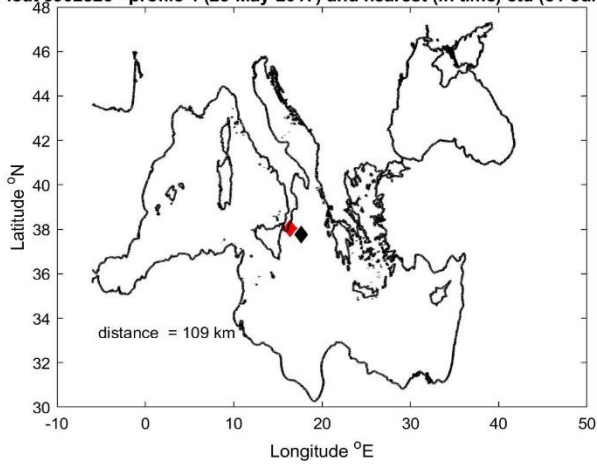
Figure 9: Float 6902826. The salinity float profile number 4 (black dots) are compared to the nearest in space (top) and in time (bottom) reference profile (red dots). The locations of the two profiles and their distance is given in the left panel.
