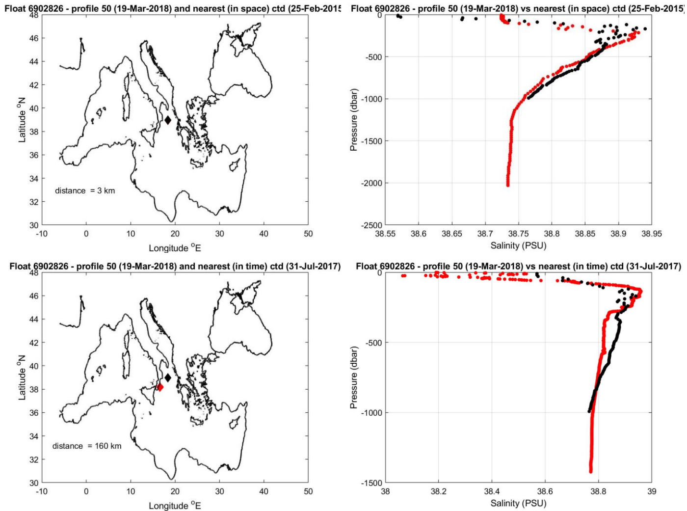
Figure 10: Float 6902826. The salinity float profile number 50 (black dots) are compared to the nearest in space (top) and in time (bottom) reference profile (red dots). The locations of the two profiles and their distance is given in the left panel.
