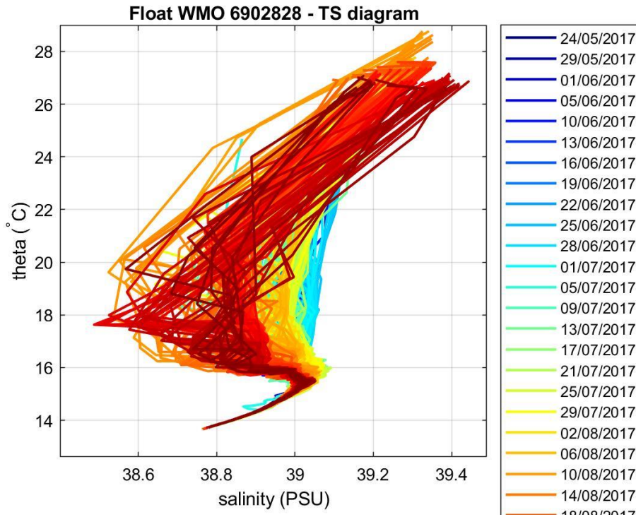
Figure 4: Float 6902828. \theta -S diagram color-coded per cycle number.
