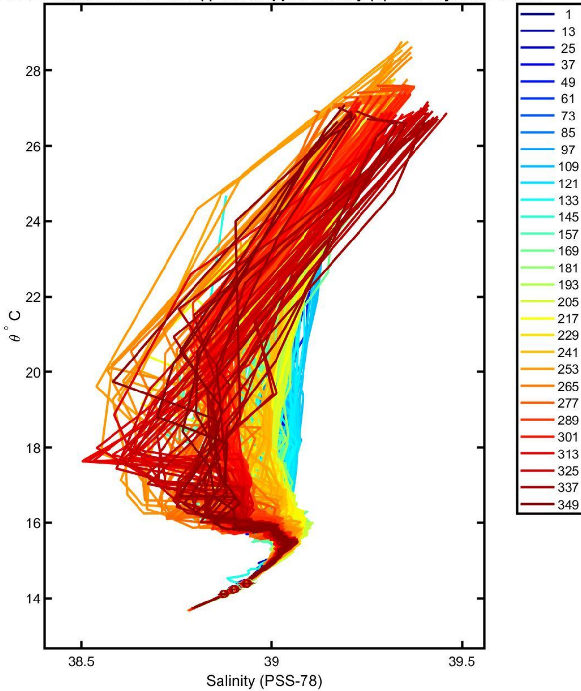
6902828 calibrated float data (-) and mapped salinity (o) with objective errors
