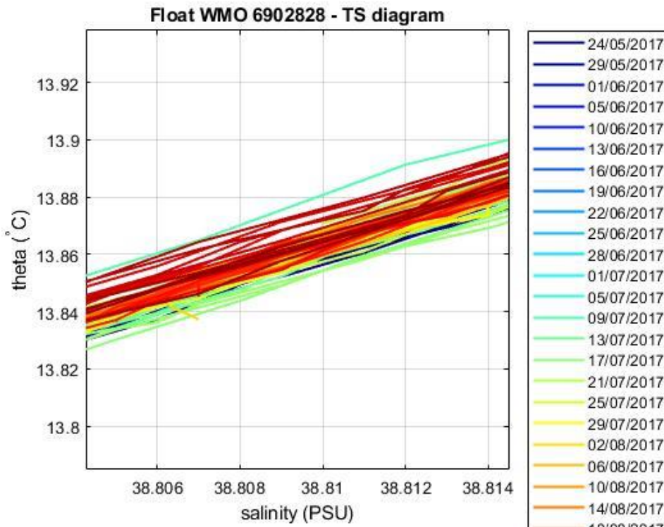
Figure 5: Float 6902828. Area of the \theta -S diagram (color-coded per cycle number) where the \theta -S relationship is more uniform.
