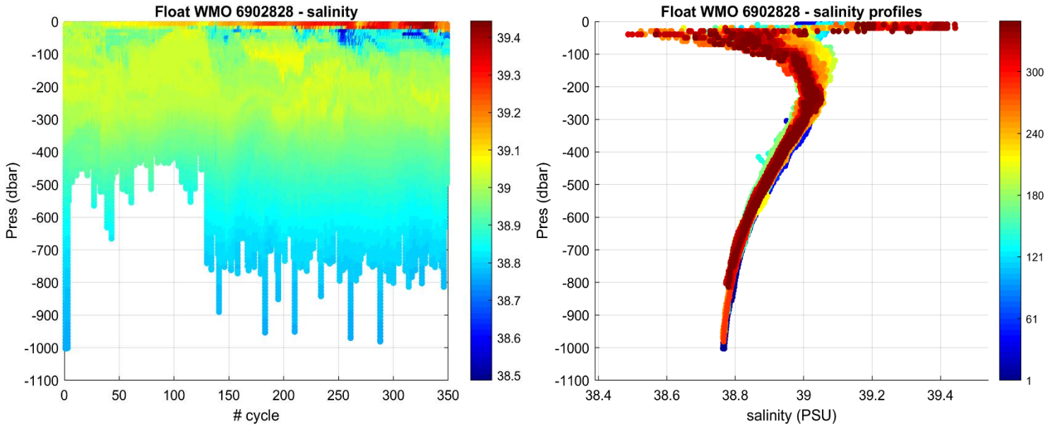
Figure 3: Float 6902828. Time series of Argo float potential salinity (PSS-78) on the left, and salinity profiles color-coded per cycle number on the right.
