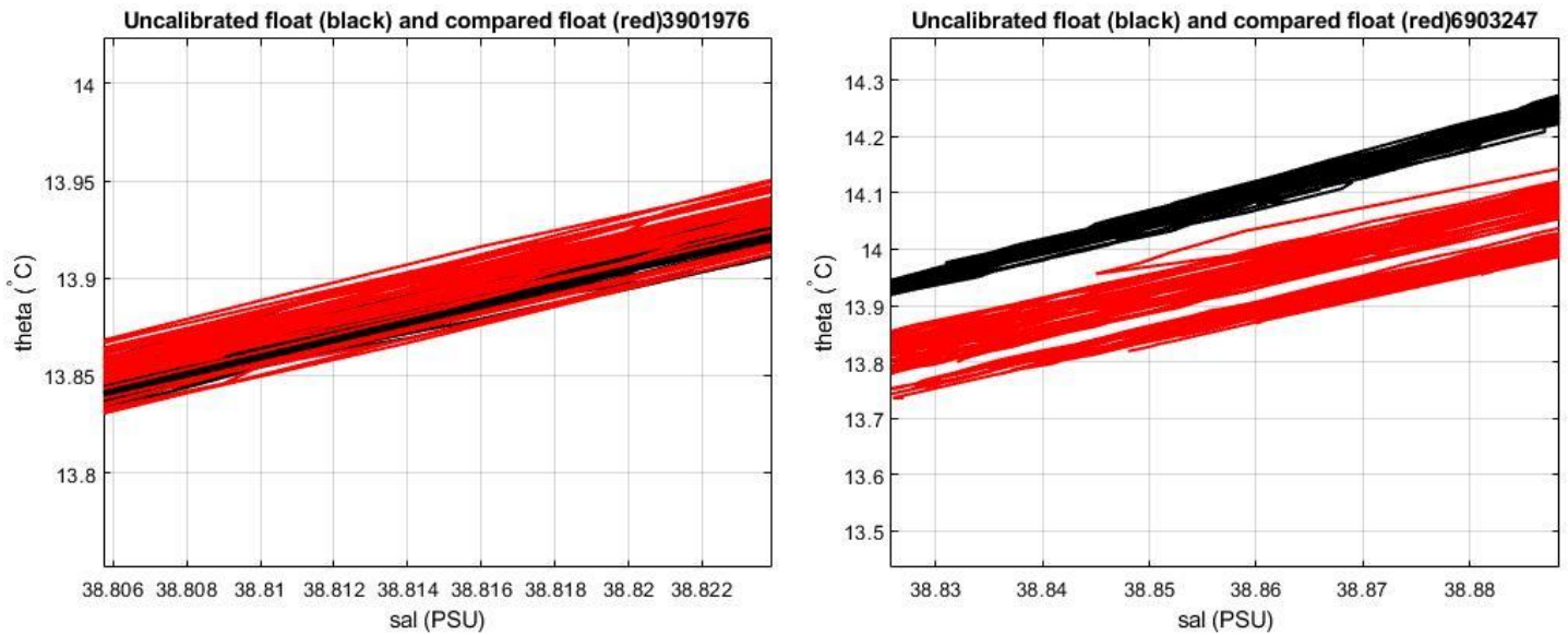
Figure 21: Float 6902828. Comparison between float 6902828 (black line) and other floats (red line), in the most uniform part of the \theta -S curve.
