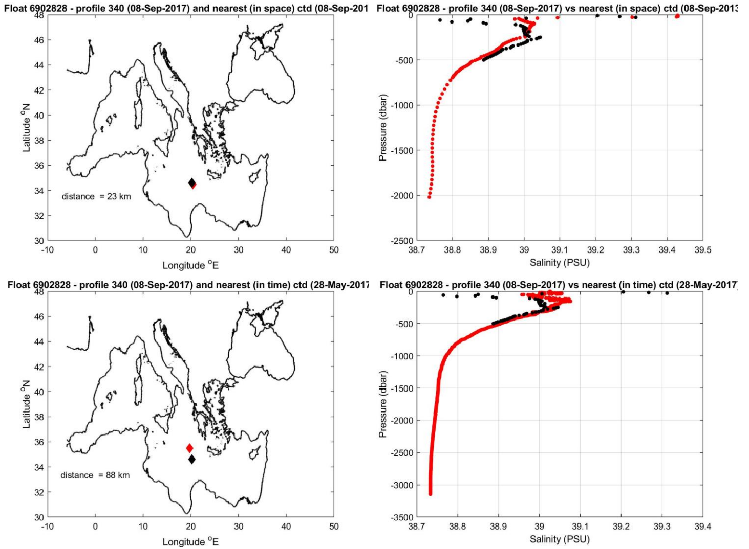
Figure 11: Float 6902828. The salinity float profile number 340 (black dots) are compared to the nearest in space (top) and in time (bottom) reference profile (red dots). The locations of the two profiles and their distance is given in the left panel.
