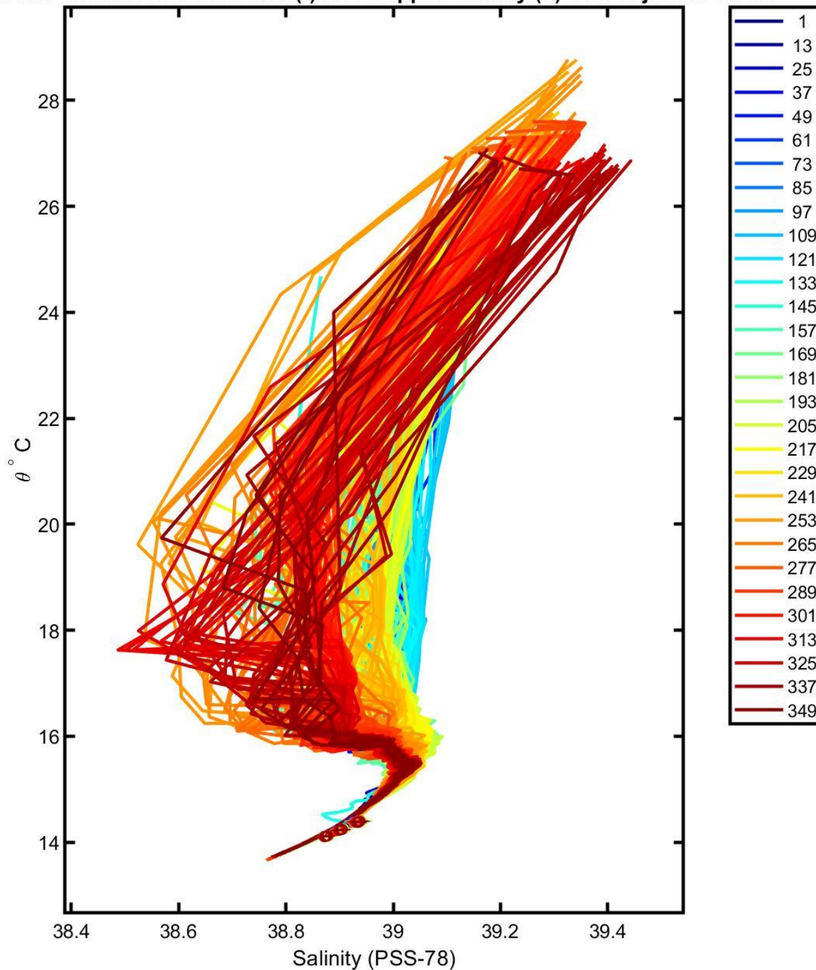
6902828 uncalibrated float data (-) and mapped salinity (o) with objective errors
