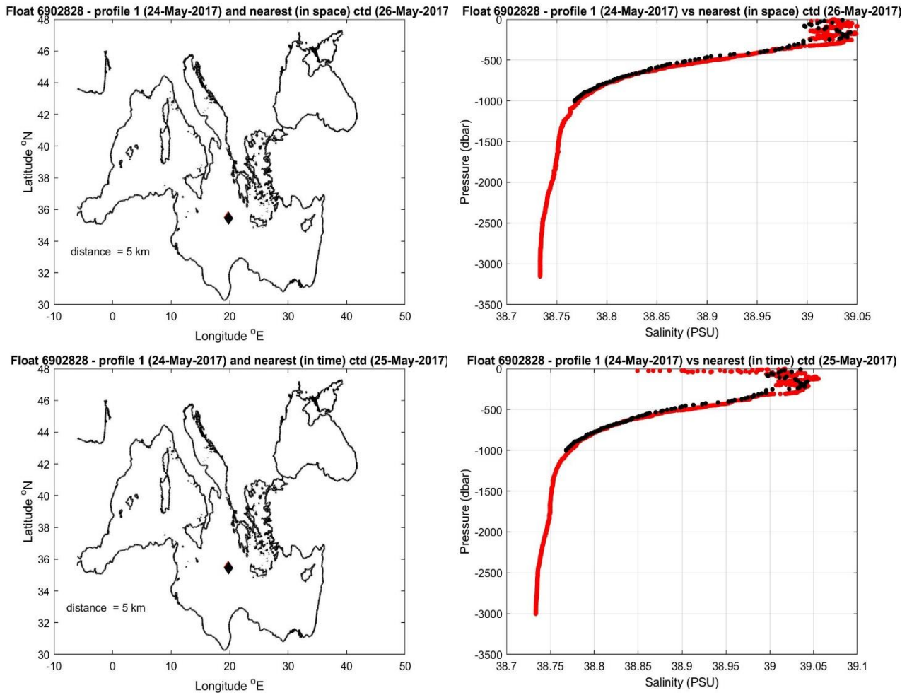
Figure 9: Float 6902828. The salinity float profile number 1 (black dots) are compared to the nearest in space (top) and in time (bottom) reference profile (red dots). The locations of the two profiles and their distance is given in the left panel.
