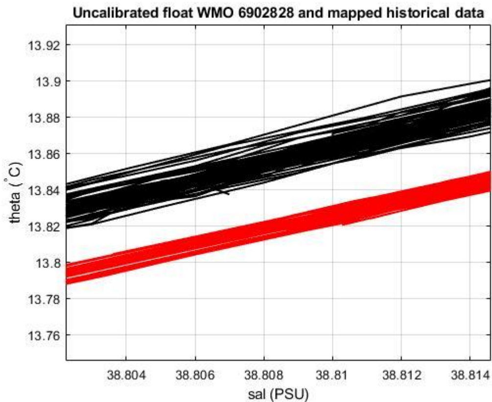
Figure 19: Float 6902828. Uncalibrated float salinity profile (black lines) and mapped historical data (red lines) in the most uniform part of the \theta -S curve.
