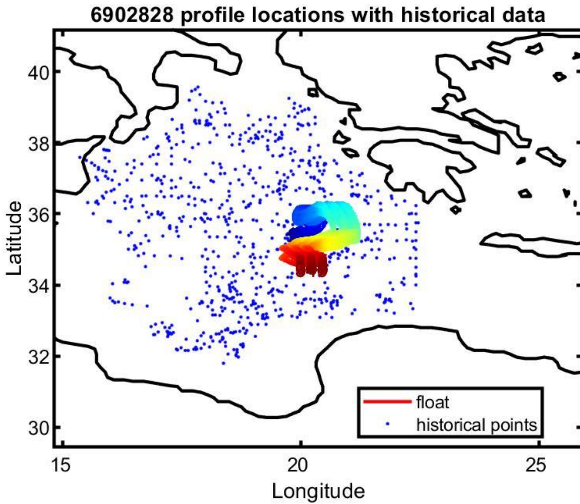
Figure 13: Float 6902828. Location of the float profiles (red line with colored numbers) and the reference data selected for mapping (blue dots).
