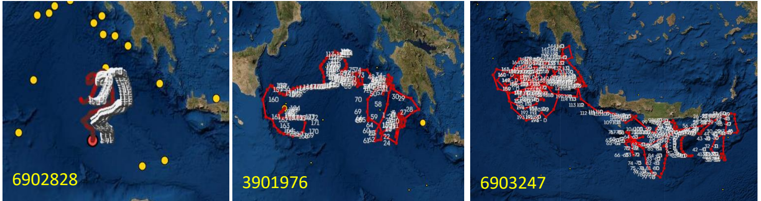
Figure 20: Float 6902828. Trajectory of the floats used for the comparison.
