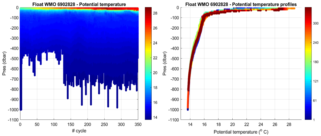
Figure 2: Float 6902828. Time series of Argo float potential temperature ( ^{\circ}\text{C} ) on the left, and potential temperature profiles color-coded per cycle number on the right.
