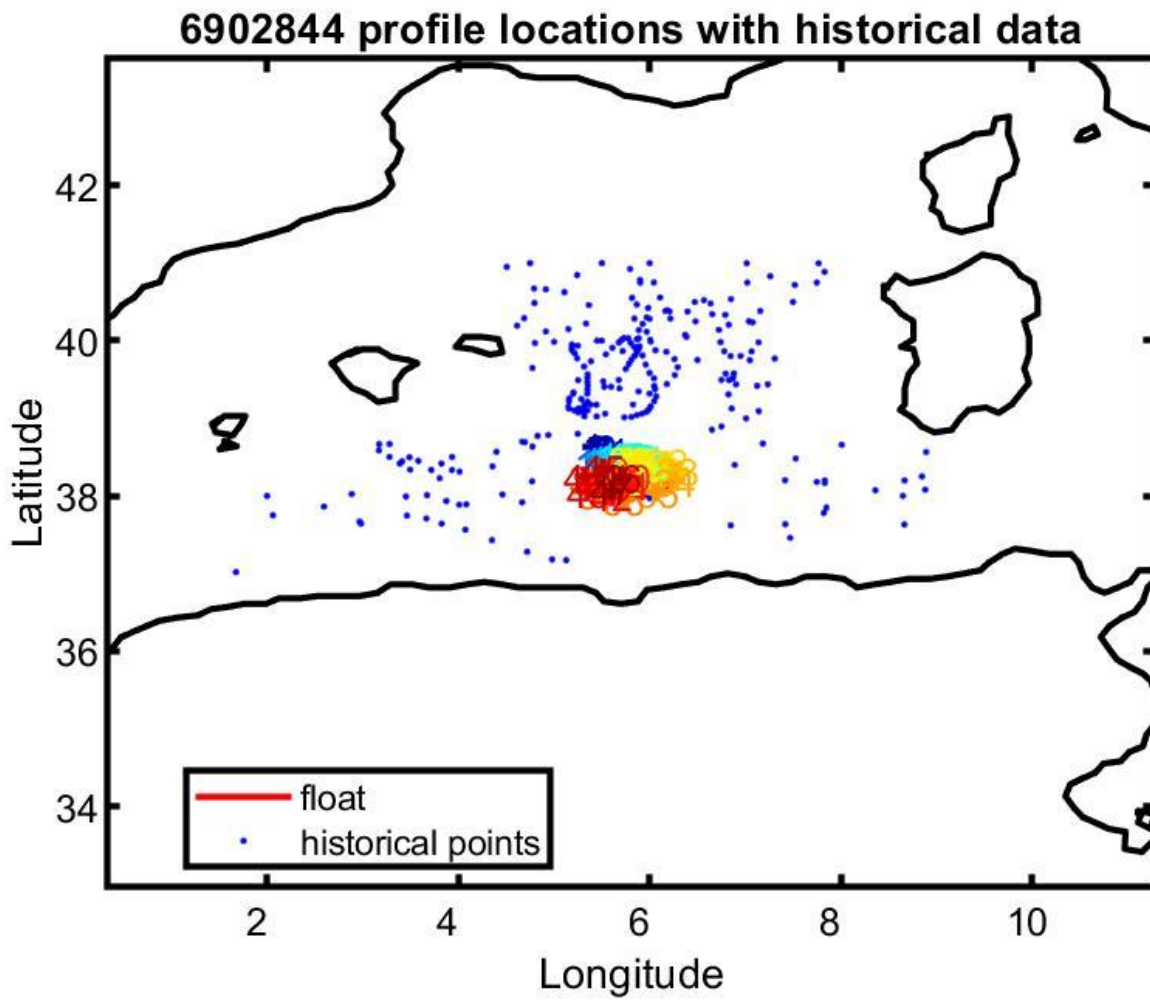
Figure 13: Float 6902844. Location of the float profiles (red line with colored numbers) and the reference data selected for mapping (blue dots).
