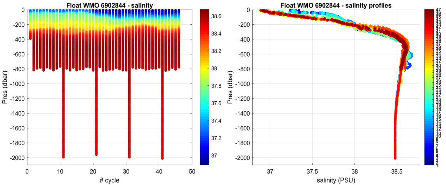
Figure 3: Float 6902844. Time series of Argo float potential salinity (PSS-78) on the left, and salinity profiles color-coded per cycle number on the right.
