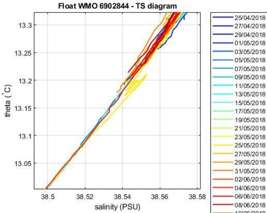
Figure 5: Float 6902844. Area of the \theta -S diagram (color-coded per cycle number) where the \theta -S relationship is more uniform.
