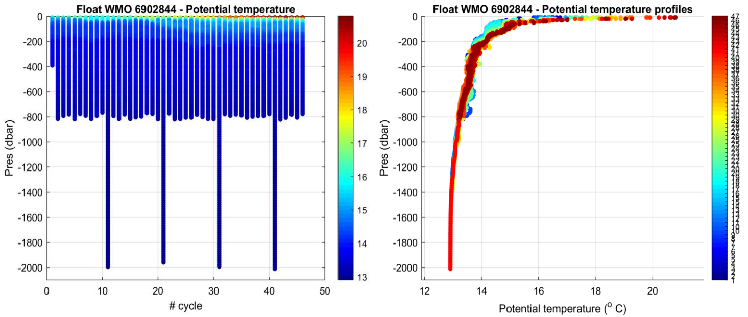
Figure 2: Float 6902844. Time series of Argo float potential temperature ( ^{\circ}\text{C} ) on the left, and potential temperature profiles color-coded per cycle number on the right.
