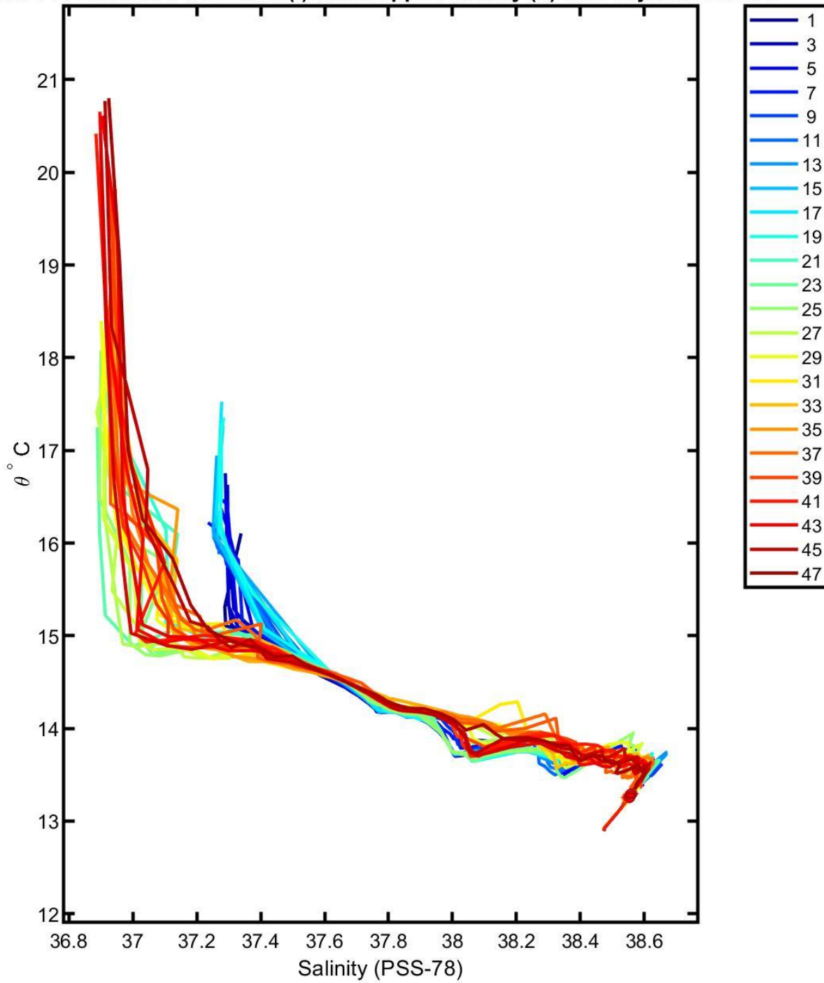
6902844 calibrated float data (-) and mapped salinity (o) with objective errors
