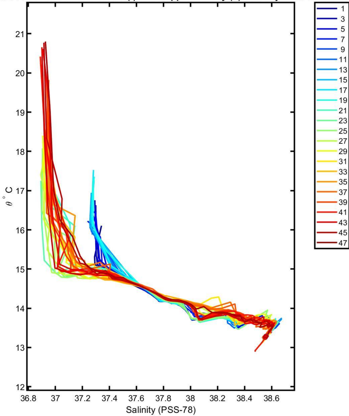
6902844 uncalibrated float data (-) and mapped salinity (o) with objective errors
