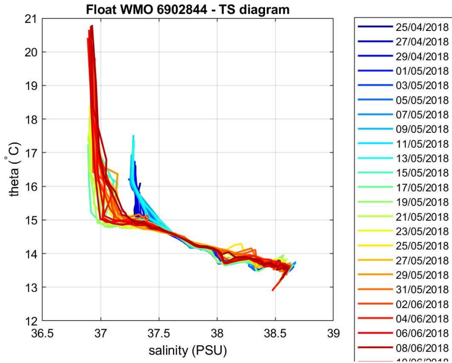
Figure 4: Float 6902844. \theta -S diagram color-coded per cycle number.
