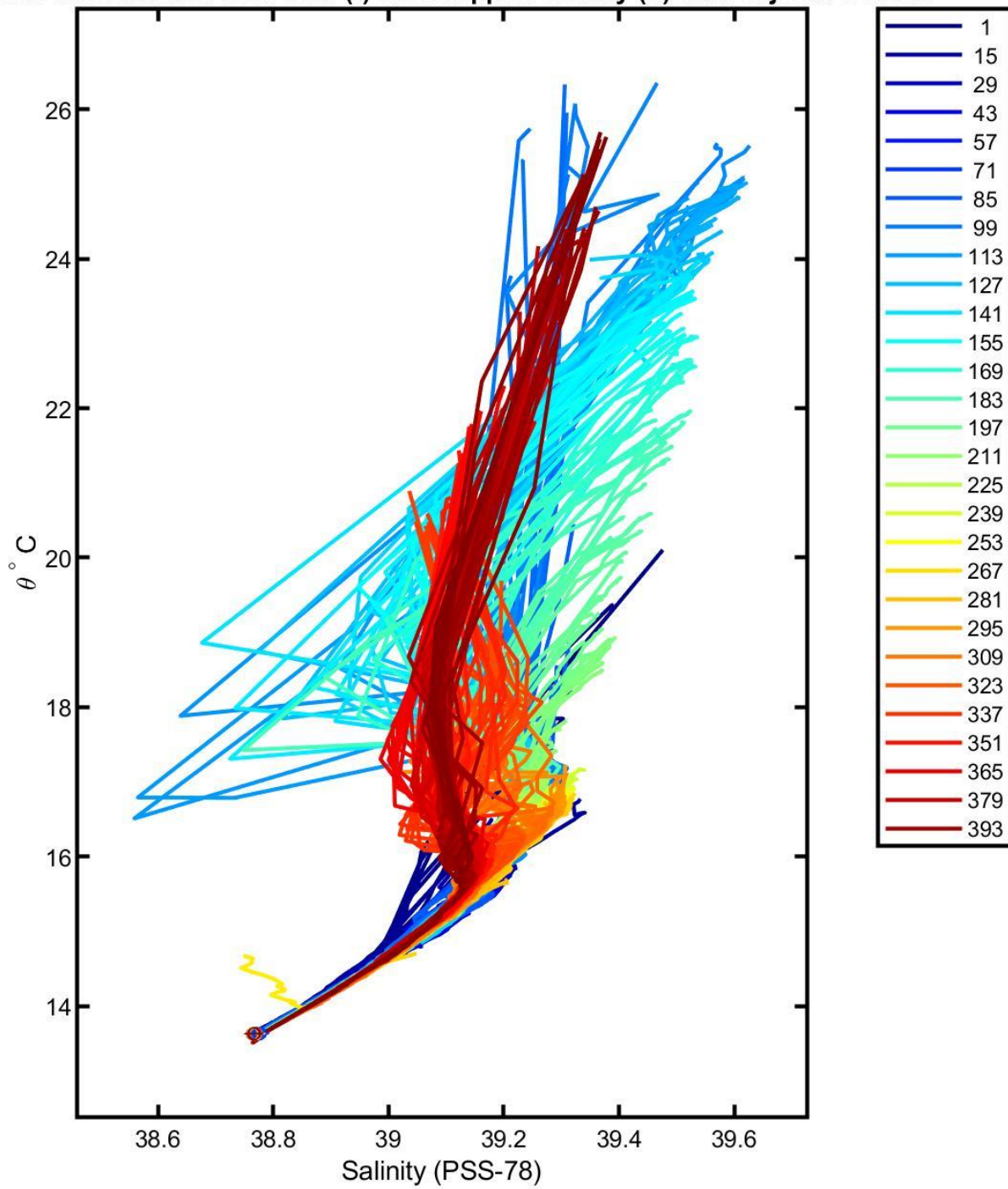
3902847 uncalibrated float data (-) and mapped salinity (o) with objective errors
