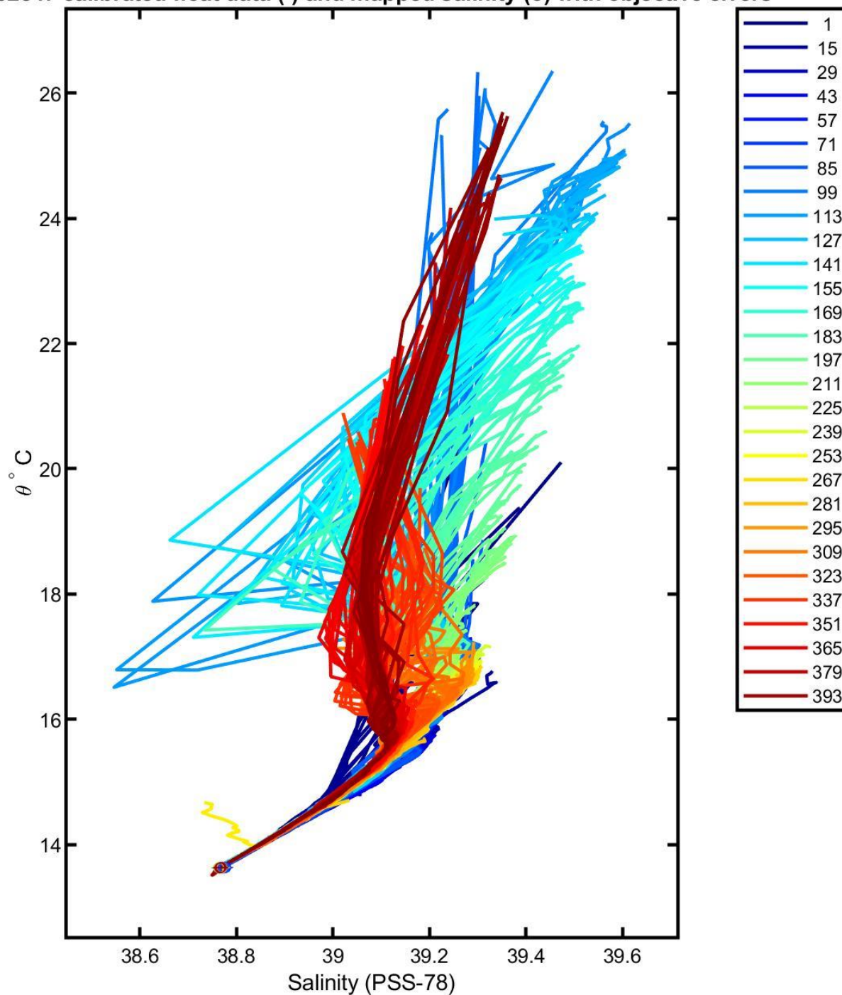
6902847 calibrated float data (-) and mapped salinity (o) with objective errors
