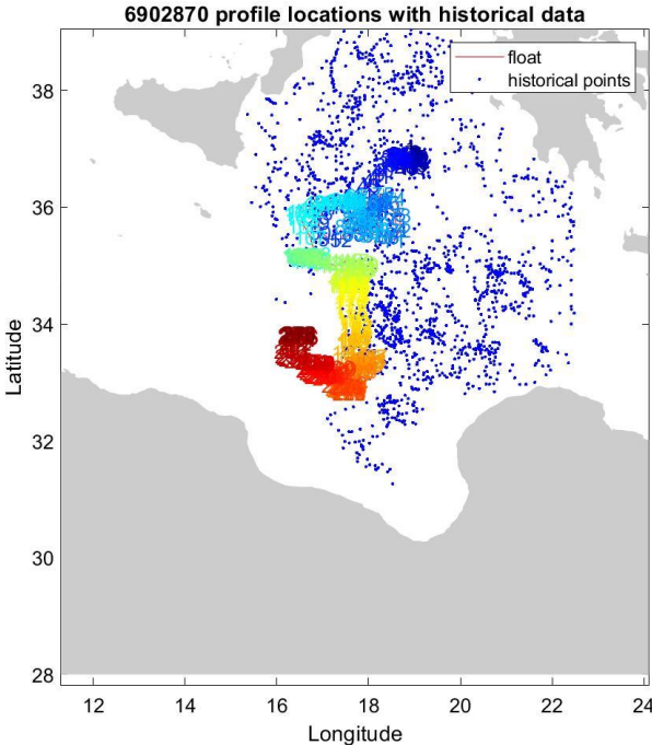
Figure 1: Location of the float profiles (red line with colored numbers) and the reference data selected for mapping (blue dots).
