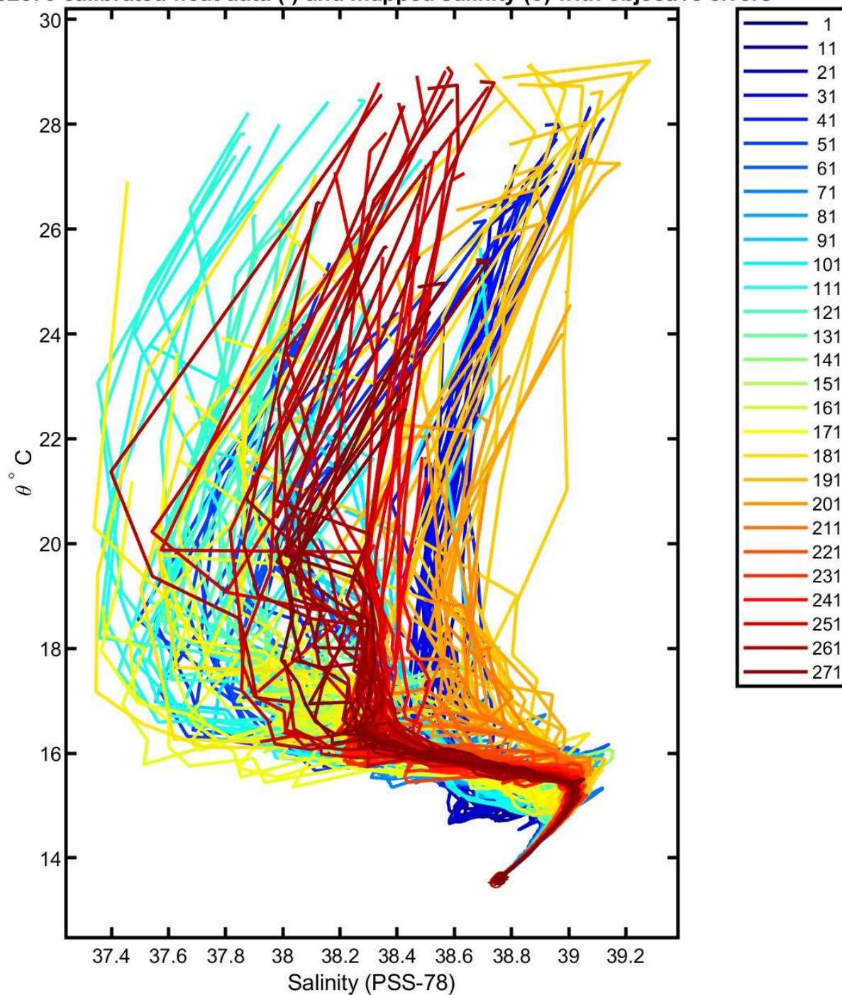
6902870 calibrated float data (-) and mapped salinity (o) with objective errors
