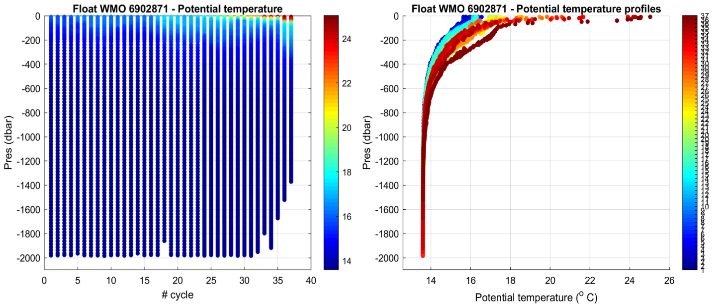
Figure 2: Float 6902871. Time series of Argo float potential temperature ( ^{\circ}\text{C} ) on the left, and potential temperature profiles color-coded per cycle number on the right.
