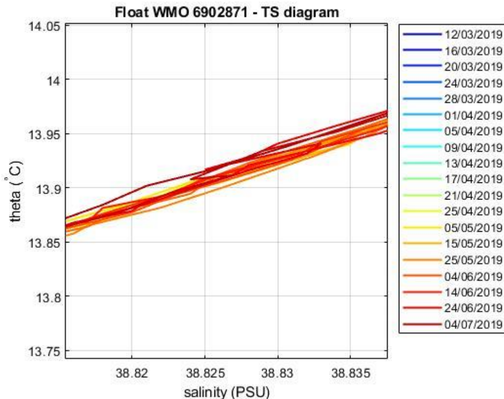
Figure 5: Float 6902871. Area of the \theta -S diagram (color-coded per cycle number) where the \theta -S relationship is more uniform.
