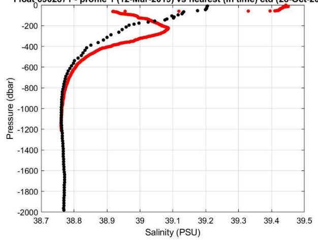
Figure 9: Float 6902871. The salinity float profile number 1 (black dots) are compared to the nearest in space (top) and in time (bottom) reference profile (red dots). The locations of the two profiles and their distance is given in the left panel.
