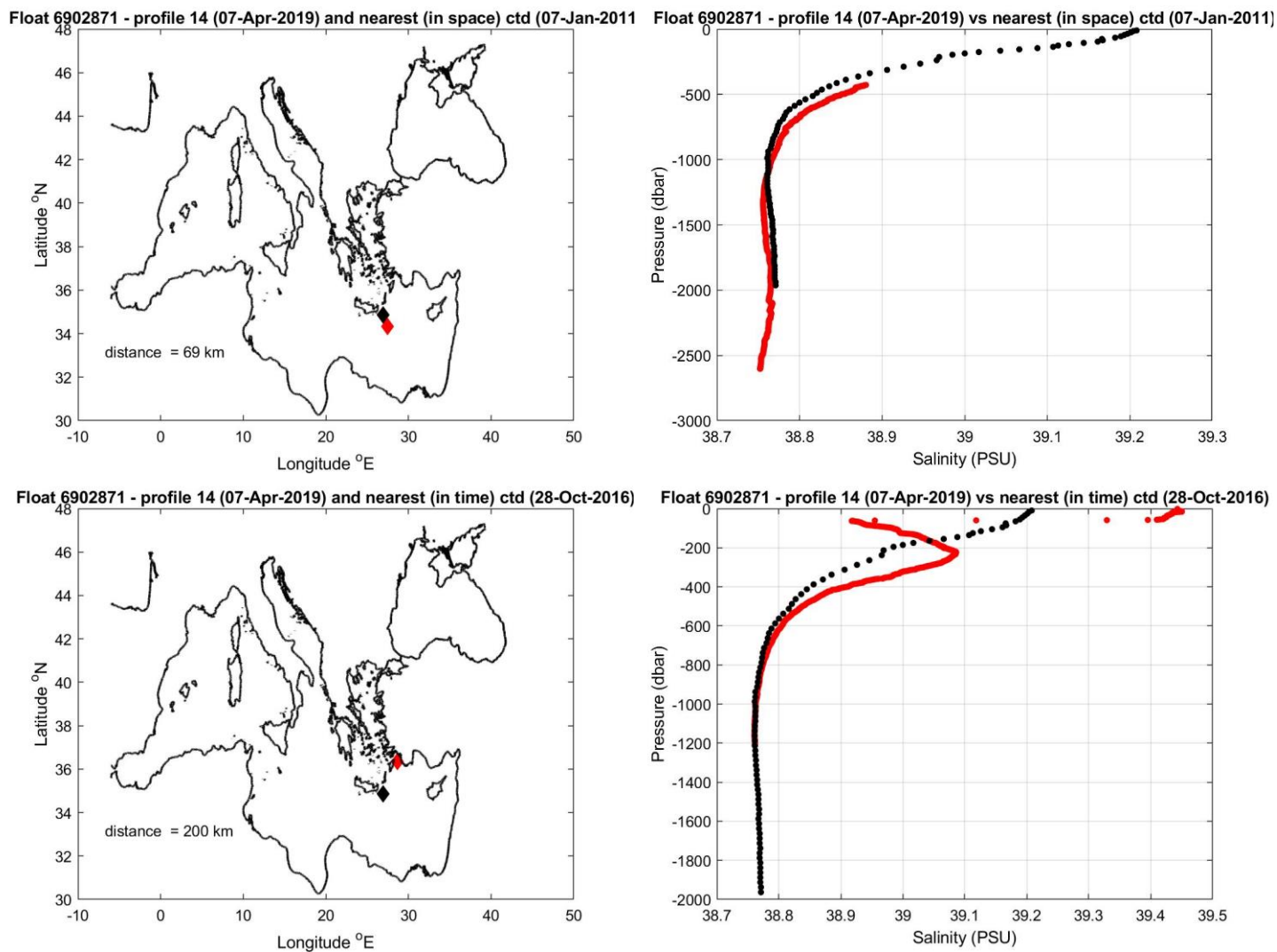
Figure 10: Float 6902871. The salinity float profile number 14 (black dots) are compared to the nearest in space (top) and in time (bottom) reference profile (red dots). The locations of the two profiles and their distance is given in the left panel.
