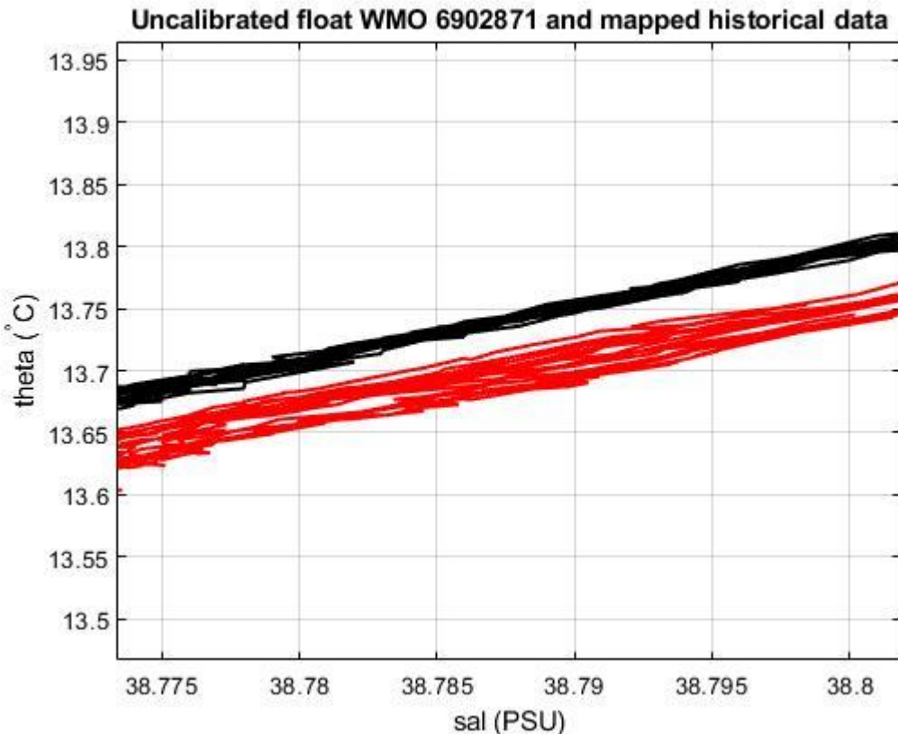
Figure 19: Float 6902871. Uncalibrated float salinity profile (black lines) and mapped historical data (red lines) in the most uniform part of the \theta -S curve.
