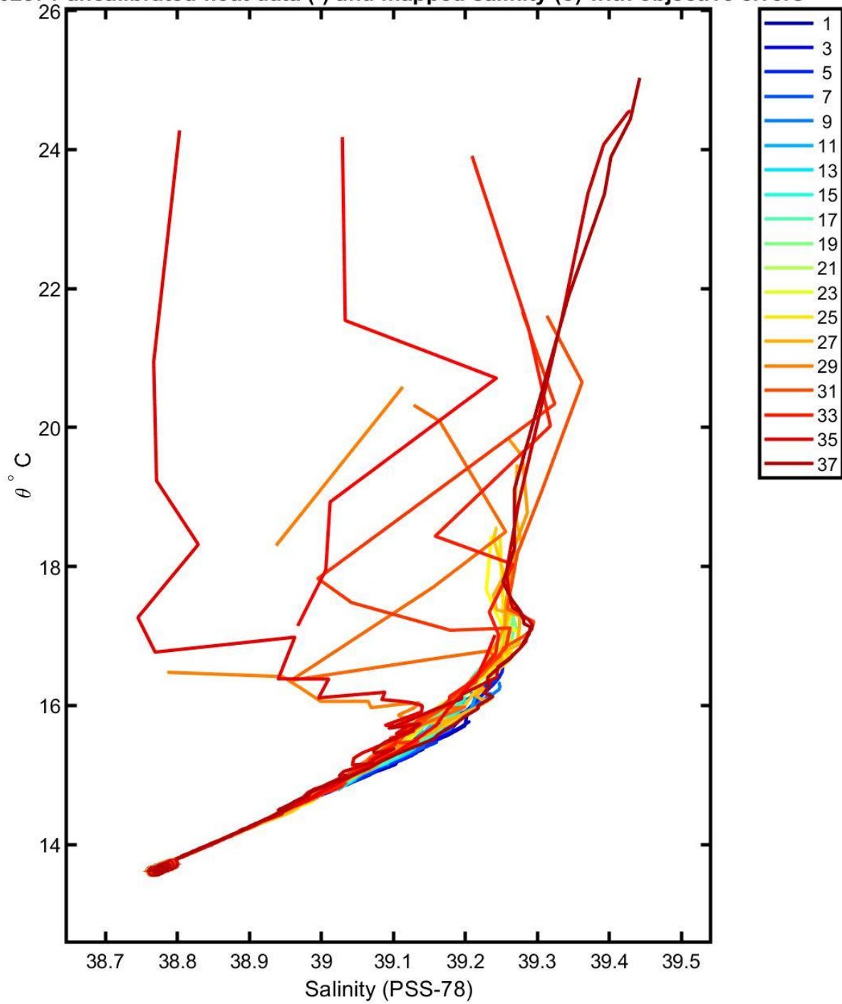
6902871 uncalibrated float data (-) and mapped salinity (o) with objective errors
