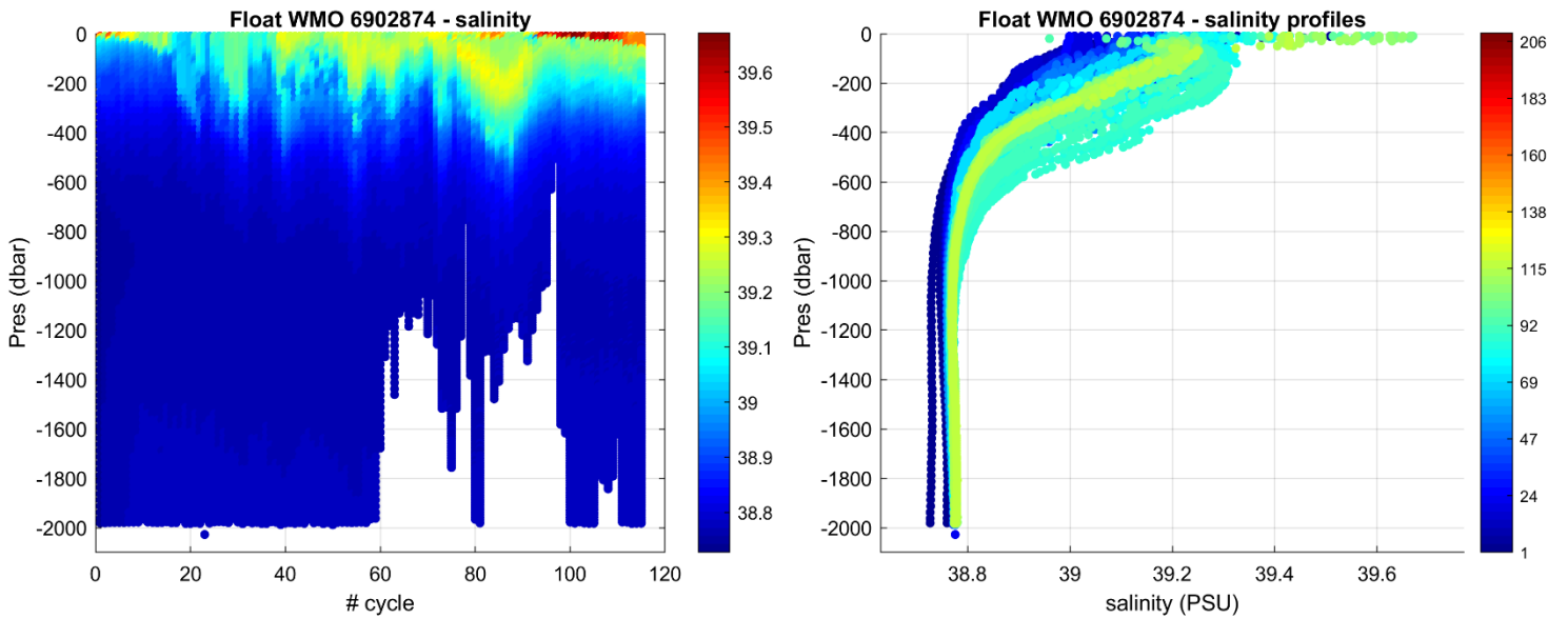
Figure 3: Float 6902874. Time series of Argo float potential salinity (PSS-78) on the left, and salinity profiles color-coded per cycle number on the right.
