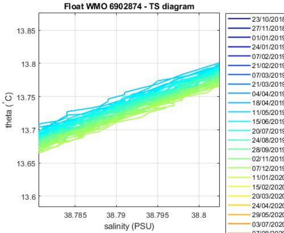
Figure 5: Float 6902874. Area of the \theta -S diagram (color-coded per cycle number) where the \theta -S relationship is more uniform.
