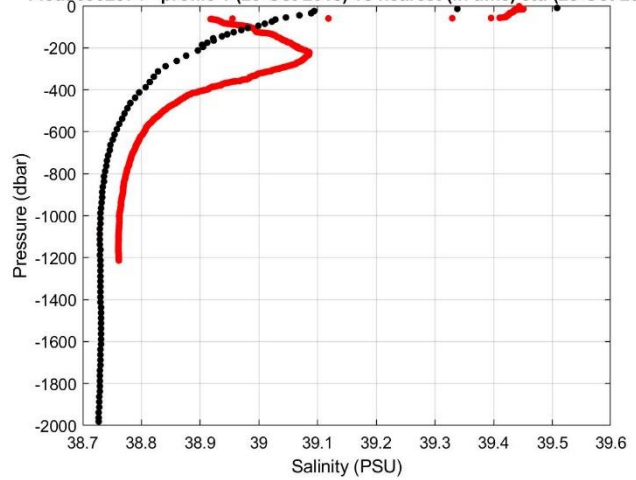
Figure 9: Float 6902874. The salinity float profile number 1 (black dots) are compared to the nearest in space (top) and in time (bottom) reference profile (red dots). The locations of the two profiles and their distance is given in the left panel.
