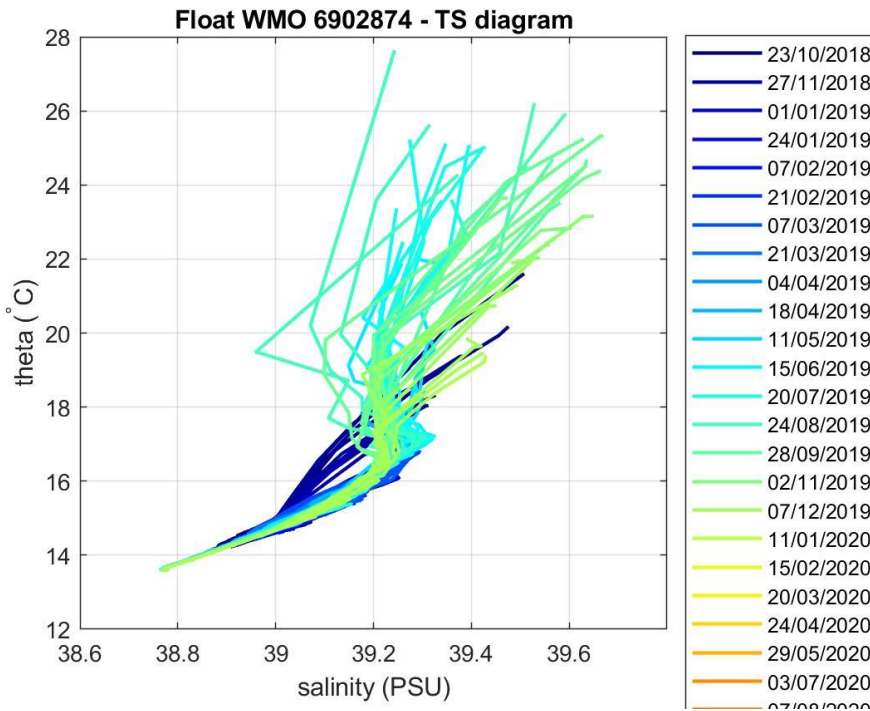
Figure 4: Float 6902874. \theta -S diagram color-coded per cycle number.
