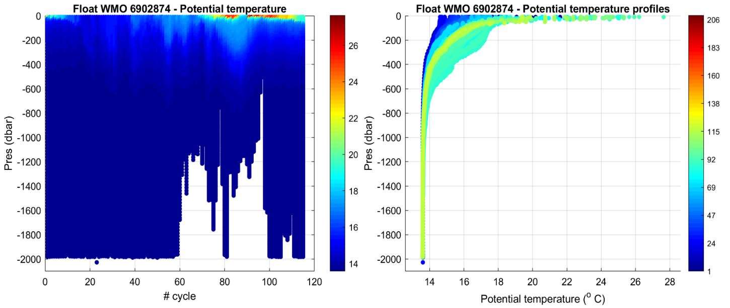
Figure 2: Float 6902874. Time series of Argo float potential temperature ( ^{\circ}\text{C} ) on the left, and potential temperature profiles color-coded per cycle number on the right.
