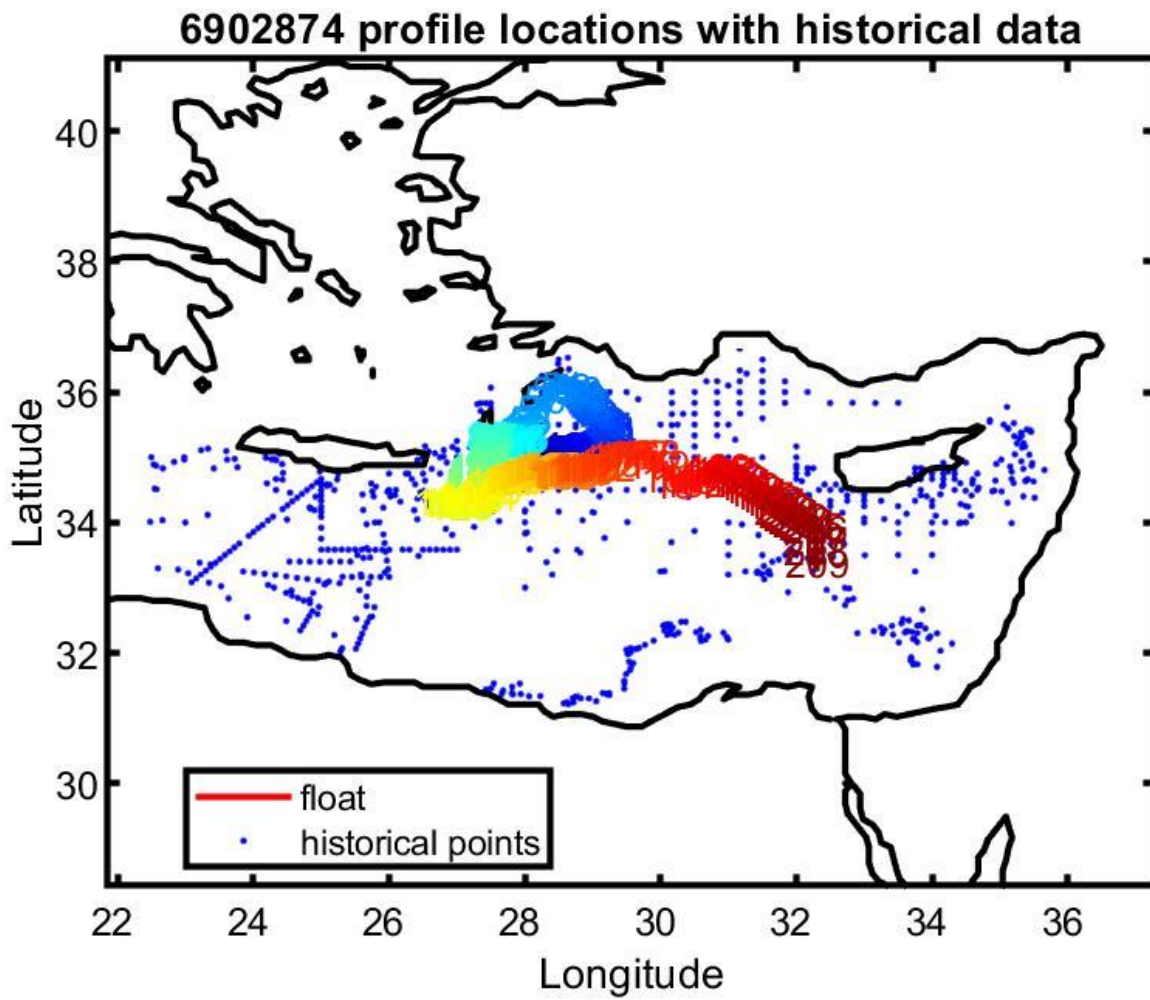
Figure 13: Float 6902874. Location of the float profiles (red line with colored numbers) and the reference data selected for mapping (blue dots).
