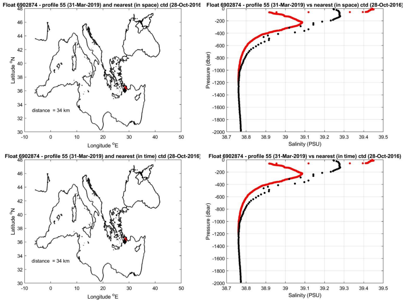
Figure 10: Float 6902874. The salinity float profile number 55 (black dots) are compared to the nearest in space (top) and in time (bottom) reference profile (red dots). The locations of the two profiles and their distance is given in the left panel.
