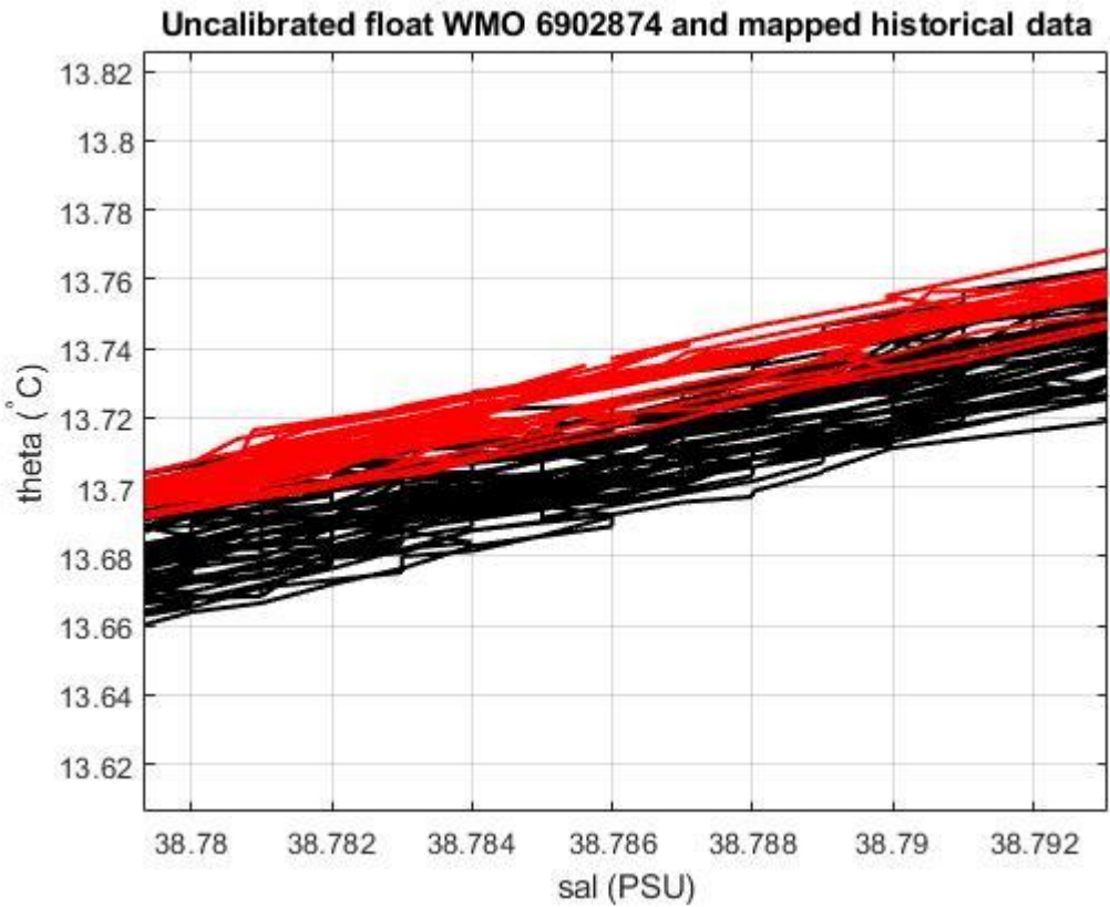
Figure 19: Float 6902874. Uncalibrated float salinity profile (black lines) and mapped historical data (red lines) in the most uniform part of the \theta -S curve.
