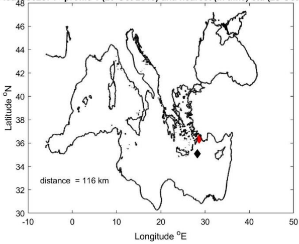
Figure 9: Float 6902874. The salinity float profile number 1 (black dots) are compared to the nearest in space (top) and in time (bottom) reference profile (red dots). The locations of the two profiles and their distance is given in the left panel.
