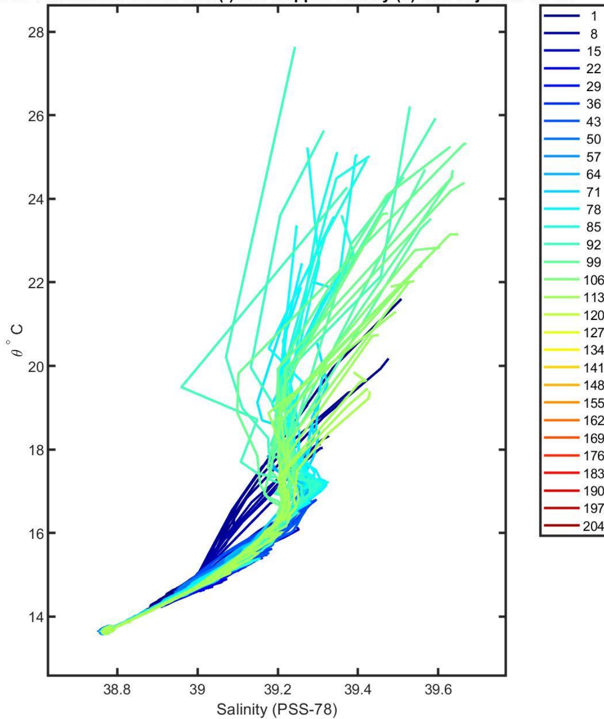
6902874 uncalibrated float data (-) and mapped salinity (o) with objective errors
