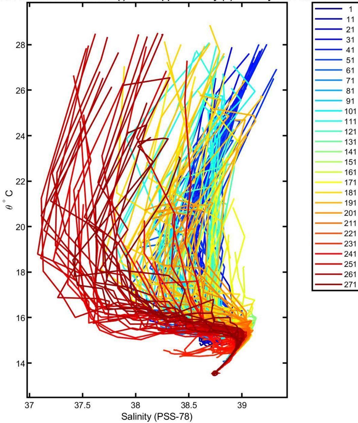
6902875 calibrated float data (-) and mapped salinity (o) with objective errors
