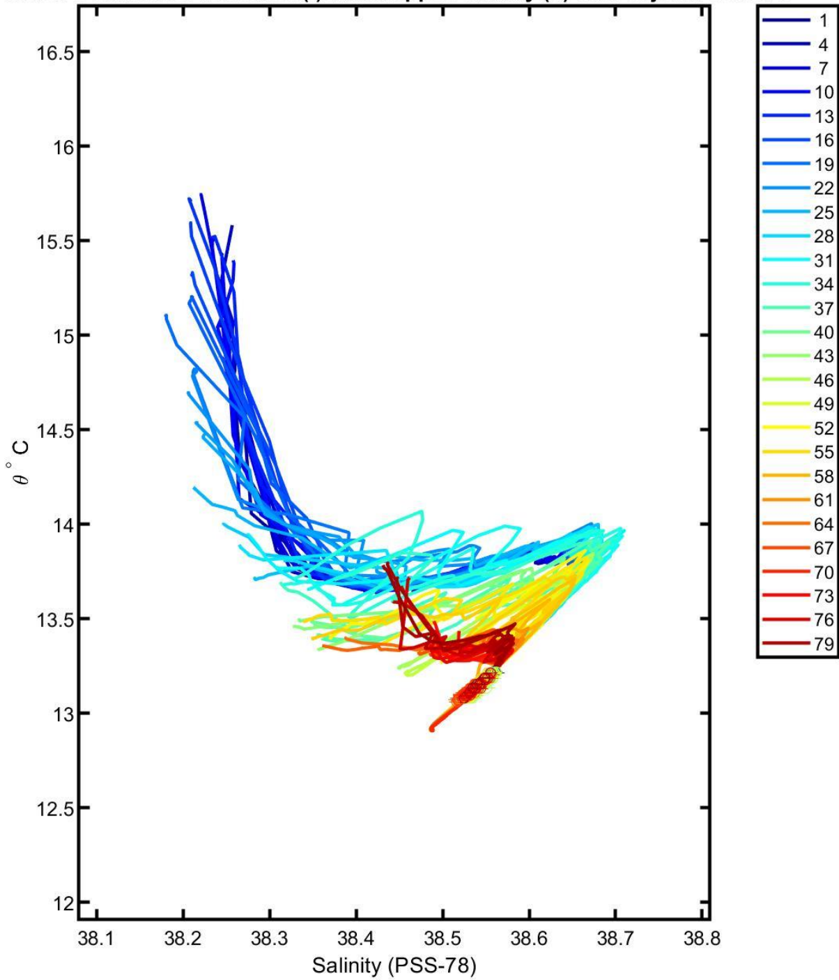
6902879 calibrated float data (-) and mapped salinity (o) with objective errors
