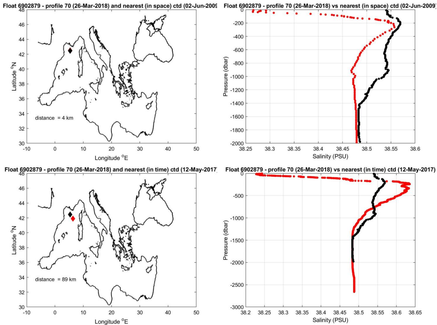
Figure 11: Float 6902879. The salinity float profile number 70 (black dots) are compared to the nearest in space (top) and in time (bottom) reference profile (red dots). The locations of the two profiles and their distance is given in the left panel.
