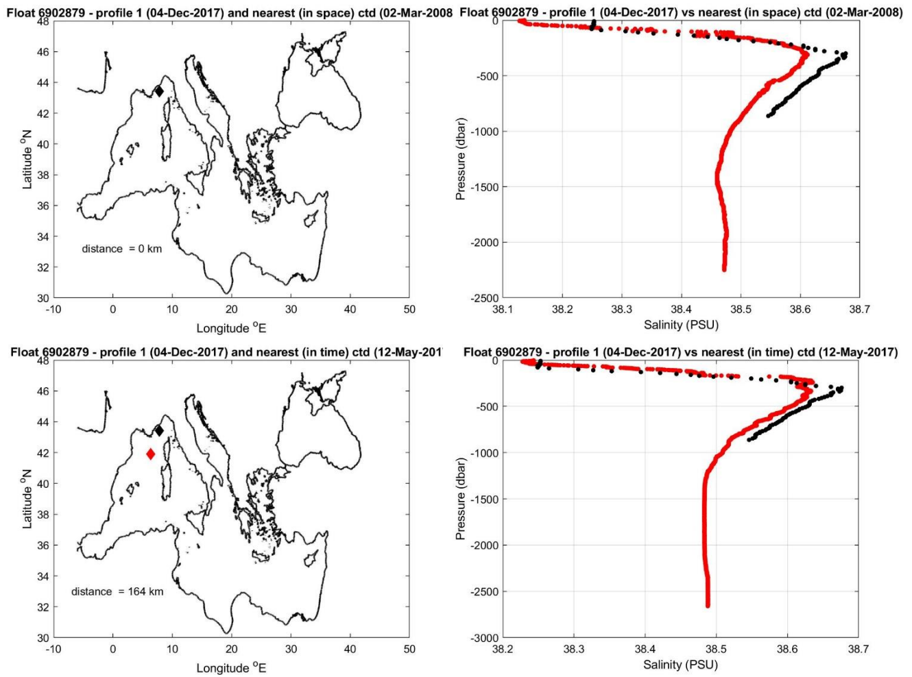
Figure 9: Float 6902879. The salinity float profile number 1 (black dots) are compared to the nearest in space (top) and in time (bottom) reference profile (red dots). The locations of the two profiles and their distance is given in the left panel.
