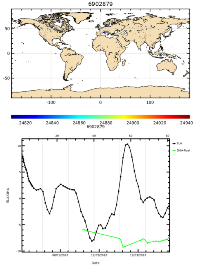
Figure 1: Float 6902879. The comparison between the sea surface height (SSH) from the satellite altimetry and dynamic height anomaly (DHA) extracted from the Argo float temperature and salinity. The figure is created by the CLS/Coriolis and distributed by Ifremer ( ftp://ftp.ifremer.fr/ifremer/argo/etc/argo-ast9-item13-AltimeterComparison/figures/ ).
