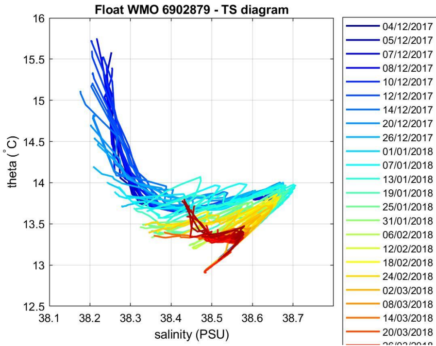
Figure 4: Float 6902879. \theta -S diagram color-coded per cycle number.
