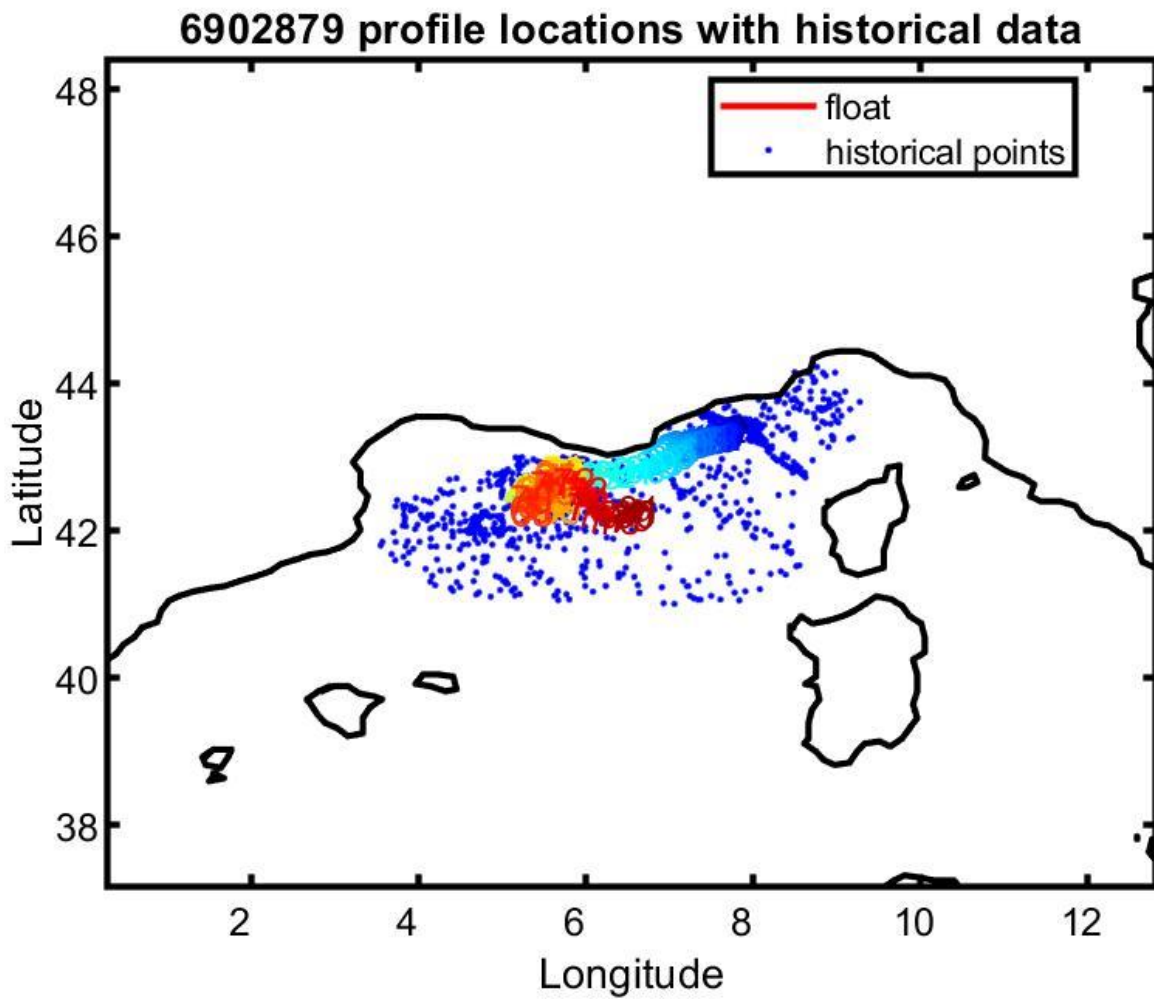
Figure 13: Float 6902879. Location of the float profiles (red line with colored numbers) and the reference data selected for mapping (blue dots).
