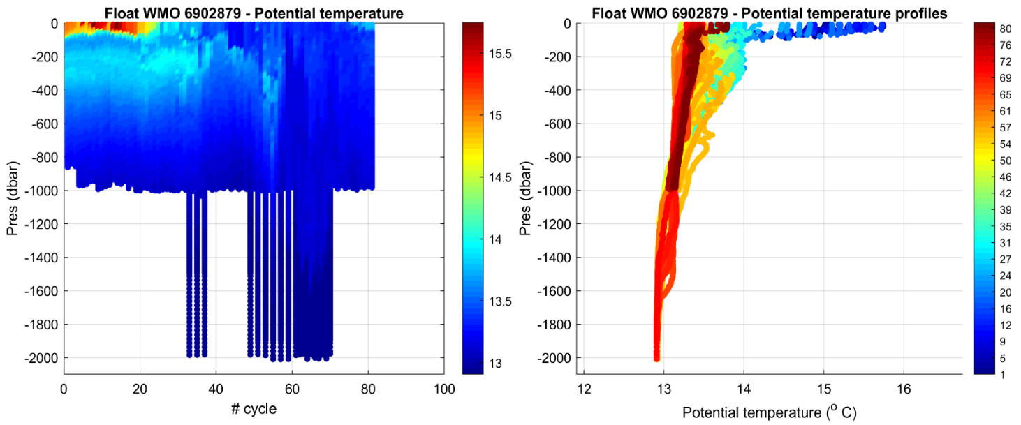
Figure 2: Float 6902879. Time series of Argo float potential temperature ( ^{\circ}\text{C} ) on the left, and potential temperature profiles color-coded per cycle number on the right.
