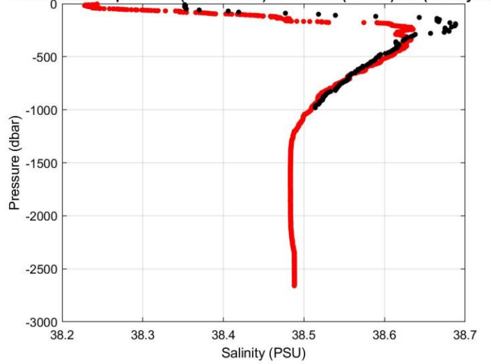
Float 6902879 - profile 38 (21-Jan-2018) vs nearest (in time) ctd (12-May-2017)
