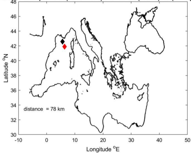
Float 6902879 - profile 38 (21-Jan-2018) and nearest (in time) ctd (12-May-2017)
