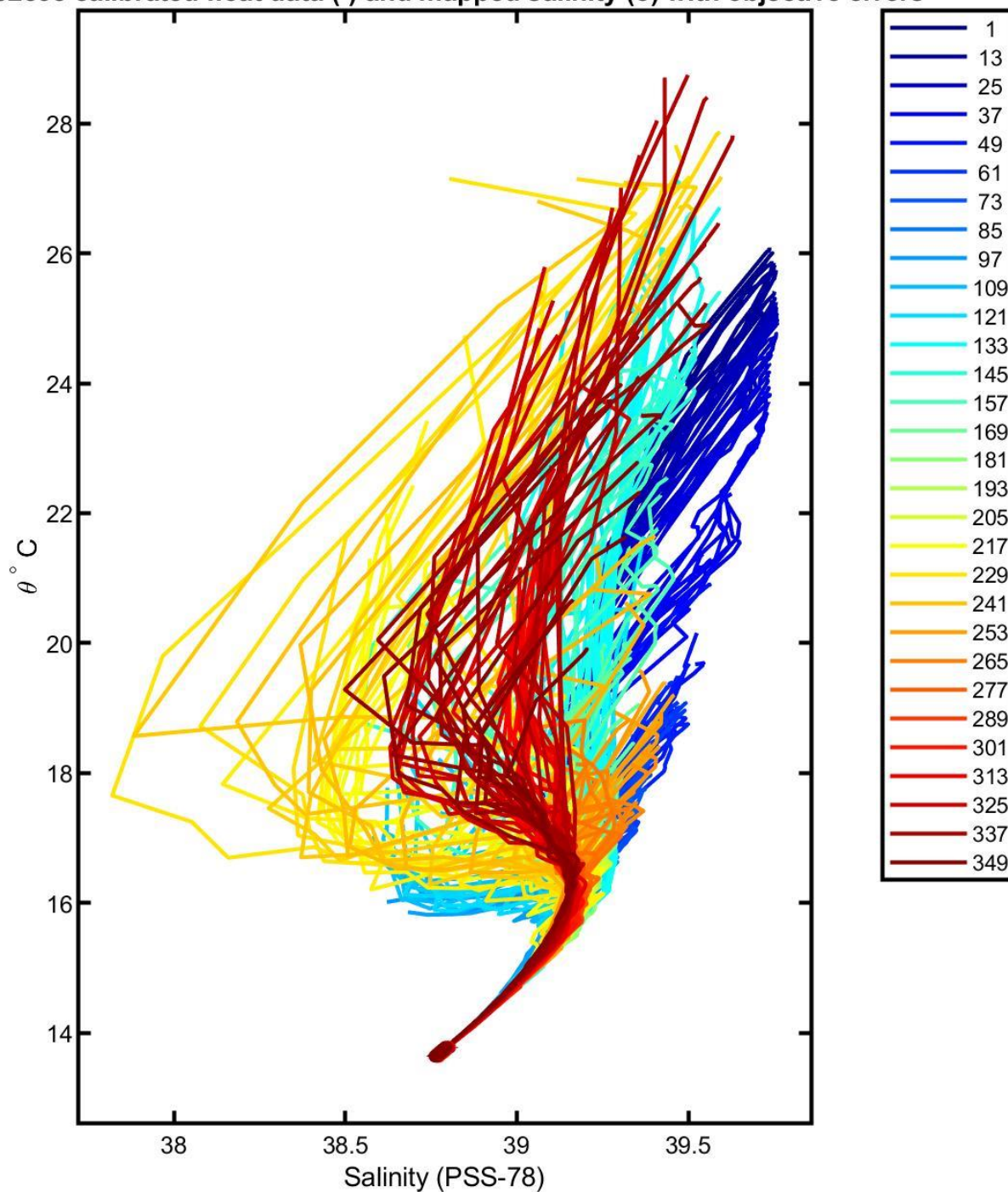
6902898 calibrated float data (-) and mapped salinity (o) with objective errors
