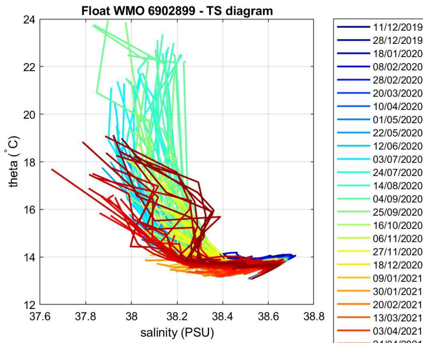
Figure 4: Float 6902899. \theta -S diagram color-coded per cycle number.
