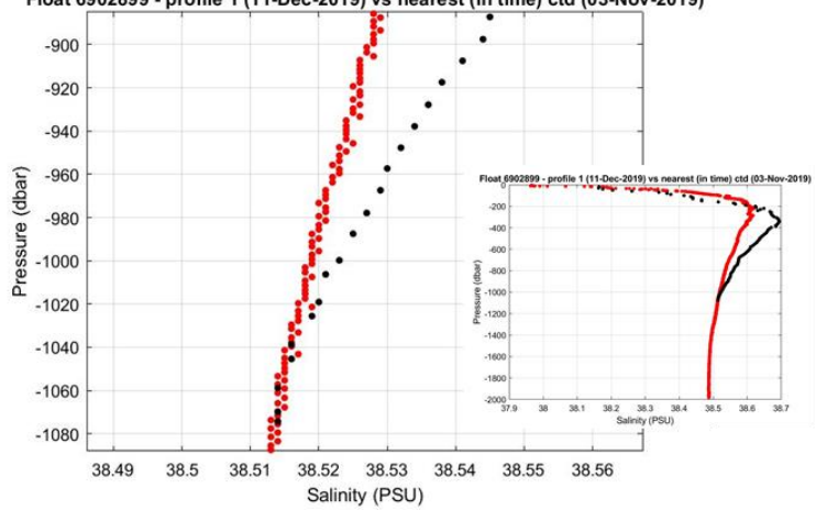
Figure 9: Float 6902899. The salinity float profile number 1 (black dots) are compared to the nearest in space (top) and in time (bottom) reference profile (red dots). The locations of the two profiles and their distance is given in the left panel.
