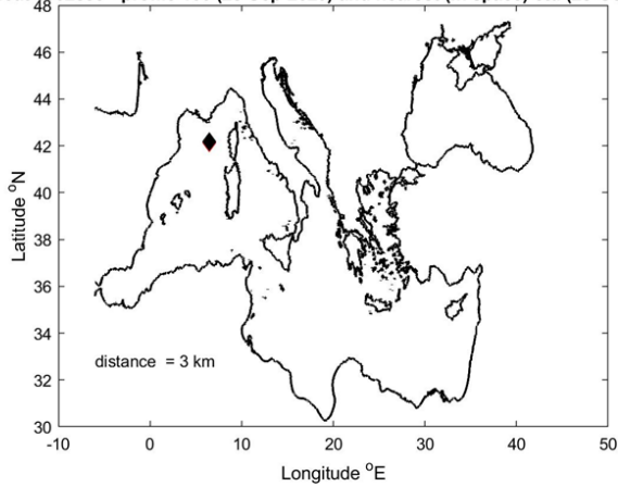
Float 6902899 - profile 100 (28-Sep-2020) and nearest (in time) ctd (28-Sep-2020)
