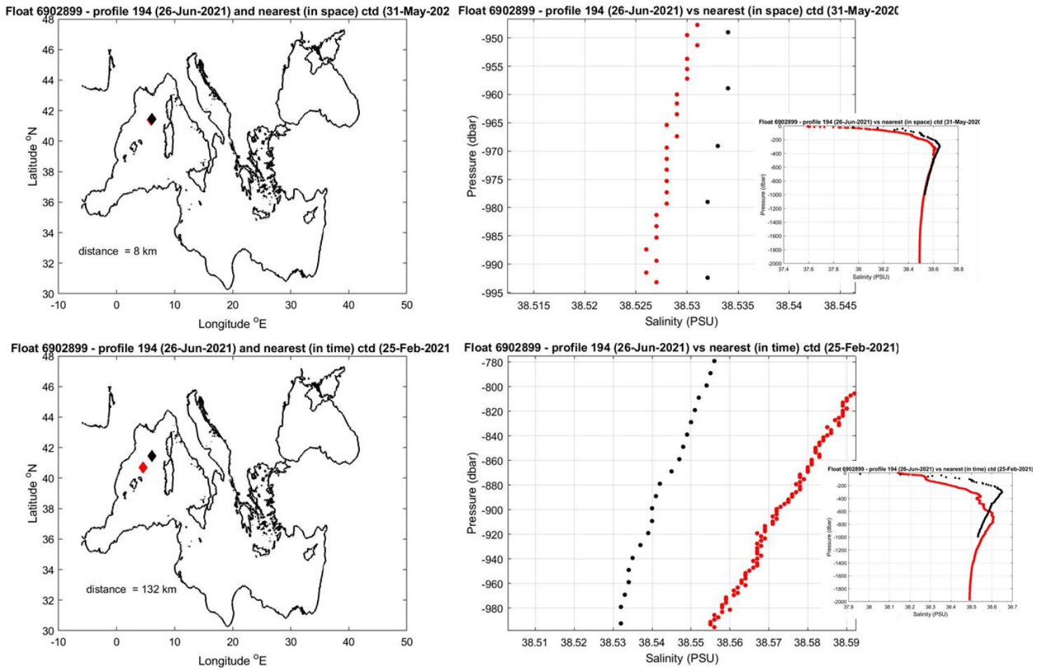
Figure 11: Float 6902899. The salinity float profile number 194 (black dots) are compared to the nearest in space (top) and in time (bottom) reference profile (red dots). The locations of the two profiles and their distance is given in the left panel.
