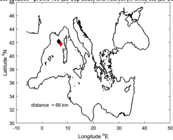
Figure 10: Float 6902899. The salinity float profile number 100 (black dots) are compared to the nearest in space (top) and in time (bottom) reference profile (red dots). The locations of the two profiles and their distance is given in the left panel.
