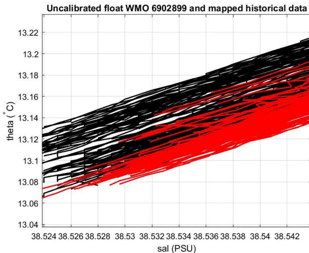
Figure 18: Float 6902899. Uncalibrated float salinity profile (black lines) and mapped historical data (red lines) in the most uniform part of the \theta -S curve.
