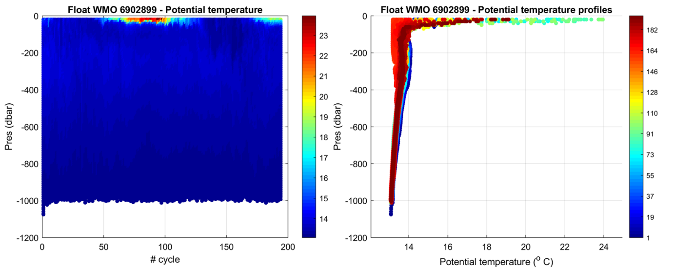
Figure 2: Float 6902899. Time series of Argo float potential temperature (°C) on the left, and potential temperature profiles color-coded per cycle number on the right.
