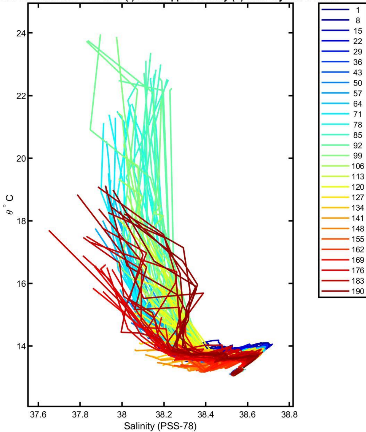
6902899 uncalibrated float data (-) and mapped salinity (o) with objective errors
