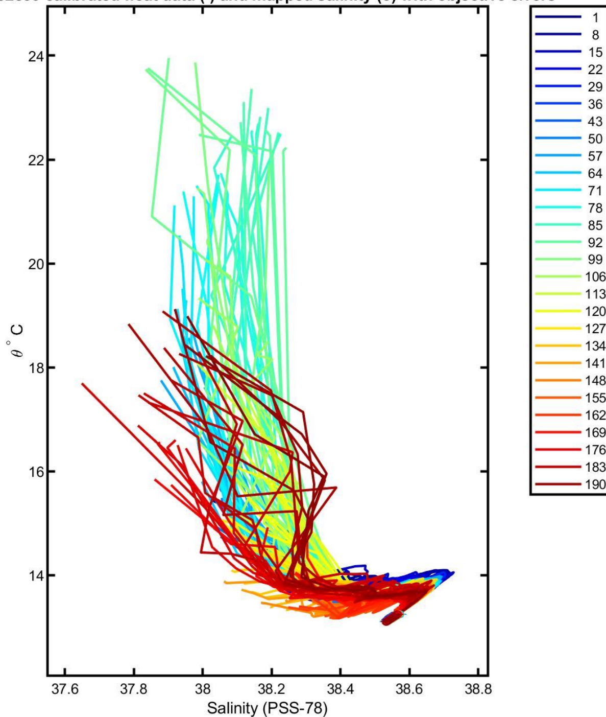
6902899 calibrated float data (-) and mapped salinity (o) with objective errors
