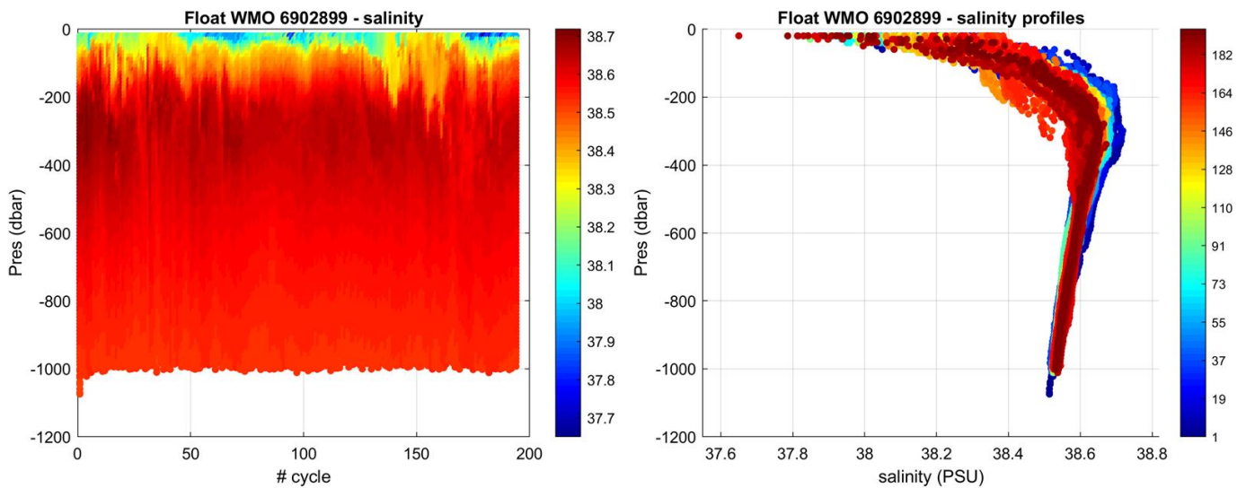
Figure 3: Float 6902899. Time series of Argo float potential salinity (PSS-78) on the left, and salinity profiles color-coded per cycle number on the right.
