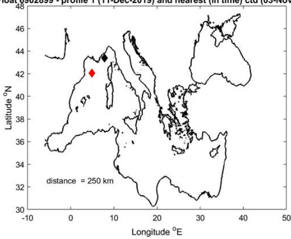
Figure 9: Float 6902899. The salinity float profile number 1 (black dots) are compared to the nearest in space (top) and in time (bottom) reference profile (red dots). The locations of the two profiles and their distance is given in the left panel.
