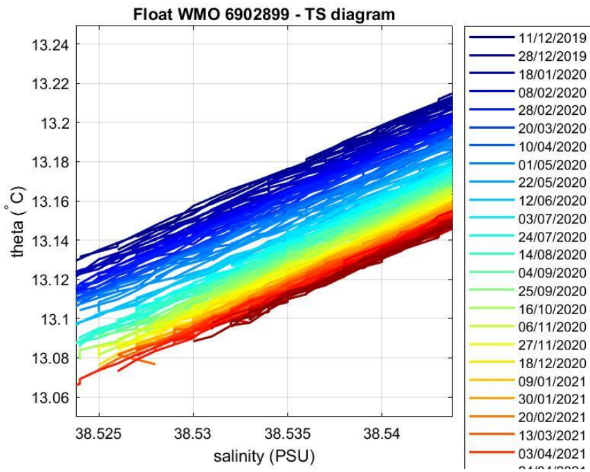
Figure 5: Float 6902899. Area of the \theta -S diagram (color-coded per cycle number) where the \theta -S relationship is more uniform.
