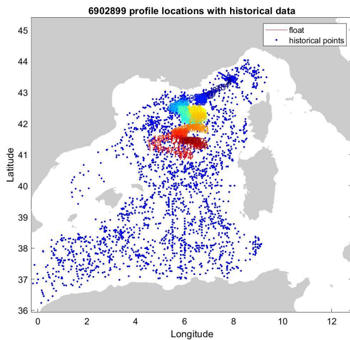
Figure 12: Float 6902899. Location of the float profiles (red line with colored numbers) and the reference data selected for mapping (blue dots).
