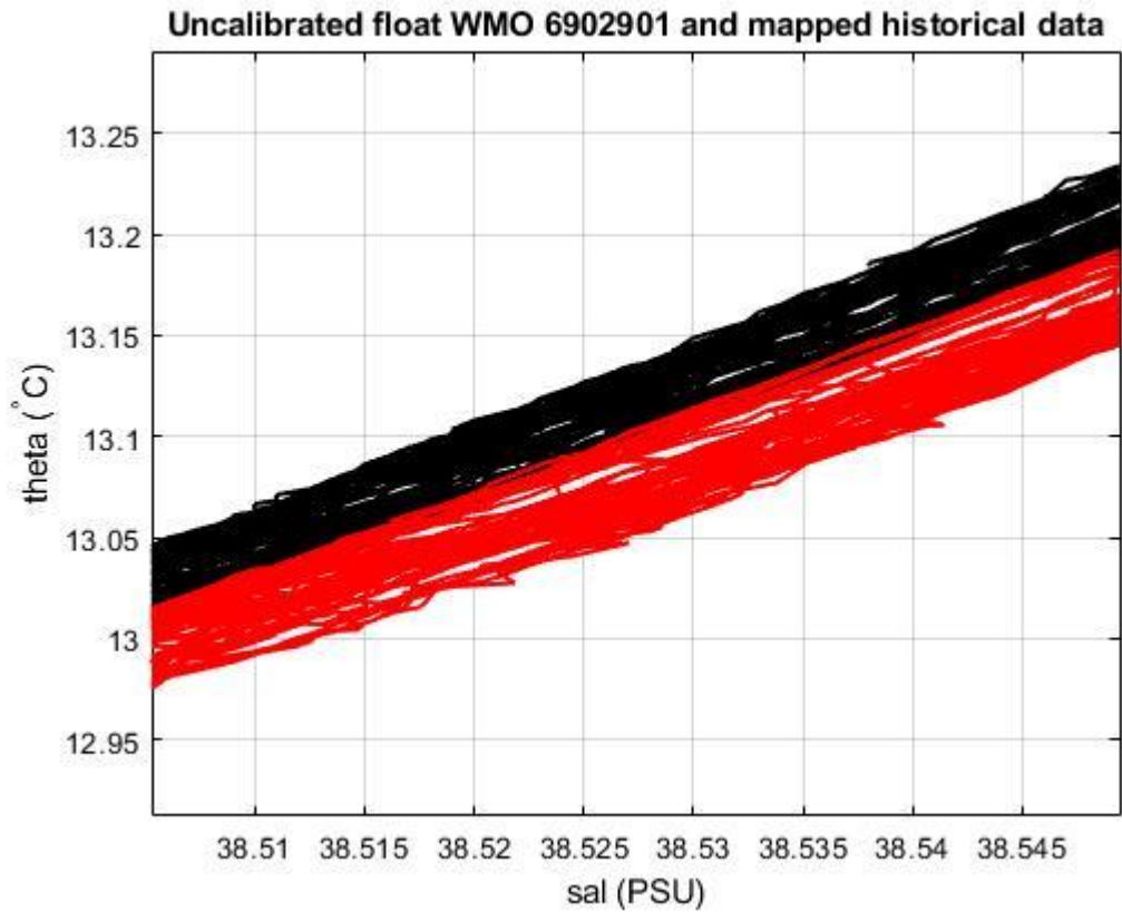
Figure 19: Float 6902901. Uncalibrated float salinity profile (black lines) and mapped historical data (red lines) in the most uniform part of the \theta -S curve.
