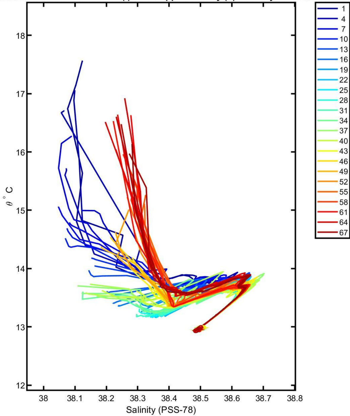
6902901 calibrated float data (-) and mapped salinity (o) with objective errors
