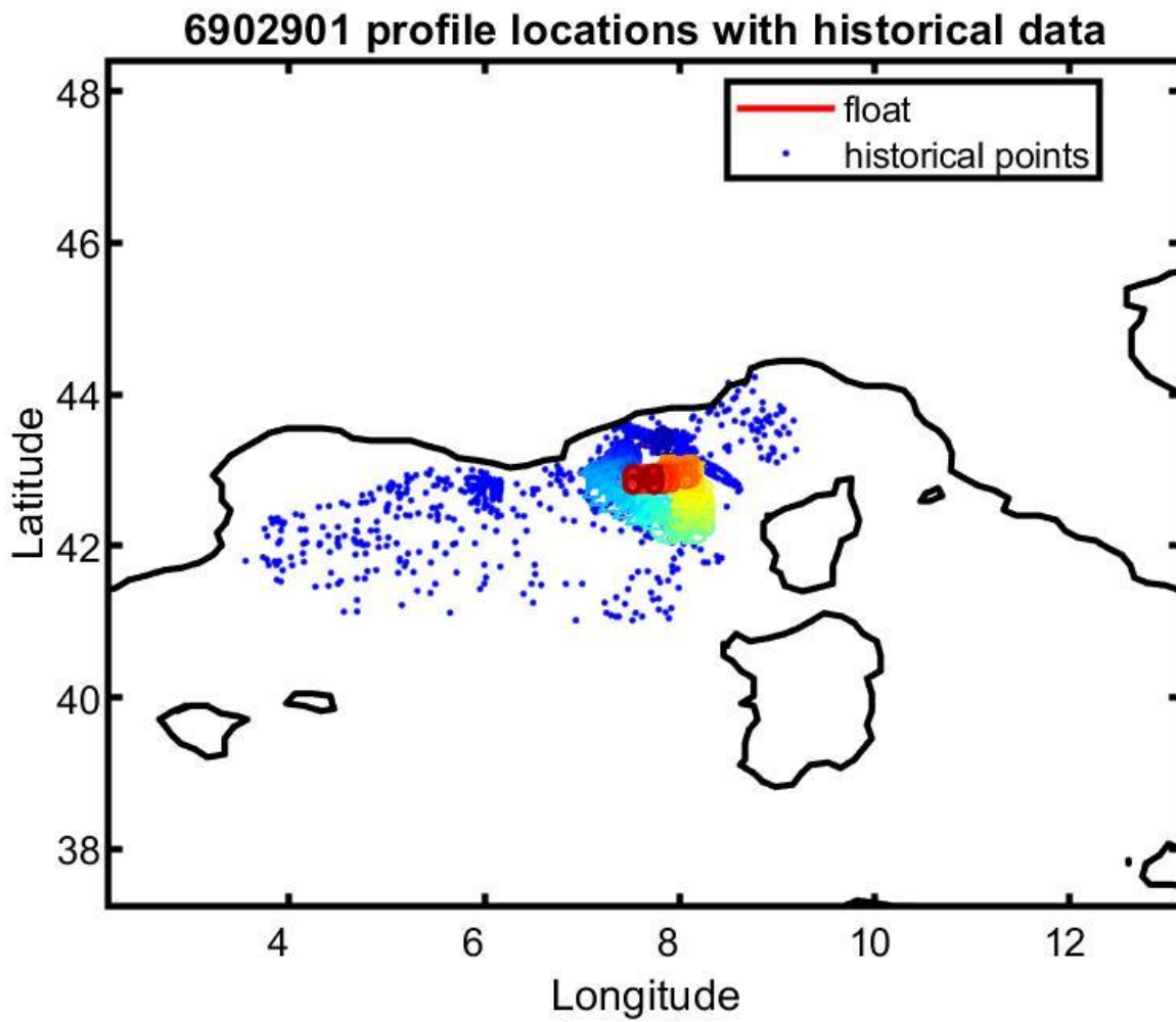
Figure 13: Float 6902901. Location of the float profiles (red line with colored numbers) and the reference data selected for mapping (blue dots).
