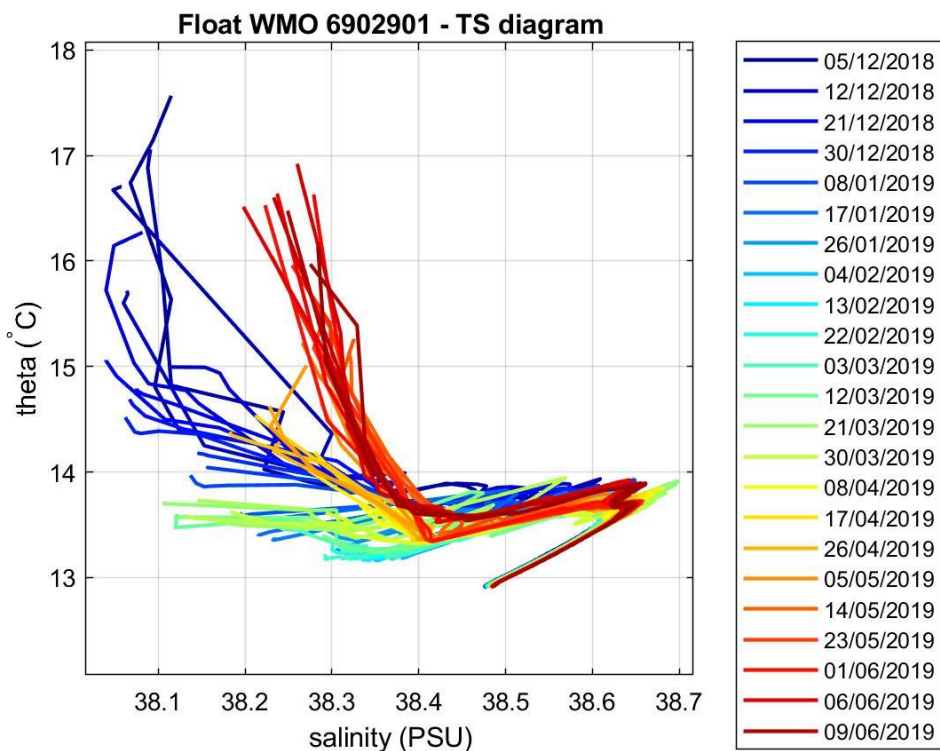
Figure 4: Float 6902901. \theta -S diagram color-coded per cycle number.
