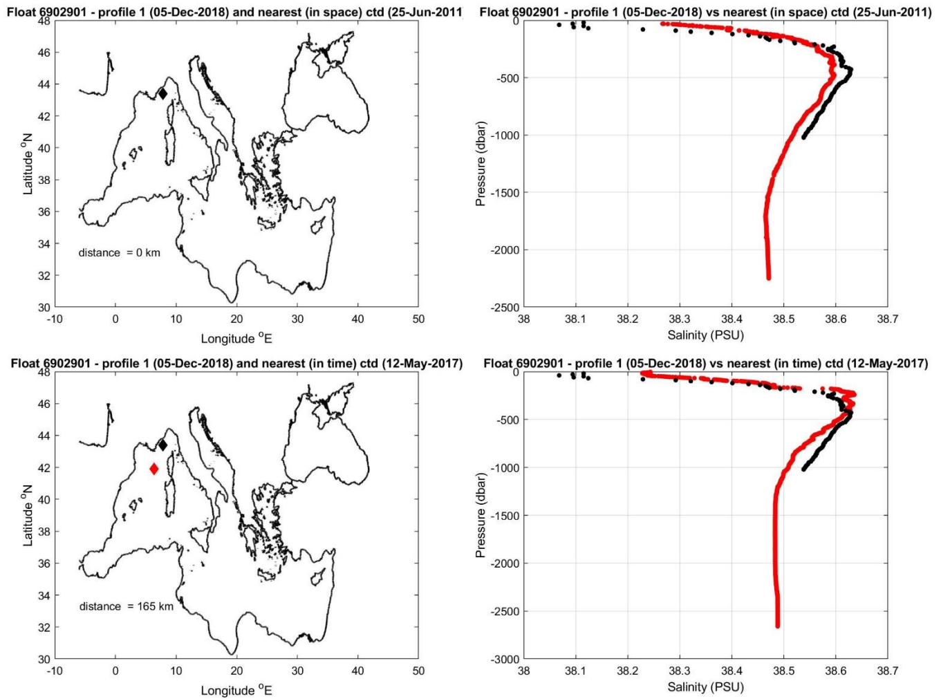
Figure 9: Float 6902901. The salinity float profile number 1 (black dots) are compared to the nearest in space (top) and in time (bottom) reference profile (red dots). The locations of the two profiles and their distance is given in the left panel.
