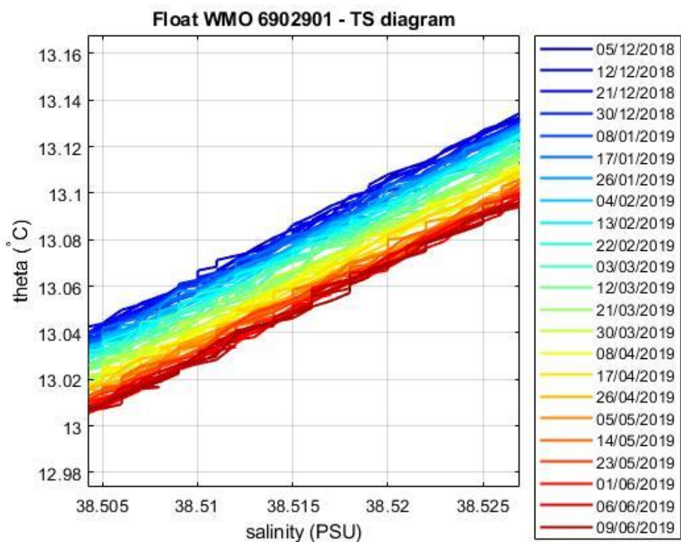
Figure 5: Float 6902901. Area of the \theta -S diagram (color-coded per cycle number) where the \theta -S relationship is more uniform.
