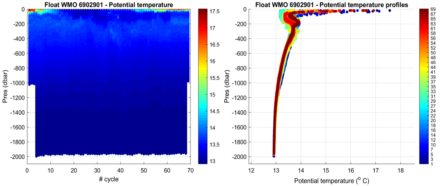
Figure 2: Float 6902901. Time series of Argo float potential temperature ( ^{\circ}\text{C} ) on the left, and potential temperature profiles color-coded per cycle number on the right.
