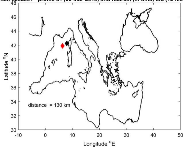
Float 6902901 - profile 31 (03-Mar-2019) and nearest (in time) ctd (12-May-2017)
