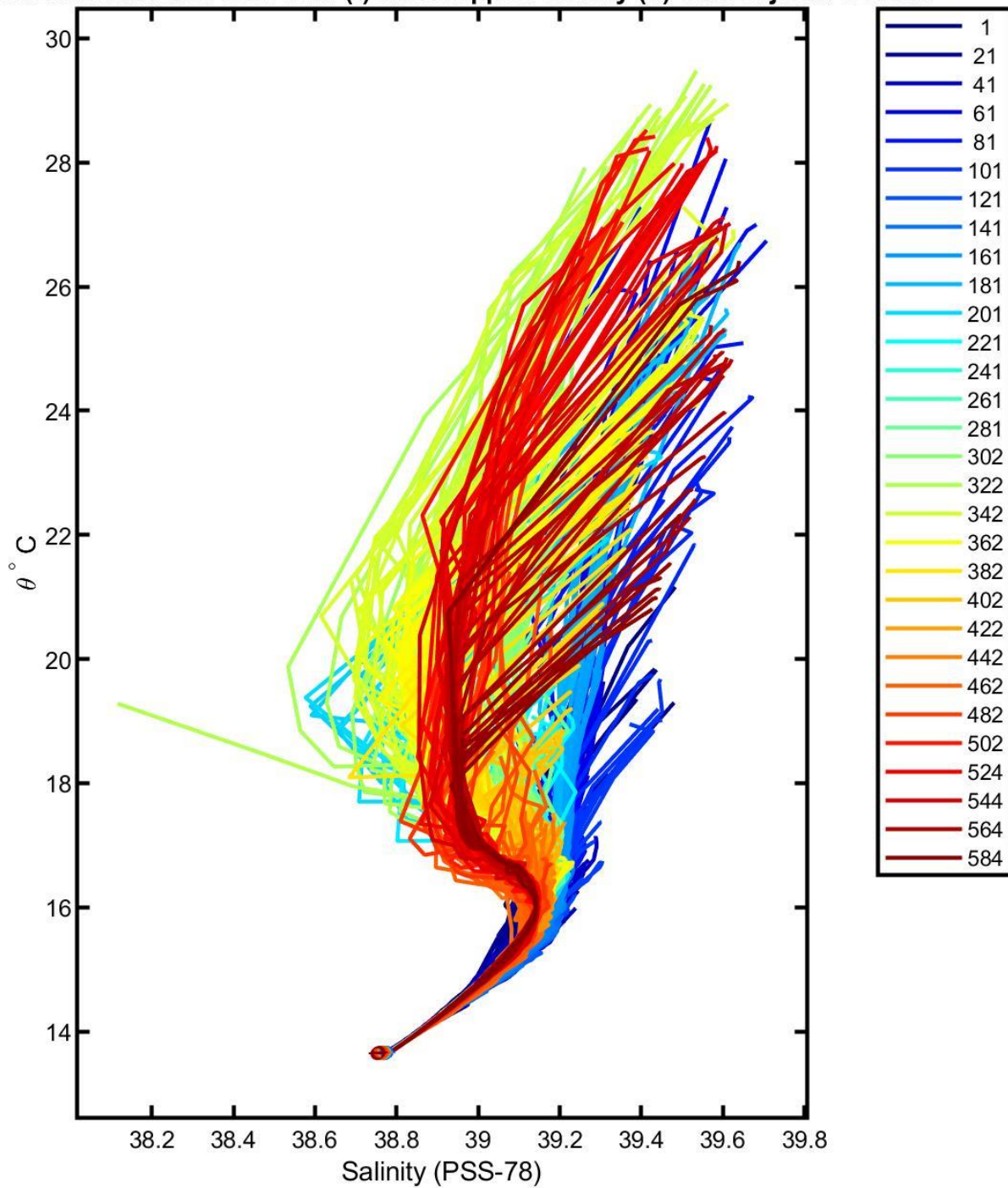
3902902 uncalibrated float data (-) and mapped salinity (o) with objective errors
