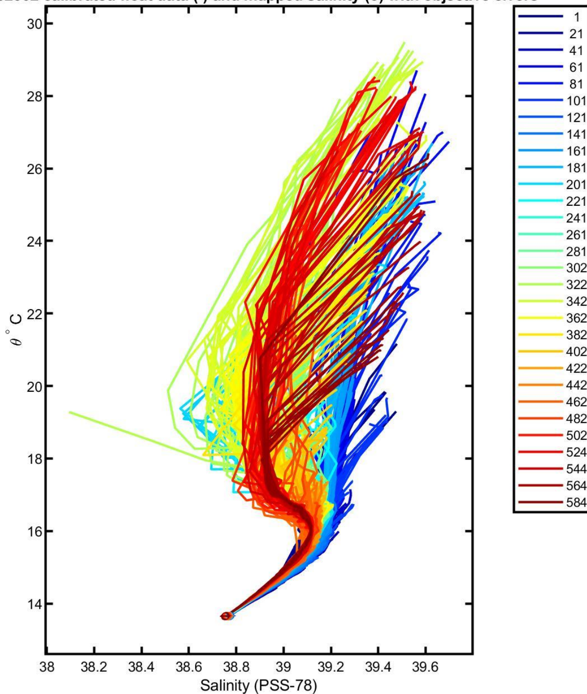
6902902 calibrated float data (-) and mapped salinity (o) with objective errors
