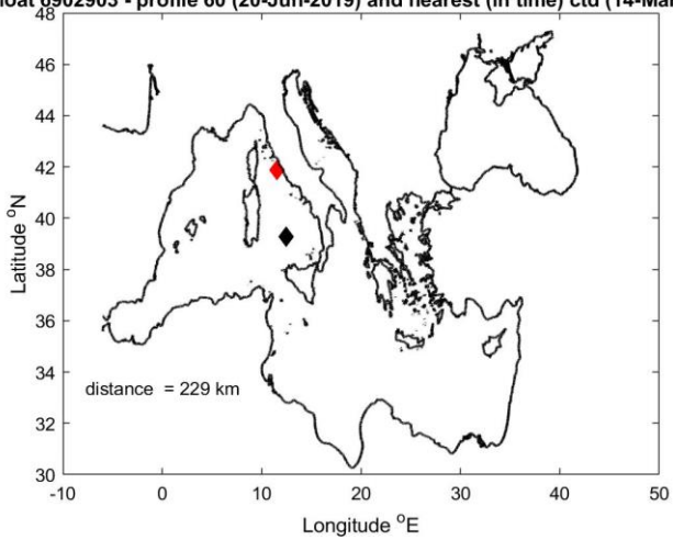
Float 6902903 - profile 60 (20-Jun-2019) and nearest (in time) ctd (14-Mar-2016)
