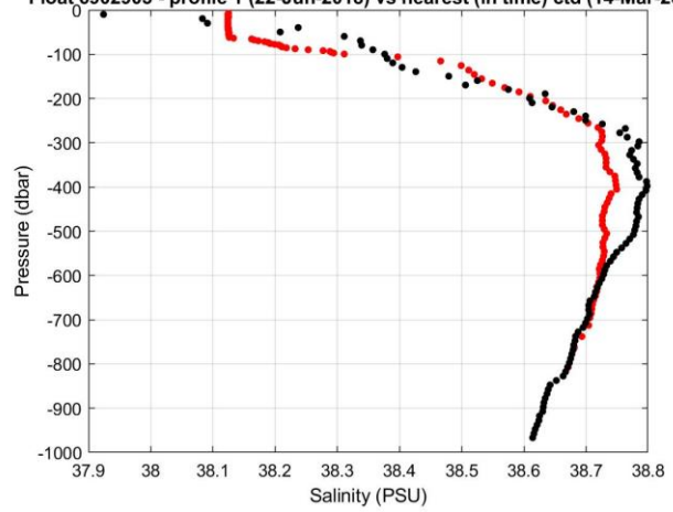
Figure 9: Float 6902903. The salinity float profile number 1 (black dots) are compared to the nearest in space (top) and in time (bottom) reference profile (red dots). The locations of the two profiles and their distance is given in the left panel.
