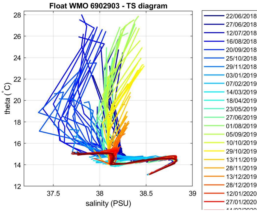
Figure 4: Float 6902903. \theta -S diagram color-coded per cycle number.
