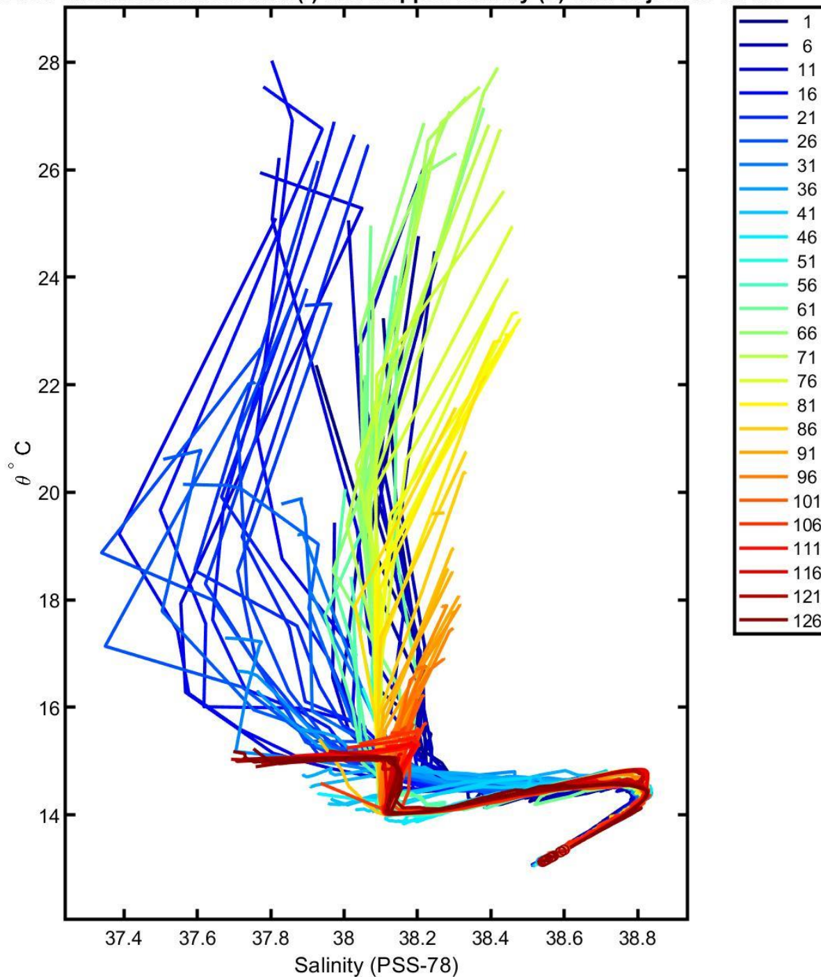
6902903 uncalibrated float data (-) and mapped salinity (o) with objective errors
