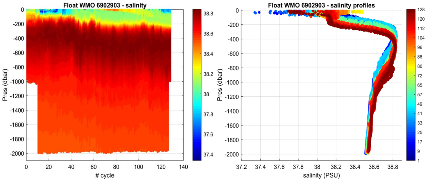
Figure 3: Float 6902903. Time series of Argo float potential salinity (PSS-78) on the left, and salinity profiles color-coded per cycle number on the right.
