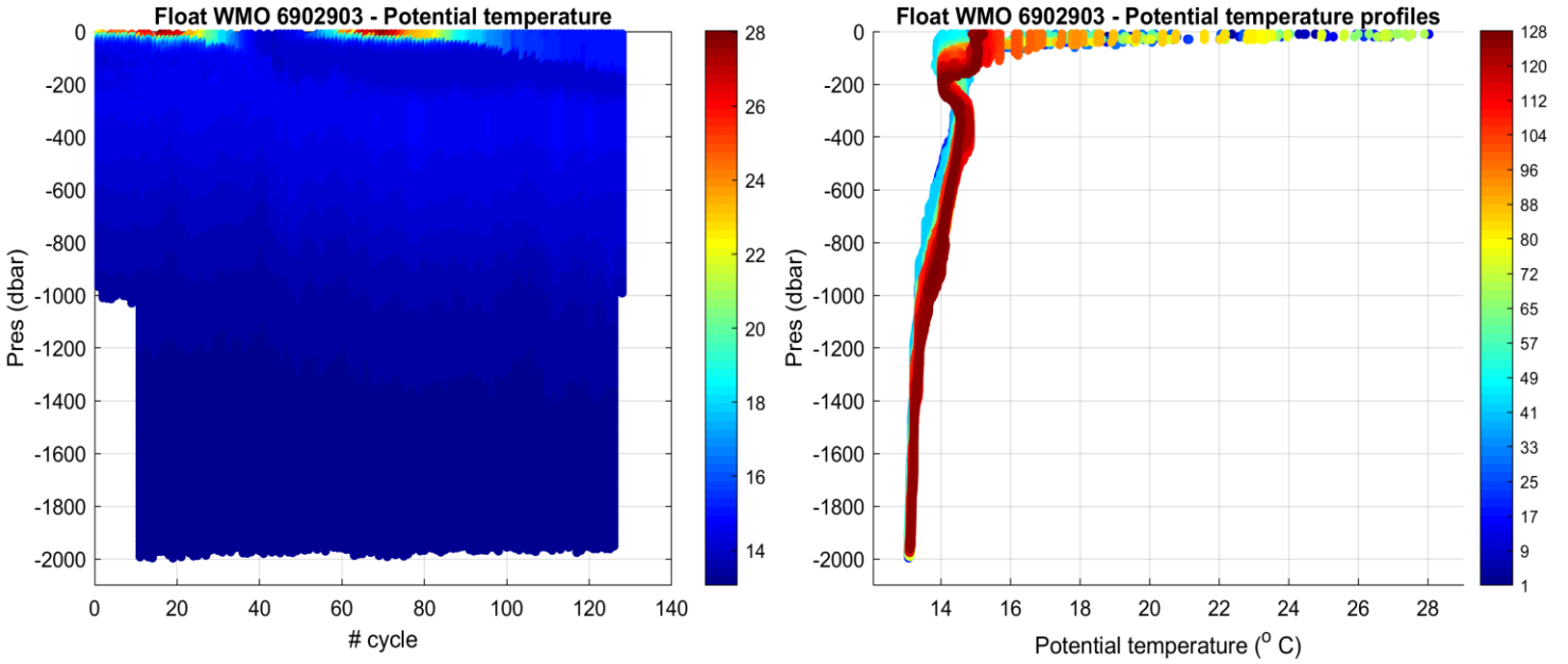
Figure 2: Float 6902903. Time series of Argo float potential temperature ( ^{\circ}\text{C} ) on the left, and potential temperature profiles color-coded per cycle number on the right.
