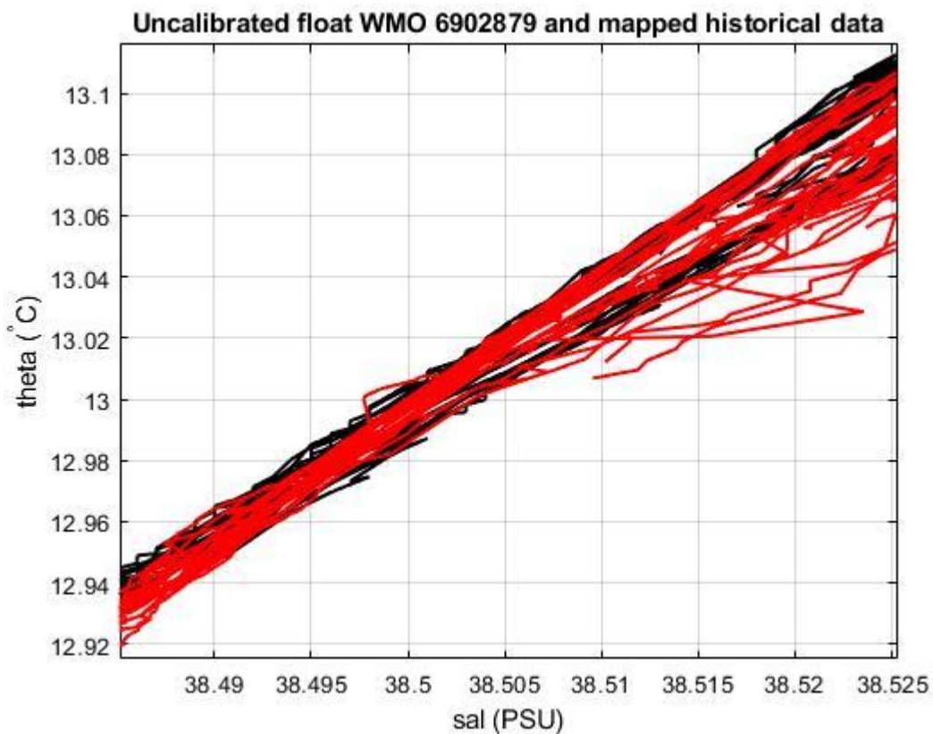
Figure 19: Float 6902879. Uncalibrated float salinity profile (black lines) and mapped historical data (red lines) in the most uniform part of the \theta -S curve.
