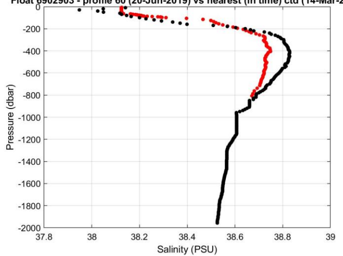
Float 6902903 - profile 60 (20-Jun-2019) vs nearest (in time) ctd (14-Mar-2016)
