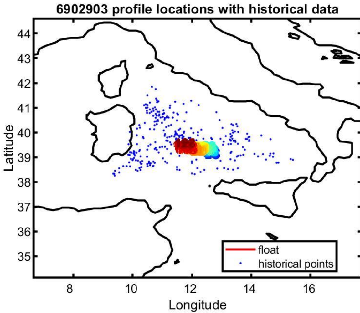
Figure 13: Float 6902903. Location of the float profiles (red line with colored numbers) and the reference data selected for mapping (blue dots).
