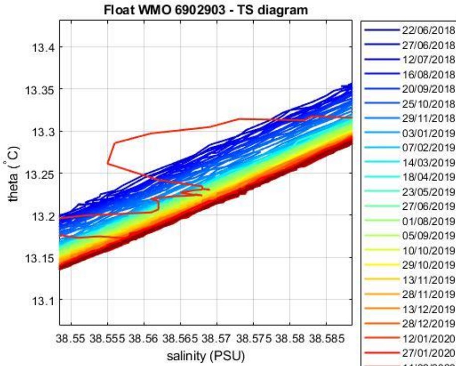
Figure 5: Float 6902903. Area of the \theta -S diagram (color-coded per cycle number) where the \theta -S relationship is more uniform.
