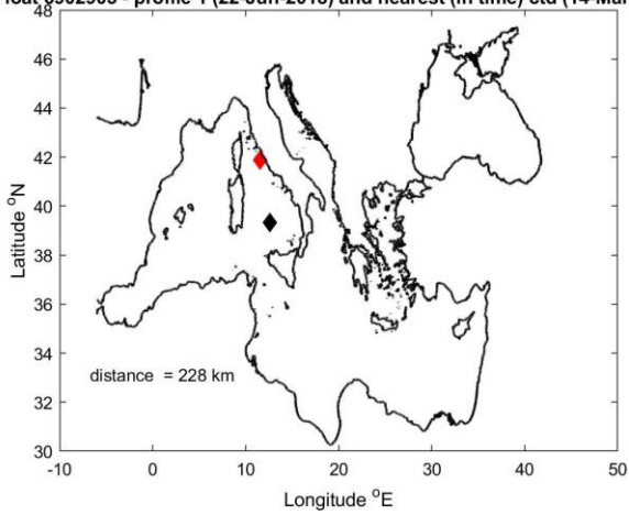
Figure 9: Float 6902903. The salinity float profile number 1 (black dots) are compared to the nearest in space (top) and in time (bottom) reference profile (red dots). The locations of the two profiles and their distance is given in the left panel.
