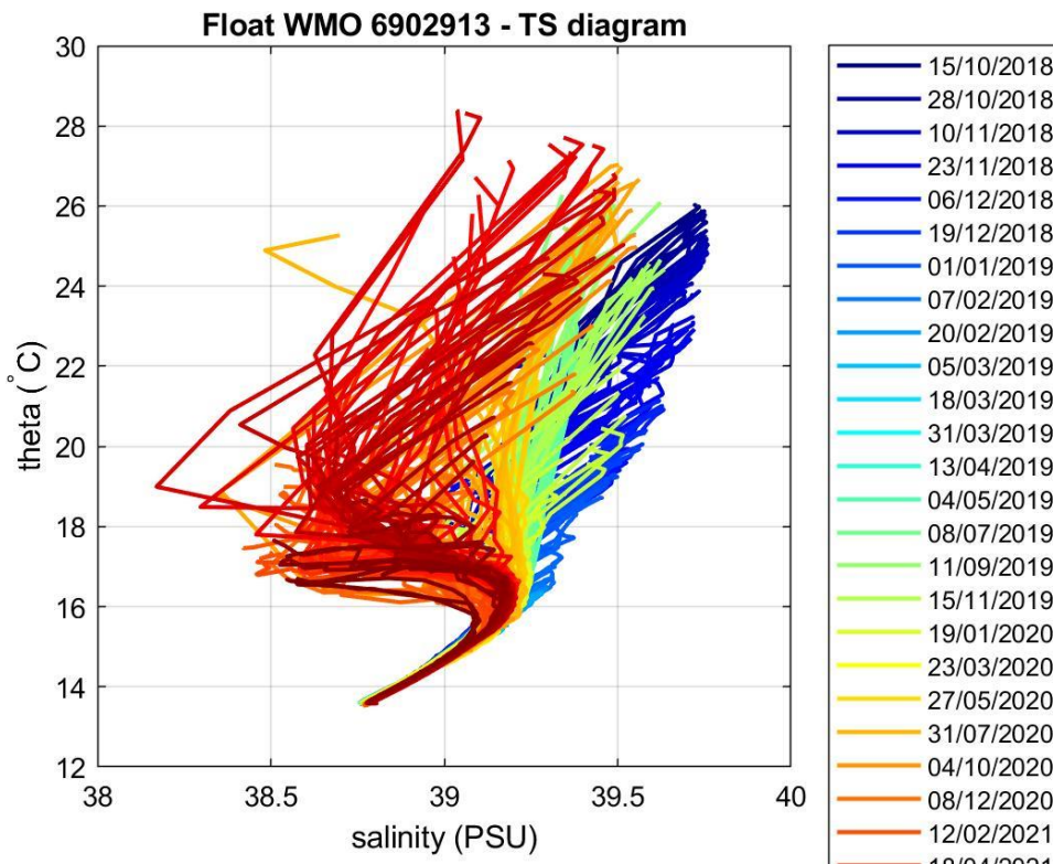
Figure 3: Float 6902913. \theta -S diagram color-coded per cycle number.
