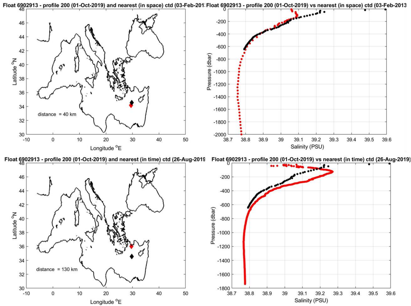
Figure 9: Float 6902913. The salinity float profile number 200 (black dots) are compared to the nearest in space (top) and in time (bottom) reference profile (red dots). The locations of the two profiles and their distance is given in the left panel.
