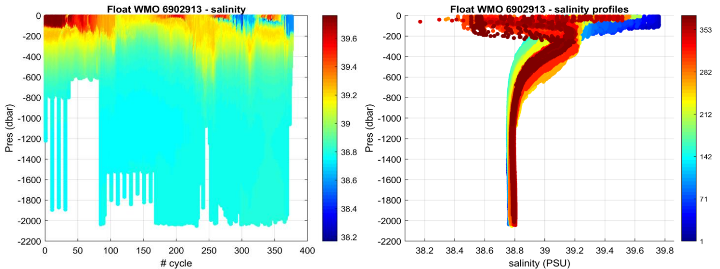
Figure 2: Float 6902913. Time series of Argo float potential salinity (PSS-78) on the left, and salinity profiles color-coded per cycle number on the right.
