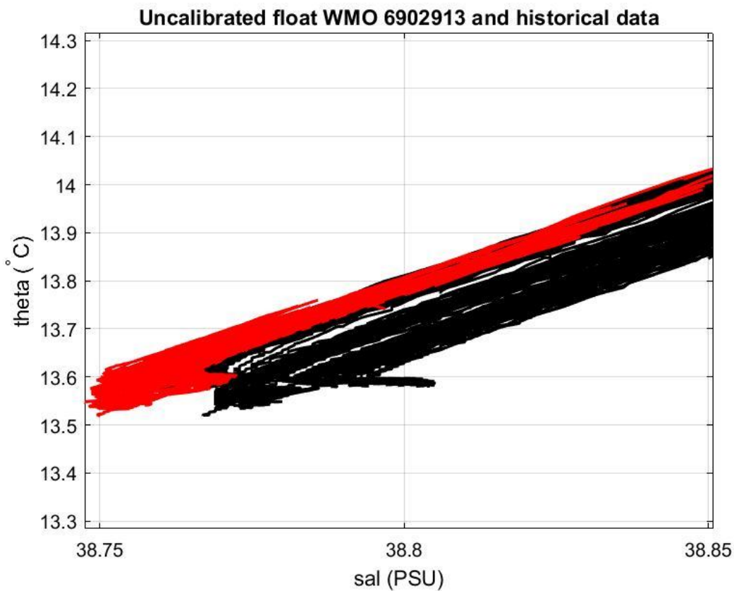
Figure 19: Float 6902913. Uncalibrated float salinity profile (black lines) and mapped historical data (red lines) in the most uniform part of the \theta -S curve.
