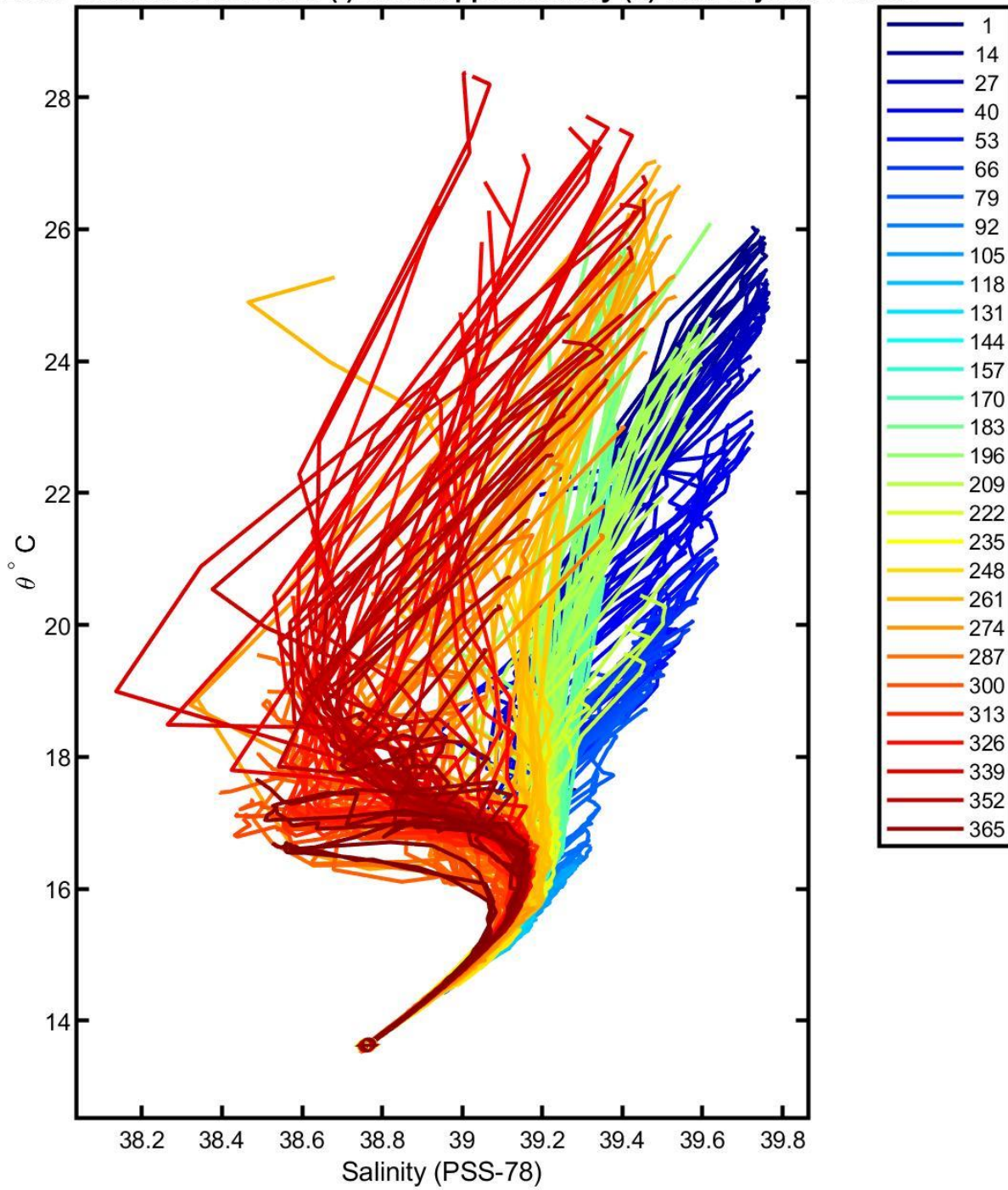
6902913 calibrated float data (-) and mapped salinity (o) with objective errors
