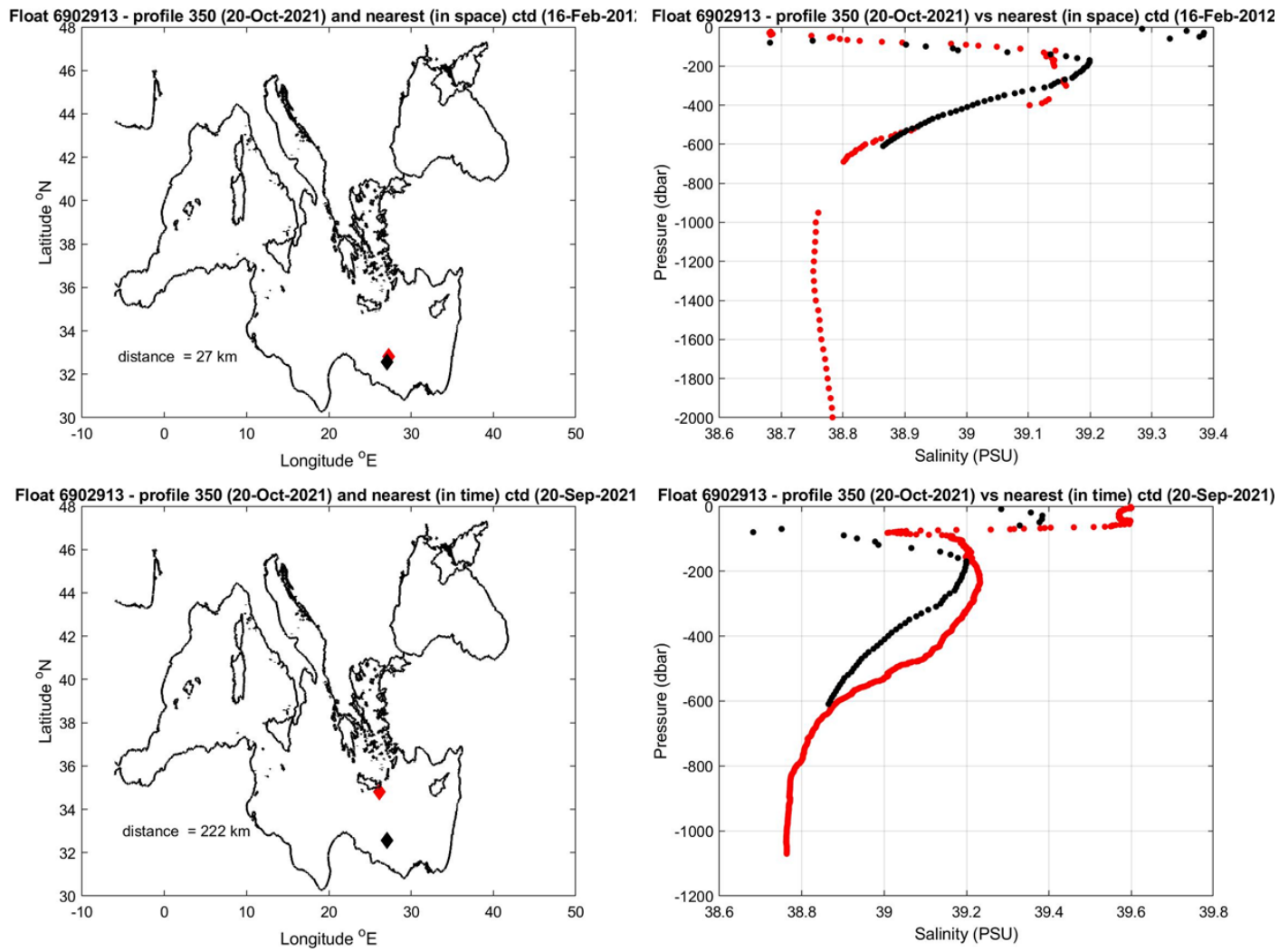
Figure 10: Float 6902913. The salinity float profile number 350 (black dots) are compared to the nearest in space (top) and in time (bottom) reference profile (red dots). The locations of the two profiles and their distance is given in the left panel.
