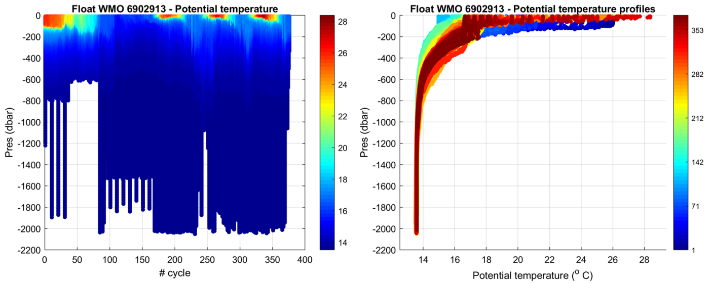
Figure 1: Float 6902913. Time series of Argo float potential temperature ( ^{\circ}\text{C} ) on the left, and potential temperature profiles color-coded per cycle number on the right.
