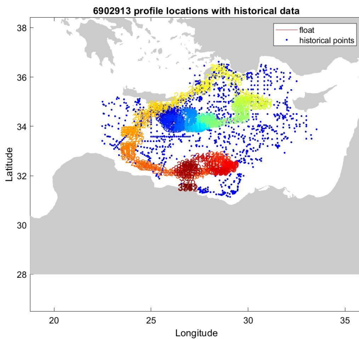
Figure 13: Float 6902913. Location of the float profiles (red line with colored numbers) and the reference data selected for mapping (blue dots).
