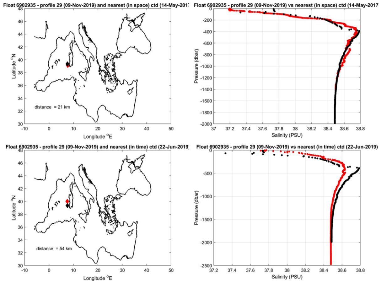
Figure 9: Float 6902935. The salinity float profile number 29 (black dots) are compared to the nearest in space (top) and in time (bottom) reference profile (red dots). The locations of the two profiles and their distance is given in the left panel.
