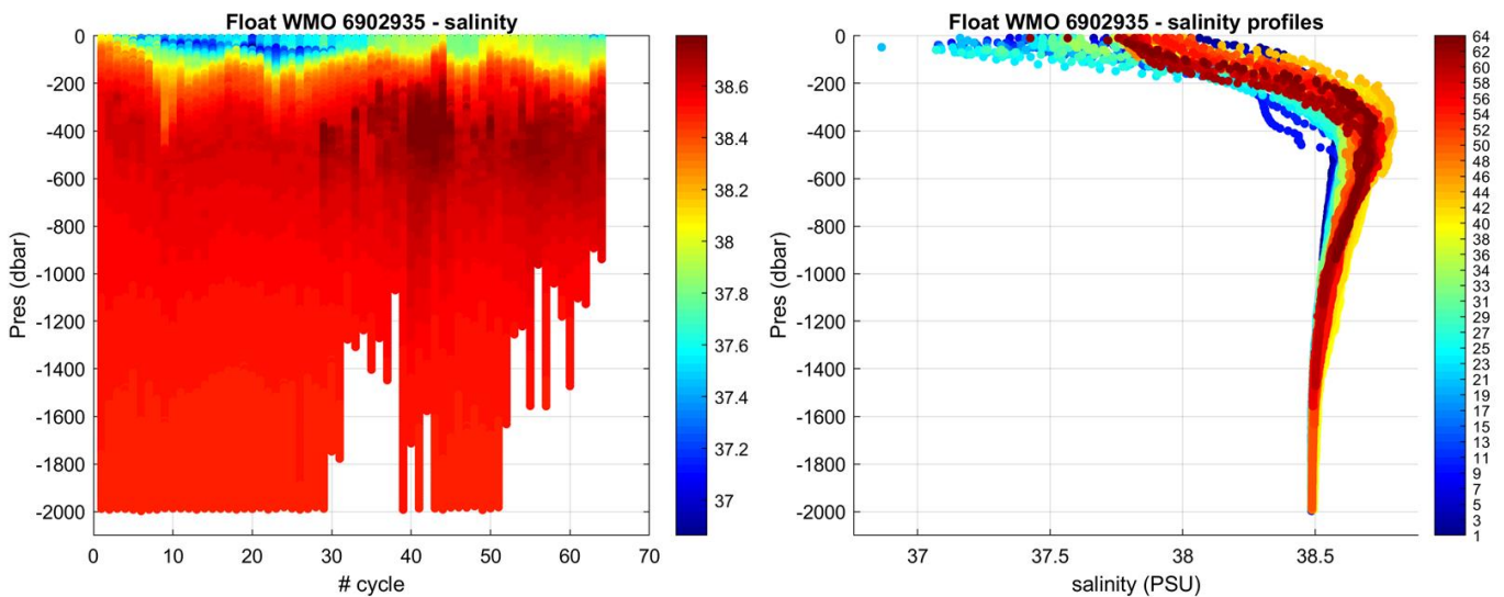
Figure 2: Float 6902935. Time series of Argo float potential salinity (PSS-78) on the left, and salinity profiles color-coded per cycle number on the right.
