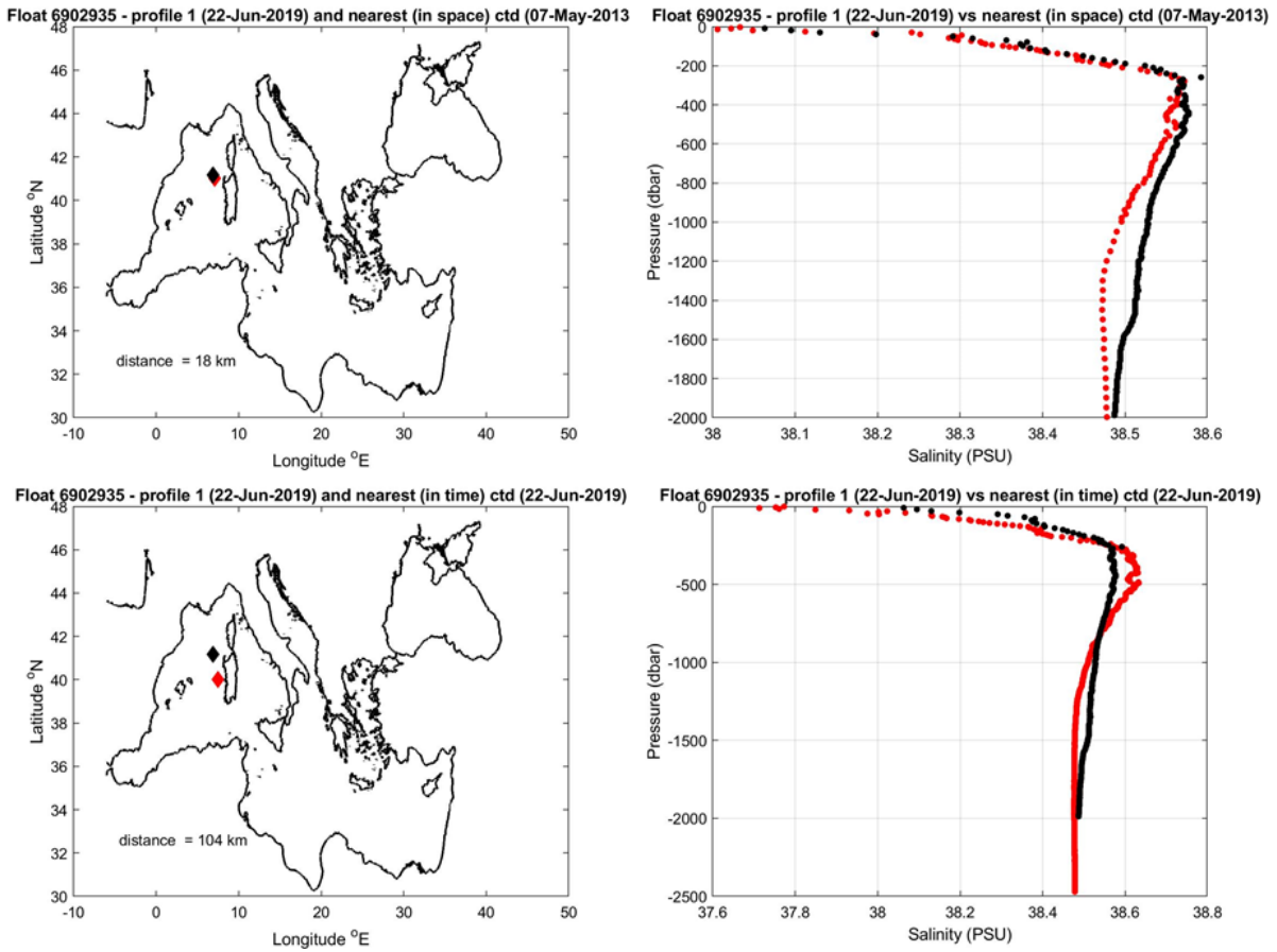
Figure 8: Float 6902935. The salinity float profile number 1 (black dots) are compared to the nearest in space (top) and in time (bottom) reference profile (red dots). The locations of the two profiles and their distance is given in the left panel.
