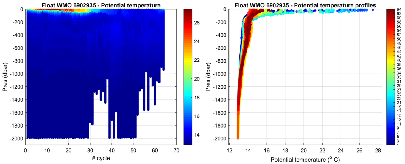
Figure 1: Float 6902935. Time series of Argo float potential temperature ( ^{\circ}\text{C} ) on the left, and potential temperature profiles color-coded per cycle number on the right.
