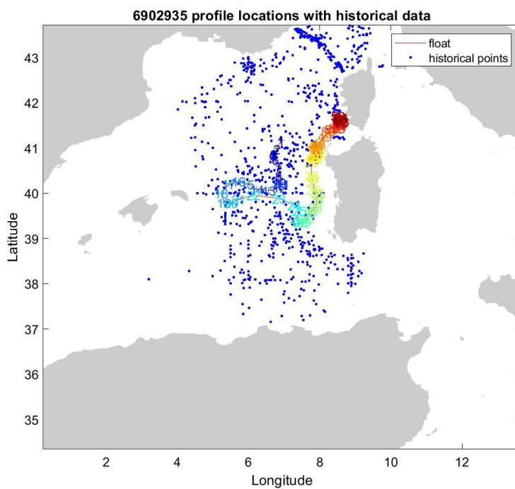
Figure 11: Float 6902935. Location of the float profiles (red line with colored numbers) and the reference data selected for mapping (blue dots).
