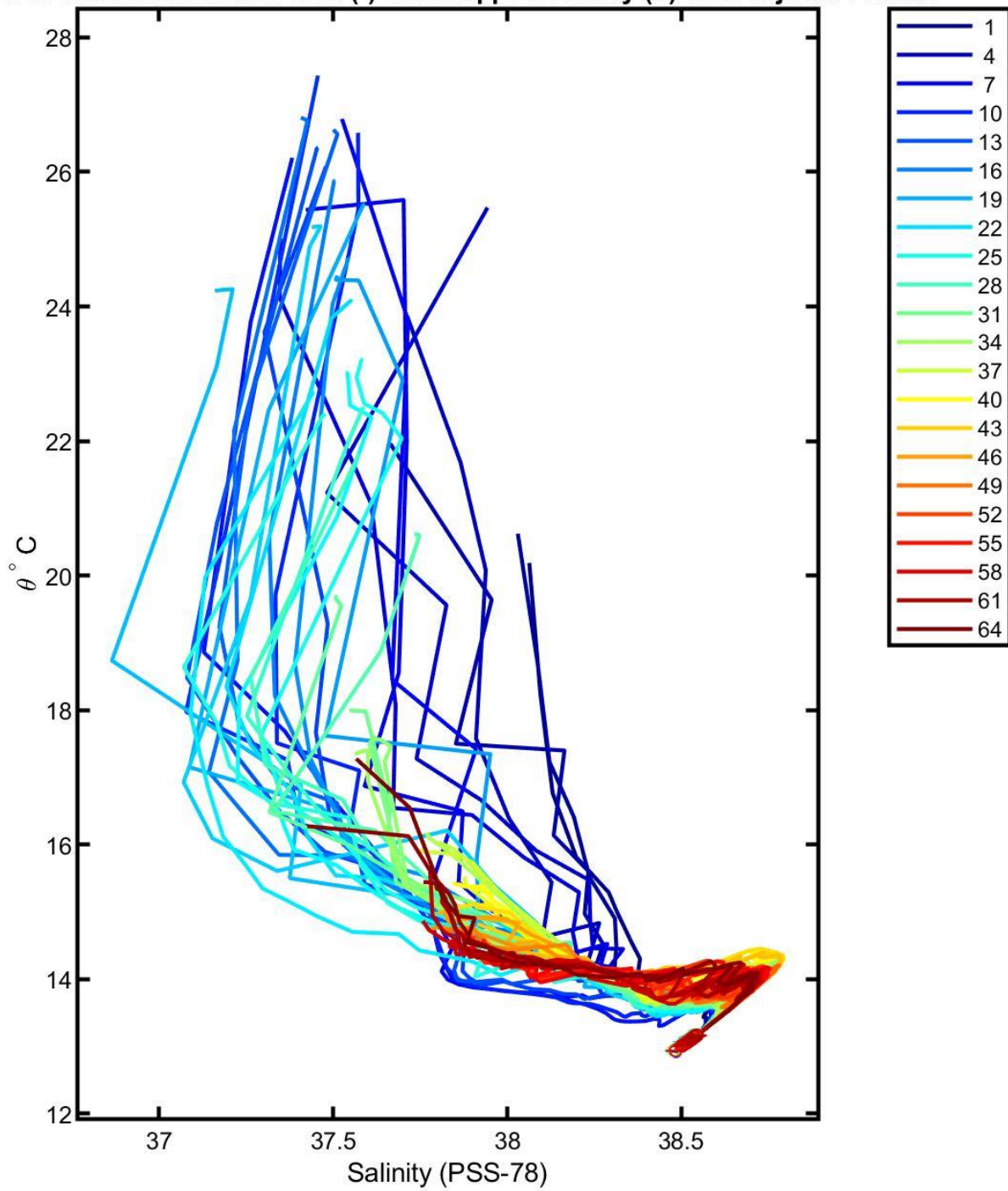
6902935 uncalibrated float data (-) and mapped salinity (o) with objective errors
