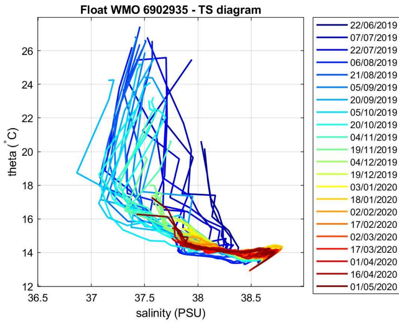
Figure 3: Float 6902935. \theta -S diagram color-coded per cycle number.
