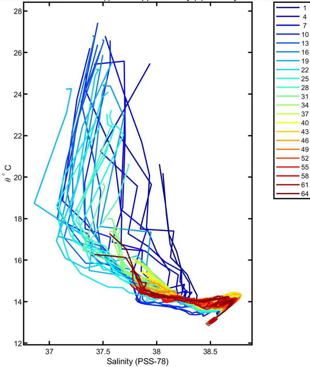
6902935 calibrated float data (-) and mapped salinity (o) with objective errors
