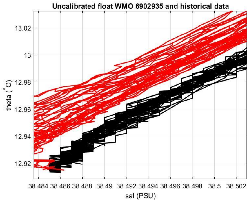
Figure 17: Float 6902935. Uncalibrated float salinity profile (black lines) and mapped historical data (red lines) in the most uniform part of the \theta -S curve.
