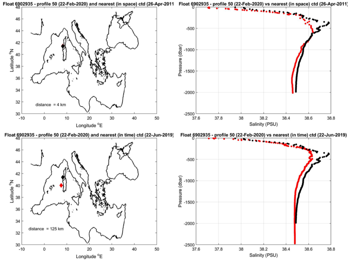
Figure 10: Float 6902935. The salinity float profile number 50 (black dots) are compared to the nearest in space (top) and in time (bottom) reference profile (red dots). The locations of the two profiles and their distance is given in the left panel.
