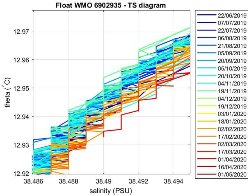
Figure 4: Float 6902935. Area of the \theta -S diagram (color-coded per cycle number) where the \theta -S relationship is more uniform.
