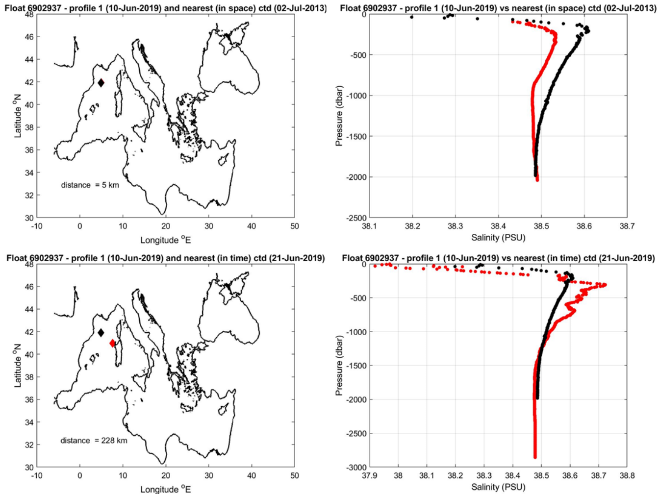
Figure 9: Float 6902937. The salinity float profile number 1 (black dots) are compared to the nearest in space (top) and in time (bottom) reference profile (red dots). The locations of the two profiles and their distance is given in the left panel.
