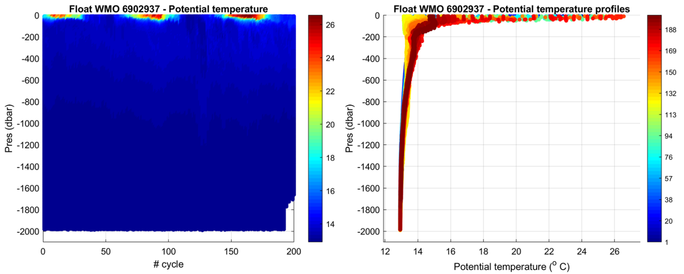
Figure 2: Float 6902937. Time series of Argo float potential temperature ( ^{\circ}\text{C} ) on the left, and potential temperature profiles color-coded per cycle number on the right.
