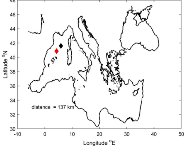
Figure 10: Float 6902937. The salinity float profile number 113 (black dots) are compared to the nearest in space (top) and in time (bottom) reference profile (red dots). The locations of the two profiles and their distance is given in the left panel.
