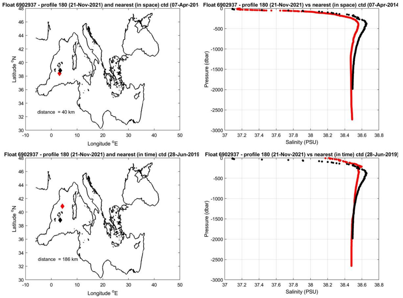
Figure 11: Float 6902937. The salinity float profile number 180 (black dots) are compared to the nearest in space (top) and in time (bottom) reference profile (red dots). The locations of the two profiles and their distance is given in the left panel.
