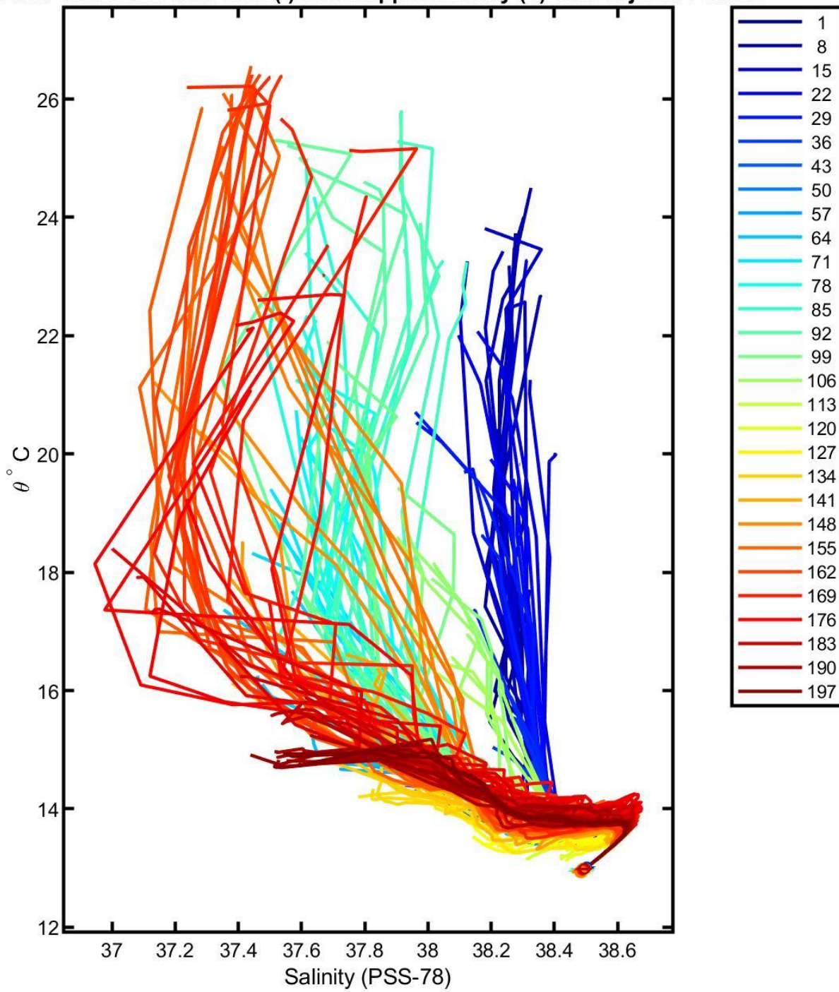
6902937 calibrated float data (-) and mapped salinity (o) with objective errors
