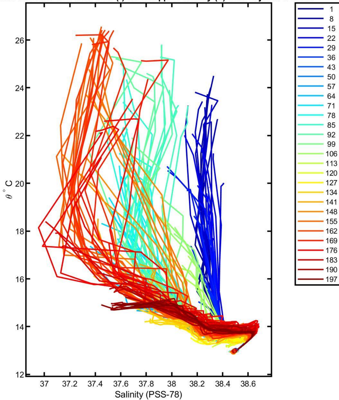
6902937 uncalibrated float data (-) and mapped salinity (o) with objective errors
