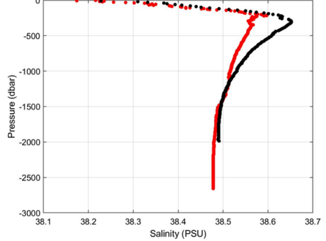
Float 6902937 - profile 113 (20-Dec-2020) vs nearest (in time) ctd (28-Jun-2019)
