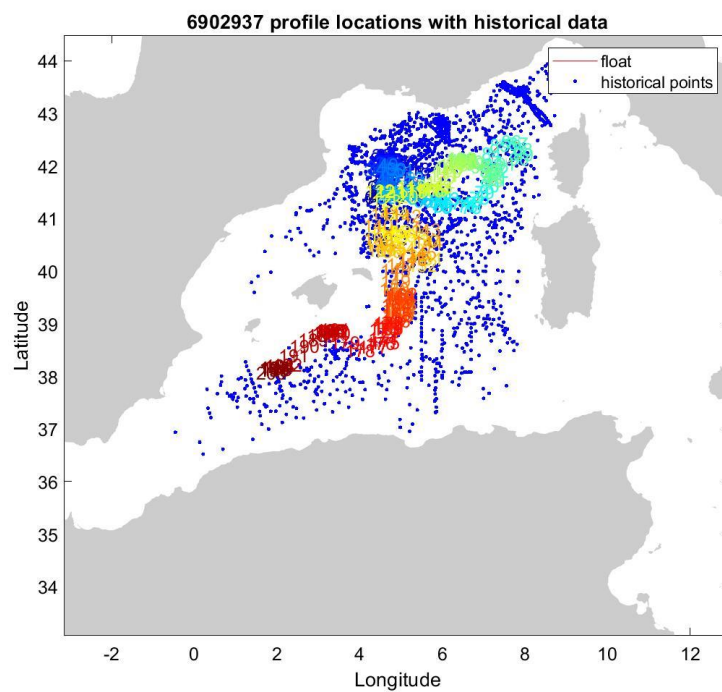
Figure 13: Float 6902937. Location of the float profiles (red line with colored numbers) and the reference data selected for mapping (blue dots).
