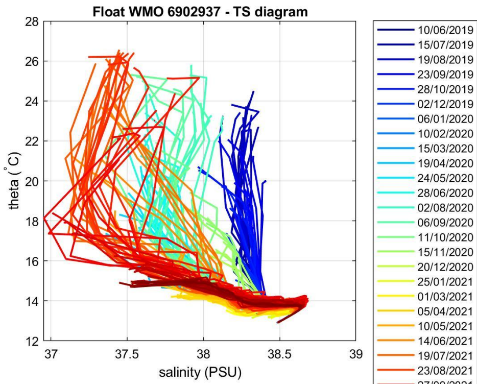
Figure 4: Float 6902937. \theta -S diagram color-coded per cycle number.
