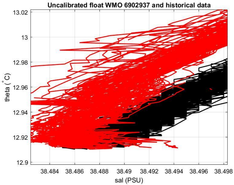
Figure 19: Float 6902937. Uncalibrated float salinity profile (black lines) and mapped historical data (red lines) in the most uniform part of the \theta -S curve.
