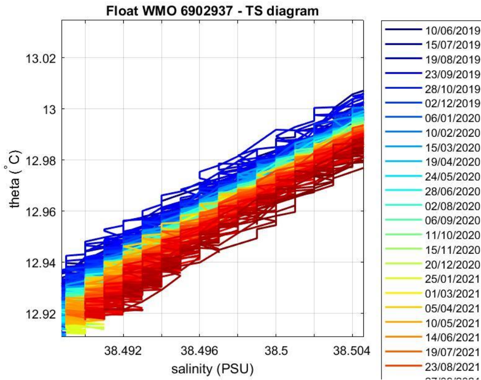
Figure 5: Float 6902937. Area of the \theta -S diagram (color-coded per cycle number) where the \theta -S relationship is more uniform.
