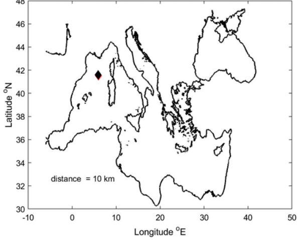
Float 6902937 - profile 113 (20-Dec-2020) and nearest (in time) ctd (28-Jun-2019)
