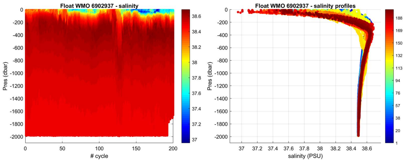
Figure 3: Float 6902937. Time series of Argo float potential salinity (PSS-78) on the left, and salinity profiles color-coded per cycle number on the right.
