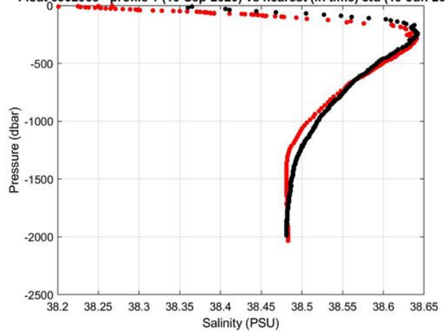
Float 6902965 - profile 1 (10-Sep-2020) vs nearest (in time) ctd (19-Jun-2015)
