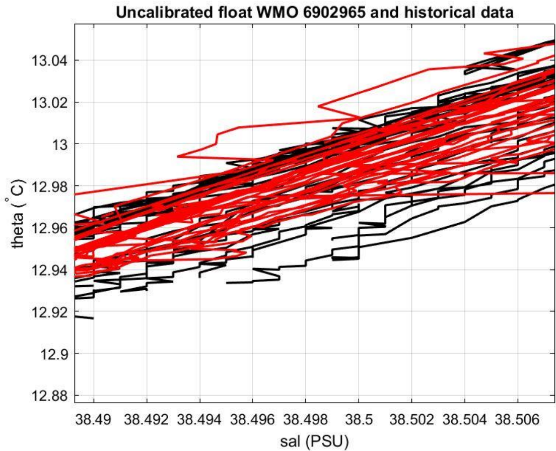
Figure 17: Float 6902965. Uncalibrated float salinity profile (black lines) and mapped historical data (red lines) in the most uniform part of the \theta -S curve.
