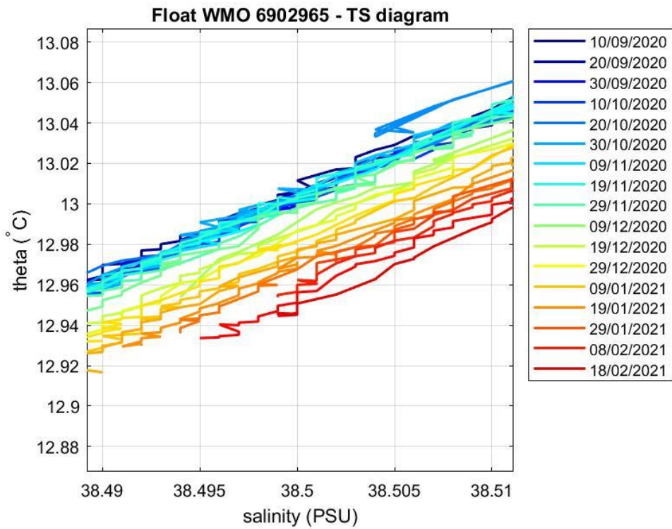
Figure 4: Float 6902965. Area of the \theta -S diagram (color-coded per cycle number) where the \theta -S relationship is more uniform.
