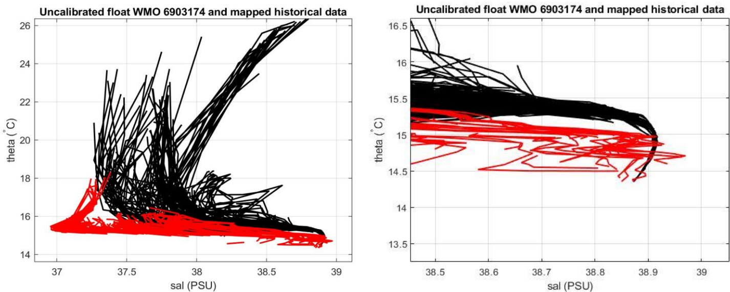
Figure 19: Float 6903174. Uncalibrated float salinity profile (black lines) and mapped historical data (red lines), on the left. Zoom in the most uniform part of the \theta -S curve, on the right.
