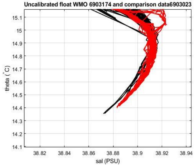
Figure 22: Float 6903174. Comparison between float 6903174 (black line) and float 6903023 (red line), on the left. On the right zoom in the most uniform part of the \theta -S curve
