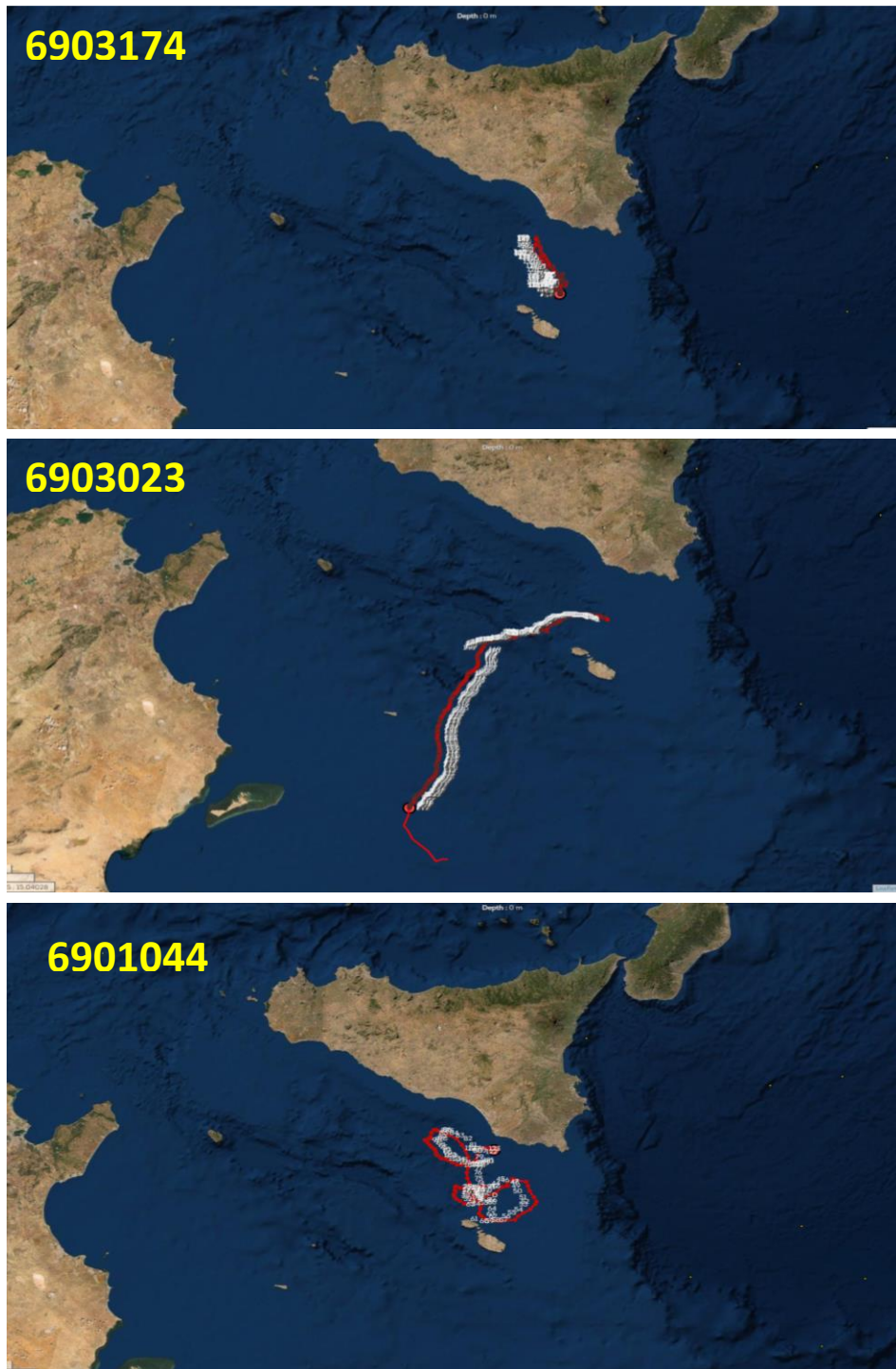
Figure 20: Float 6903174. Trajectory of the floats used for the comparison.
