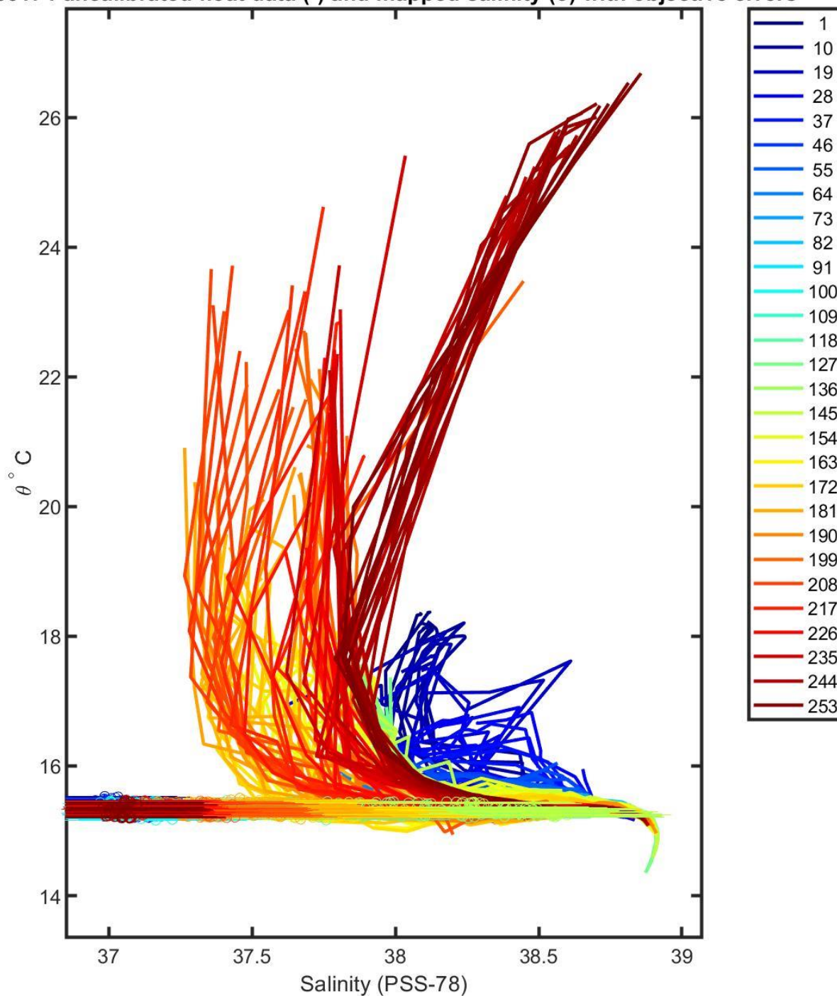
6903174 uncalibrated float data (-) and mapped salinity (o) with objective errors
