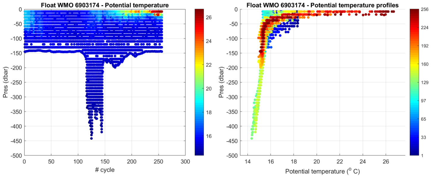
Figure 2: Float 6903174. Time series of Argo float potential temperature ( ^{\circ}\text{C} ) on the left, and potential temperature profiles color-coded per cycle number on the right.
