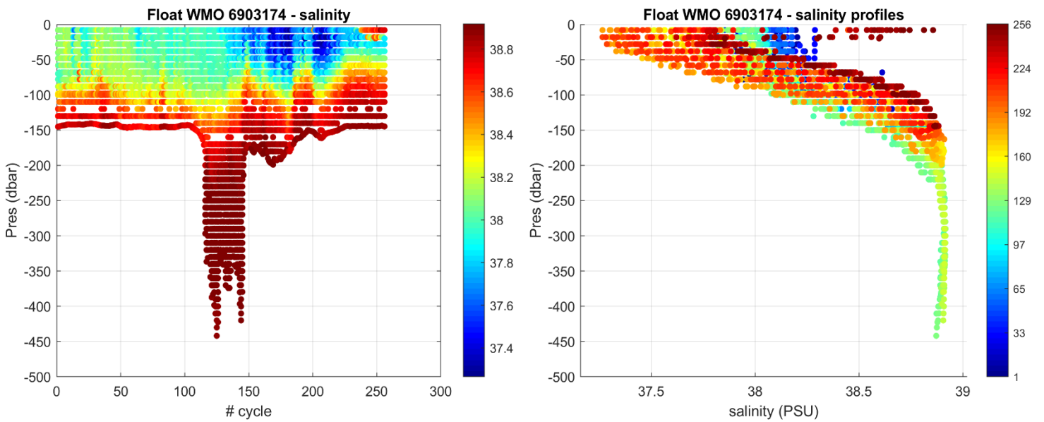
Figure 3: Float 6903174. Time series of Argo float potential salinity (PSS-78) on the left, and salinity profiles color-coded per cycle number on the right.
