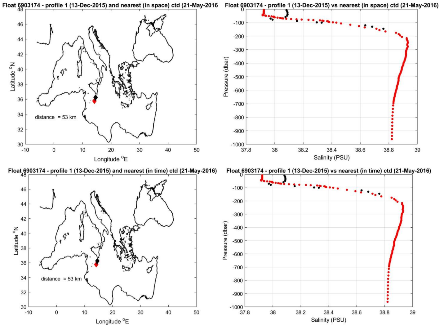
Figure 9: Float 6903174. The salinity float profile number 1 (black dots) are compared to the nearest in space (top) and in time (bottom) reference profile (red dots). The locations of the two profiles and their distance is given in the left panel.
