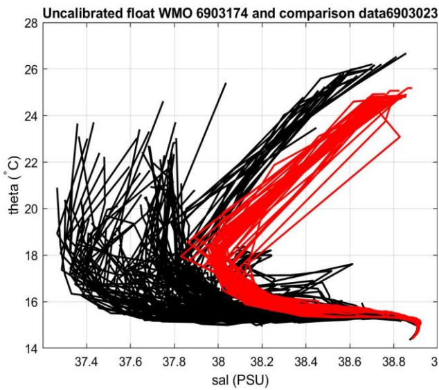
Figure 22: Float 6903174. Comparison between float 6903174 (black line) and float 6903023 (red line), on the left. On the right zoom in the most uniform part of the \theta -S curve
