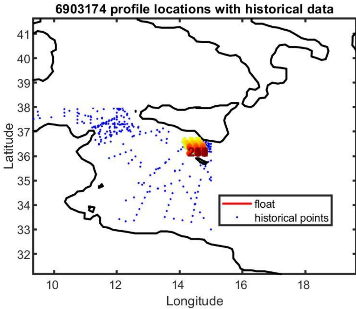
Figure 13: Float 6903174. Location of the float profiles (red line with colored numbers) and the reference data selected for mapping (blue dots).
