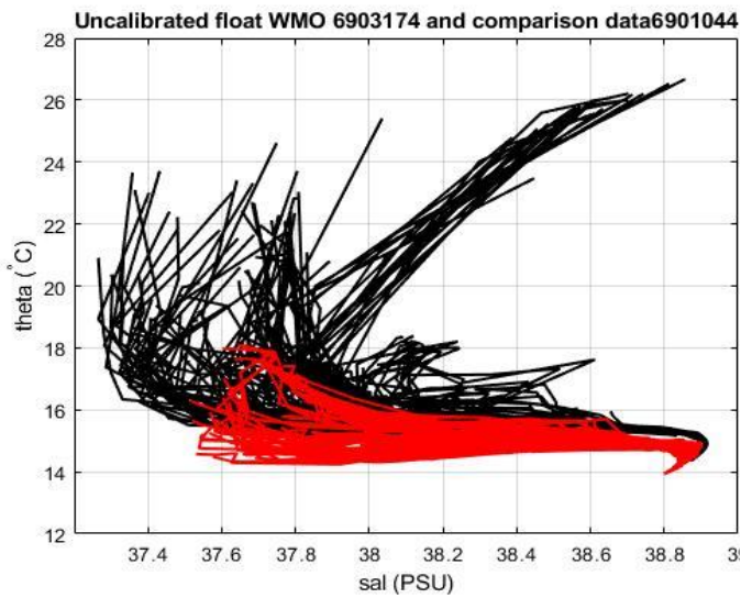
Figure 21: Float 6903174. Comparison between float 6903174 (black line) and float 6901044 (red line), on the left. On the right zoom in the most uniform part of the \theta -S curve
