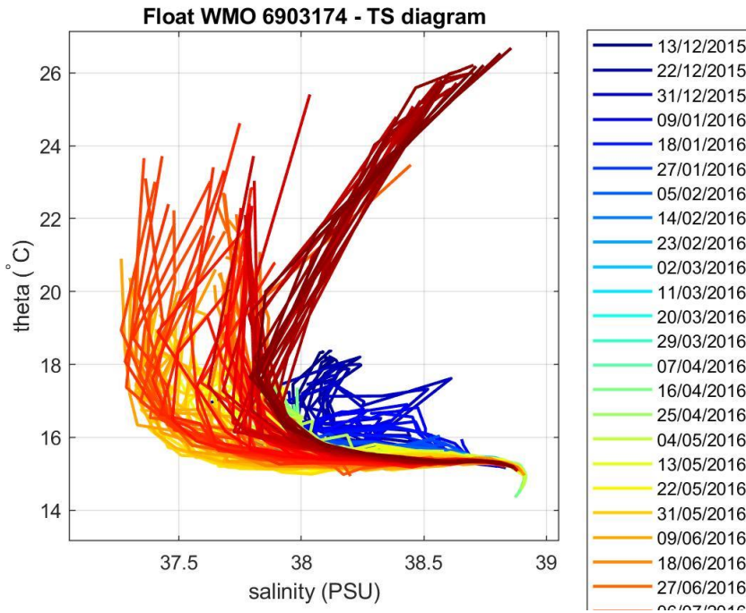
Figure 4: Float 6903174. \theta -S diagram color-coded per cycle number.
