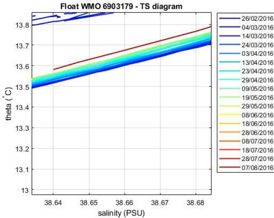
Figure 4: Float 6903179. \theta -S diagram color-coded per cycle number.
