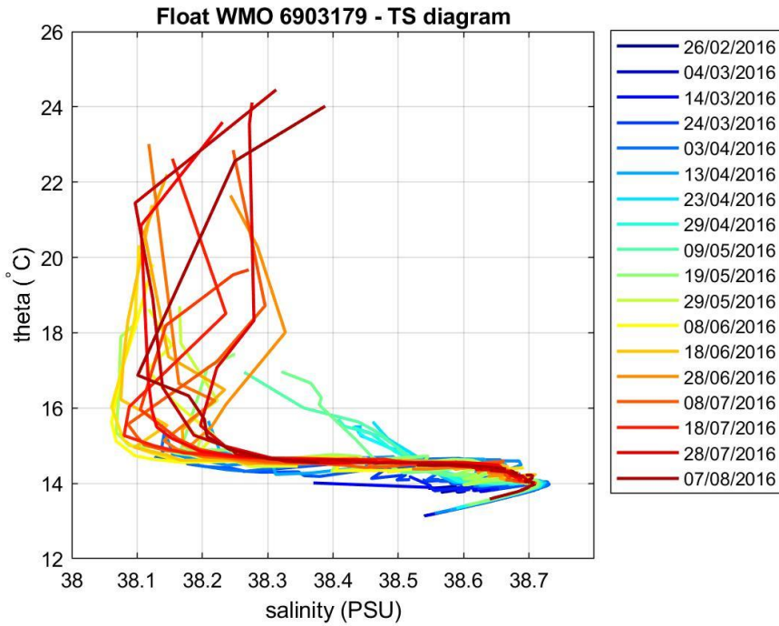
Figure 4: Float 6903179. \theta -S diagram color-coded per cycle number.
