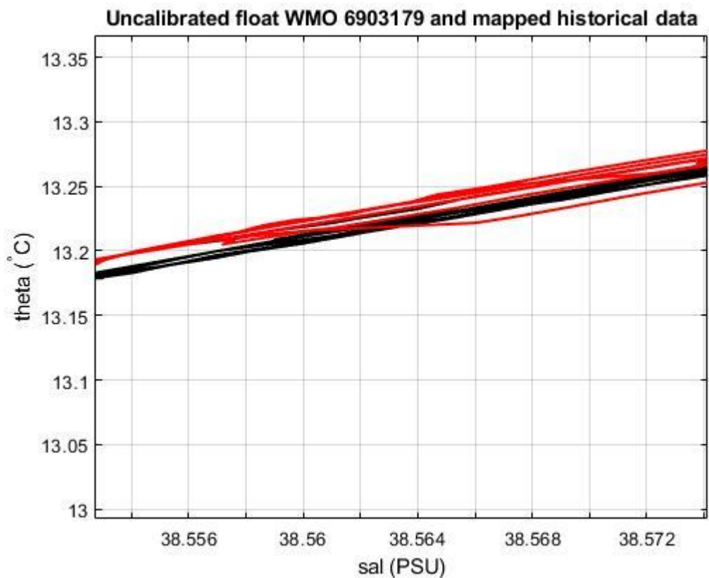
Figure 19: Float 6903179. Uncalibrated float salinity profile (black lines) and mapped historical data (red lines) in the most uniform part of the \theta -S curve.
