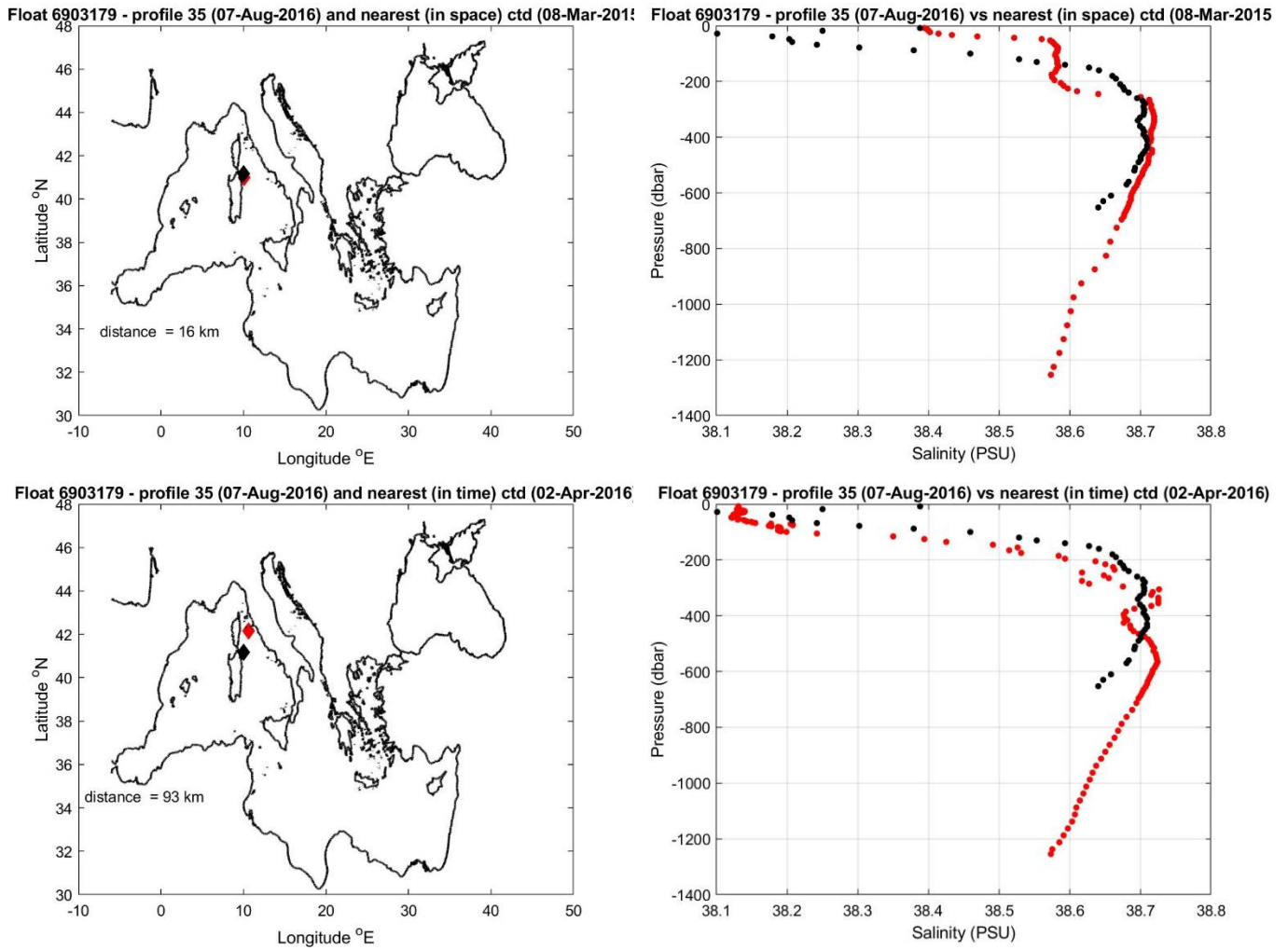
Figure 11: Float 6903179. The salinity float profile number 35 (black dots) are compared to the nearest in space (top) and in time (bottom) reference profile (red dots). The locations of the two profiles and their distance is given in the left panel.
