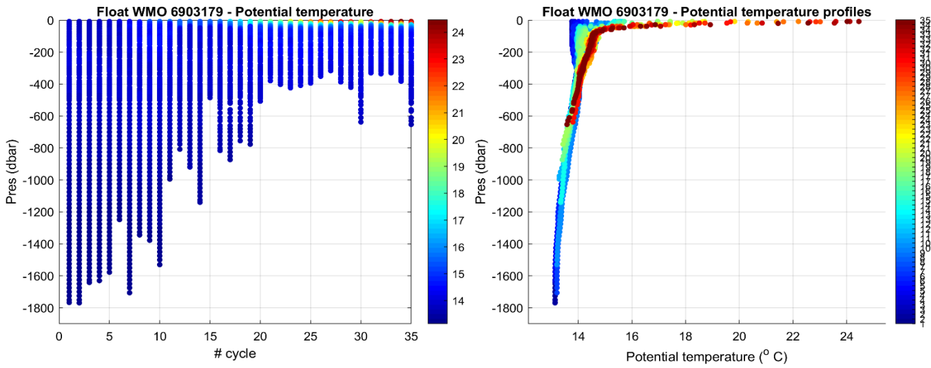
Figure 2: Float 6903179. Time series of Argo float potential temperature ( ^{\circ}\text{C} ) on the left, and potential temperature profiles color-coded per cycle number on the right.
