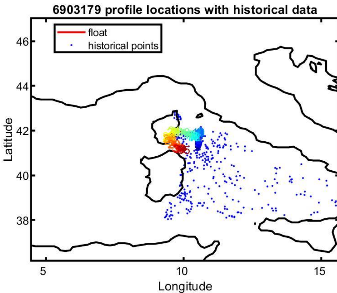
Figure 13: Float 6903179. Location of the float profiles (red line with colored numbers) and the reference data selected for mapping (blue dots).
