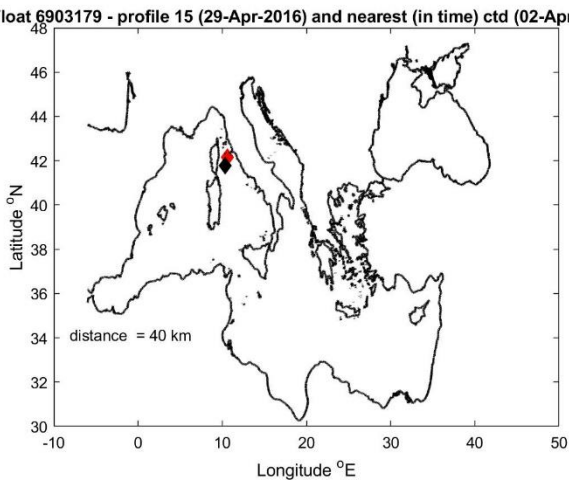
Figure 10: Float 6903179. The salinity float profile number 15 (black dots) are compared to the nearest in space (top) and in time (bottom) reference profile (red dots). The locations of the two profiles and their distance is given in the left panel.
