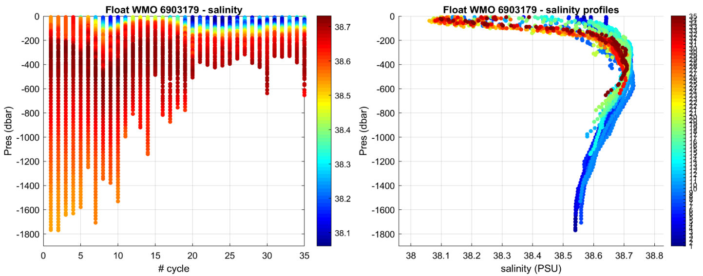
Figure 3: Float 6903179. Time series of Argo float potential salinity (PSS-78) on the left, and salinity profiles color-coded per cycle number on the right.
