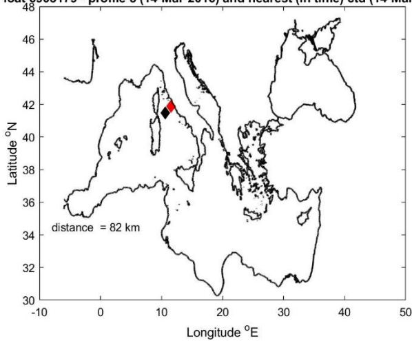
Figure 9: Float 6903179. The salinity float profile number 5 (black dots) are compared to the nearest in space (top) and in time (bottom) reference profile (red dots). The locations of the two profiles and their distance is given in the left panel.
