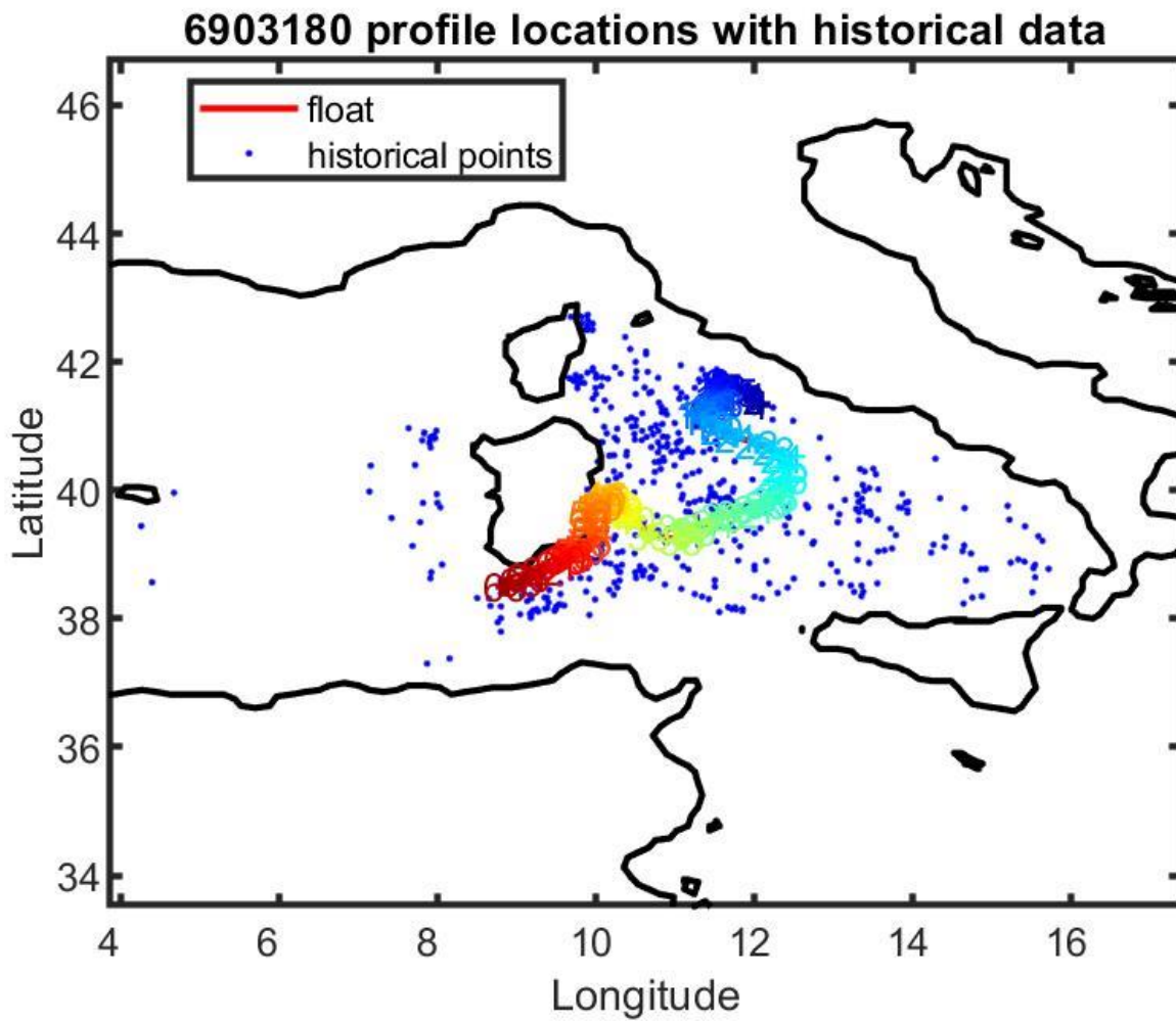
Figure 13: Float 6903180. Location of the float profiles (red line with colored numbers) and the reference data selected for mapping (blue dots).
