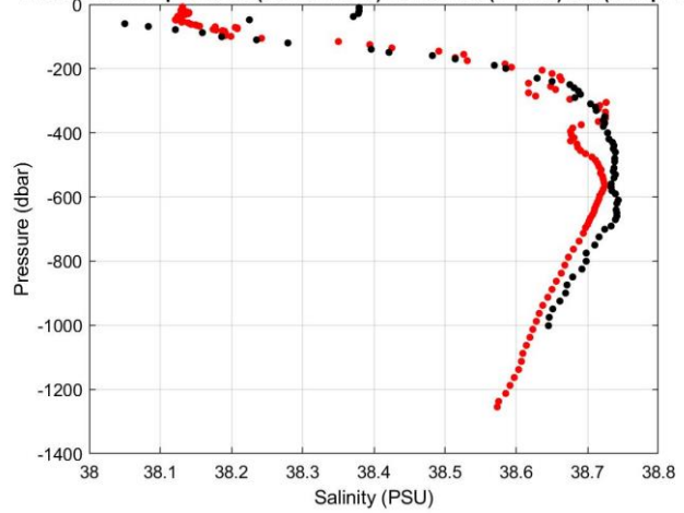
Float 6903180 - profile 33 (05-Nov-2016) vs nearest (in time) ctd (02-Apr-2016)
