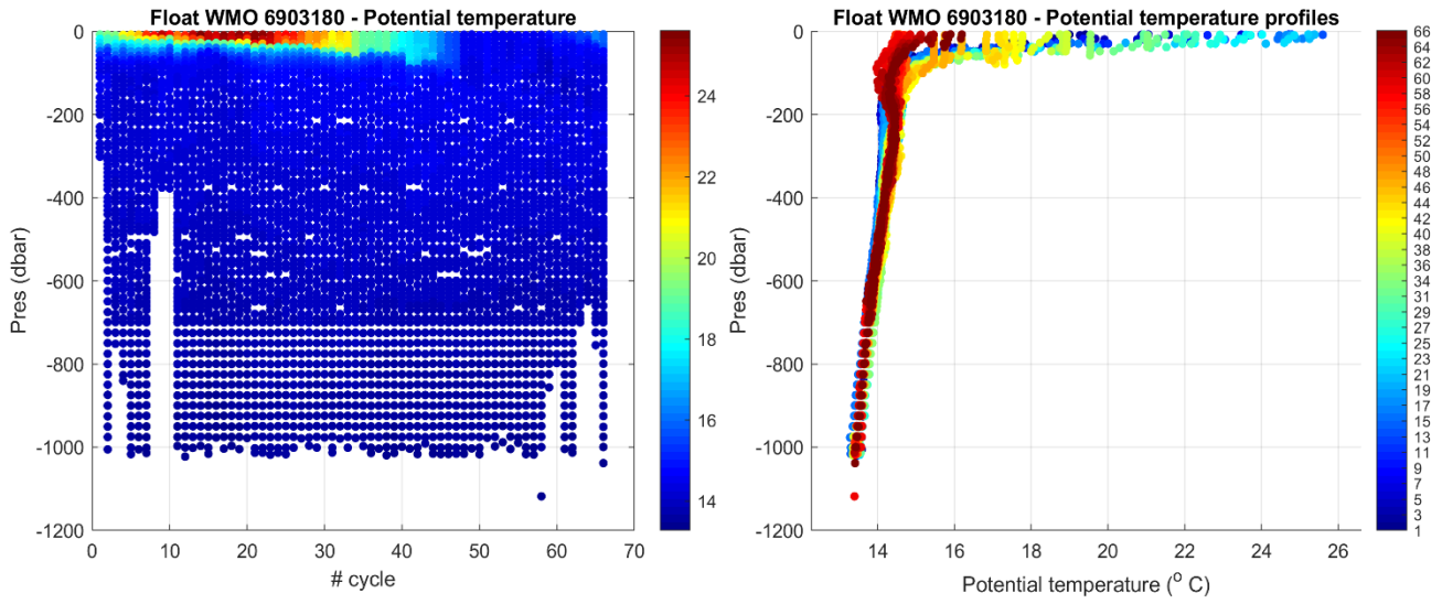
Figure 2: Float 6903180. Time series of Argo float potential temperature ( ^{\circ}\text{C} ) on the left, and potential temperature profiles color-coded per cycle number on the right.
