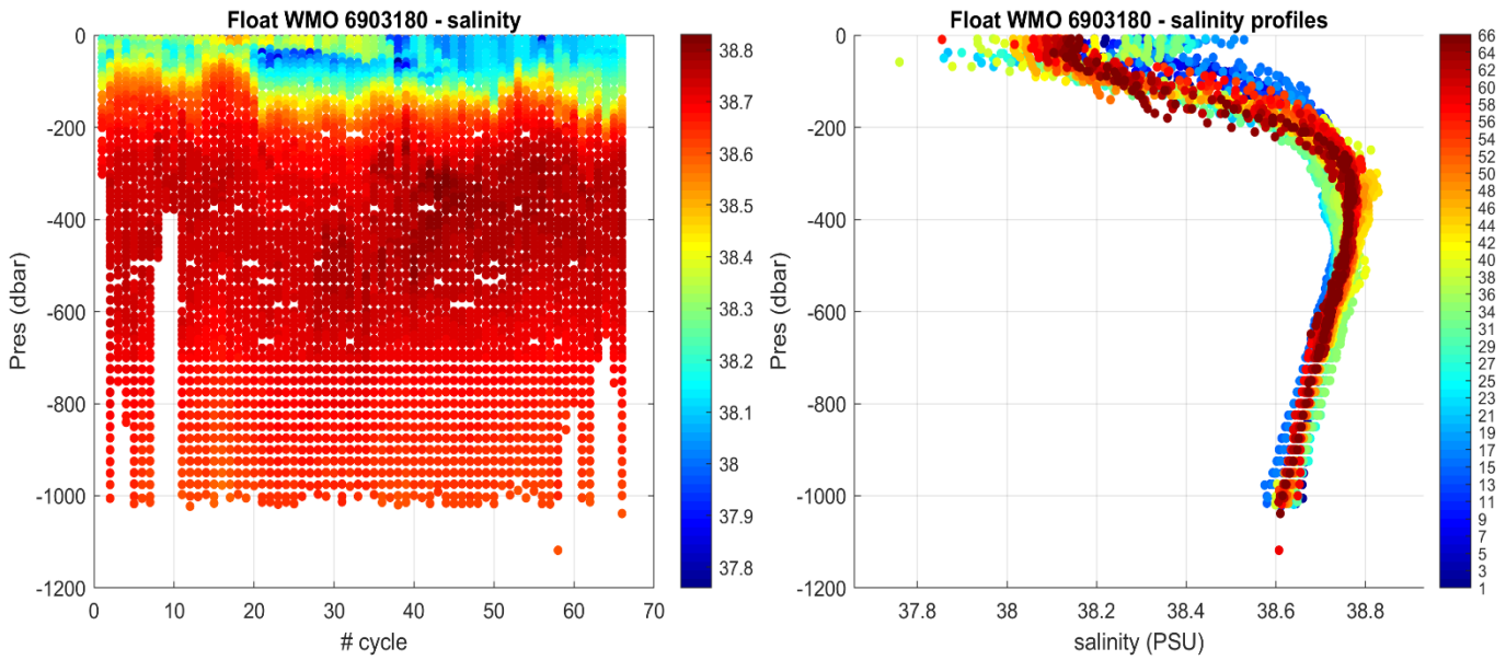
Figure 3: Float 6903180. Time series of Argo float potential salinity (PSS-78) on the left, and salinity profiles color-coded per cycle number on the right.
