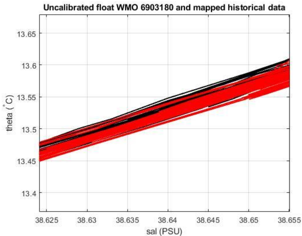
Figure 19: Float 6903180. Uncalibrated float salinity profile (black lines) and mapped historical data (red lines) in the most uniform part of the \theta -S curve.
