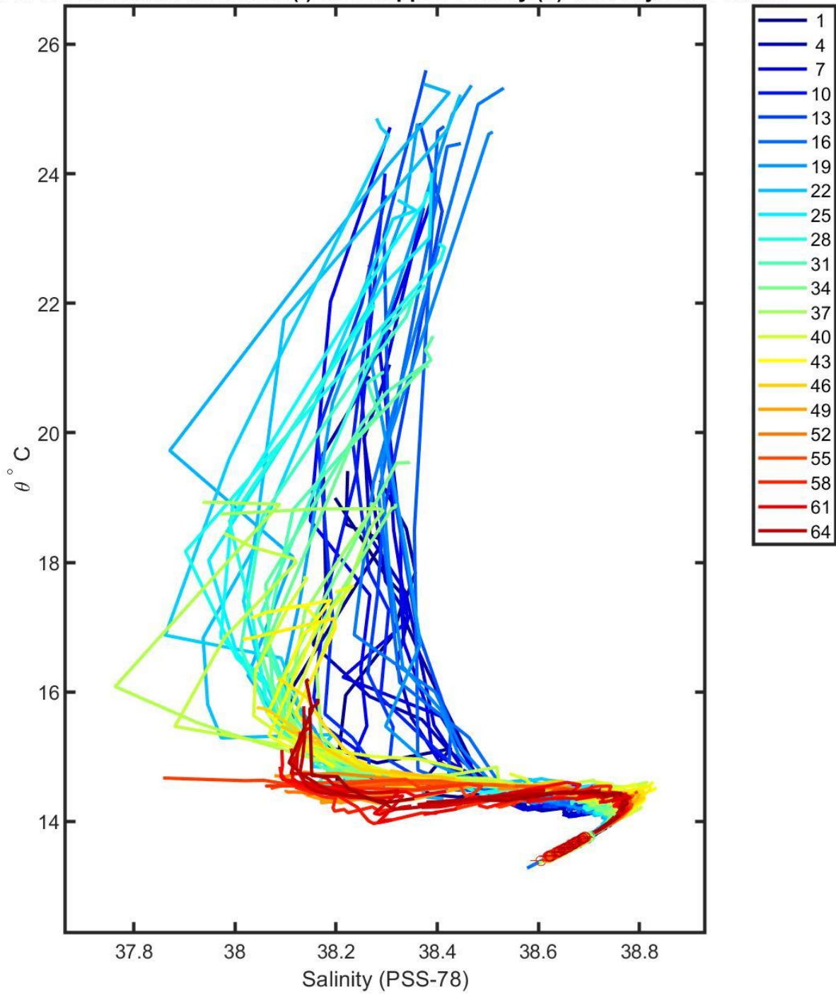
6903180 calibrated float data (-) and mapped salinity (o) with objective errors
