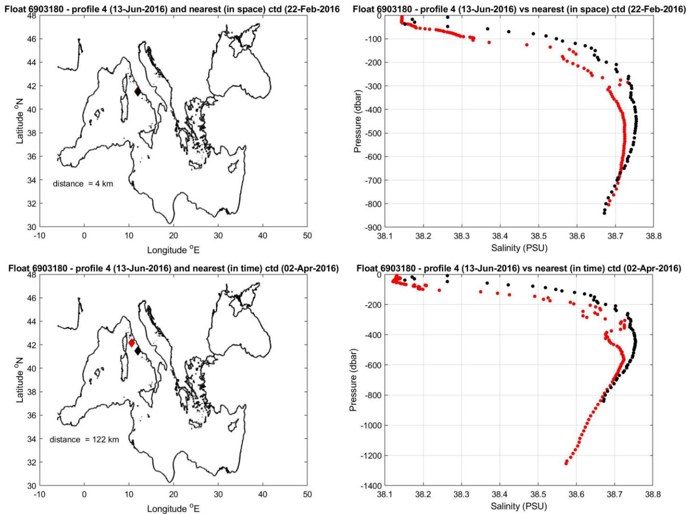
Figure 9: Float 6903180. The salinity float profile number 4 (black dots) are compared to the nearest in space (top) and in time (bottom) reference profile (red dots). The locations of the two profiles and their distance is given in the left panel.
