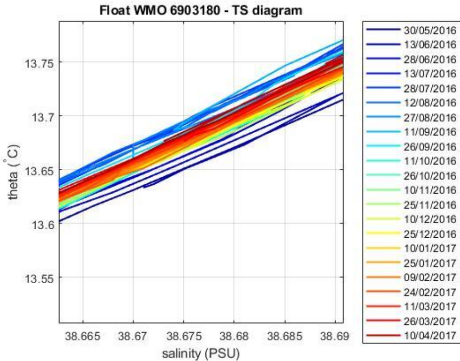
Figure 4: Float 6903180. \theta -S diagram color-coded per cycle number.
