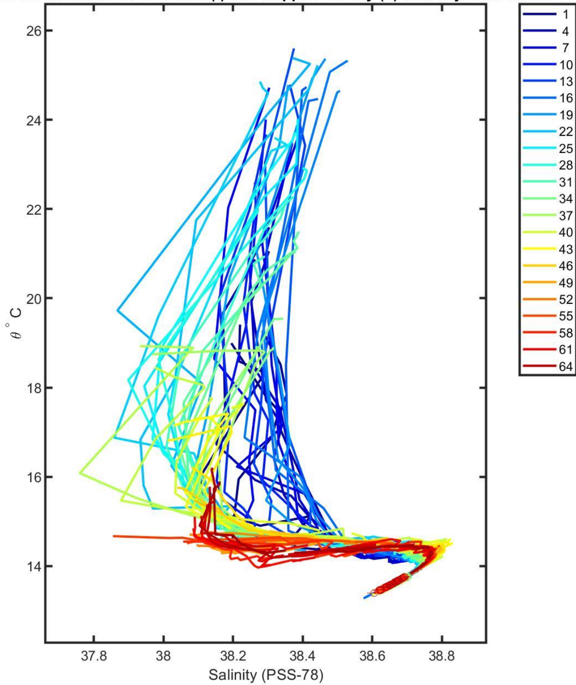
6903180 uncalibrated float data (-) and mapped salinity (o) with objective errors
