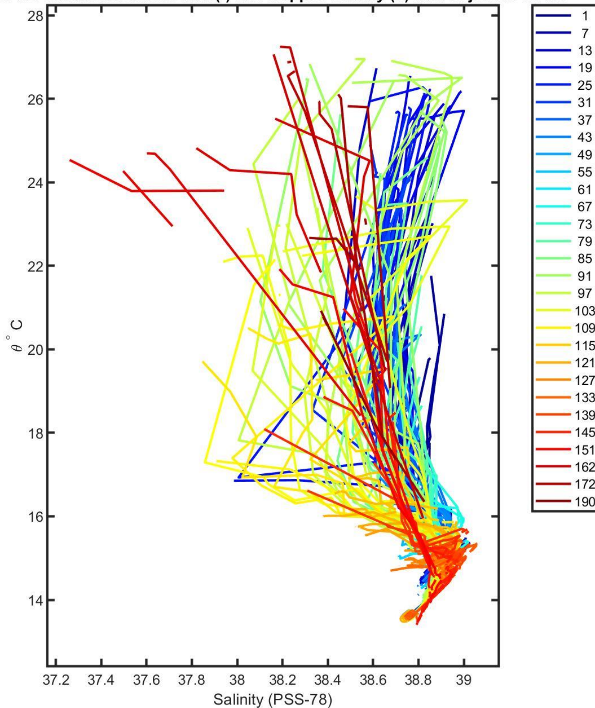
6903196 uncalibrated float data (-) and mapped salinity (o) with objective errors
