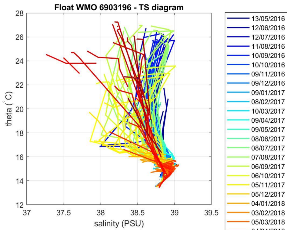
Figure 4: Float 6903196. \theta -S diagram color-coded per cycle number.
