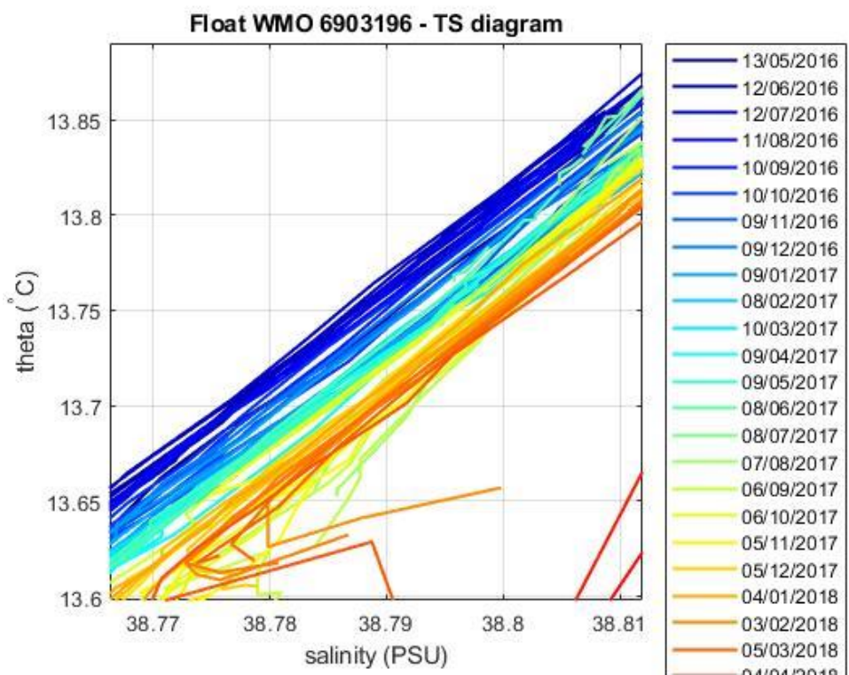
Figure 5: Float 6903196. Area of the \theta -S diagram (color-coded per cycle number) where the \theta -S relationship is more uniform.
