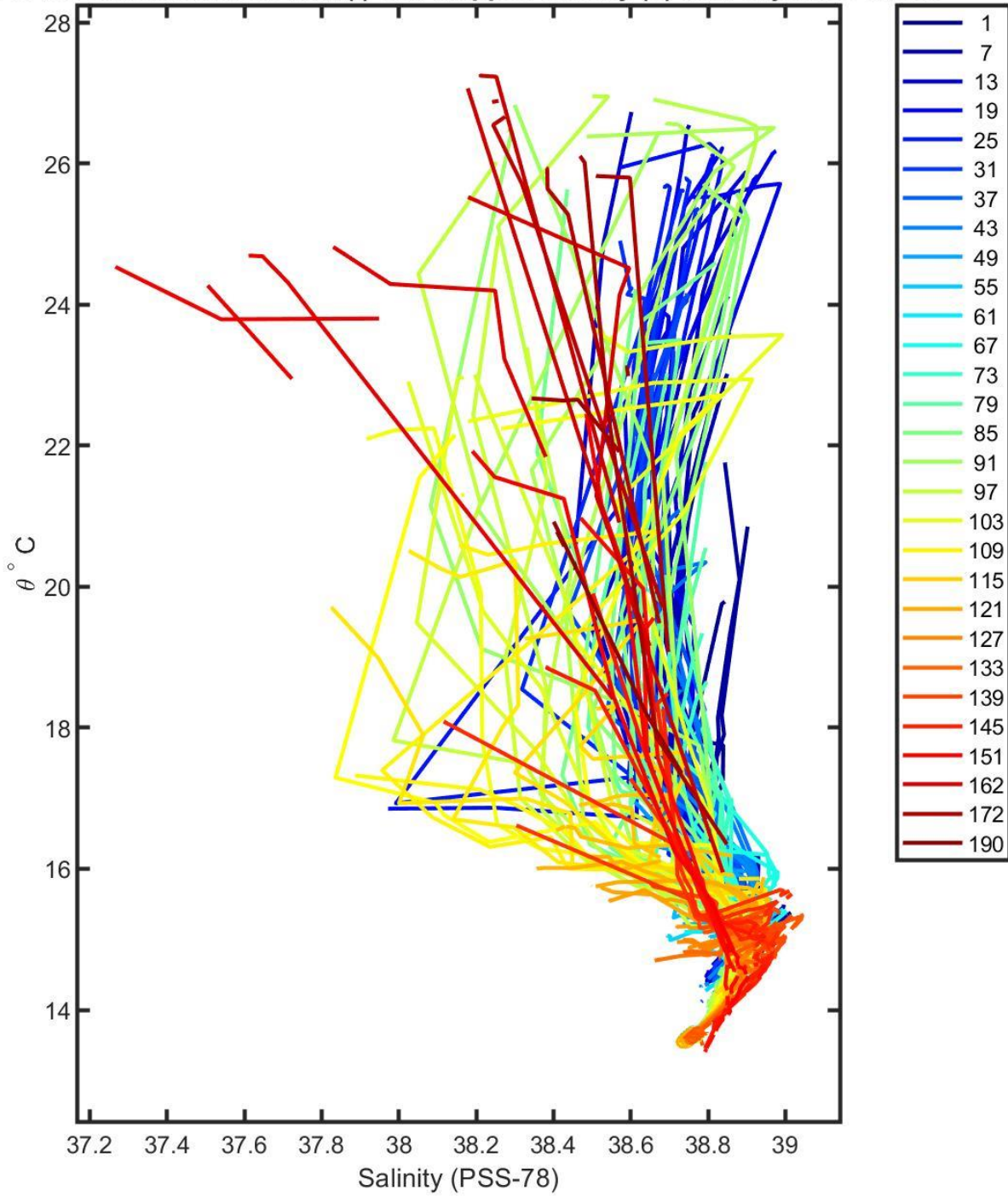
6903196 calibrated float data (-) and mapped salinity (o) with objective errors
