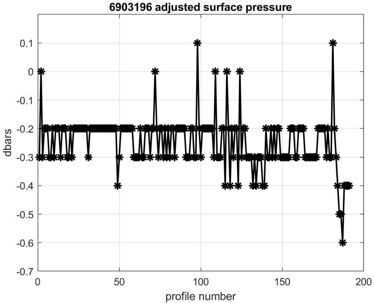
Figure 13: Float 6903196. Adjusted surface pressure values versus profile number.
