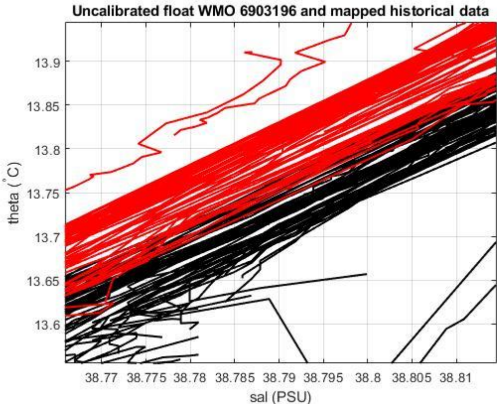
Figure 20: Float 6903196. Uncalibrated float salinity profile (black lines) and mapped historical data (red lines) in the most uniform part of the \theta -S curve.
