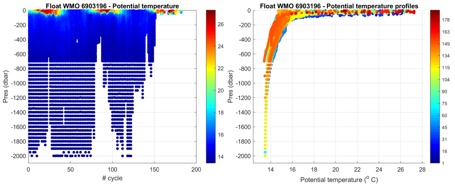
Figure 2: Float 6903196. Time series of Argo float potential temperature ( ^{\circ}\text{C} ) on the left, and potential temperature profiles color-coded per cycle number on the right.
