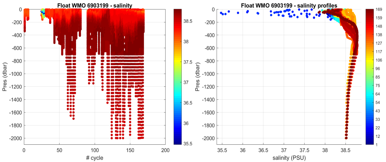
Figure 2: Float 6903199. Time series of Argo float potential salinity (PSS-78) on the left, and salinity profiles color-coded per cycle number on the right.
