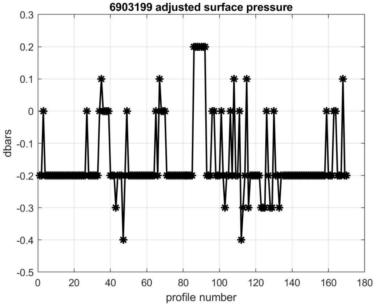
Figure 11: Float 6903199. Adjusted surface pressure values versus profile number.
