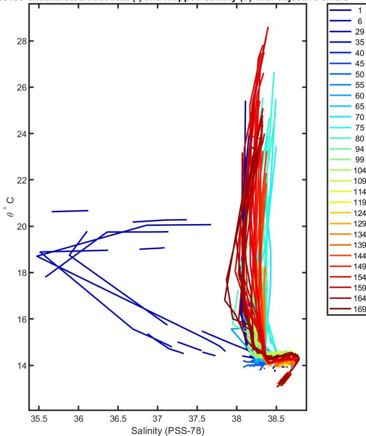
6903199 uncalibrated float data (-) and mapped salinity (o) with objective errors
