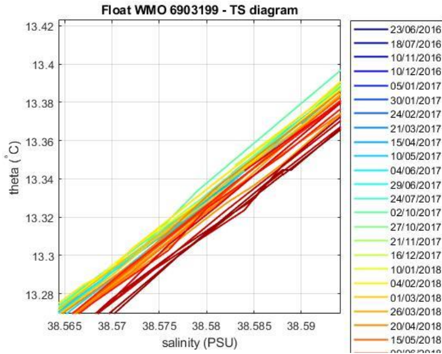
Figure 4: Float 6903199. Area of the \theta -S diagram (color-coded per cycle number) where the \theta -S relationship is more uniform.
