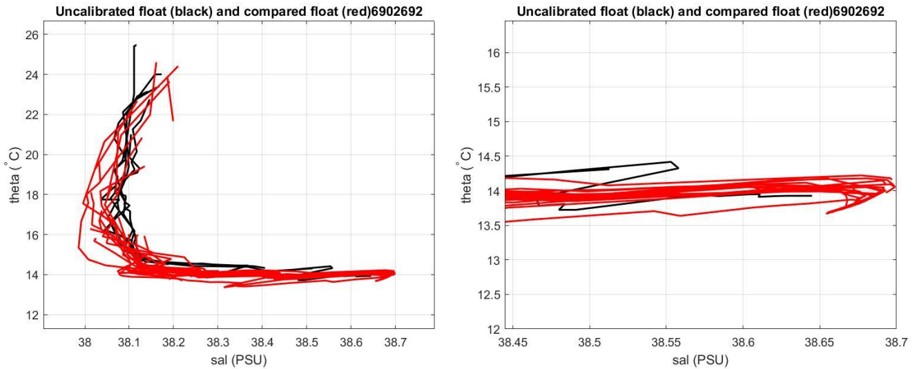
Figure 20: Float 6903199. Comparison between float 6903199 (black line) and 6902692 (red line), in the most uniform part of the \theta -S curve.
