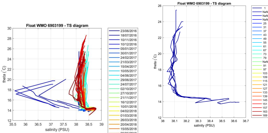
Figure 3: Float 6903199. \theta -S diagram color-coded per cycle number. On the left all profiles have been included, on the right only profile with QC 1.
