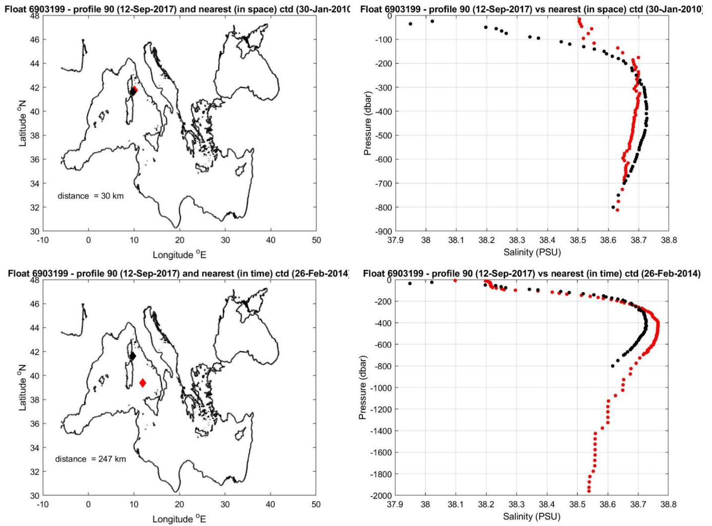
Figure 9: Float 6903199. The salinity float profile number 90 (black dots) are compared to the nearest in space (top) and in time (bottom) reference profile (red dots). The locations of the two profiles and their distance is given in the left panel.
