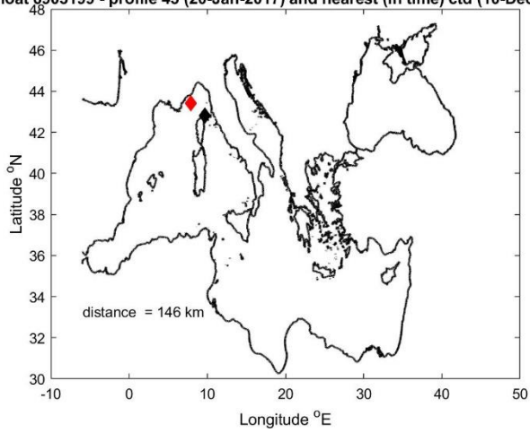
Float 6903199 - profile 43 (20-Jan-2017) and nearest (in time) ctd (10-Dec-2013)
