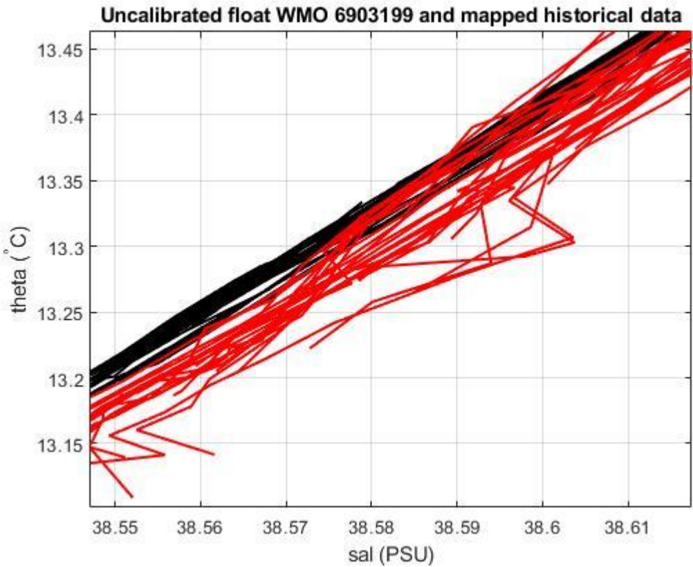
Figure 18: Float 6903199. Uncalibrated float salinity profile (black lines) and mapped historical data (red lines) in the most uniform part of the \theta -S curve.
