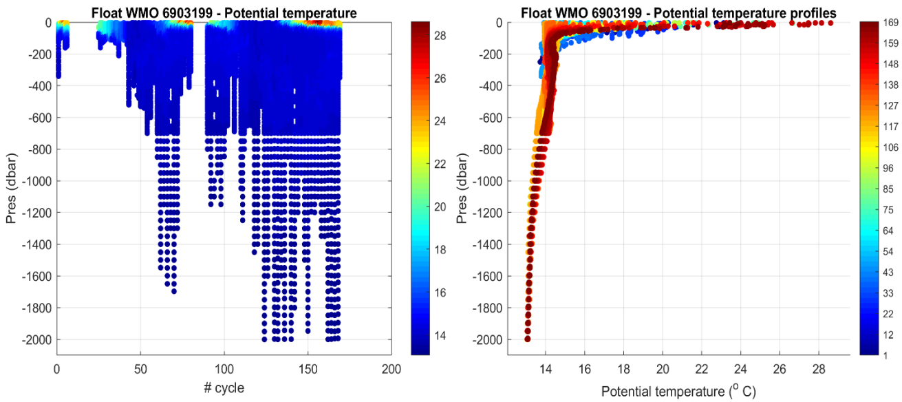
Figure 1: Float 6903199. Time series of Argo float potential temperature ( ^{\circ}\text{C} ) on the left, and potential temperature profiles color-coded per cycle number on the right.
