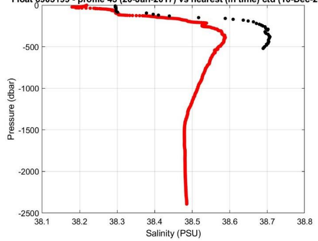
Float 6903199 - profile 43 (20-Jan-2017) vs nearest (in time) ctd (10-Dec-2013)
