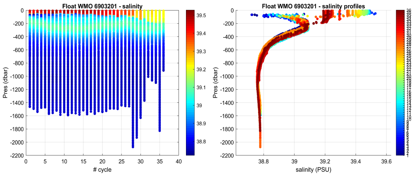
Figure 3: Float 6903201. Time series of Argo float potential salinity (PSS-78) on the left, and salinity profiles color-coded per cycle number on the right.
