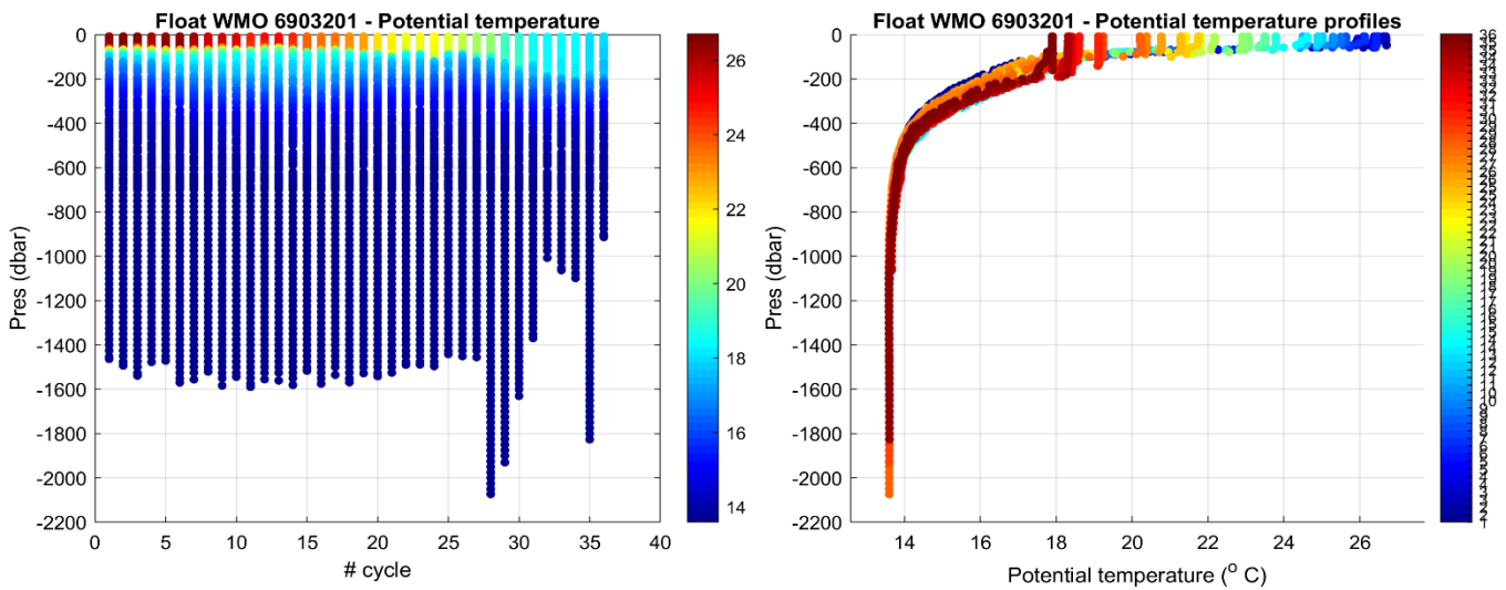
Figure 2: Float 6903201. Time series of Argo float potential temperature ( ^{\circ}\text{C} ) on the left, and potential temperature profiles color-coded per cycle number on the right.
