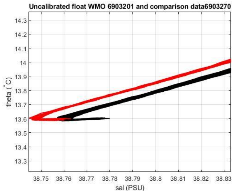
Figure 20: Float 6903201. Uncalibrated float salinity profile (black lines) and compared float data (red lines) in the most uniform part of the \theta -S curve.
