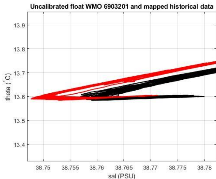
Figure 19: Float 6903201. Uncalibrated float salinity profile (black lines) and mapped historical data (red lines) in the most uniform part of the \theta -S curve.
