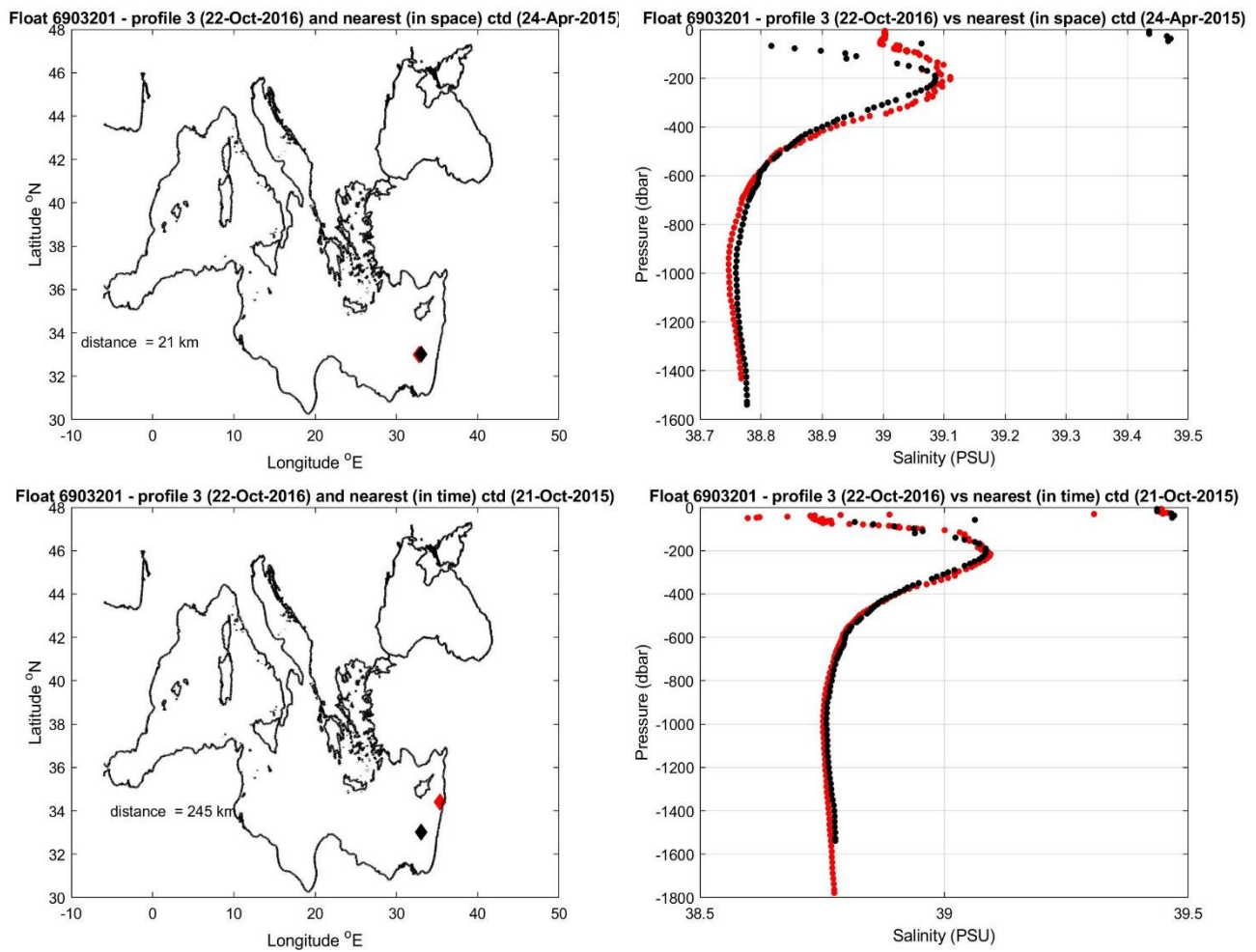
Figure 9: Float 6903201. The salinity float profile number 3 (black dots) are compared to the nearest in space (top) and in time (bottom) reference profile (red dots). The locations of the two profiles and their distance is given in the left panel.
