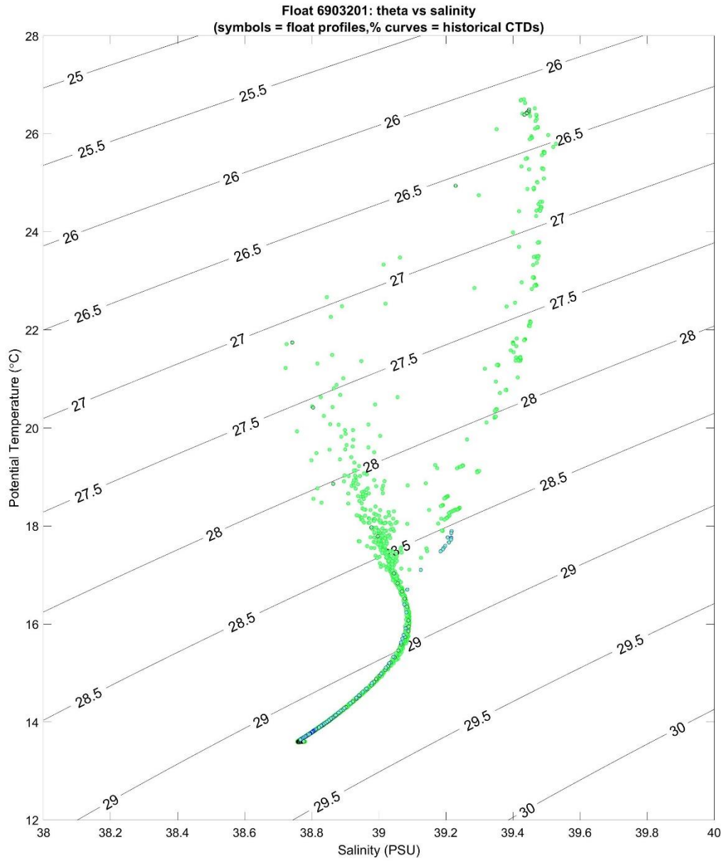
Figure 12: Float 6903201. T/S diagram plotted with and data from WMO boxes of CTD reference data +/- 10° of latitude and longitude. The black and blue cycles indicate the first and the last Argo profile, respectively. Green symbols represent other Argo profiles from this float. The thin colour lines indicate the reference data.
