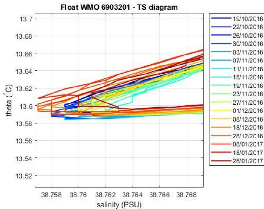
Figure 4: Float 6903201. \theta -S diagram color-coded per cycle number.
