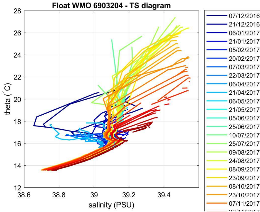
Figure 4: Float 6903204. \theta -S diagram color-coded per cycle number.
