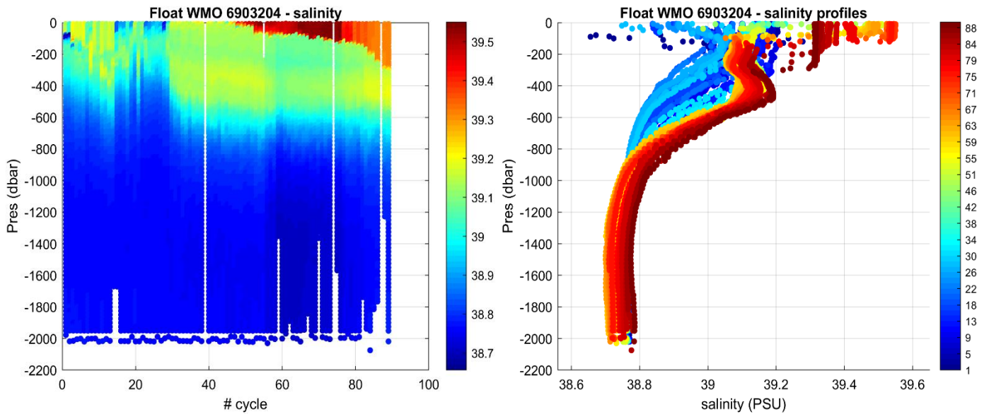
Figure 3: Float 6903204. Time series of Argo float potential salinity (PSS-78) on the left, and salinity profiles color-coded per cycle number on the right.
