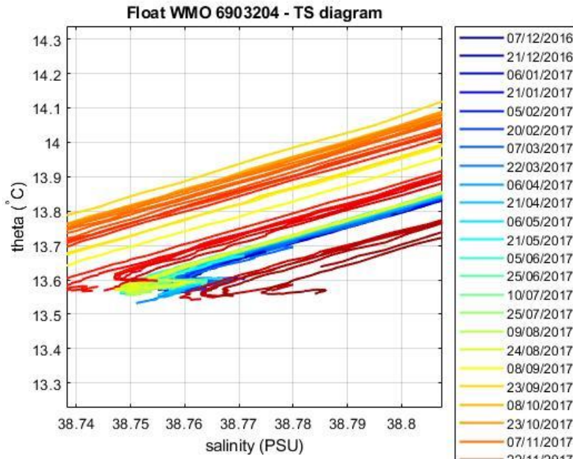
Figure 5: Float 6903204. Area of the \theta -S diagram (color-coded per cycle number) where the \theta -S relationship is more uniform.
