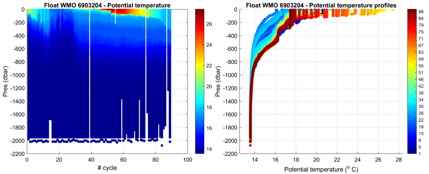
Figure 2: Float 6903204. Time series of Argo float potential temperature ( ^{\circ}\text{C} ) on the left, and potential temperature profiles color-coded per cycle number on the right.
