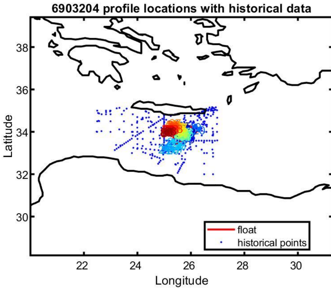
Figure 13: Float 6903204. Location of the float profiles (red line with colored numbers) and the reference data selected for mapping (blue dots).
