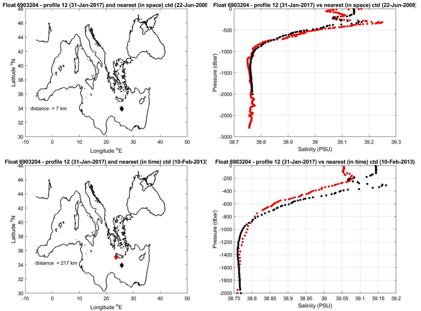
Figure 9: Float 6903204. The salinity float profile number 12 (black dots) are compared to the nearest in space (top) and in time (bottom) reference profile (red dots). The locations of the two profiles and their distance is given in the left panel.
