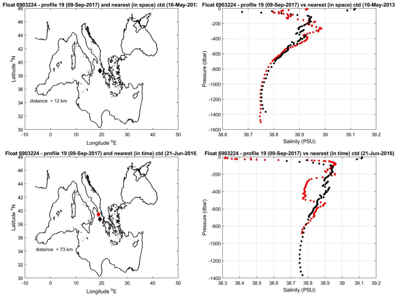
Figure 9: Float 6903224. The salinity float profile number 19 (black dots) are compared to the nearest in space (top) and in time (bottom) reference profile (red dots). The locations of the two profiles and their distance is given in the left panel.
