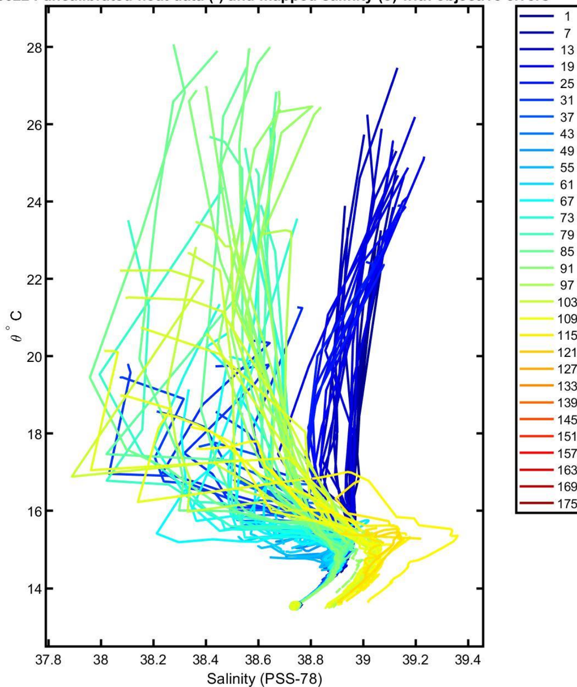
6903224 uncalibrated float data (-) and mapped salinity (o) with objective errors
