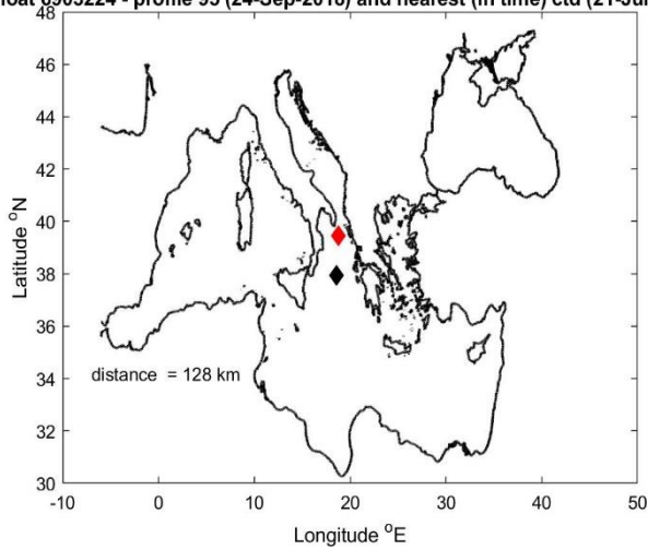
Float 6903224 - profile 95 (24-Sep-2018) and nearest (in time) ctd (21-Jun-2016)
