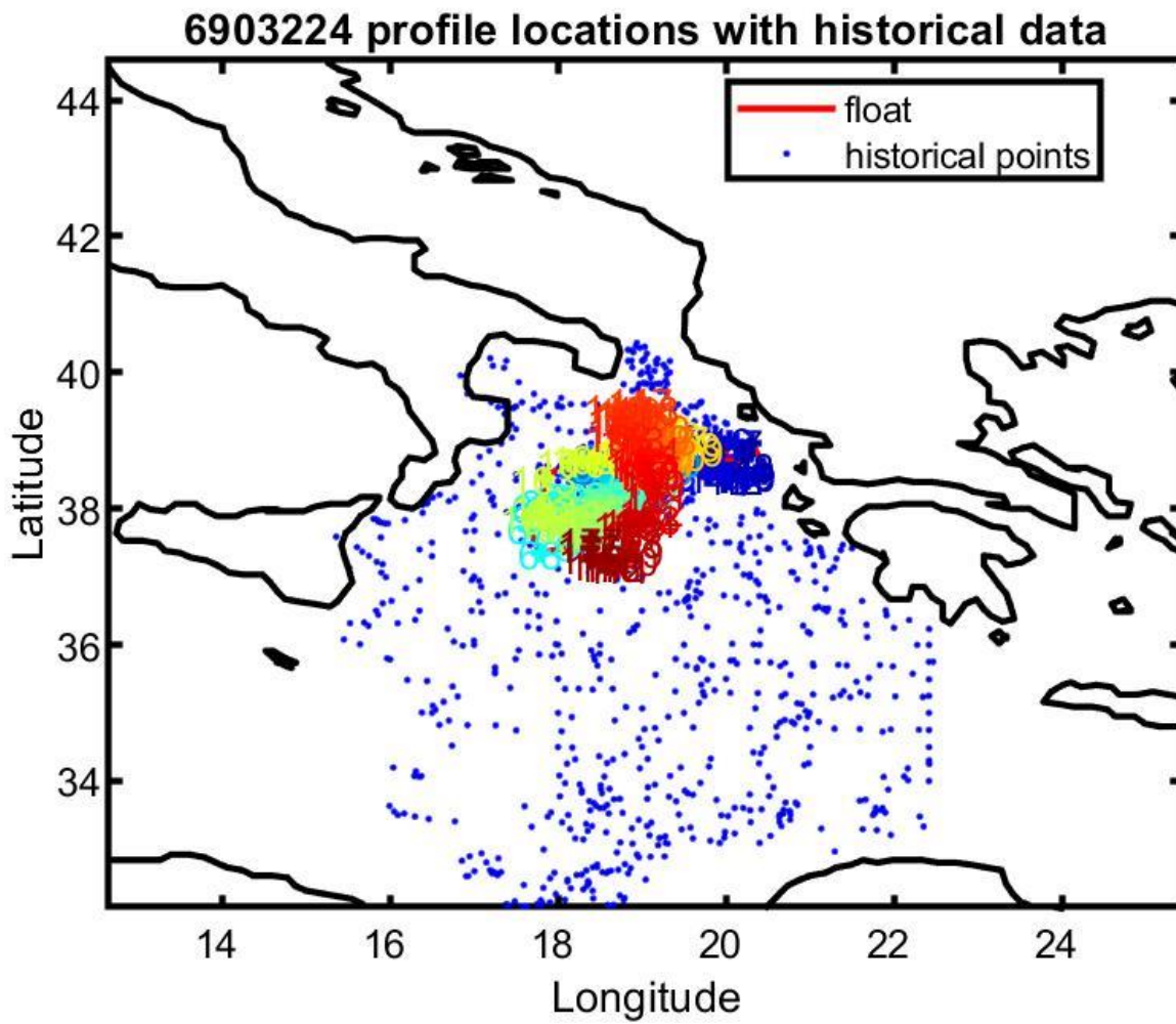
Figure 13: Float 6903224. Location of the float profiles (red line with colored numbers) and the reference data selected for mapping (blue dots).
