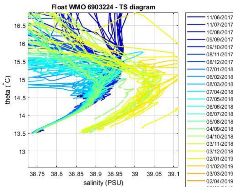
Figure 5: Float 6903224. Area of the \theta -S diagram (color-coded per cycle number) where the \theta -S relationship is more uniform.
