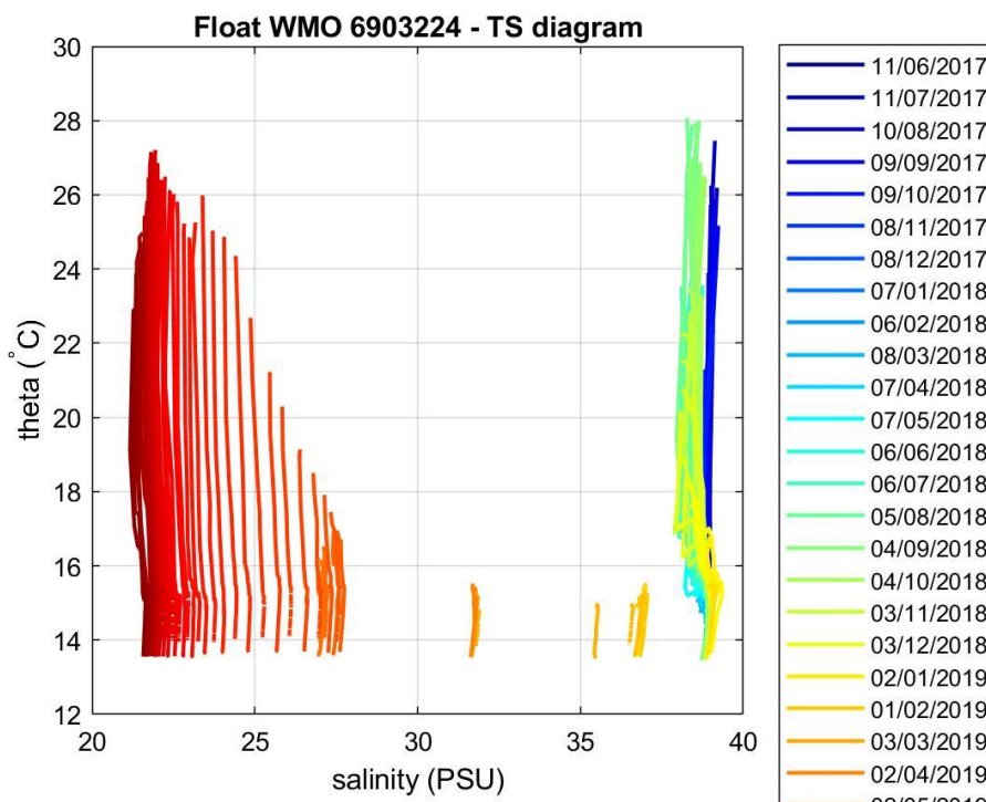
Figure 4: Float 6903224. \theta -S diagram color-coded per cycle number.
