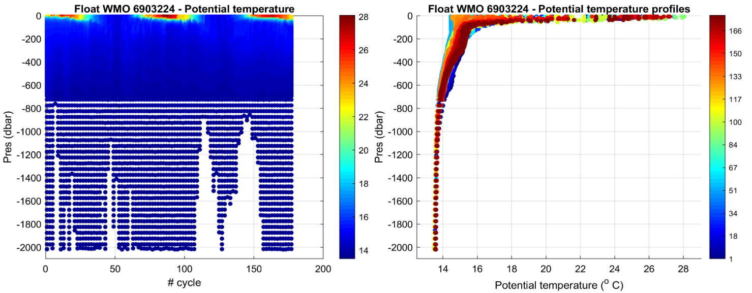
Figure 2: Float 6903224. Time series of Argo float potential temperature ( ^{\circ}\text{C} ) on the left, and potential temperature profiles color-coded per cycle number on the right.
