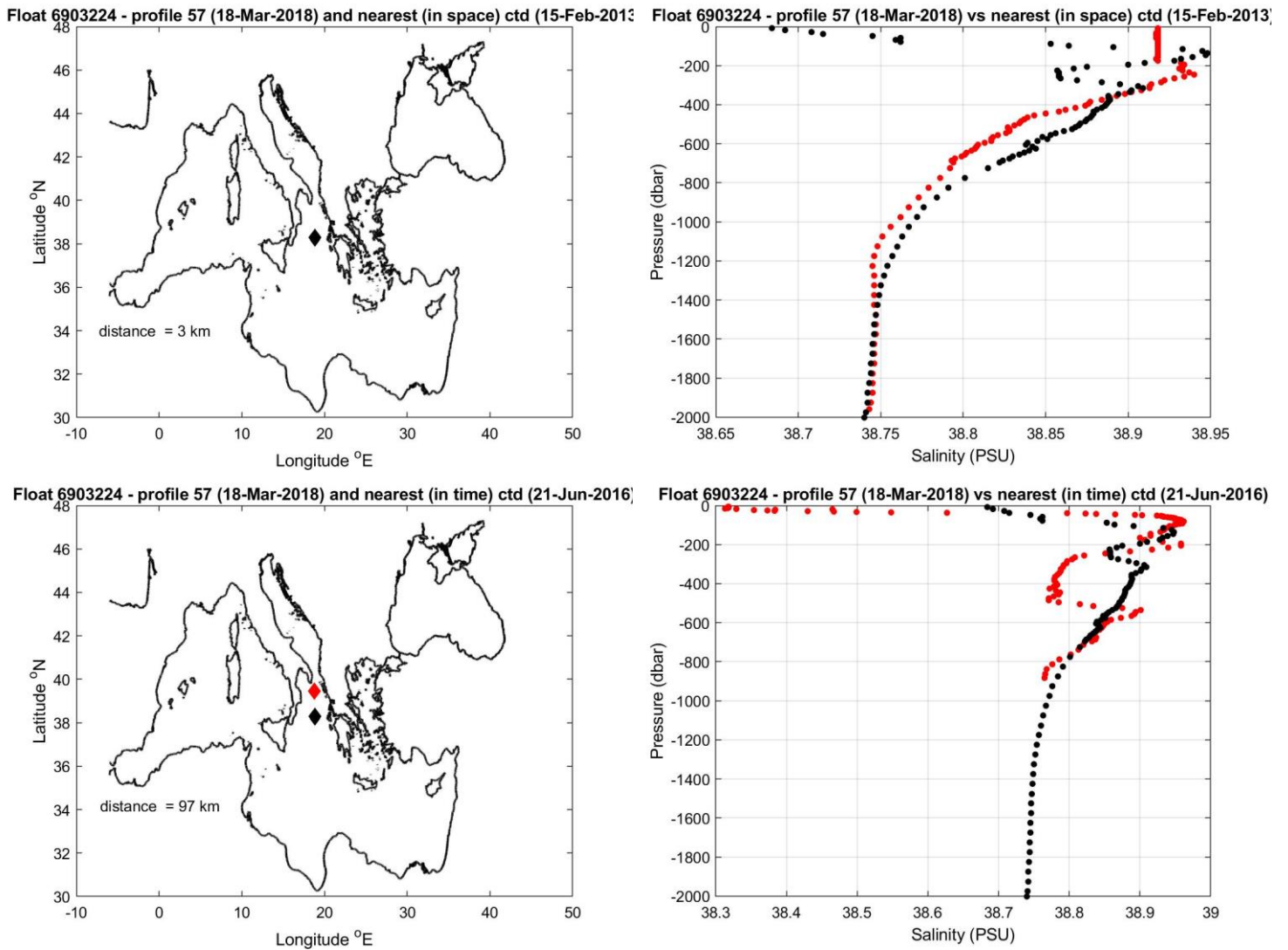
Figure 10: Float 6903224. The salinity float profile number 57 (black dots) are compared to the nearest in space (top) and in time (bottom) reference profile (red dots). The locations of the two profiles and their distance is given in the left panel.
