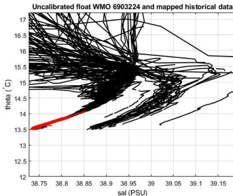
Figure 19: Float 6903224. Uncalibrated float salinity profile (black lines) and mapped historical data (red lines) in the most uniform part of the \theta -S curve.
