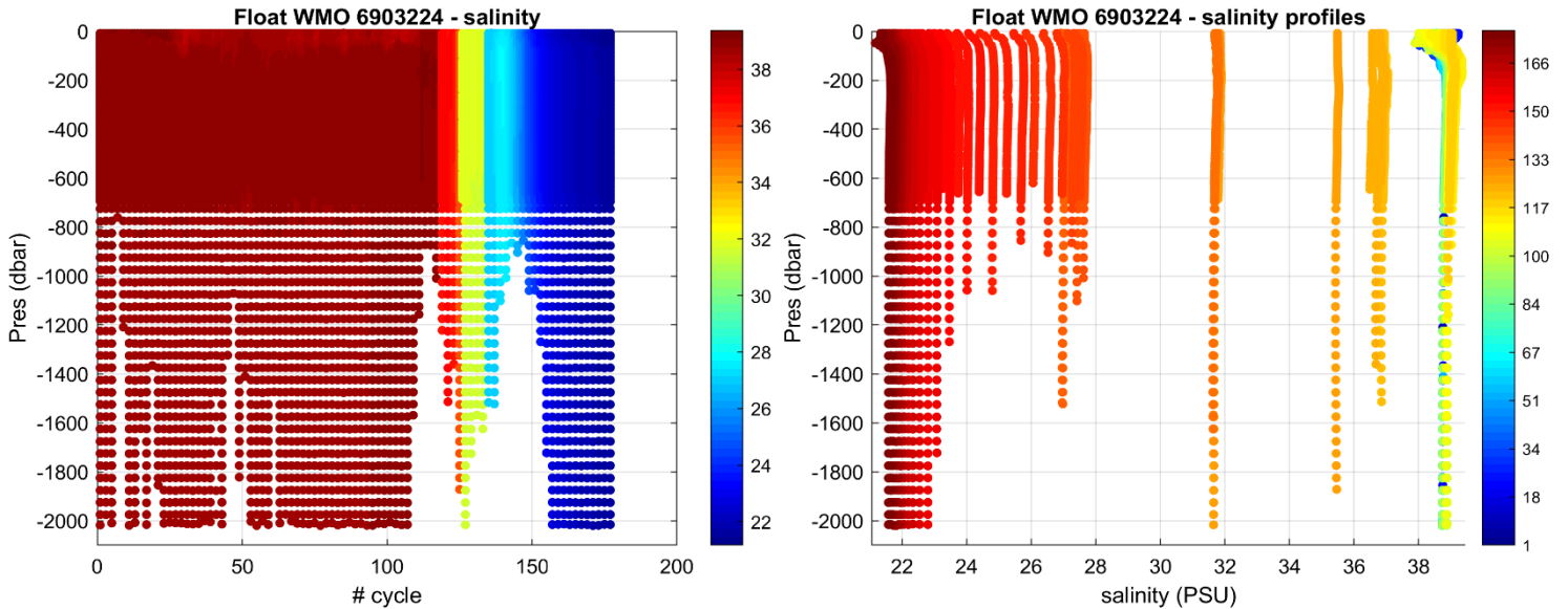
Figure 3: Float 6903224. Time series of Argo float potential salinity (PSS-78) on the left, and salinity profiles color-coded per cycle number on the right.
