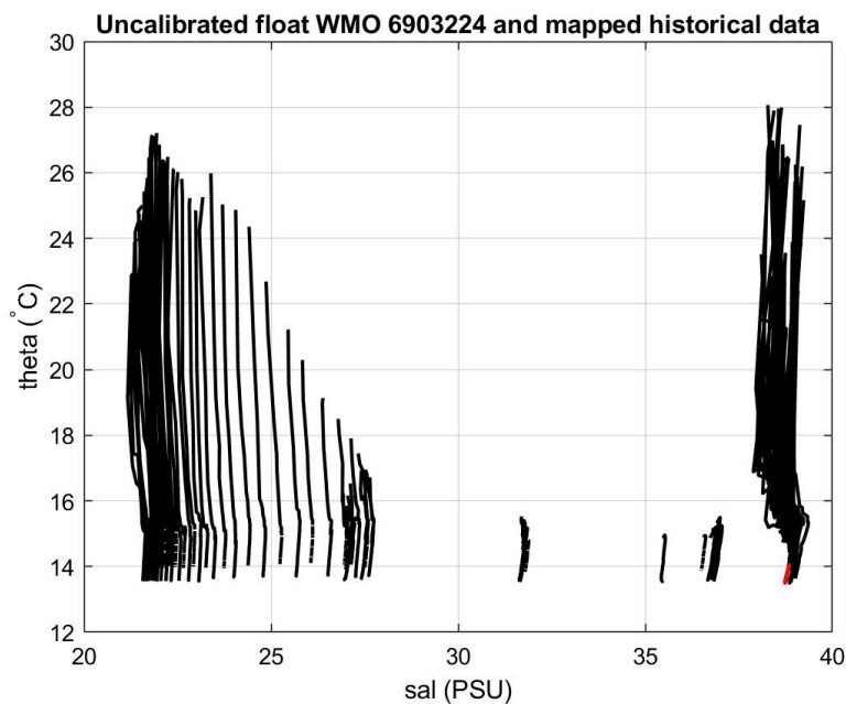
Figure 19: Float 6903224. Uncalibrated float salinity profile (black lines) and mapped historical data (red lines).
