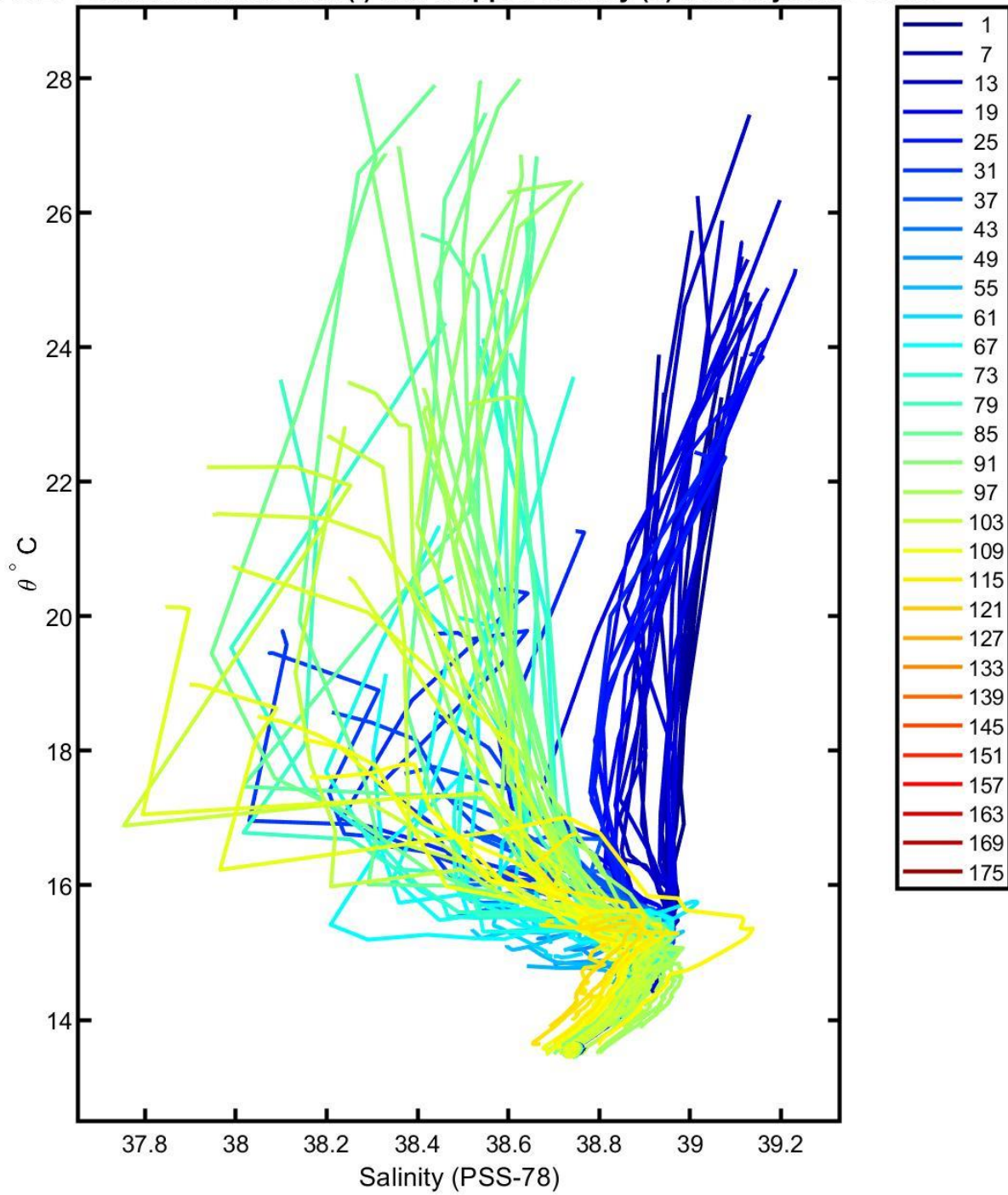
6903224 calibrated float data (-) and mapped salinity (o) with objective errors
