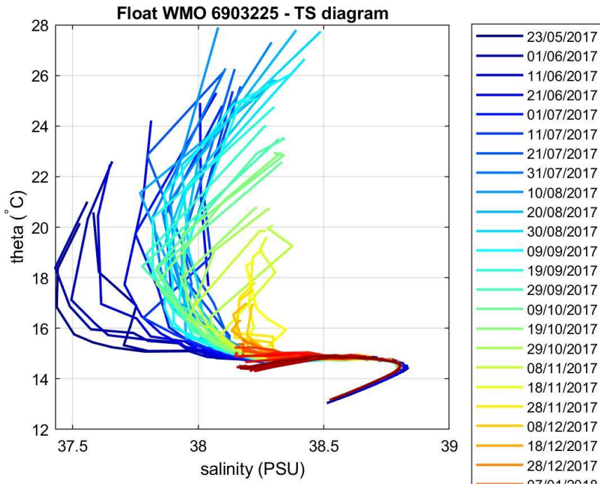
Figure 4: Float 6903225. \theta -S diagram color-coded per cycle number.
