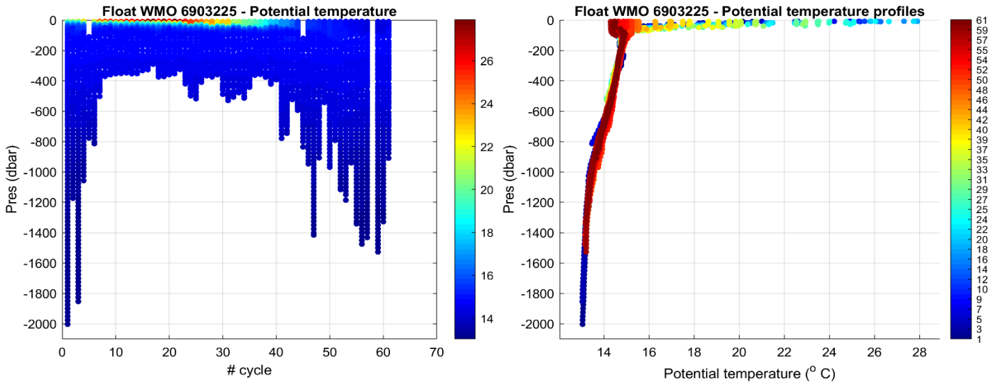
Figure 2: Float 6903225. Time series of Argo float potential temperature (°C) on the left, and potential temperature profiles color-coded per cycle number on the right.
