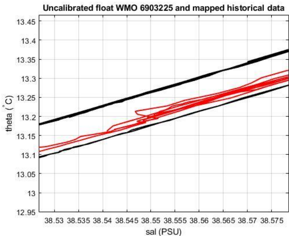
Figure 19: Float 6903225. Uncalibrated float salinity profile (black lines) and mapped historical data (red lines) in the most uniform part of the \theta -S curve.
