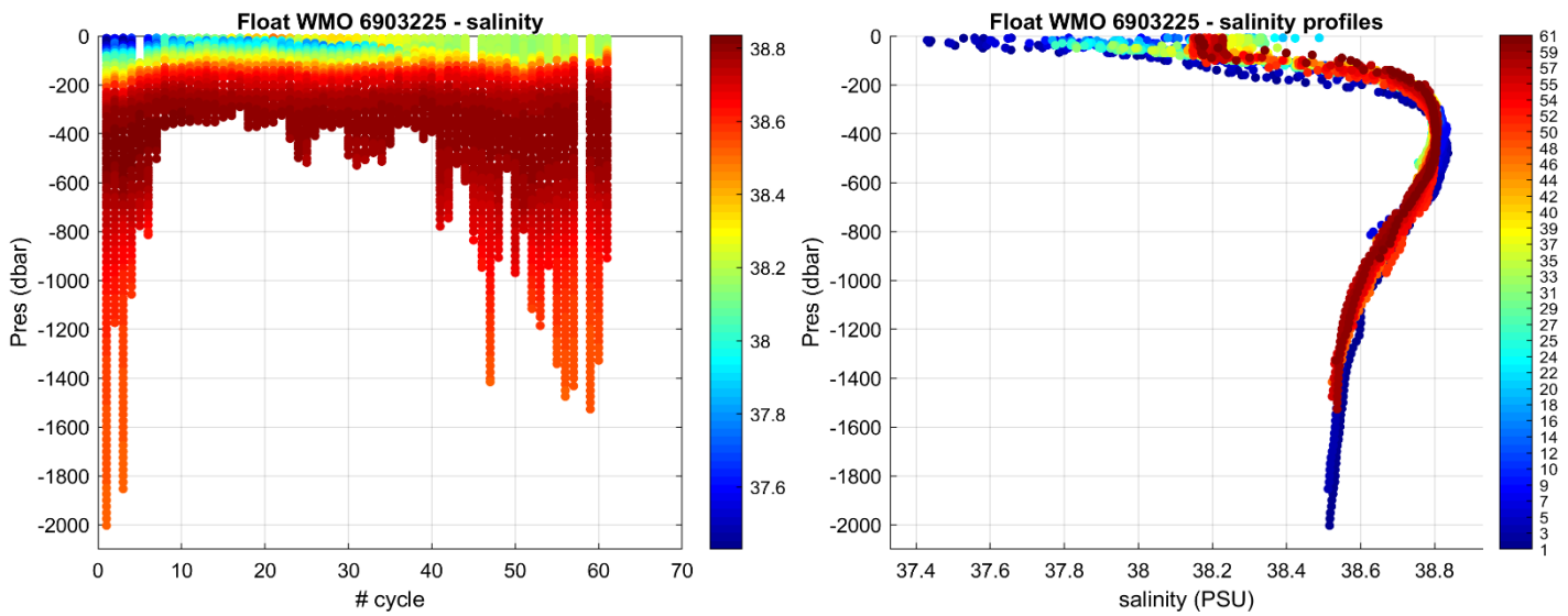
Figure 3: Float 6903225. Time series of Argo float potential salinity (PSS-78) on the left, and salinity profiles color-coded per cycle number on the right.
