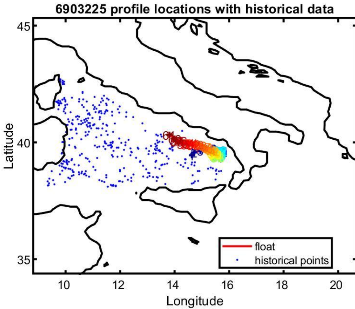
Figure 13: Float 6903225. Location of the float profiles (red line with colored numbers) and the reference data selected for mapping (blue dots).
