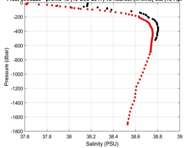
Float 6903225 - profile 43 (18-Dec-2017) vs nearest (in time) ctd (18-Apr-2014)
