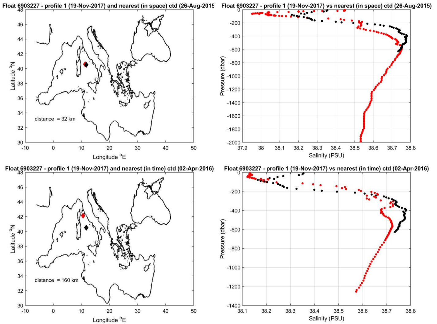
Figure 8: Float 6903227. The salinity float profile number 1 (black dots) are compared to the nearest in space (top) and in time (bottom) reference profile (red dots). The locations of the two profiles and their distance is given in the left panel.
