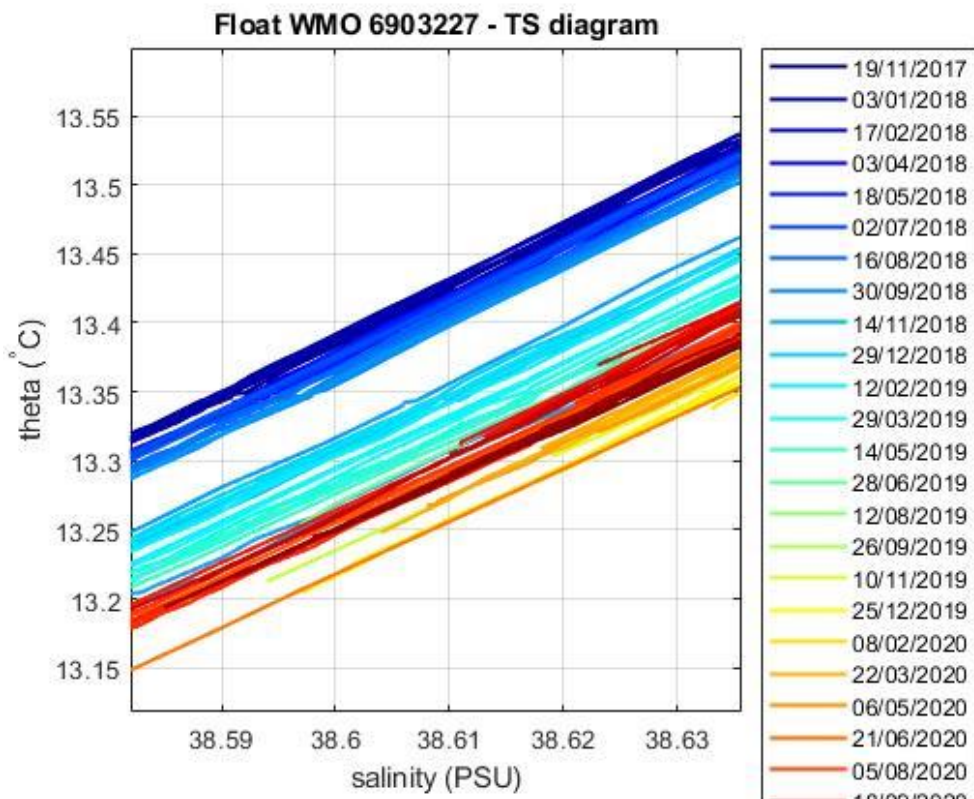
Figure 4: Float 6903227. Area of the \theta -S diagram (color-coded per cycle number) where the \theta -S relationship is more uniform.
