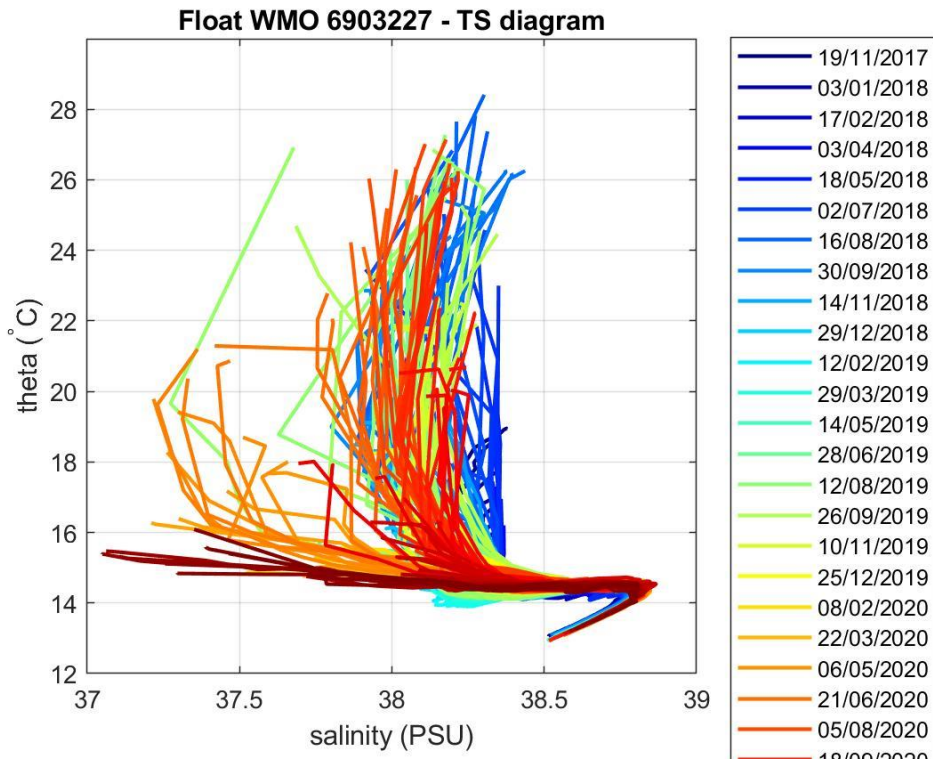
Figure 3: Float 6903227. \theta -S diagram color-coded per cycle number.
