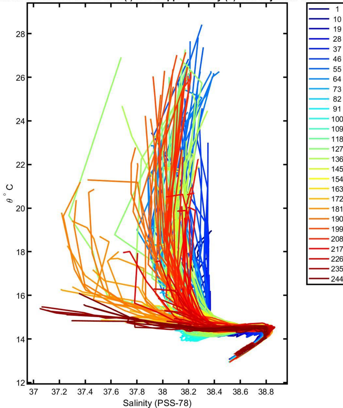
6903227 uncalibrated float data (-) and mapped salinity (o) with objective errors
