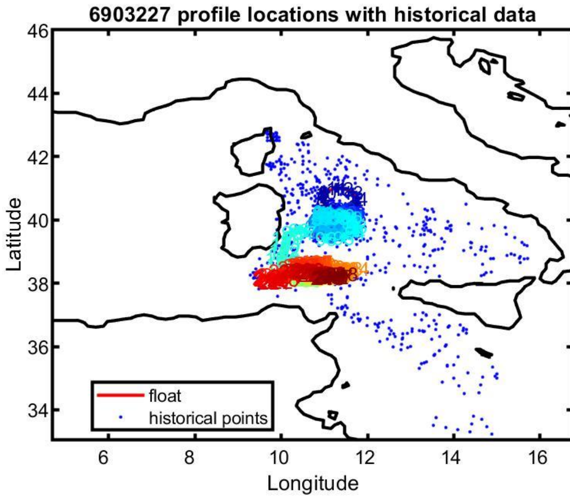
Figure 12: Float 6903227. Location of the float profiles (red line with colored numbers) and the reference data selected for mapping (blue dots).
