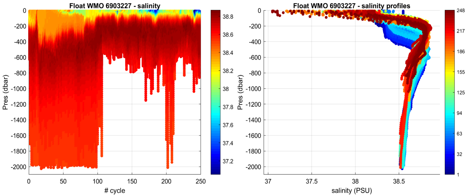
Figure 2: Float 6903227. Time series of Argo float potential salinity (PSS-78) on the left, and salinity profiles color-coded per cycle number on the right.
