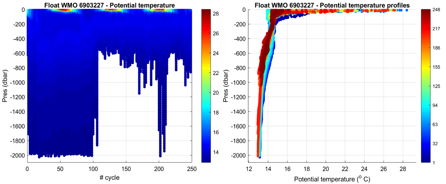
Figure 1: Float 6903227. Time series of Argo float potential temperature ( ^{\circ}\text{C} ) on the left, and potential temperature profiles color-coded per cycle number on the right.
