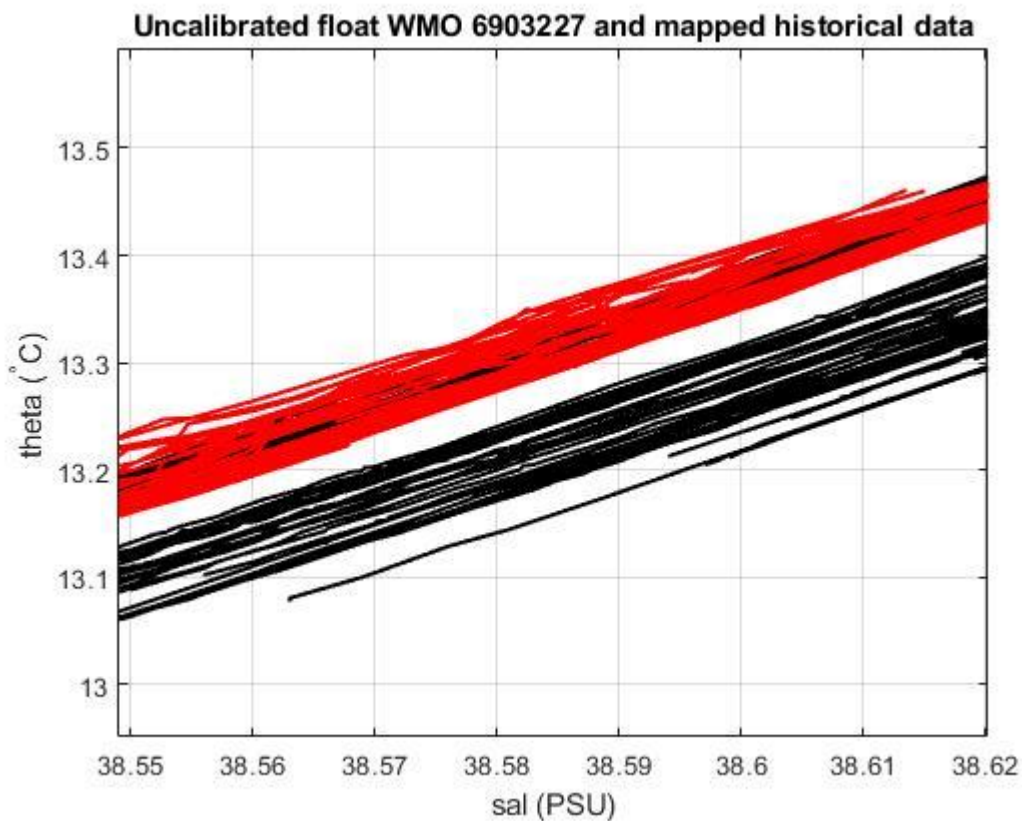
Figure 18: Float 6903227. Uncalibrated float salinity profile (black lines) and mapped historical data (red lines) in the most uniform part of the \theta -S curve.
