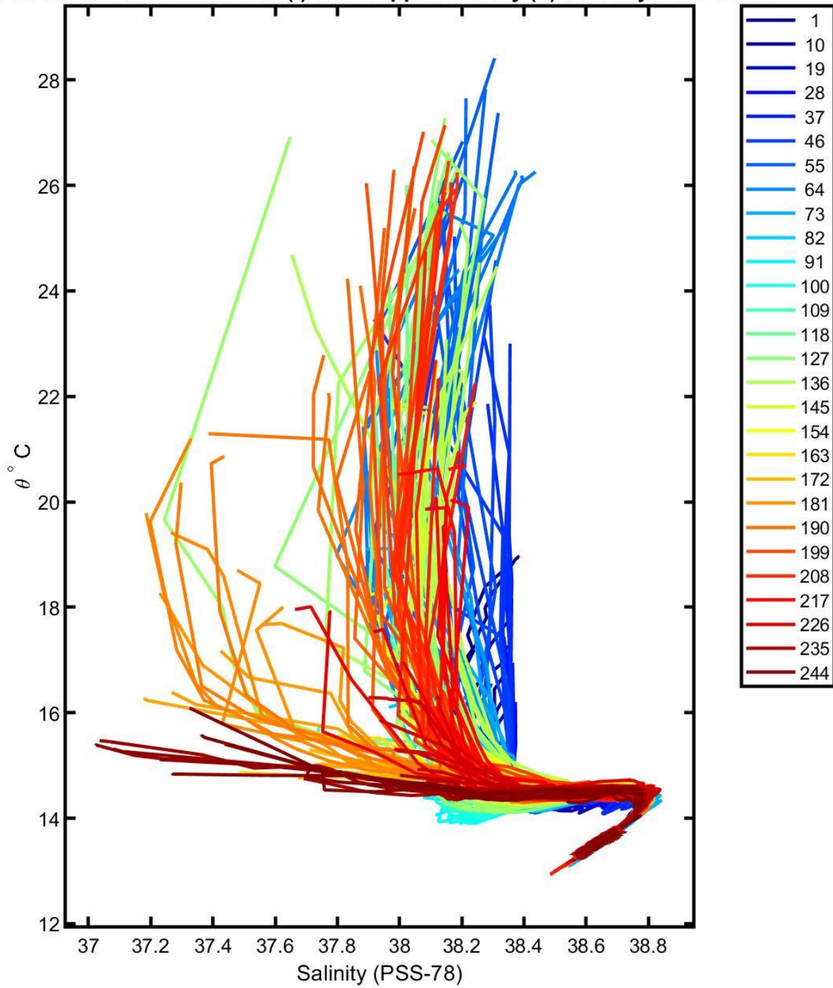
6903227 calibrated float data (-) and mapped salinity (o) with objective errors
