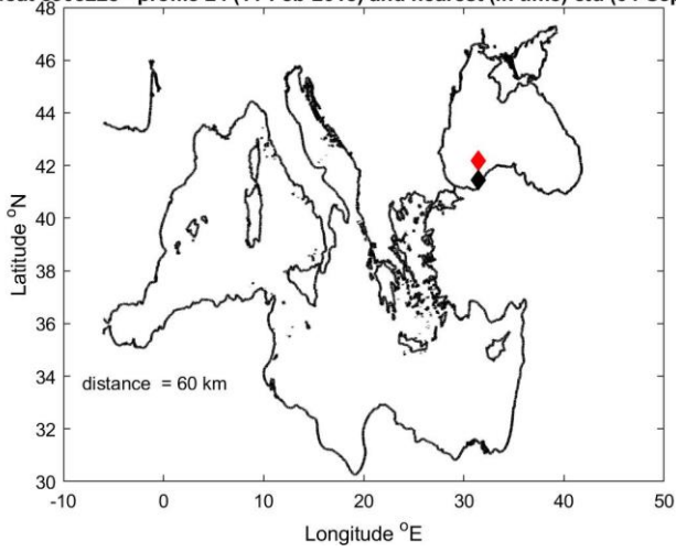
Float 6903228 - profile 24 (11-Feb-2018) and nearest (in time) ctd (04-Sep-2017)
