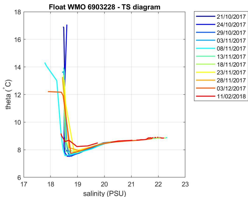
Figure 4: Float 6903228. \theta -S diagram color-coded per cycle number.
