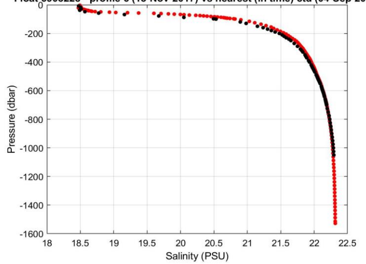
Float 6903228 - profile 6 (13-Nov-2017) vs nearest (in time) ctd (04-Sep-2017)
