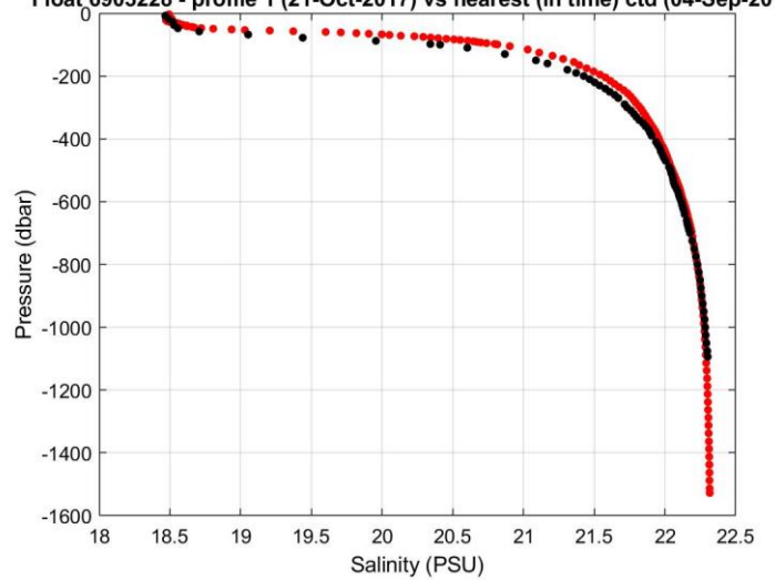
Float 6903228 - profile 1 (21-Oct-2017) vs nearest (in time) ctd (04-Sep-2017)
