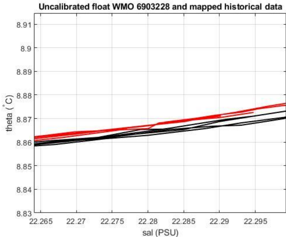
Figure 19: Float 6903228. Uncalibrated float salinity profile (black lines) and mapped historical data (red lines), in the most uniform part of the \theta -S curve.
