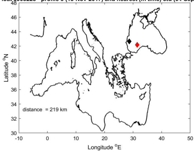
Float 6903228 - profile 6 (13-Nov-2017) and nearest (in time) ctd (04-Sep-2017)
