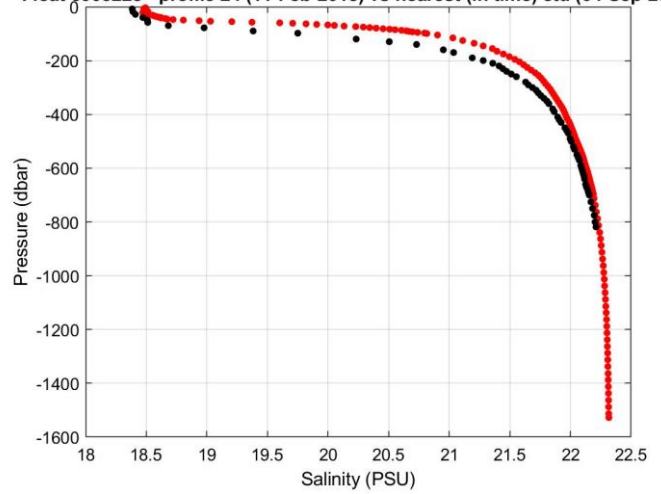
Float 6903228 - profile 24 (11-Feb-2018) vs nearest (in time) ctd (04-Sep-2017)
