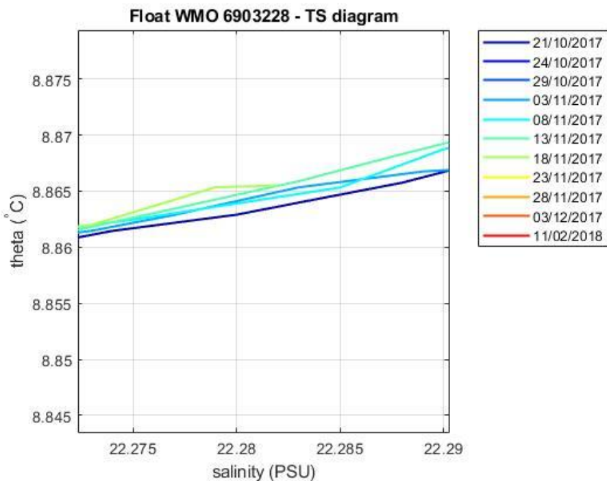
Figure 5: Float 6903228. Area of the \theta -S diagram (color-coded per cycle number) where the \theta -S relationship is more uniform.
