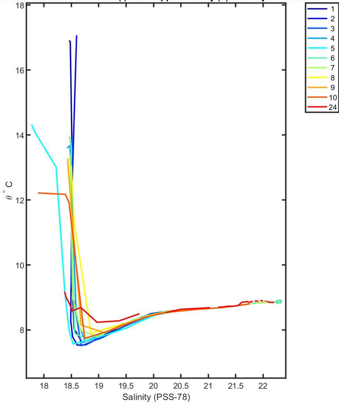
6903228 calibrated float data (-) and mapped salinity (o) with objective errors
