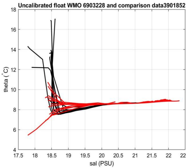
Figure 21: Float 6903228. Comparison between float 6903228 (black line) and float 3901852 (red line), on the left. On the right zoom in the most uniform part of the \theta -S curve.
