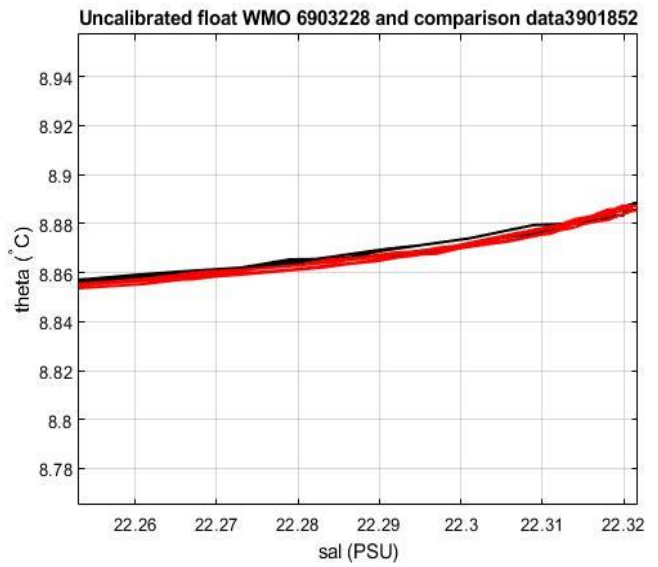
Figure 21: Float 6903228. Comparison between float 6903228 (black line) and float 3901852 (red line), on the left. On the right zoom in the most uniform part of the \theta -S curve.
