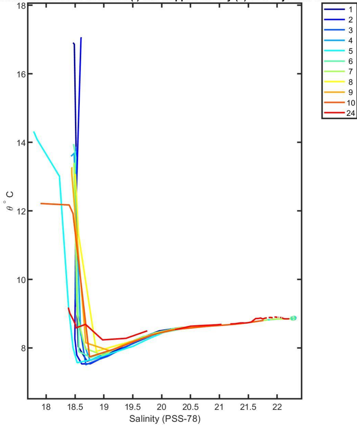
6903228 uncalibrated float data (-) and mapped salinity (o) with objective errors
