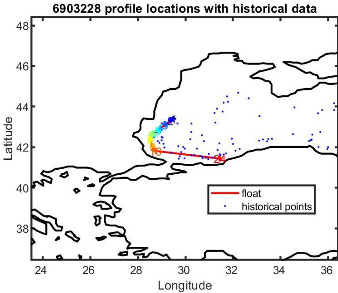
Figure 13: Float 6903228. Location of the float profiles (red line with colored numbers) and the reference data selected for mapping (blue dots).
