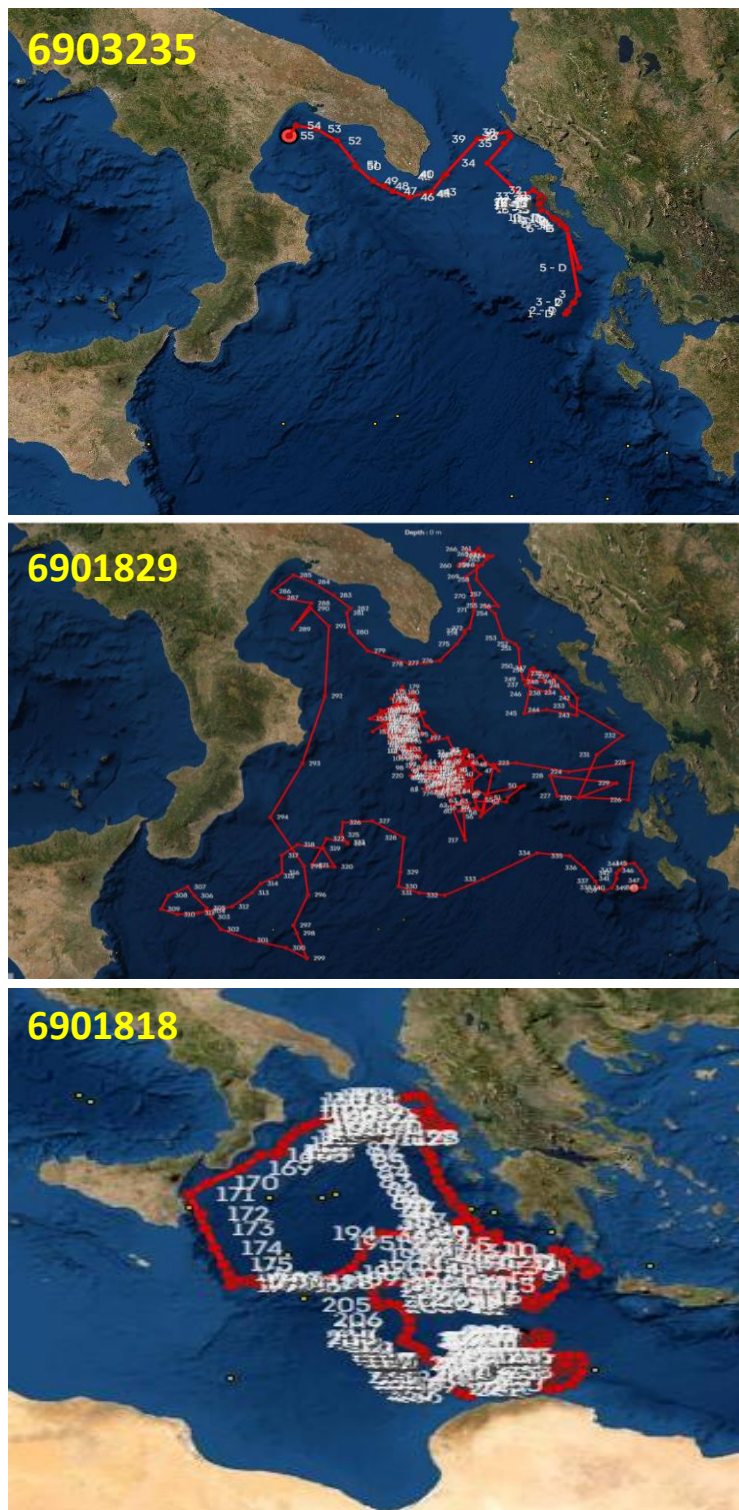
Figure 20: Float 6903235. Trajectory of the floats used for the comparison.
