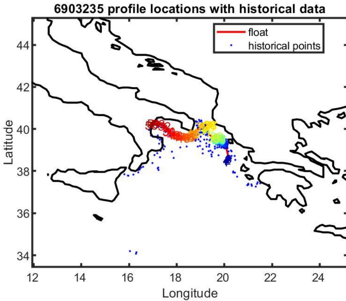
Figure 13: Float 6903235. Location of the float profiles (red line with colored numbers) and the reference data selected for mapping (blue dots).
