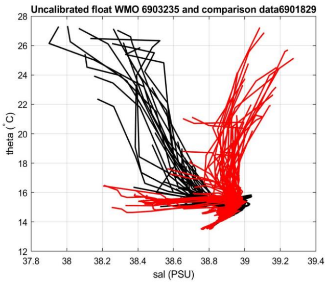
Figure 21: Float 6903235. Comparison between float 6903235 (black line) and float 6901829 (red line), on the left. On the right zoom in the most uniform part of the \theta -S curve
