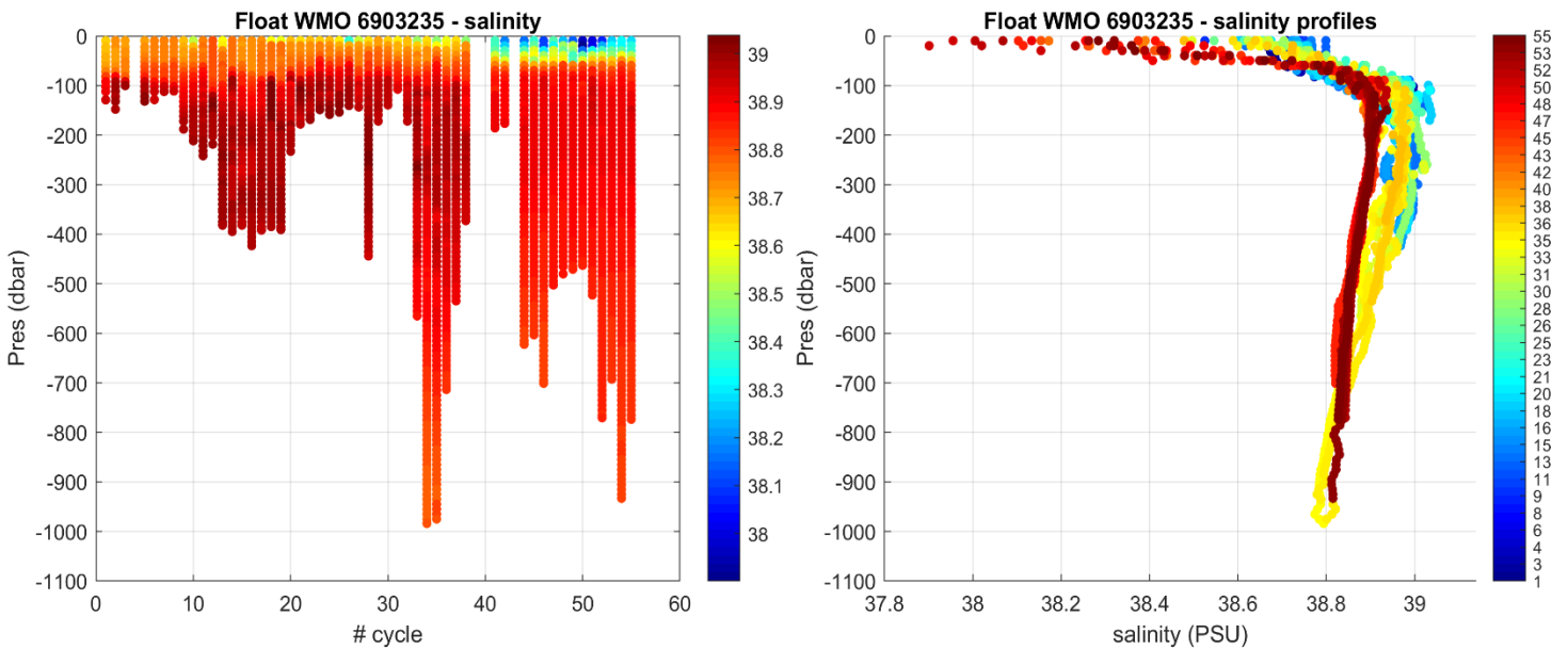
Figure 3: Float 6903235. Time series of Argo float potential salinity (PSS-78) on the left, and salinity profiles color-coded per cycle number on the right.
