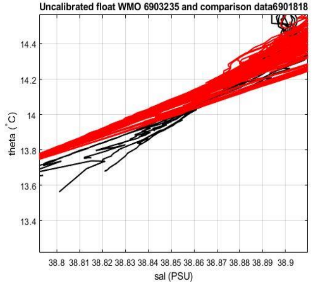
Figure 22: Float 6903235. Comparison between float 6903235 (black line) and float 6901818 (red line), on the left. On the right zoom in the most uniform part of the \theta -S curve
