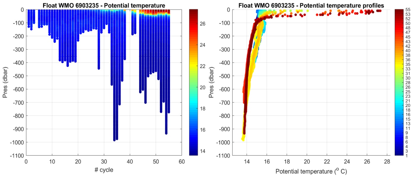
Figure 2: Float 6903235. Time series of Argo float potential temperature ( ^{\circ}\text{C} ) on the left, and potential temperature profiles color-coded per cycle number on the right.
