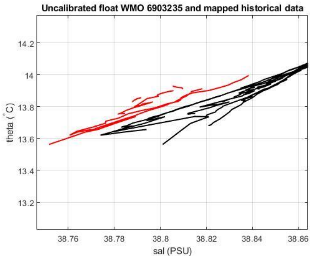
Figure 19: Float 6903235. Uncalibrated float salinity profile (black lines) and mapped historical data (red lines) in the most uniform part of the \theta -S curve.
