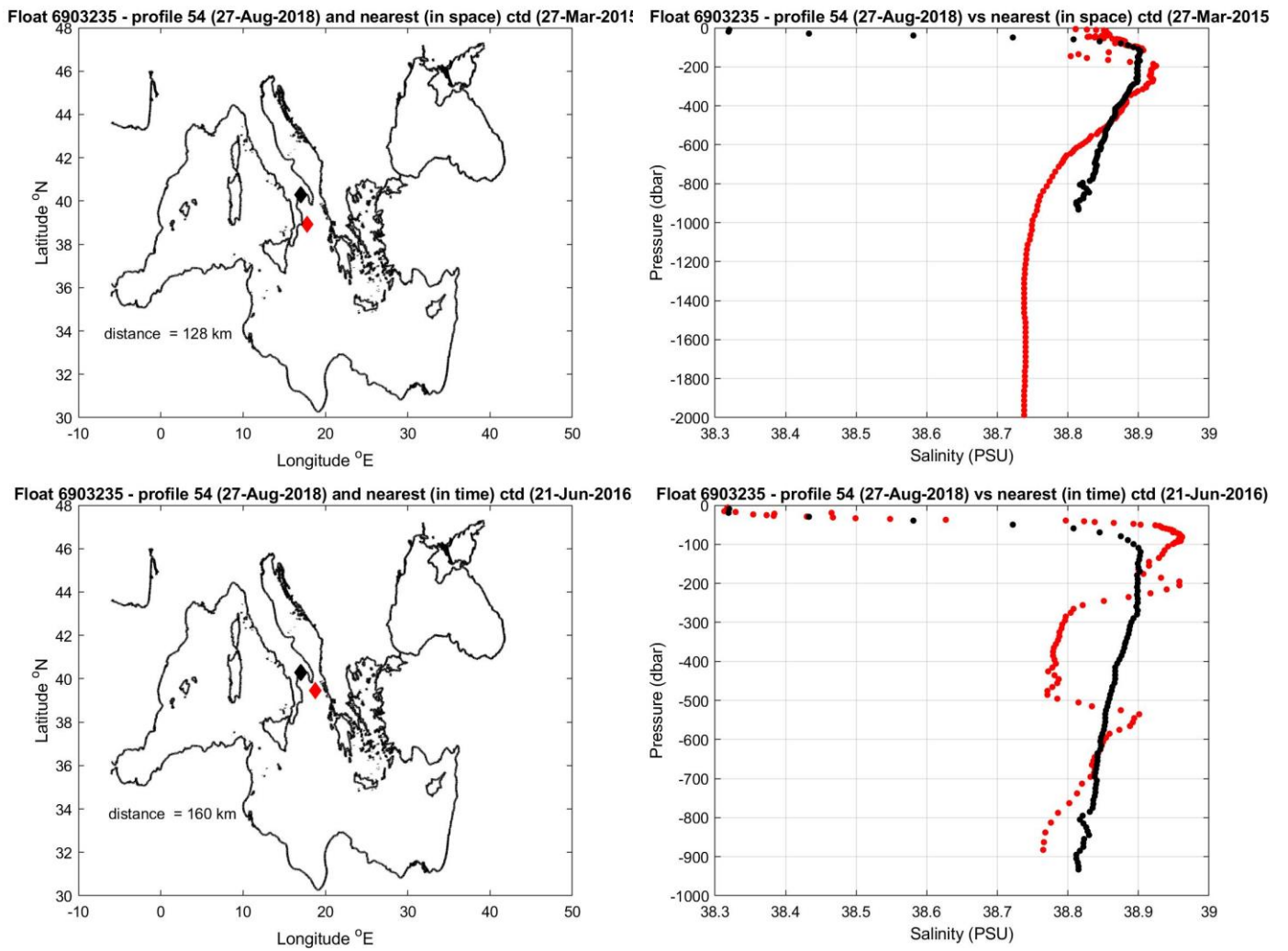
Figure 11: Float 6903235. The salinity float profile number 54 (black dots) are compared to the nearest in space (top) and in time (bottom) reference profile (red dots). The locations of the two profiles and their distance is given in the left panel.
