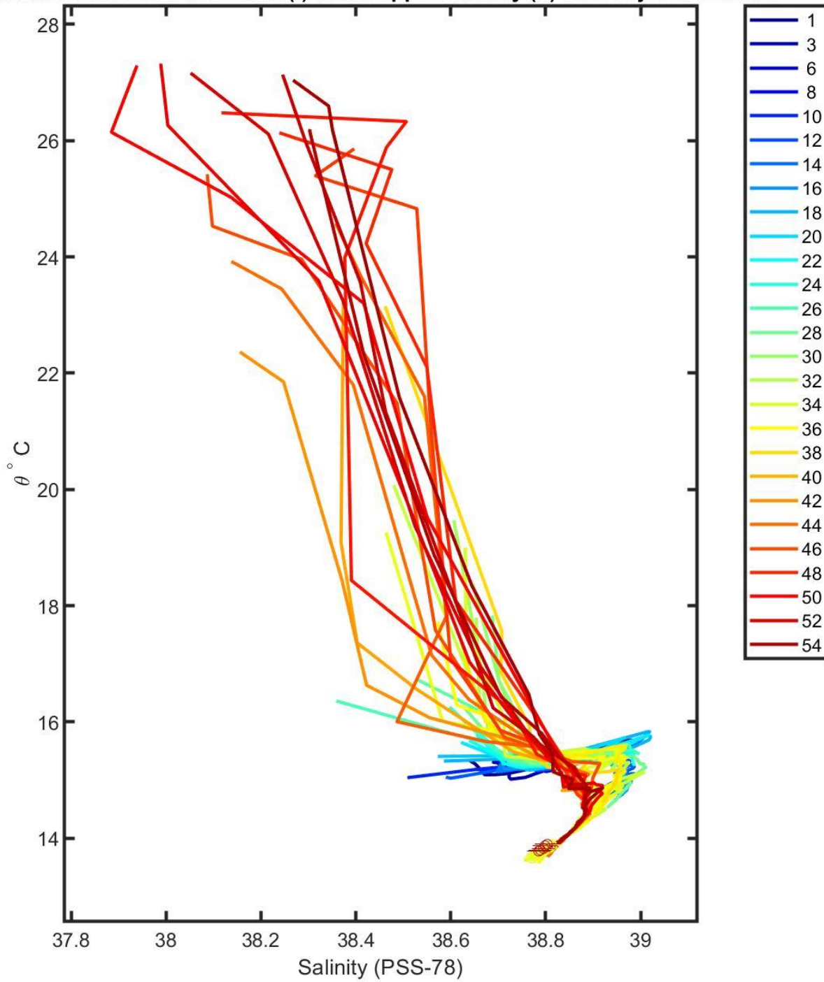
6903235 calibrated float data (-) and mapped salinity (o) with objective errors
