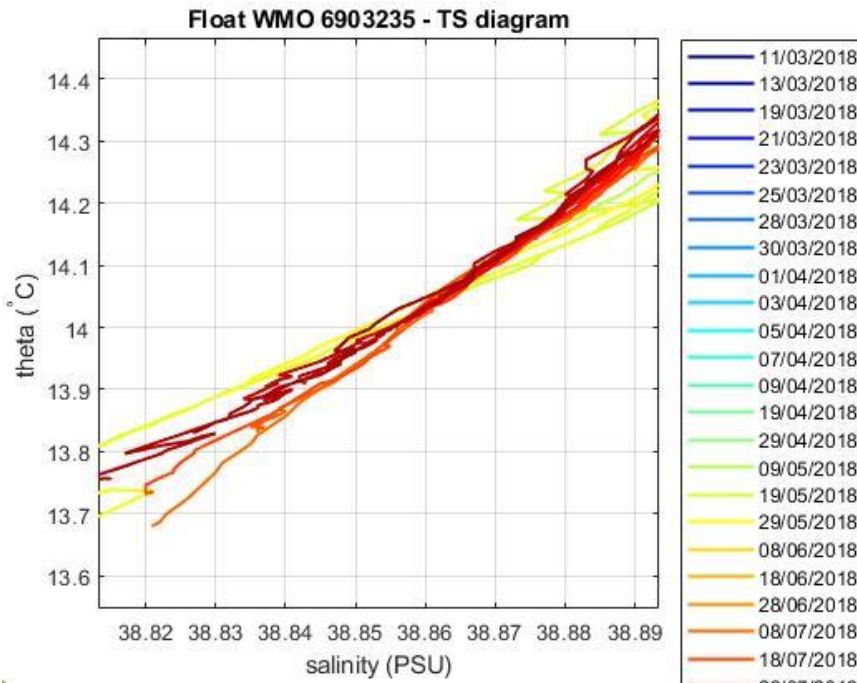
Figure 5: Float 6903235. Area of the \theta -S diagram (color-coded per cycle number) where the \theta -S relationship is more uniform.
