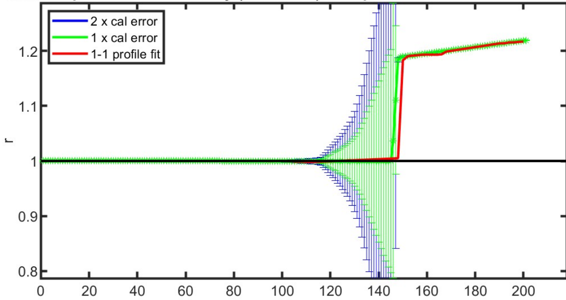
6903238 potential conductivity (mmho/cm) multiplicative correction r with errors
