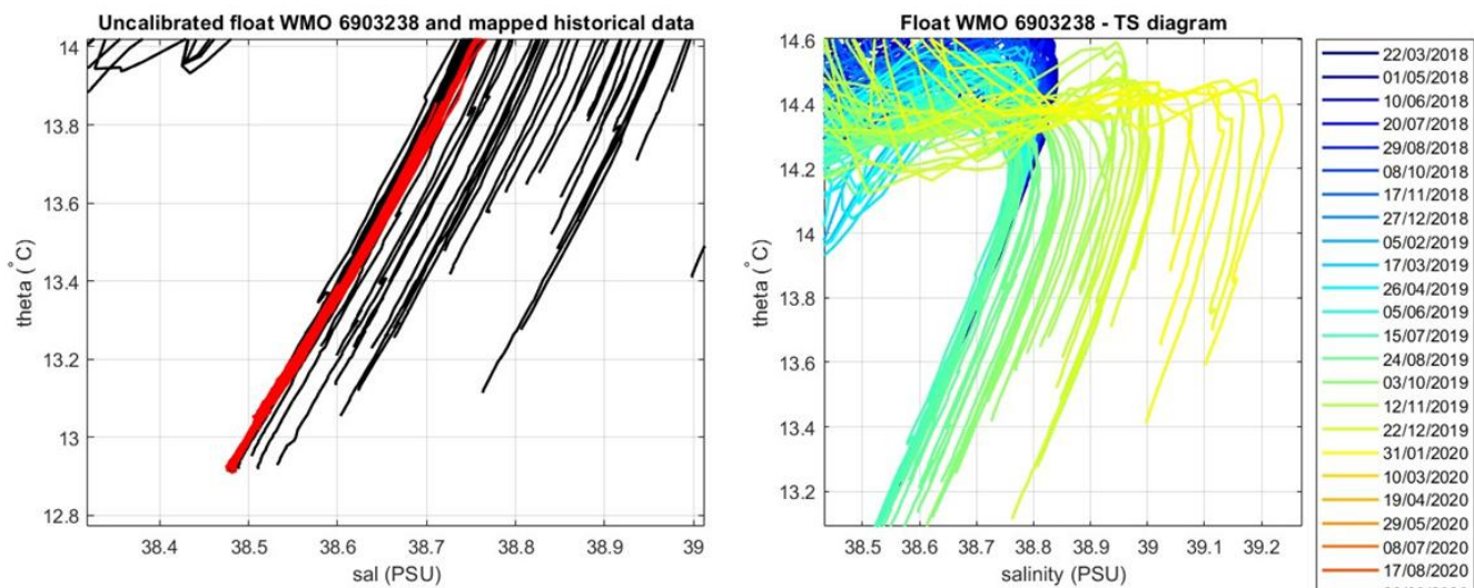
Figure 7: Comparison between float 6903238 and historical CTD on the left and \theta -S diagram color-coded per cycle number on the right, in the most uniform part of the \theta -S curve.
