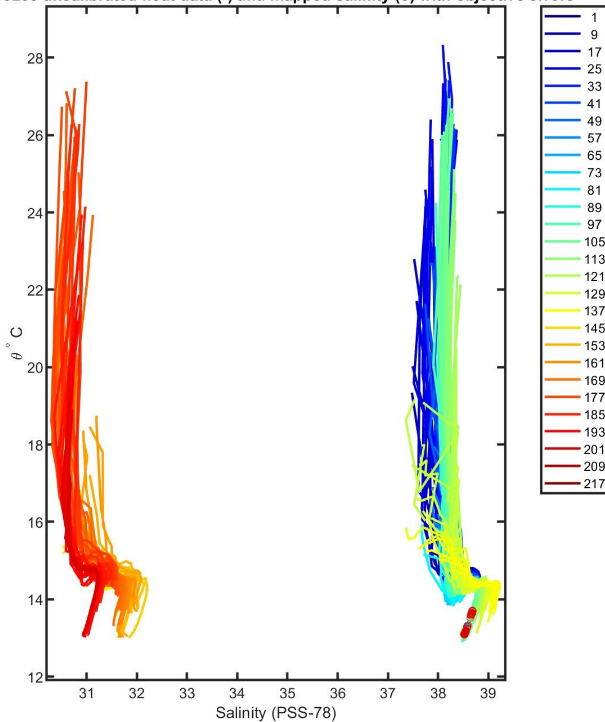
6903238 uncalibrated float data (-) and mapped salinity (o) with objective errors
