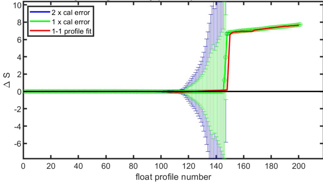
6903238 vertically-averaged salinity (PSS-78) additive correction \Delta S with errors
