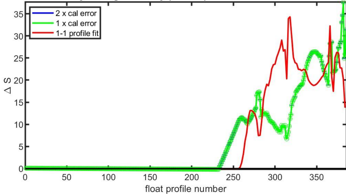
6903239 vertically-averaged salinity (PSS-78) additive correction \Delta S with errors
