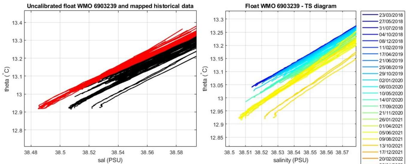
Figure 7: Comparison between float 6903239 – cycles 1-251 - and historical CTD on the left and \theta -S diagram color-coded per cycle number on the right, in the most uniform part of the \theta -S curve.
