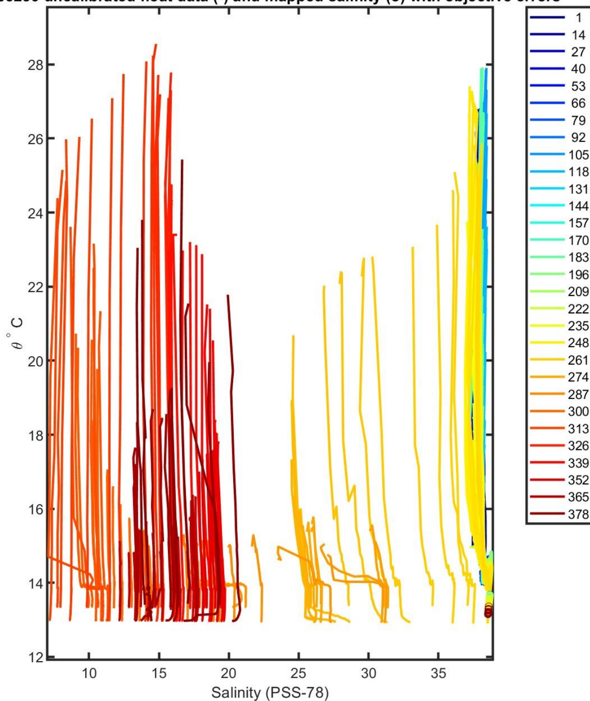
6903239 uncalibrated float data (-) and mapped salinity (o) with objective errors
