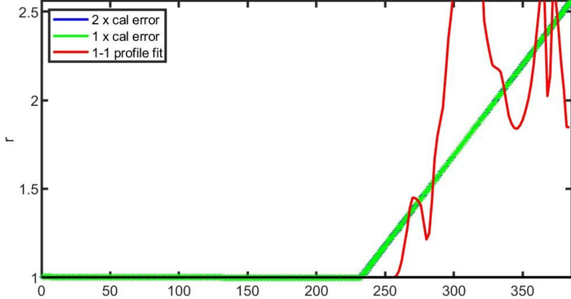
6903239 potential conductivity (mmho/cm) multiplicative correction r with errors
