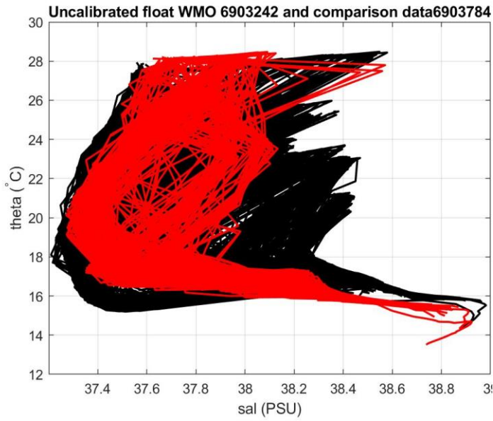
Figure 21: Float 6903242. Comparison between float 6903242 (black line) and float 6903784 (red line), on the left. On the right zoom in the most uniform part of the \theta -S curve
