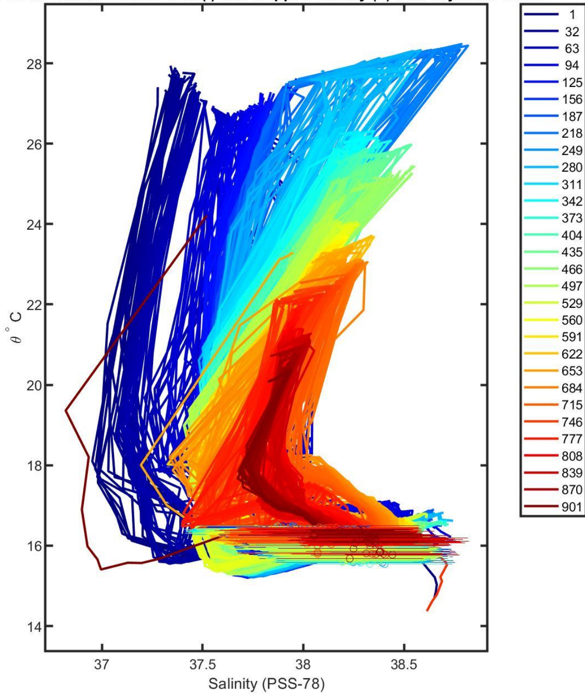
6903242 calibrated float data (-) and mapped salinity (o) with objective errors
