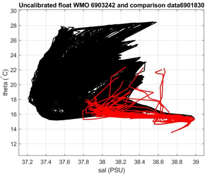
Figure 22: Float 6903242. Comparison between float 6903242 (black line) and float 6901830 (red line), on the left. On the right zoom in the most uniform part of the \theta -S curve
