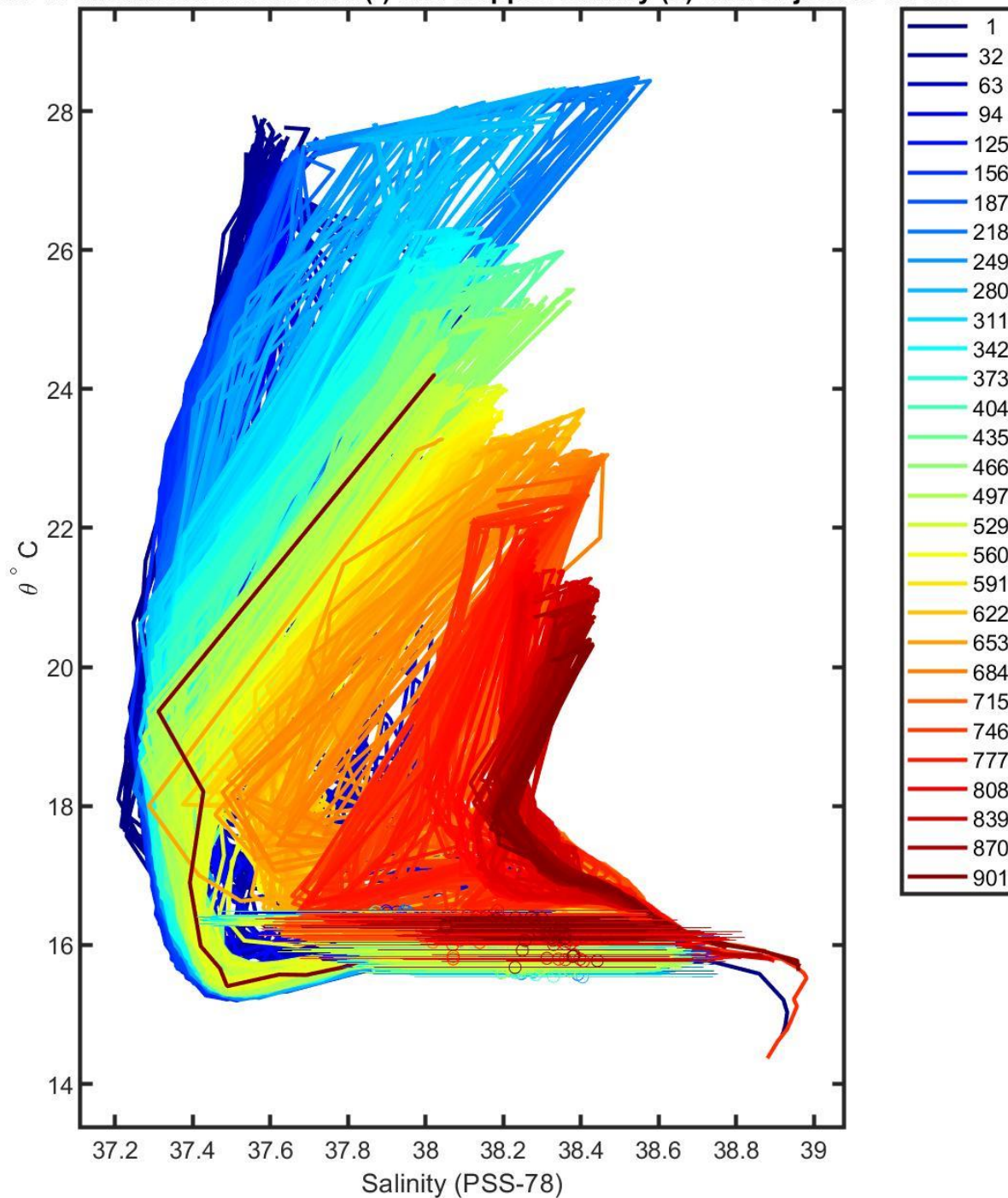
6903242 uncalibrated float data (-) and mapped salinity (o) with objective errors
