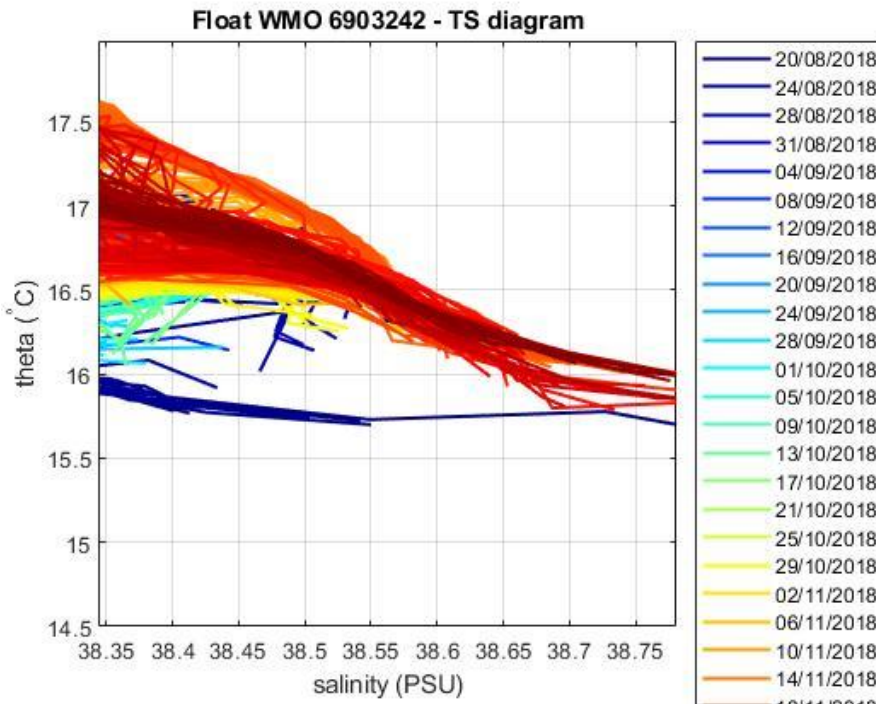
Figure 5: Float 6903242. Area of the \theta -S diagram (color-coded per cycle number) where the \theta -S relationship is more uniform.
