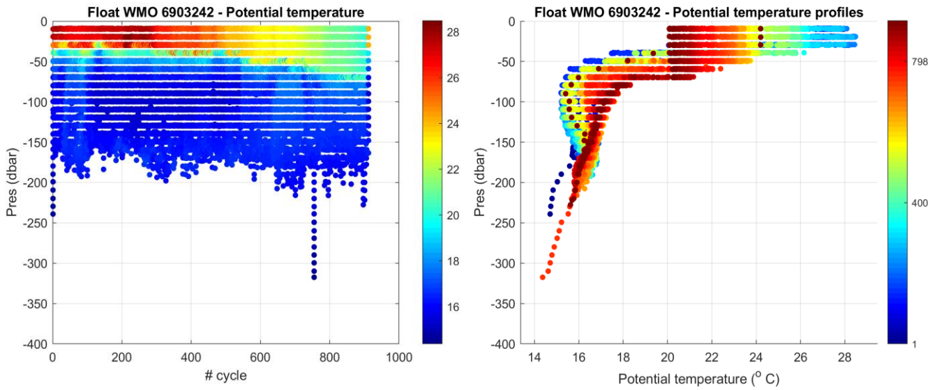
Figure 2: Float 6903242. Time series of Argo float potential temperature ( ^{\circ}\text{C} ) on the left, and potential temperature profiles color-coded per cycle number on the right.
