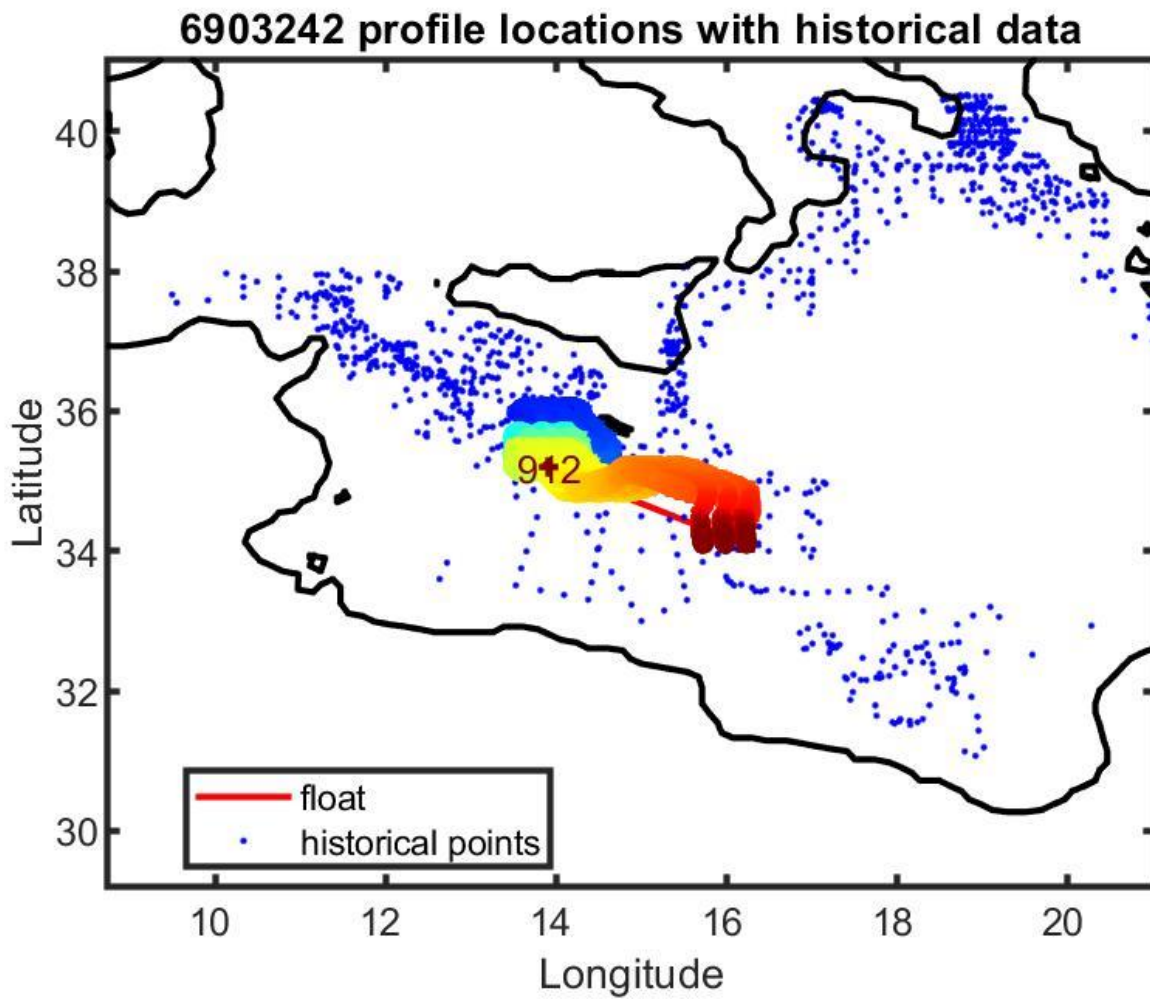
Figure 13: Float 6903242. Location of the float profiles (red line with colored numbers) and the reference data selected for mapping (blue dots).
