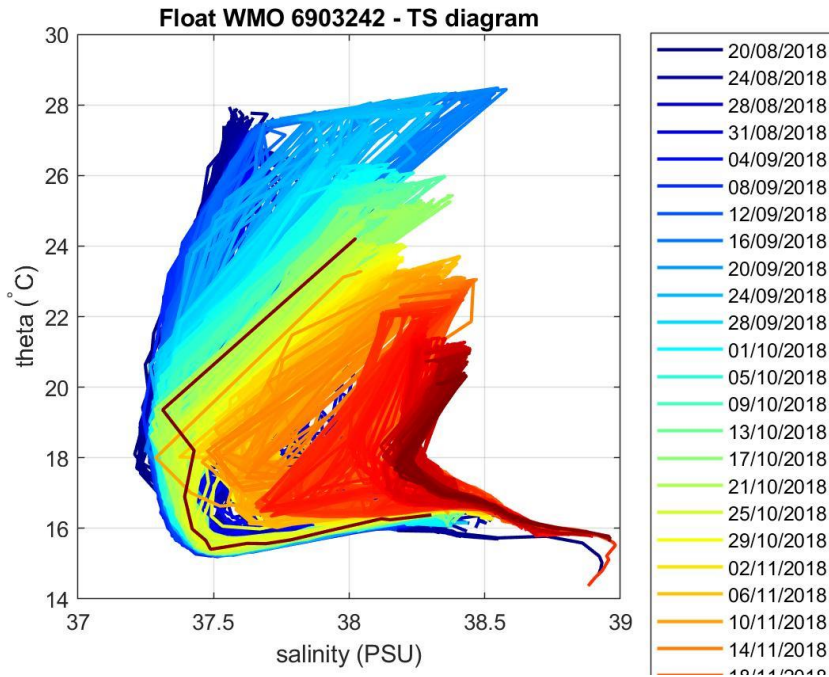
Figure 4: Float 6903242. \theta -S diagram color-coded per cycle number.
