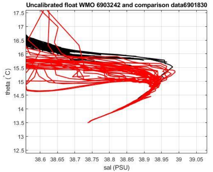
Figure 22: Float 6903242. Comparison between float 6903242 (black line) and float 6901830 (red line), on the left. On the right zoom in the most uniform part of the \theta -S curve
