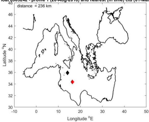
Float 6903242 - profile 1 (20-Aug-2018) and nearest (in time) ctd (01-Mar-2013)
