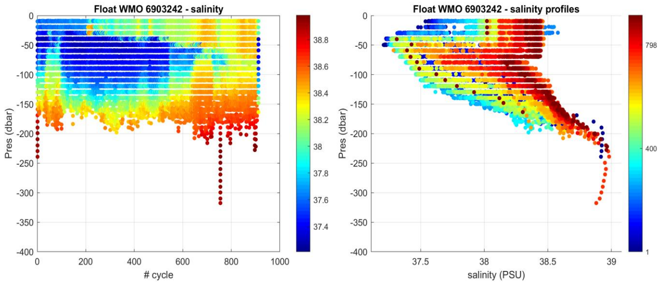
Figure 3: Float 6903242. Time series of Argo float potential salinity (PSS-78) on the left, and salinity profiles color-coded per cycle number on the right.
