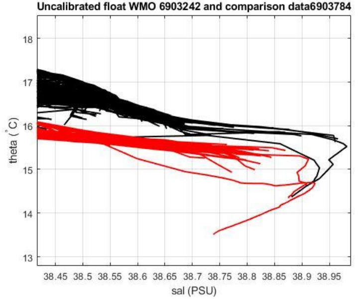
Figure 21: Float 6903242. Comparison between float 6903242 (black line) and float 6903784 (red line), on the left. On the right zoom in the most uniform part of the \theta -S curve
