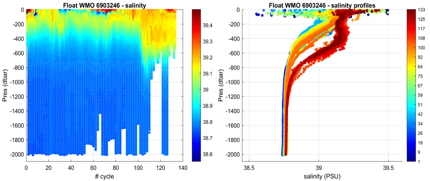
Figure 2: Float 6903246. Time series of Argo float potential salinity (PSS-78) on the left, and salinity profiles color-coded per cycle number on the right.
