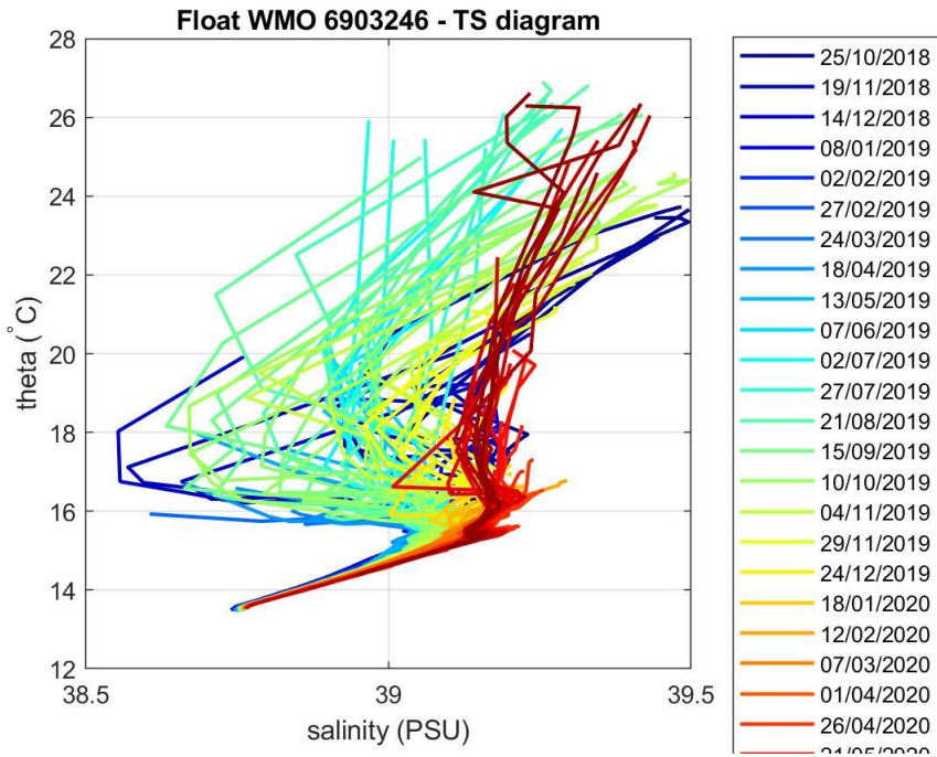
Figure 3: Float 6903246. \theta -S diagram color-coded per cycle number.
