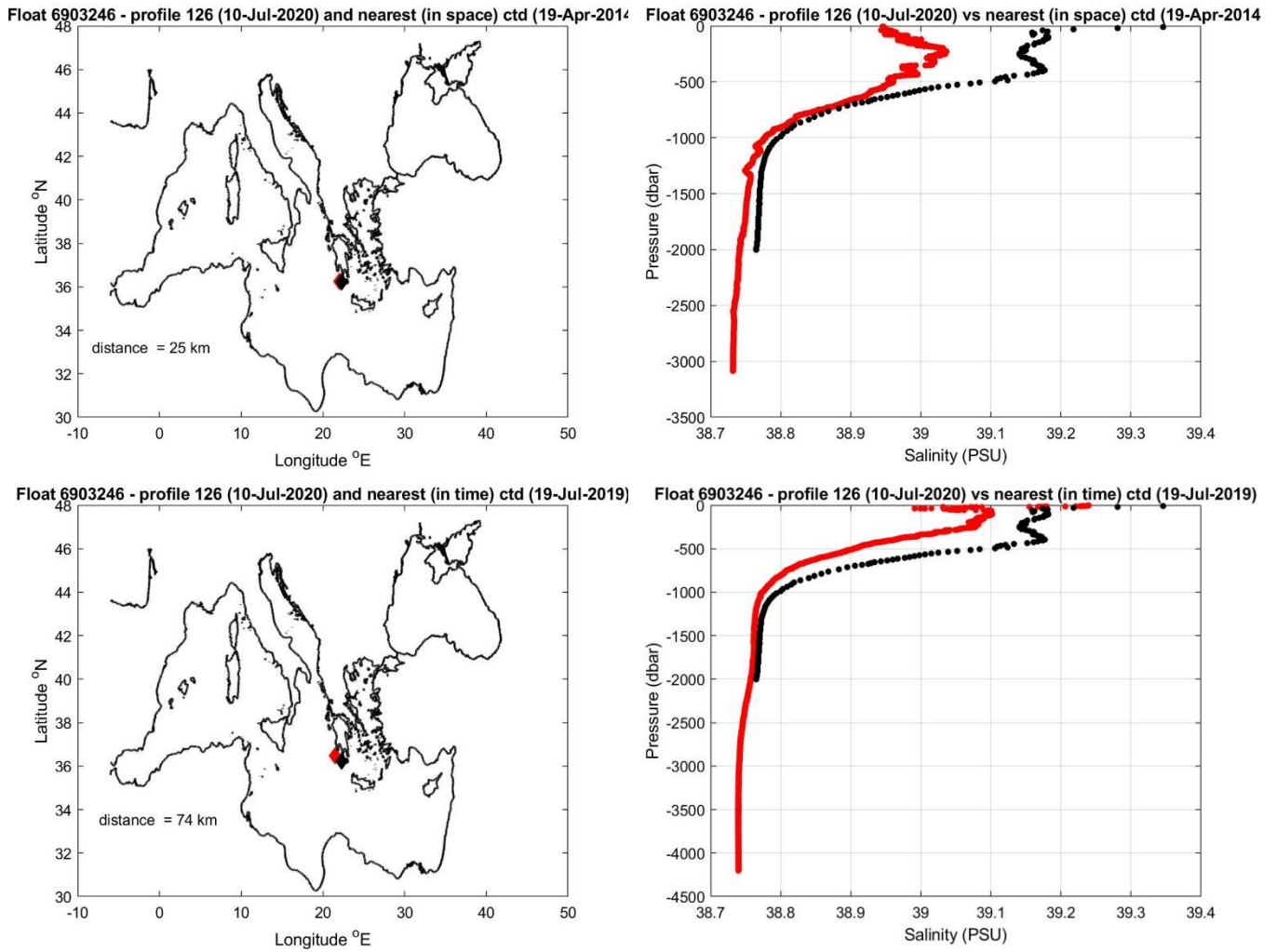
Figure 10: Float 6903246. The salinity float profile number 126 (black dots) are compared to the nearest in space (top) and in time (bottom) reference profile (red dots). The locations of the two profiles and their distance is given in the left panel.
