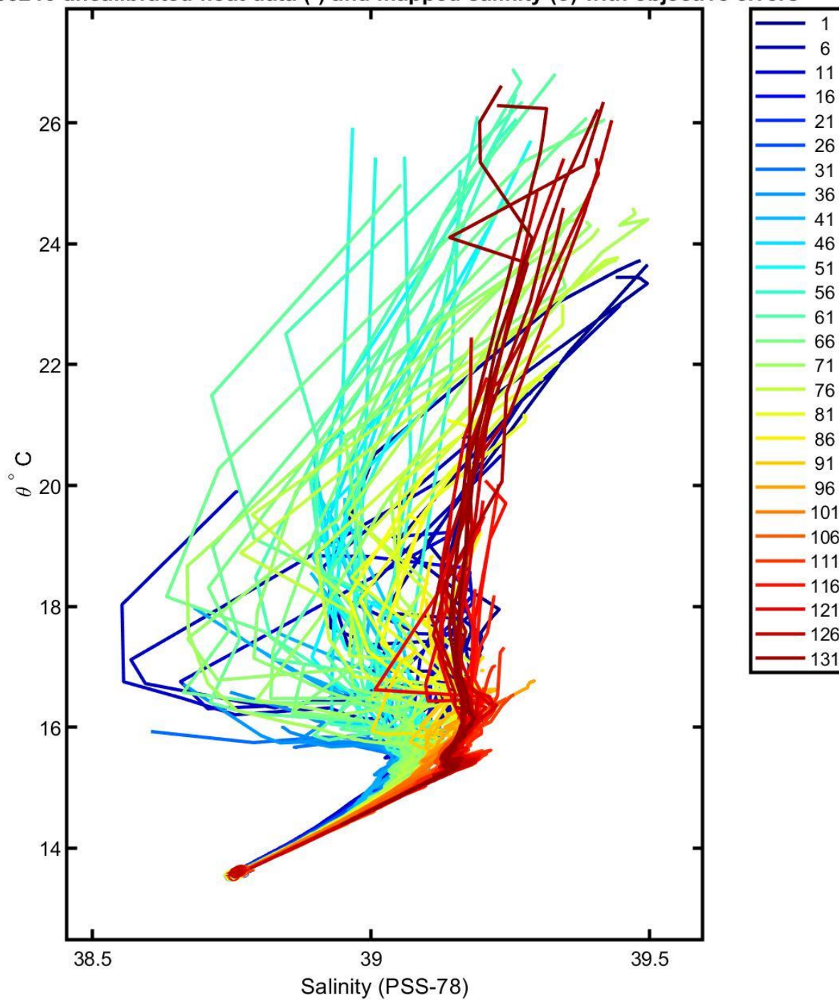
6903246 uncalibrated float data (-) and mapped salinity (o) with objective errors
