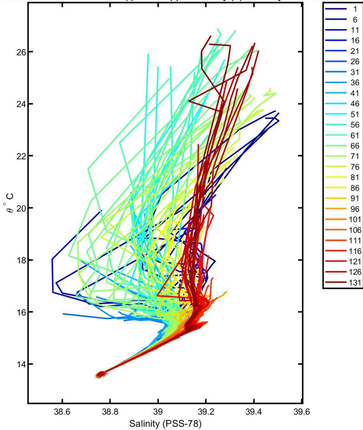
6903246 calibrated float data (-) and mapped salinity (o) with objective errors
