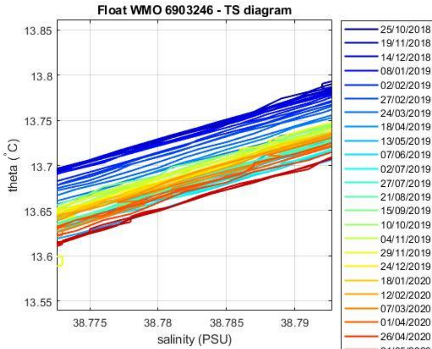
Figure 4: Float 6903246. Area of the \theta -S diagram (color-coded per cycle number) where the \theta -S relationship is more uniform.
