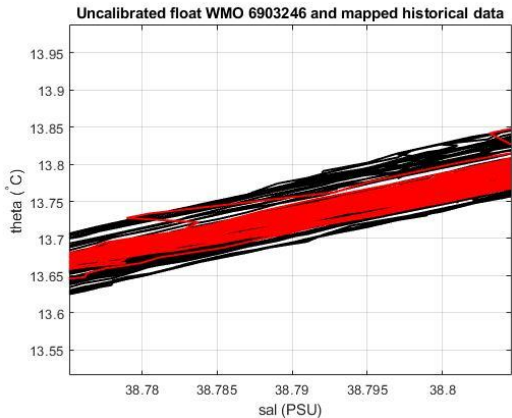
Figure 18: Float 6903246. Uncalibrated float salinity profile (black lines) and mapped historical data (red lines) in the most uniform part of the \theta -S curve.
