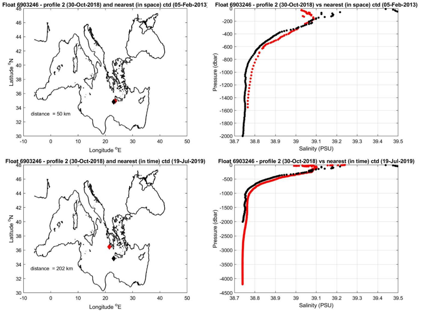
Figure 8: Float 6903246. The salinity float profile number 2 (black dots) are compared to the nearest in space (top) and in time (bottom) reference profile (red dots). The locations of the two profiles and their distance is given in the left panel.
