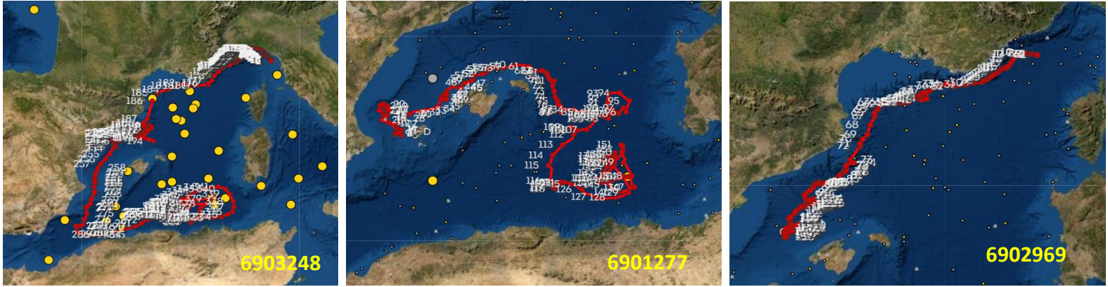
Figure 19: Float 6903248. Trajectory of the floats used for the comparison.
