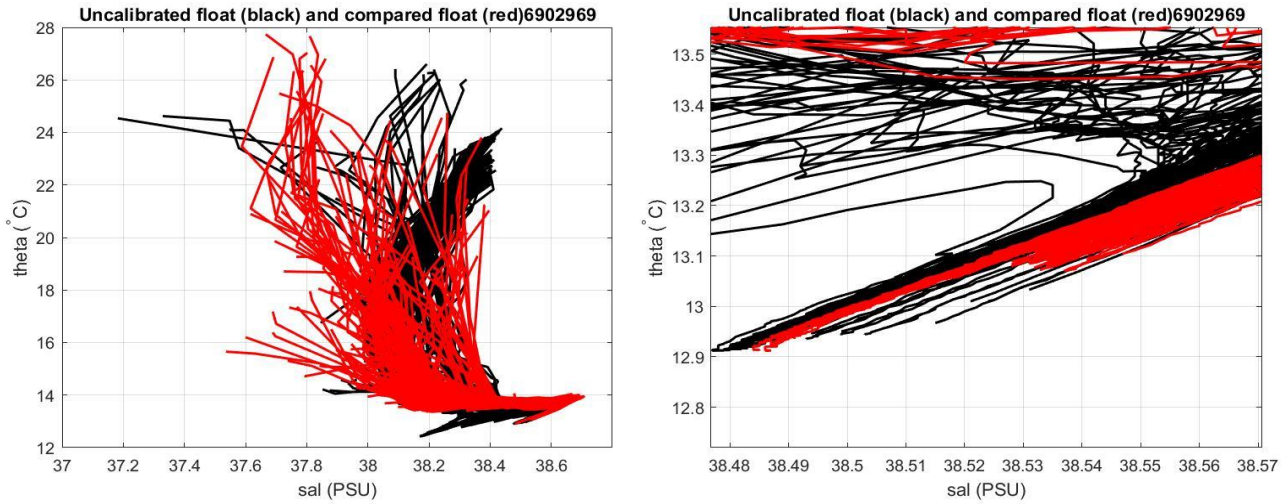
Figure 20: Float 6903248. Comparison between float 6903248 (black line) and 6902969 (red line), in the most uniform part of the \theta -S curve, for cycles in the Liguro Provençal and Catalan sub basins.
