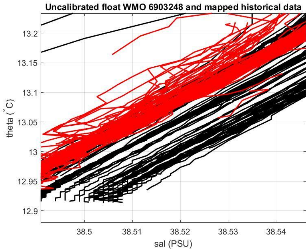
Figure 18: Float 6903248. Uncalibrated float salinity profile (black lines) and mapped historical data (red lines) in the most uniform part of the \theta -S curve.
