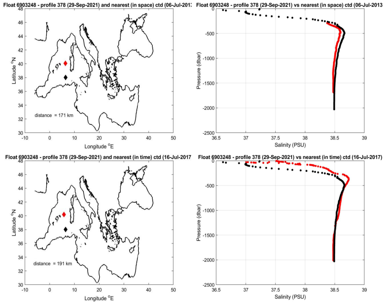
Figure 10: Float 6903248. The salinity float profile number 378 (black dots) are compared to the nearest in space (top) and in time (bottom) reference profile (red dots). The locations of the two profiles and their distance is given in the left panel.
