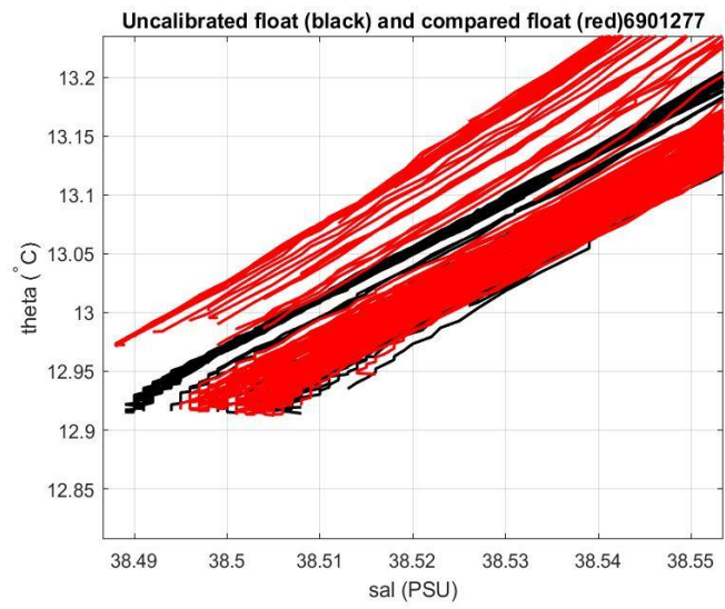
Figure 20: Float 6903248. Comparison between float 6903248 (black line) and 6901277 (red line), in the most uniform part of the \theta -S curve, for cycles in the Algerian sub basin.
