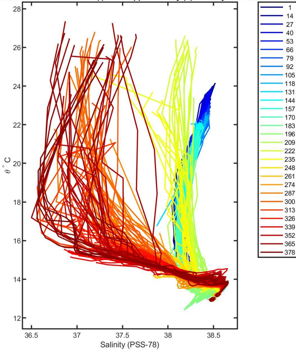
6903248 calibrated float data (-) and mapped salinity (o) with objective errors
