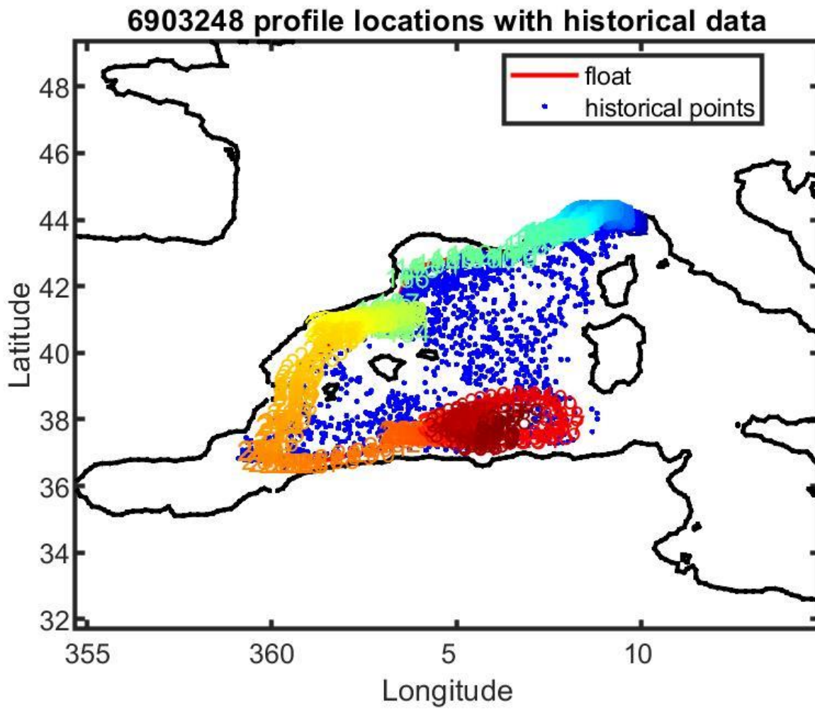
Figure 12: Float 6903248. Location of the float profiles (red line with colored numbers) and the reference data selected for mapping (blue dots).
