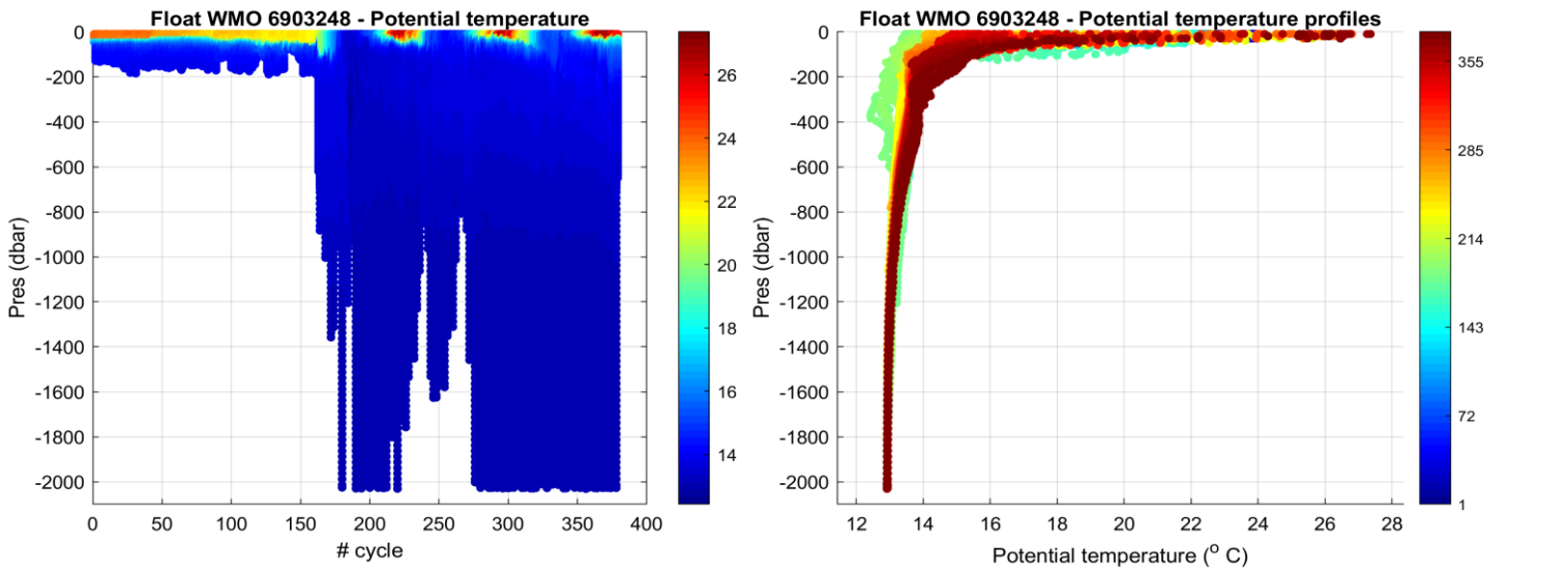
Figure 1: Float 6903248. Time series of Argo float potential temperature ( ^{\circ}\text{C} ) on the left, and potential temperature profiles color-coded per cycle number on the right.
