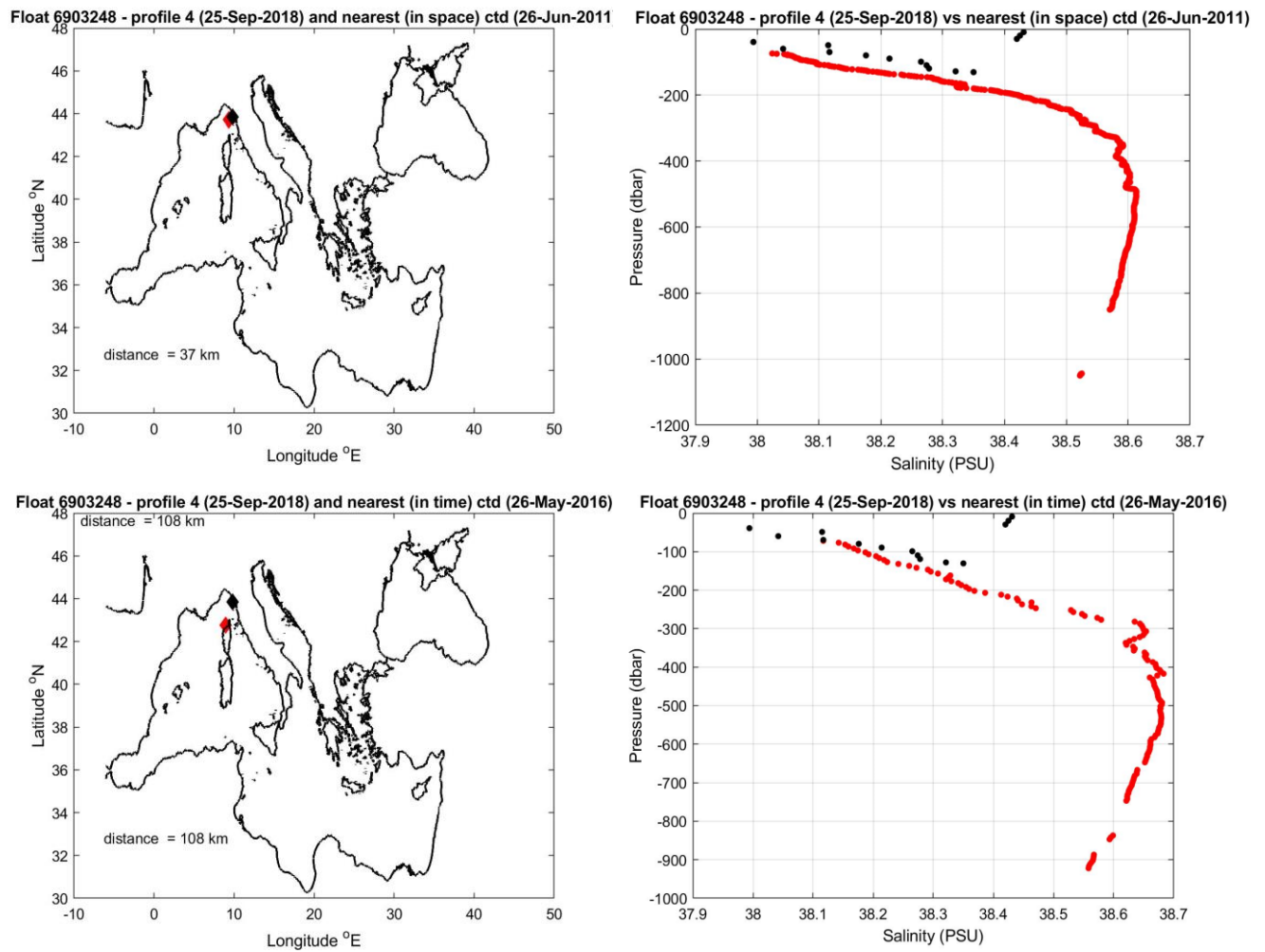
Figure 8: Float 6903248. The salinity float profile number 4 (black dots) are compared to the nearest in space (top) and in time (bottom) reference profile (red dots). The locations of the two profiles and their distance is given in the left panel.
