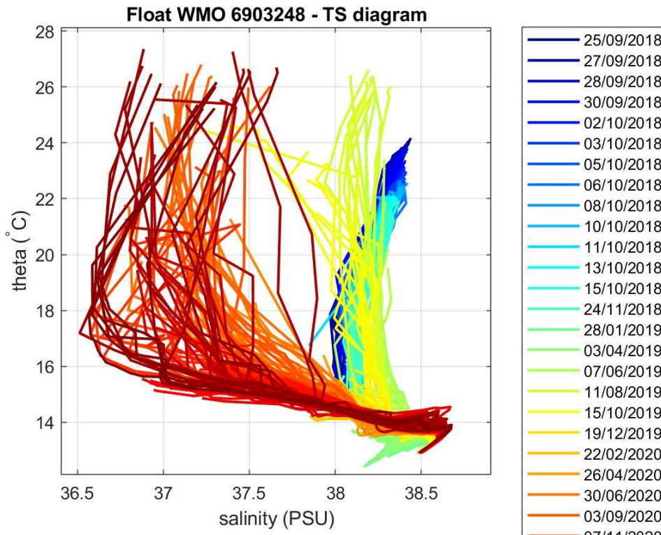
Figure 3: Float 6903248. \theta -S diagram color-coded per cycle number.
