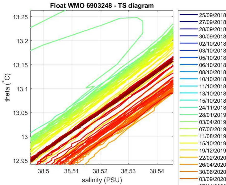
Figure 4: Float 6903248. Area of the \theta -S diagram (color-coded per cycle number) where the \theta -S relationship is more uniform.
