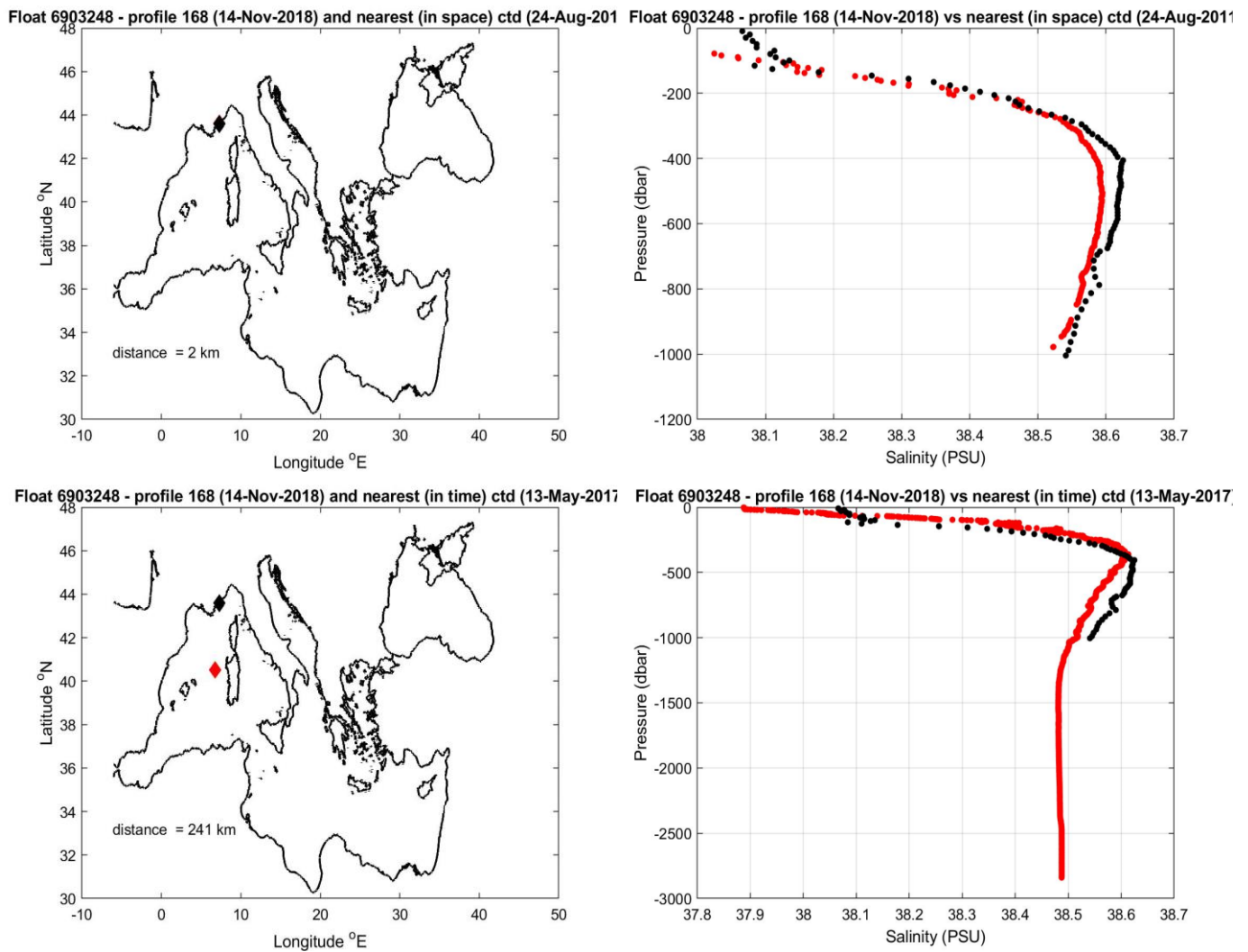
Figure 9: Float 6903248. The salinity float profile number 168 (black dots) are compared to the nearest in space (top) and in time (bottom) reference profile (red dots). The locations of the two profiles and their distance is given in the left panel.
