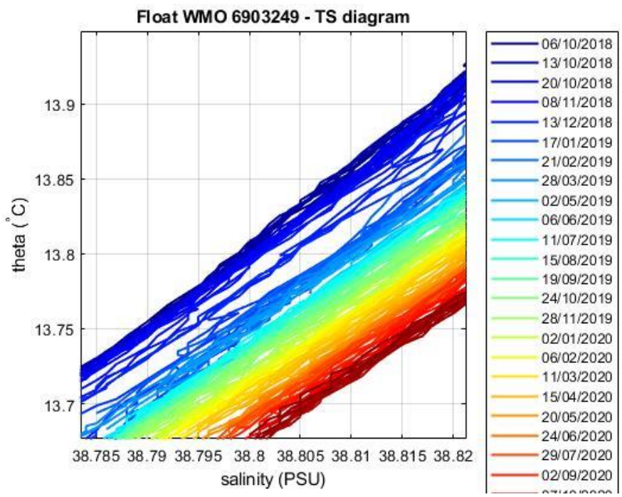
Figure 5: Float 6903249. Area of the \theta -S diagram (color-coded per cycle number) where the \theta -S relationship is more uniform.
