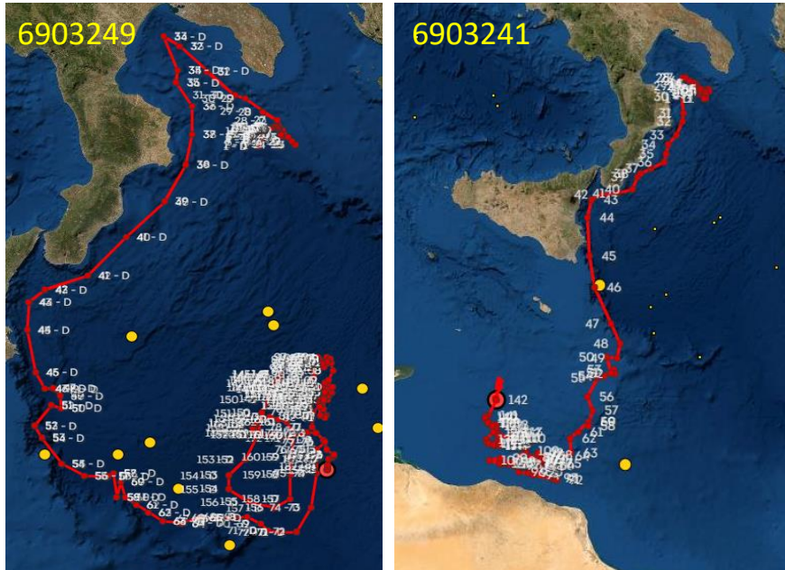
Figure 20: Float 6903249. Trajectory of the floats used for the comparison.
