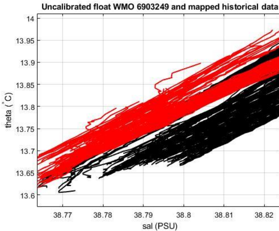
Figure 19: Float 6903249. Uncalibrated float salinity profile (black lines) and mapped historical data (red lines) in the most uniform part of the \theta -S curve.
