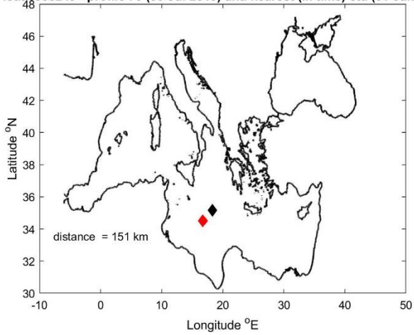
Float 6903249 - profile 70 (06-Jul-2019) and nearest (in time) ctd (01-Jan-2016)
