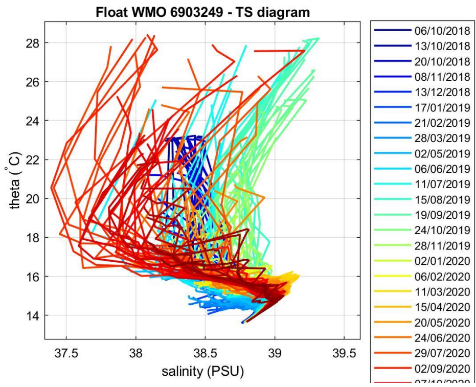
Figure 4: Float 6903249. \theta -S diagram color-coded per cycle number.
