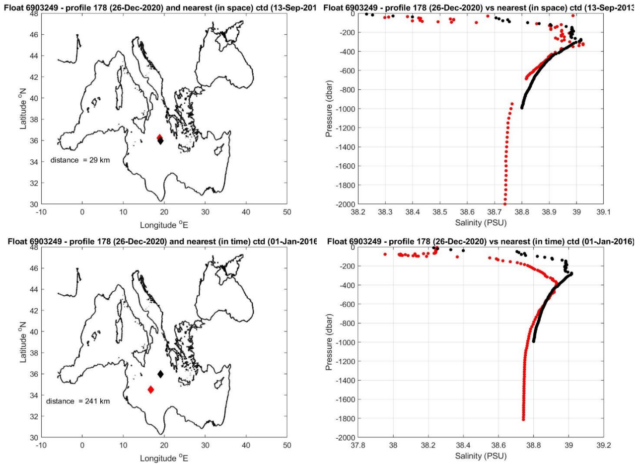
Figure 11: Float 6903249. The salinity float profile number 178 (black dots) are compared to the nearest in space (top) and in time (bottom) reference profile (red dots). The locations of the two profiles and their distance is given in the left panel.
