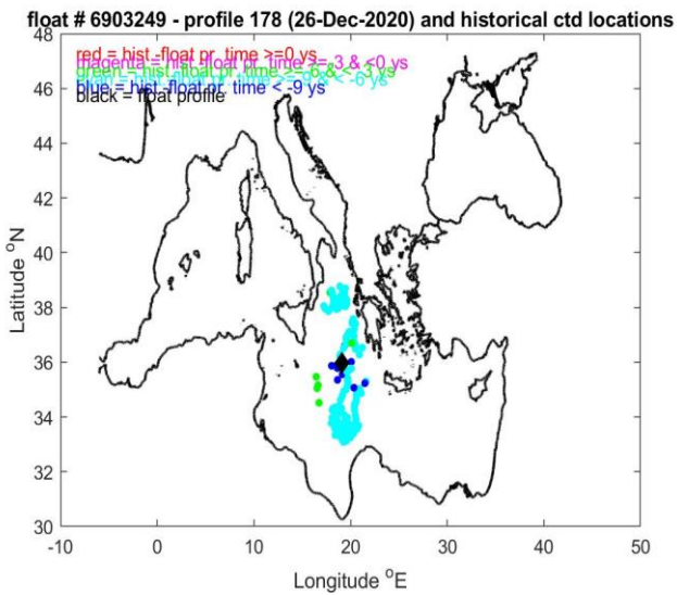
Figure 8: Float 6903249. Locations of the salinity float profile number 178 and historical CTD data (right panel) and the respective salinity profiles (left panel).
