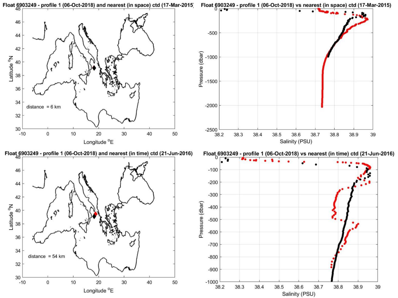
Figure 9: Float 6903249. The salinity float profile number 1 (black dots) are compared to the nearest in space (top) and in time (bottom) reference profile (red dots). The locations of the two profiles and their distance is given in the left panel.
