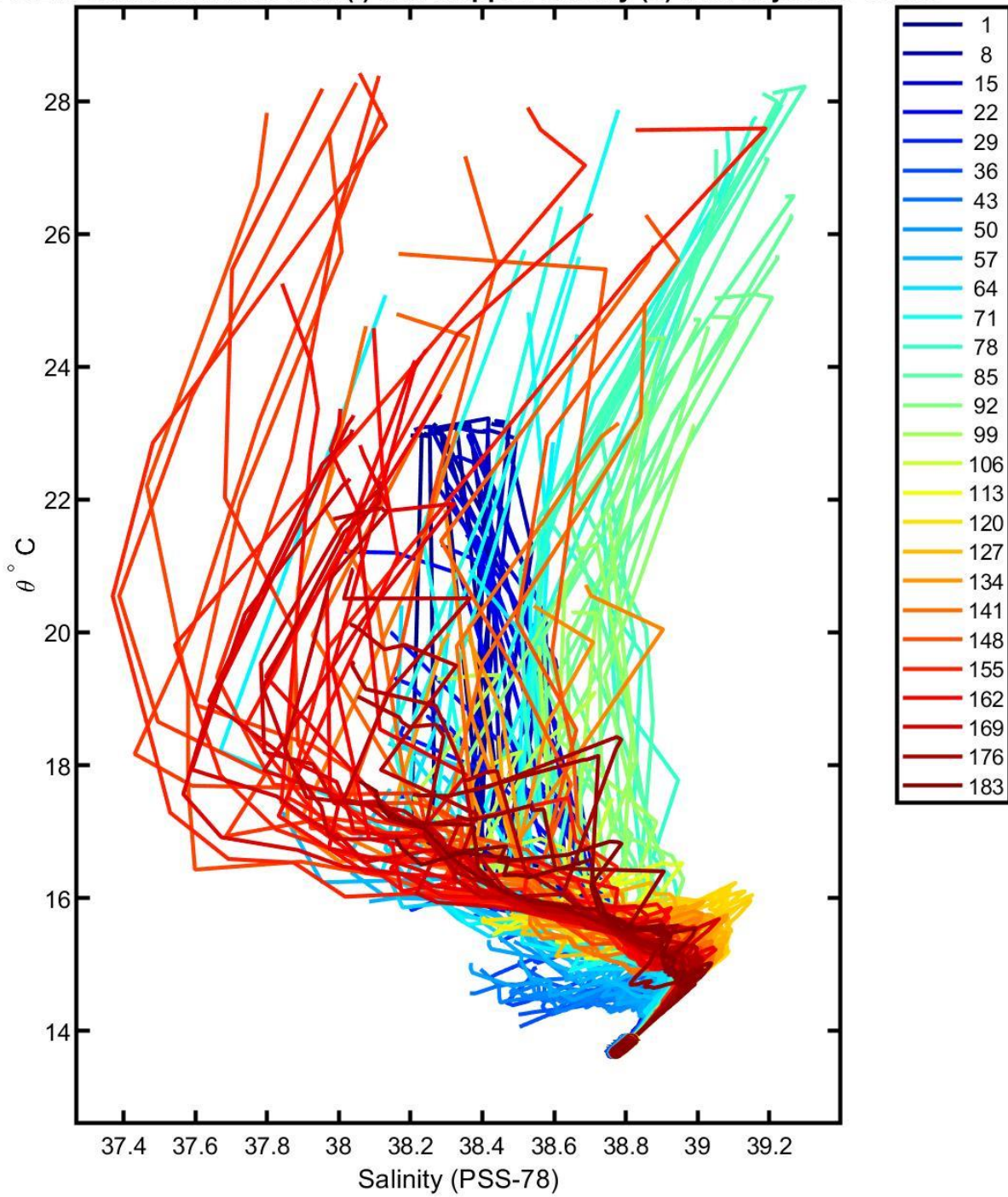
6903249 calibrated float data (-) and mapped salinity (o) with objective errors
