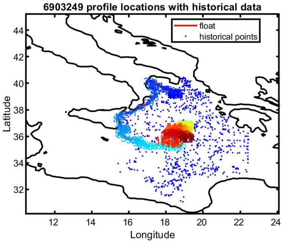
Figure 13: Float 6903249. Location of the float profiles (red line with colored numbers) and the reference data selected for mapping (blue dots).
