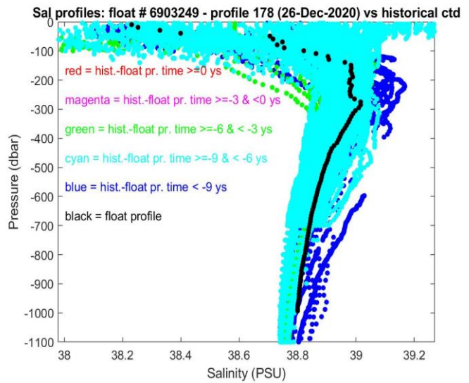
Figure 8: Float 6903249. Locations of the salinity float profile number 178 and historical CTD data (right panel) and the respective salinity profiles (left panel).
