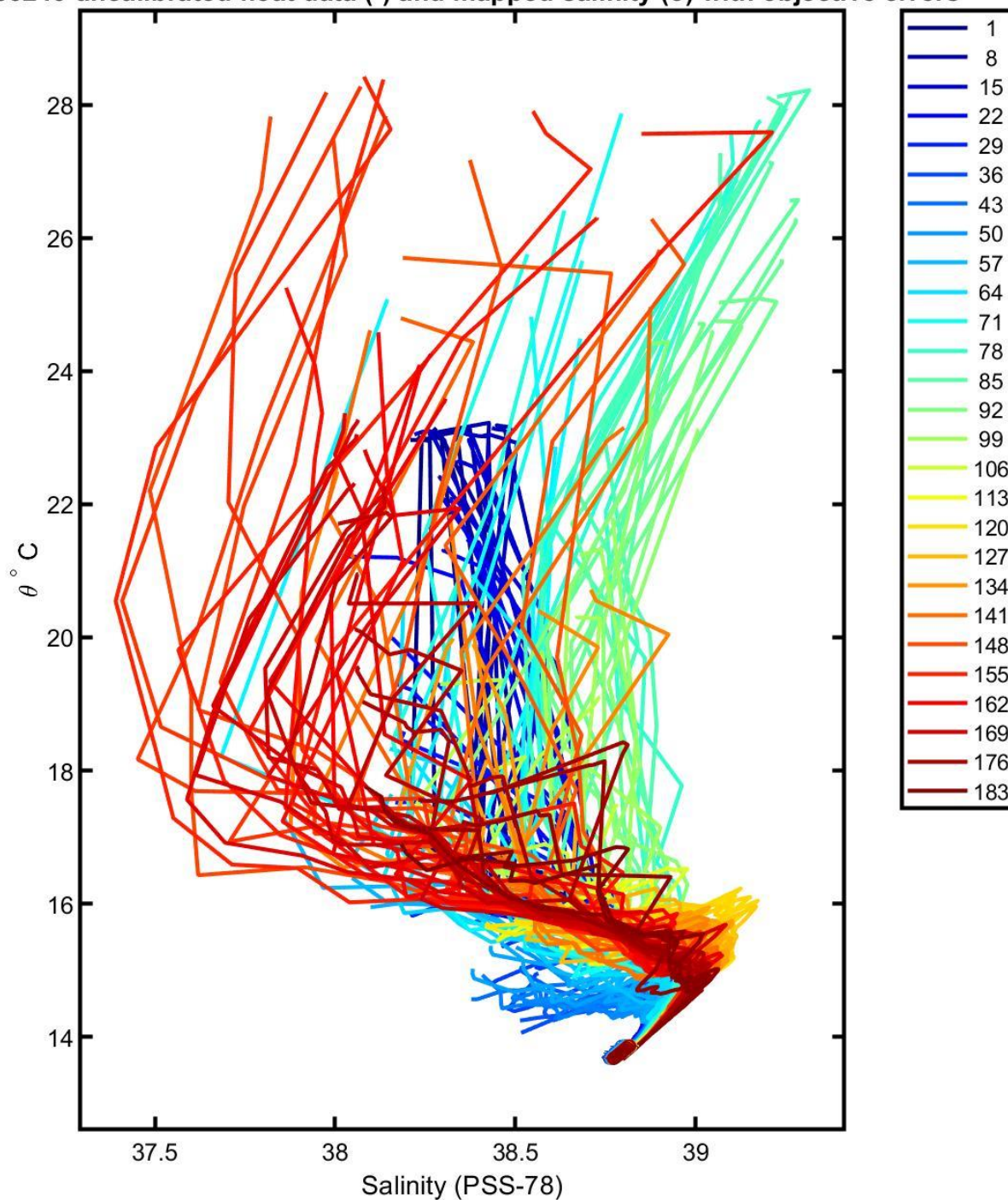
6903249 uncalibrated float data (-) and mapped salinity (o) with objective errors
