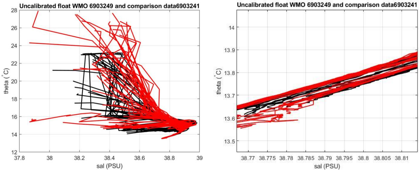
Figure 21: Float 6903249. Comparison between float 6903249 (black line) and float 6903241 (red line), on the left. On the right zoom in the most uniform part of the \theta -S curve.
