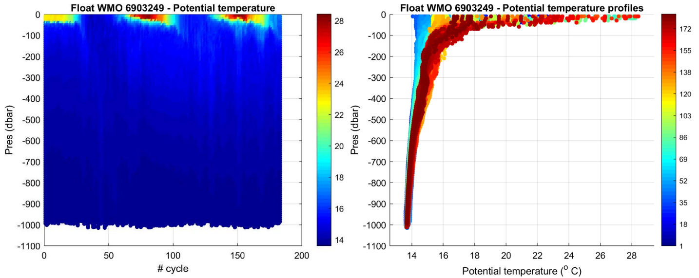
Figure 2: Float 6903249. Time series of Argo float potential temperature ( ^{\circ}\text{C} ) on the left, and potential temperature profiles color-coded per cycle number on the right.
