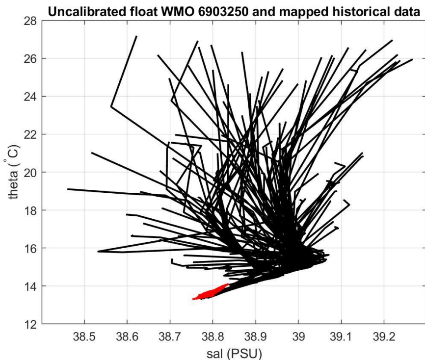
Figure 19: Float 6903250. Uncalibrated float salinity profile (black lines) and mapped historical data (red lines).
