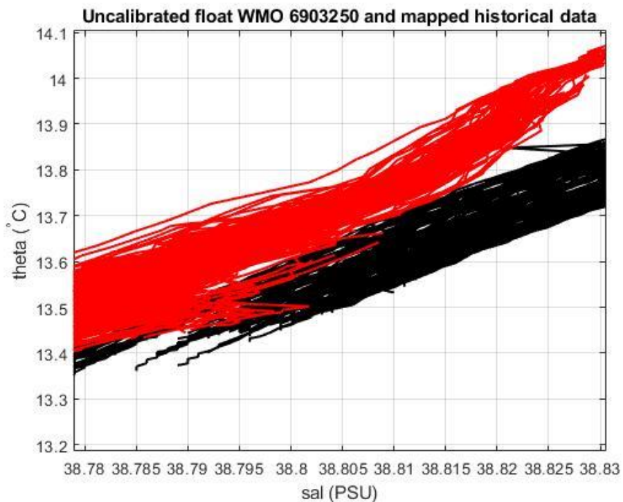
Figure 19: Float 6903250. Uncalibrated float salinity profile (black lines) and mapped historical data (red lines) in the most uniform part of the \theta -S curve.
