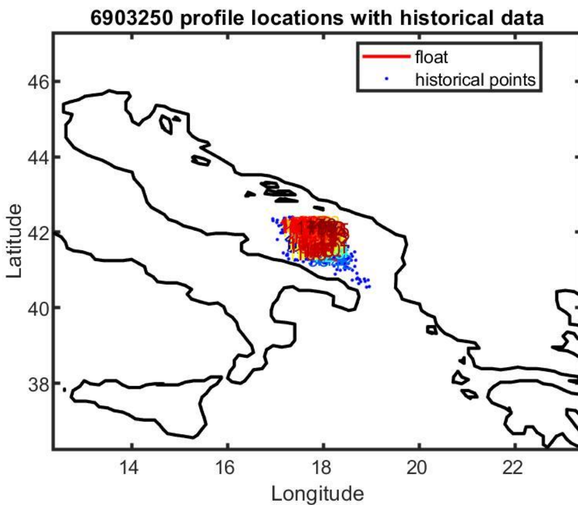
Figure 13: Float 6903250. Location of the float profiles (red line with colored numbers) and the reference data selected for mapping (blue dots).
