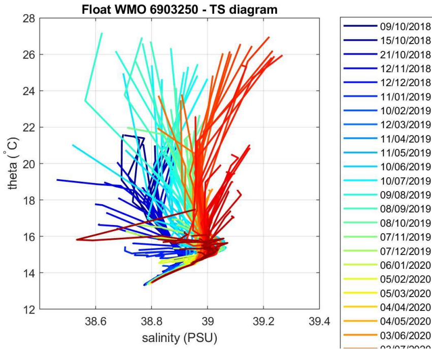
Figure 4: Float 6903250. \theta -S diagram color-coded per cycle number.
