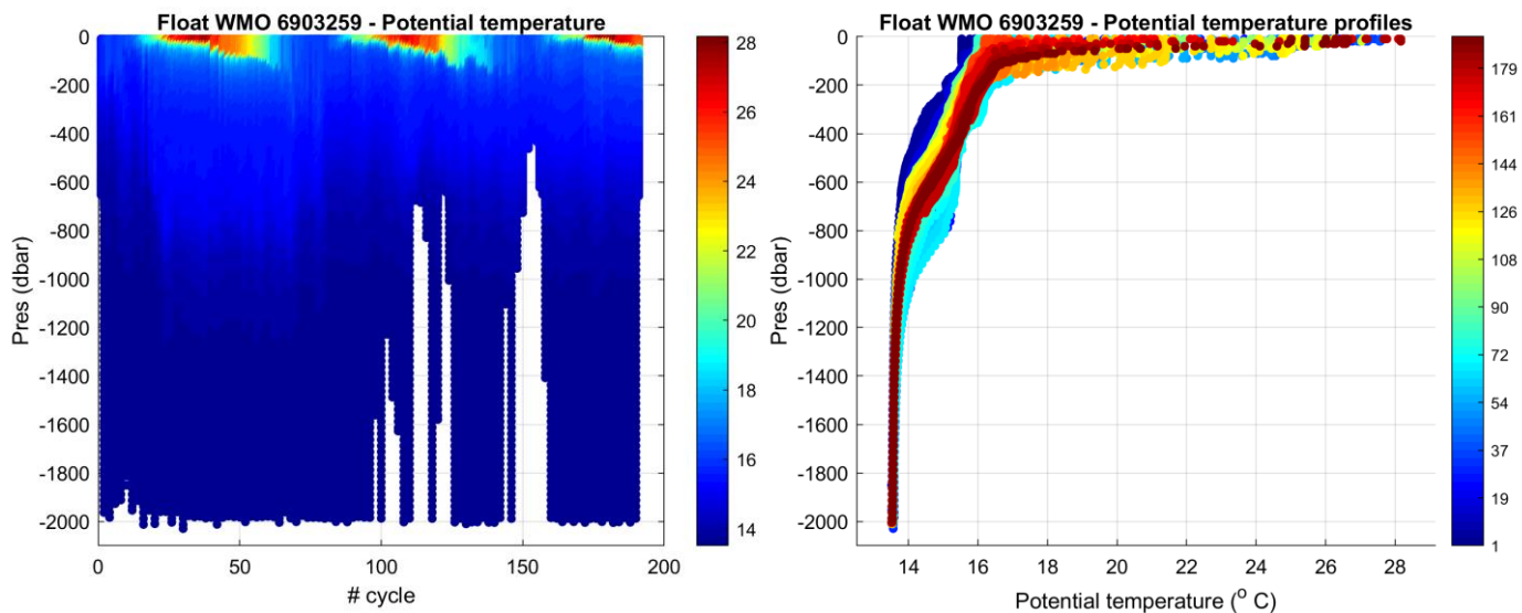
Figure 1: Float 6903259. Time series of Argo float potential temperature ( ^{\circ}\text{C} ) on the left, and potential temperature profiles color-coded per cycle number on the right.
