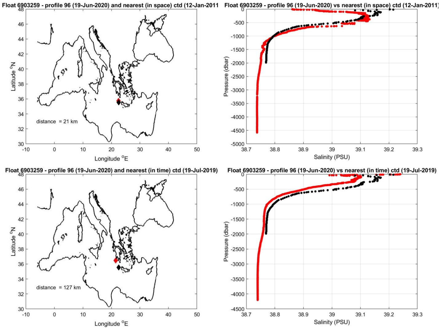
Figure 9: Float 6903259. The salinity float profile number 96 (black dots) are compared to the nearest in space (top) and in time (bottom) reference profile (red dots). The locations of the two profiles and their distance is given in the left panel.
