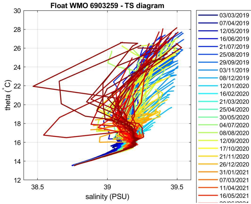
Figure 3: Float 6903259. \theta -S diagram color-coded per cycle number.
