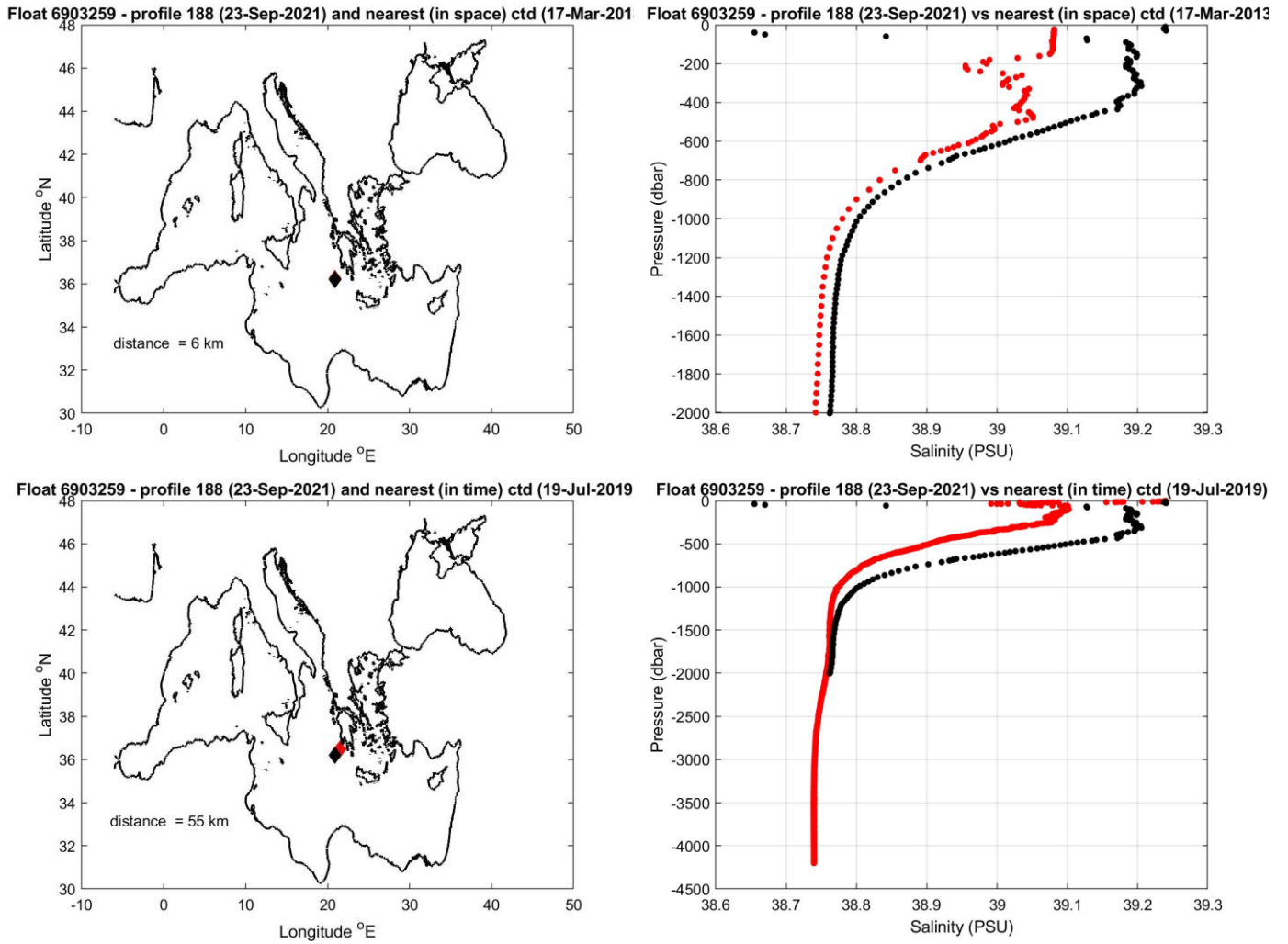
Figure 10: Float 6903259. The salinity float profile number 188 (black dots) are compared to the nearest in space (top) and in time (bottom) reference profile (red dots). The locations of the two profiles and their distance is given in the left panel.
