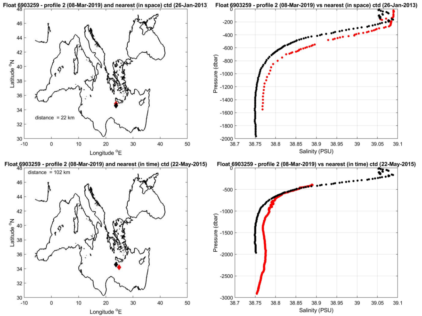
Figure 8: Float 6903259. The salinity float profile number 2 (black dots) are compared to the nearest in space (top) and in time (bottom) reference profile (red dots). The locations of the two profiles and their distance is given in the left panel.
