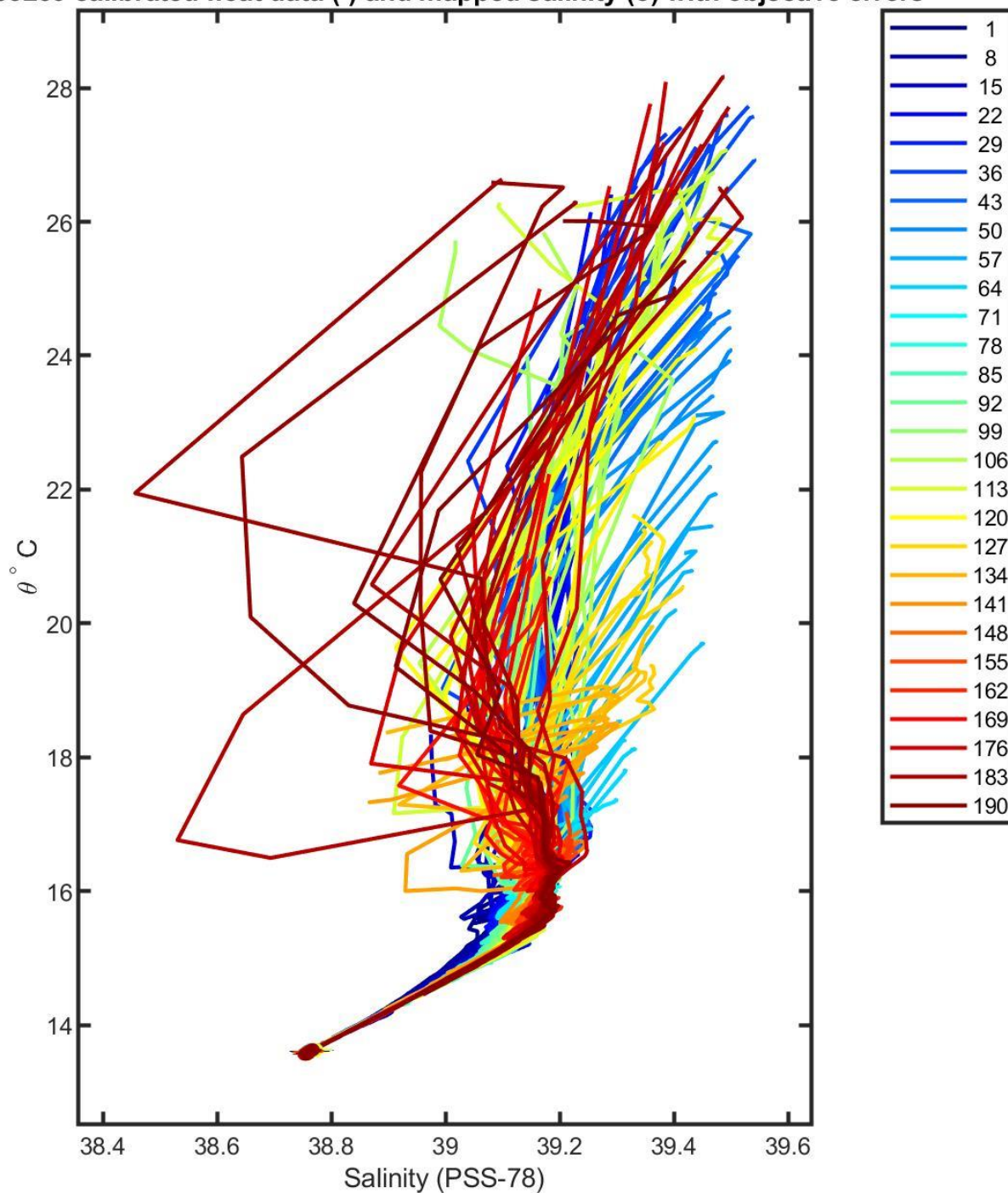
6903259 calibrated float data (-) and mapped salinity (o) with objective errors
