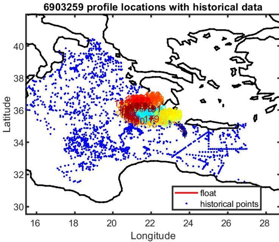
Figure 12: Float 6903259. Location of the float profiles (red line with colored numbers) and the reference data selected for mapping (blue dots).
