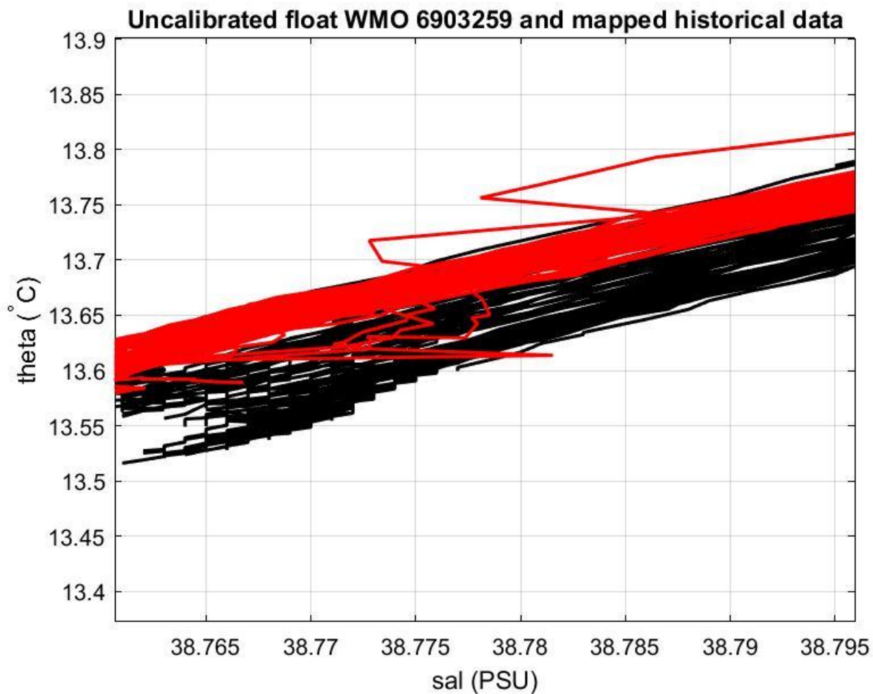
Figure 20: Float 6903259. Uncalibrated float salinity profile (black lines) and mapped historical data (red lines) in the most uniform part of the \theta -S curve.
