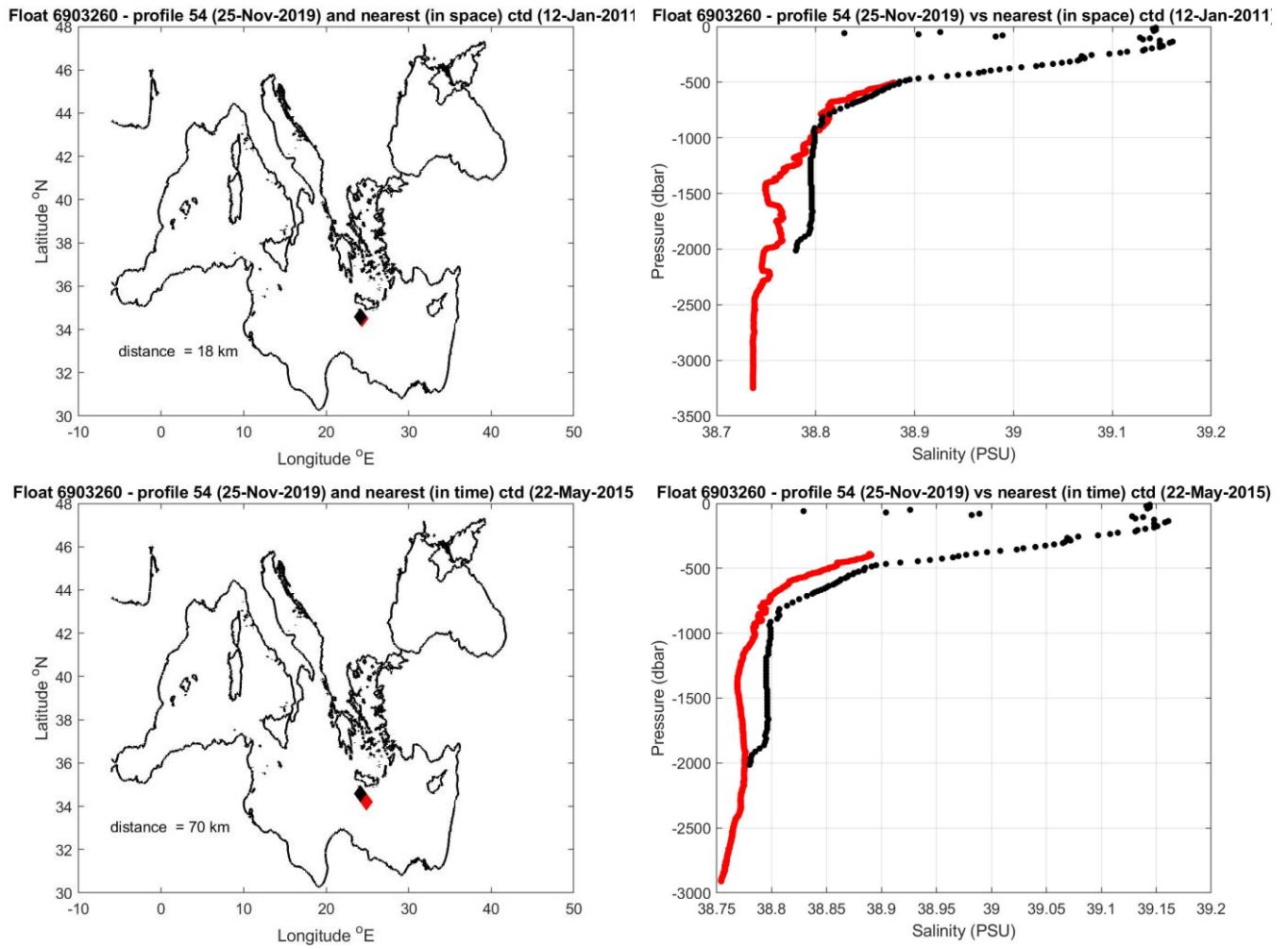
Figure 9: Float 6903260. The salinity float profile number 54 (black dots) are compared to the nearest in space (top) and in time (bottom) reference profile (red dots). The locations of the two profiles and their distance is given in the left panel.
