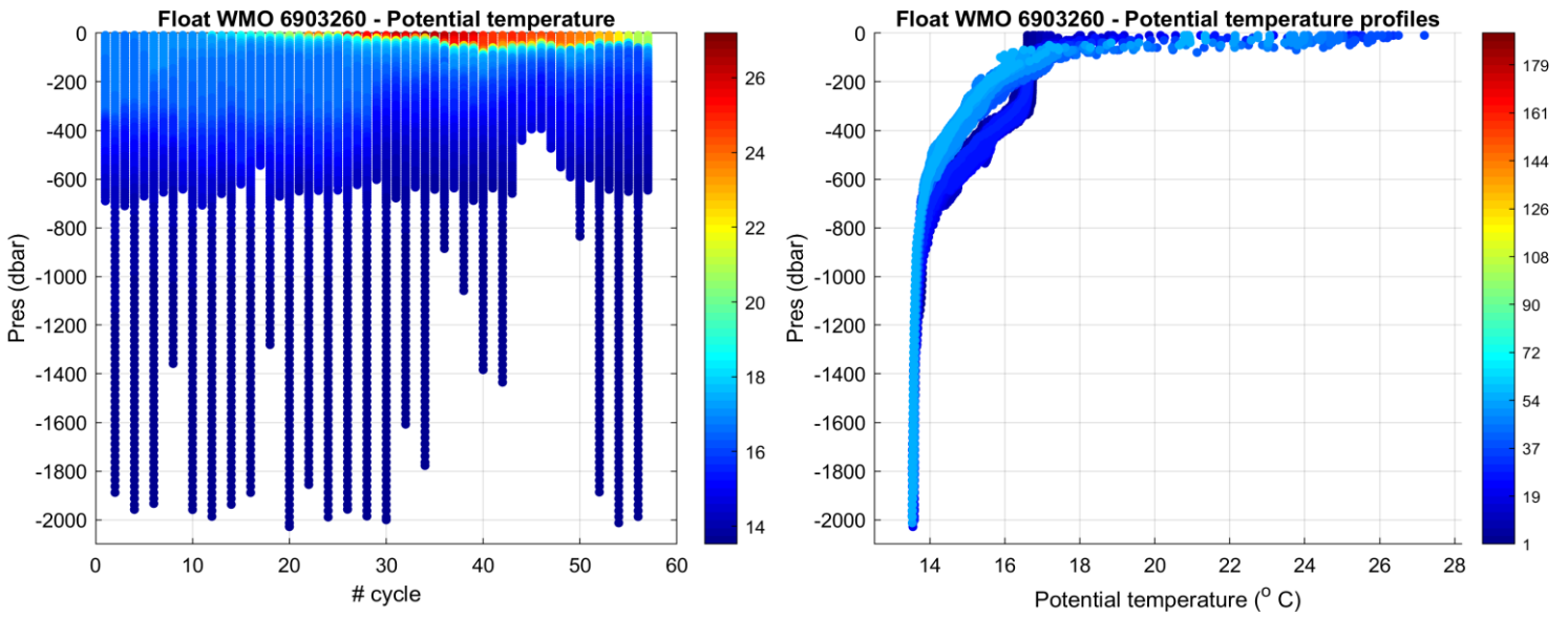
Figure 1: Float 6903260. Time series of Argo float potential temperature ( ^{\circ}\text{C} ) on the left, and potential temperature profiles color-coded per cycle number on the right.
