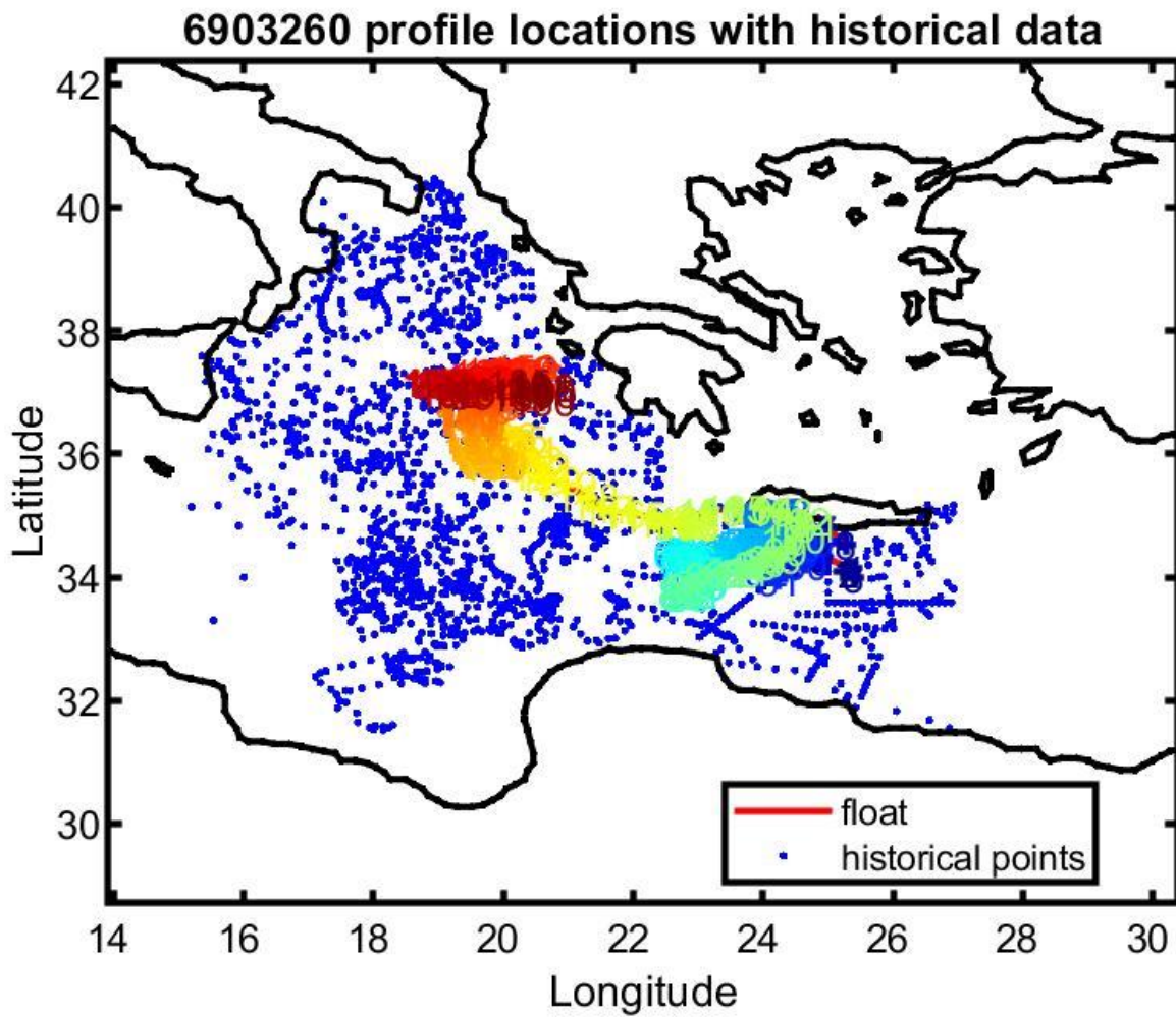
Figure 12: Float 6903260. Location of the float profiles (red line with colored numbers) and the reference data selected for mapping (blue dots).
