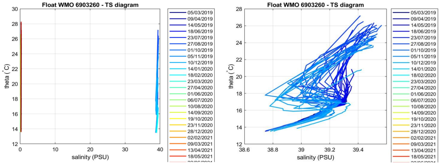
Figure 3: Float 6903260. \theta -S diagram color-coded per cycle number. On the left all cycles, on the right only cycles with QC 1 and QC 3.
