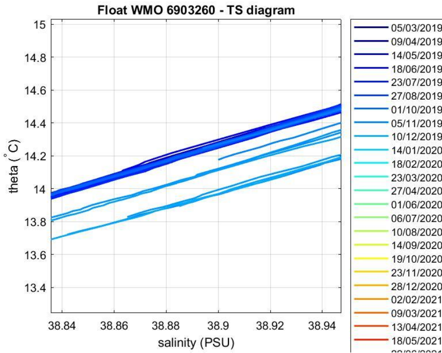
Figure 3: Float 6903260. \theta -S diagram color-coded per cycle number. On the left all cycles, on the right only cycles with QC 1 and QC 3.
