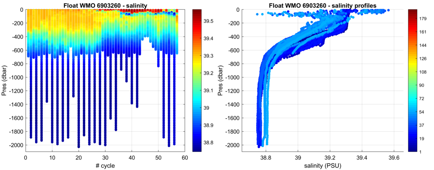
Figure 2: Float 6903260. Time series of Argo float potential salinity (PSS-78) on the left, and salinity profiles color-coded per cycle number on the right.
