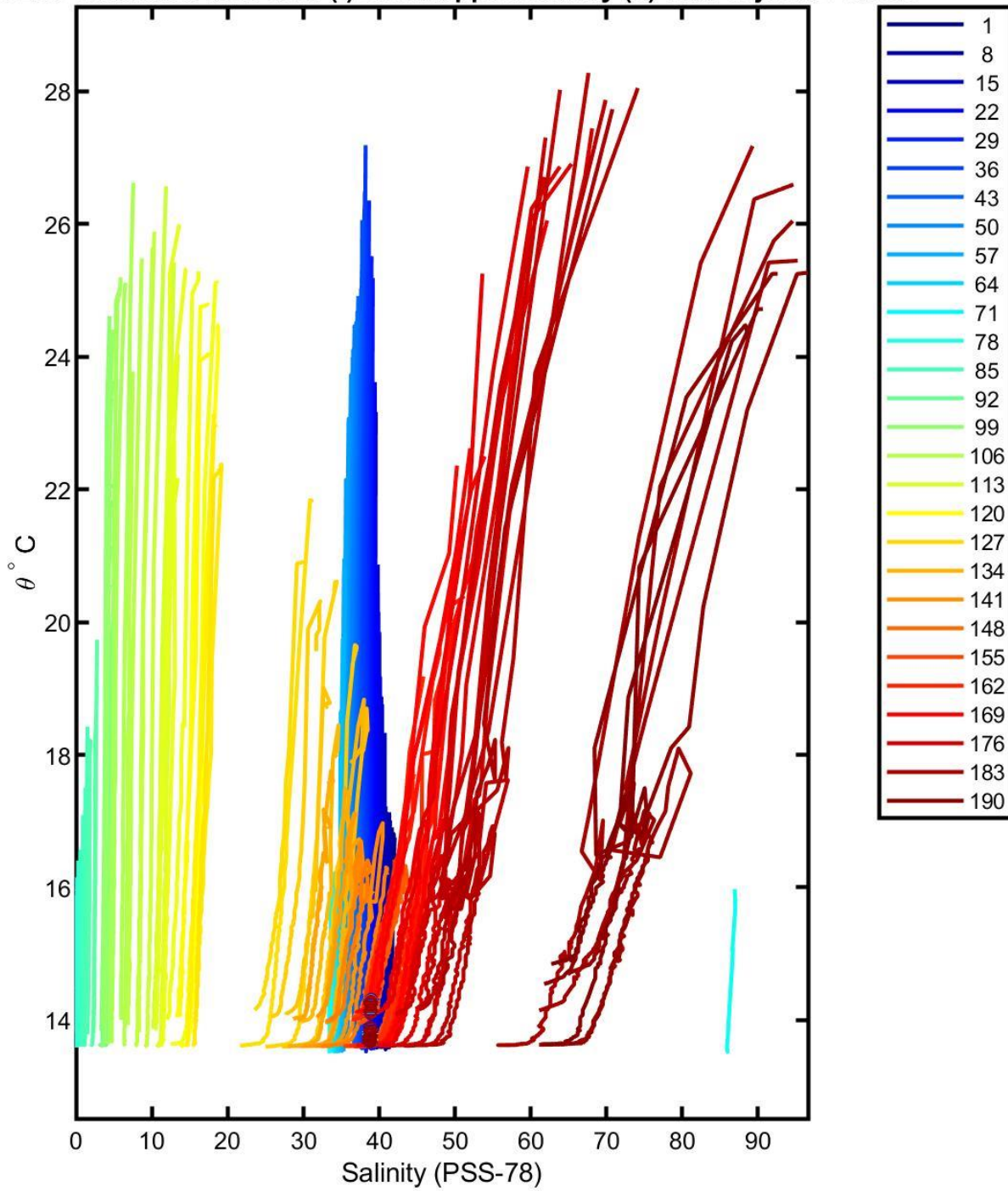
6903260 calibrated float data (-) and mapped salinity (o) with objective errors
