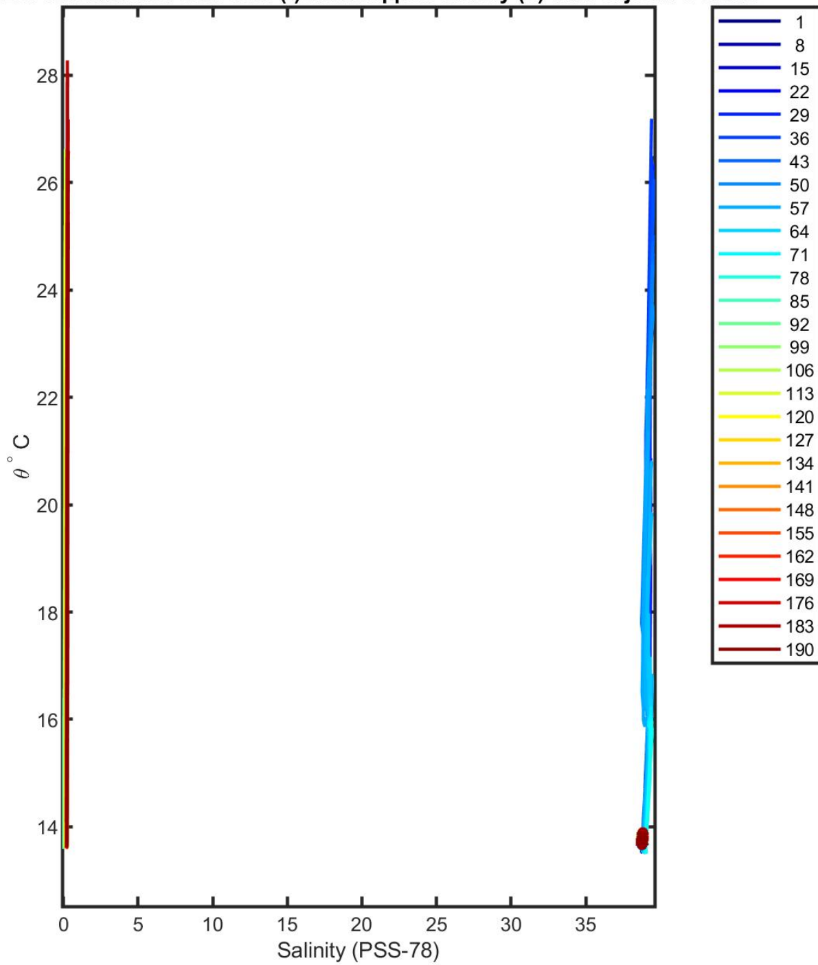
5903260 uncalibrated float data (-) and mapped salinity (o) with objective errors
