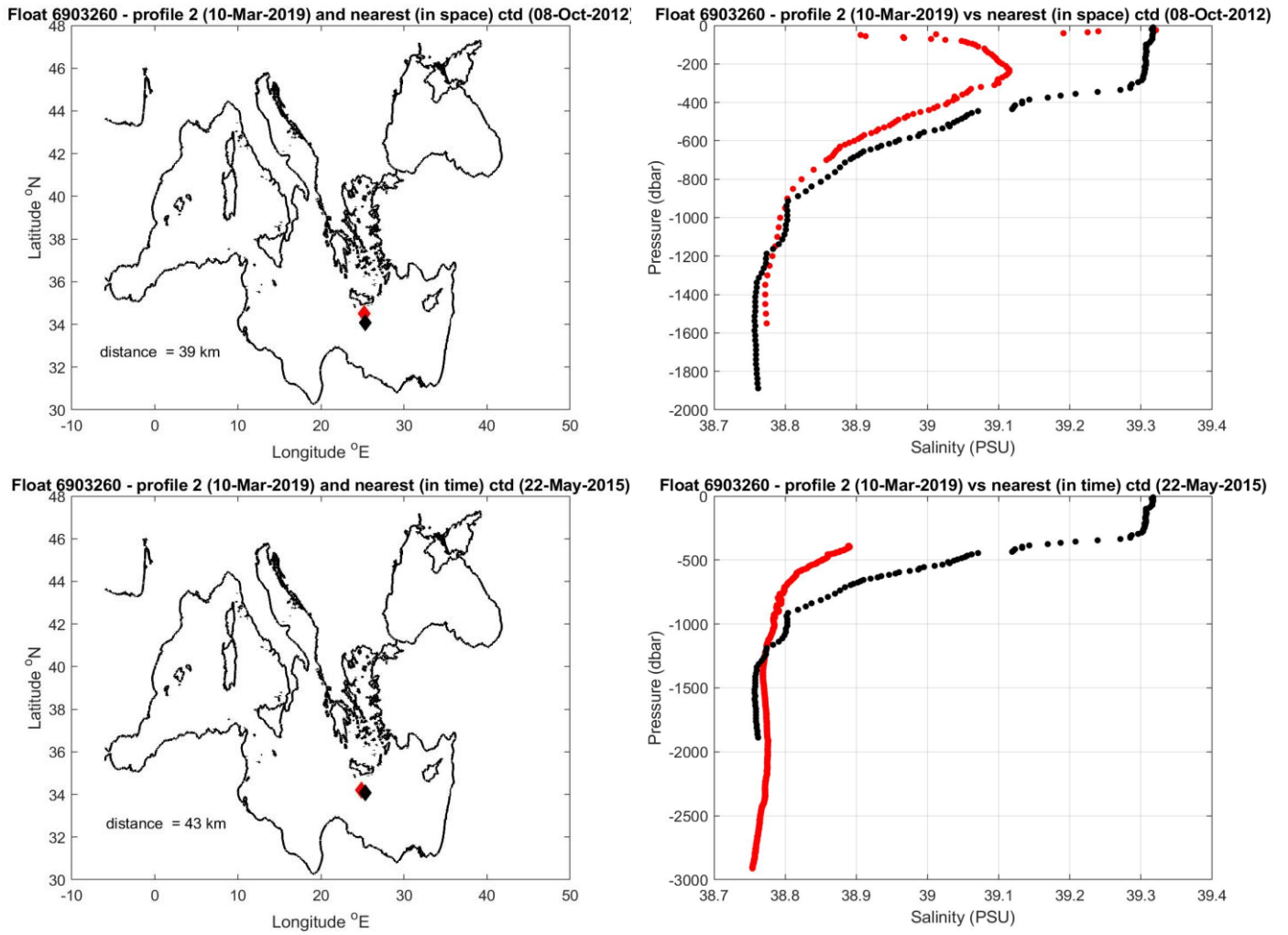
Figure 8: Float 6903260. The salinity float profile number 2 (black dots) are compared to the nearest in space (top) and in time (bottom) reference profile (red dots). The locations of the two profiles and their distance is given in the left panel.
