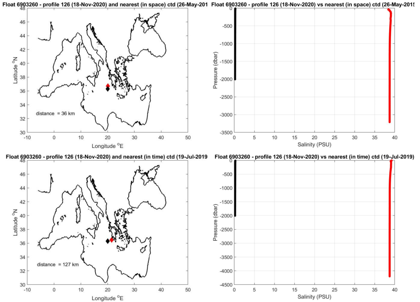
Figure 10: Float 6903260. The salinity float profile number 126 (black dots) are compared to the nearest in space (top) and in time (bottom) reference profile (red dots). The locations of the two profiles and their distance is given in the left panel.
