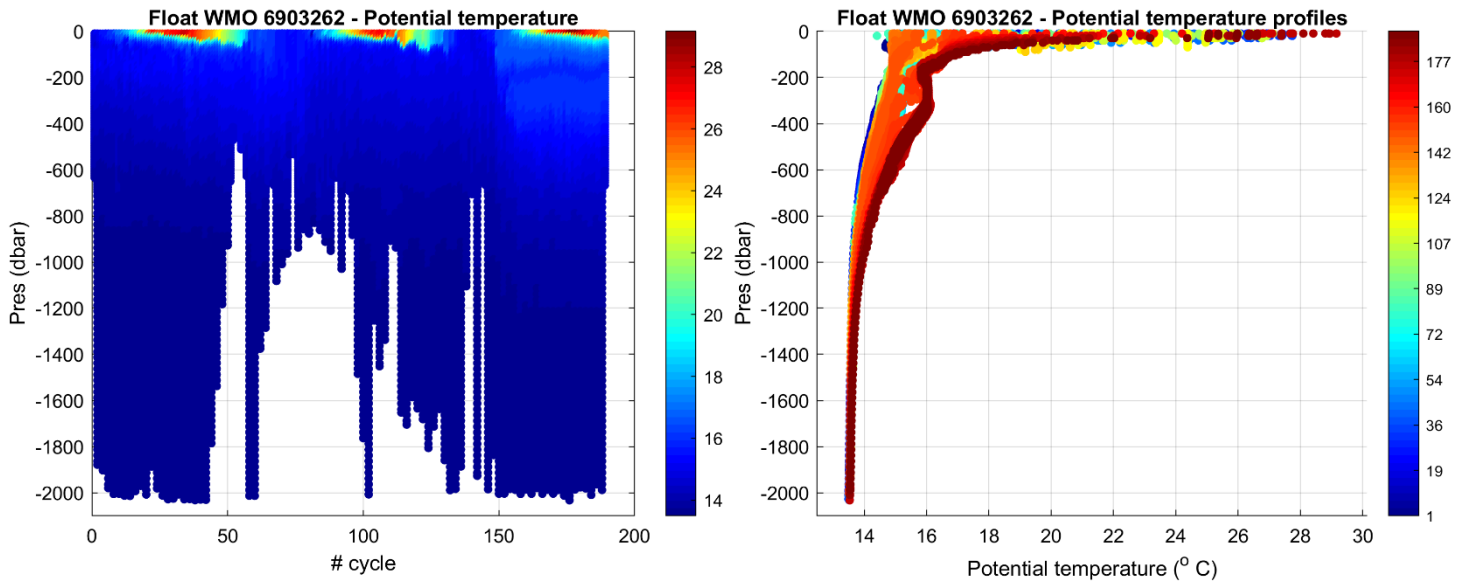
Figure 1: Float 6903262. Time series of Argo float potential temperature ( ^{\circ}\text{C} ) on the left, and potential temperature profiles color-coded per cycle number on the right.
