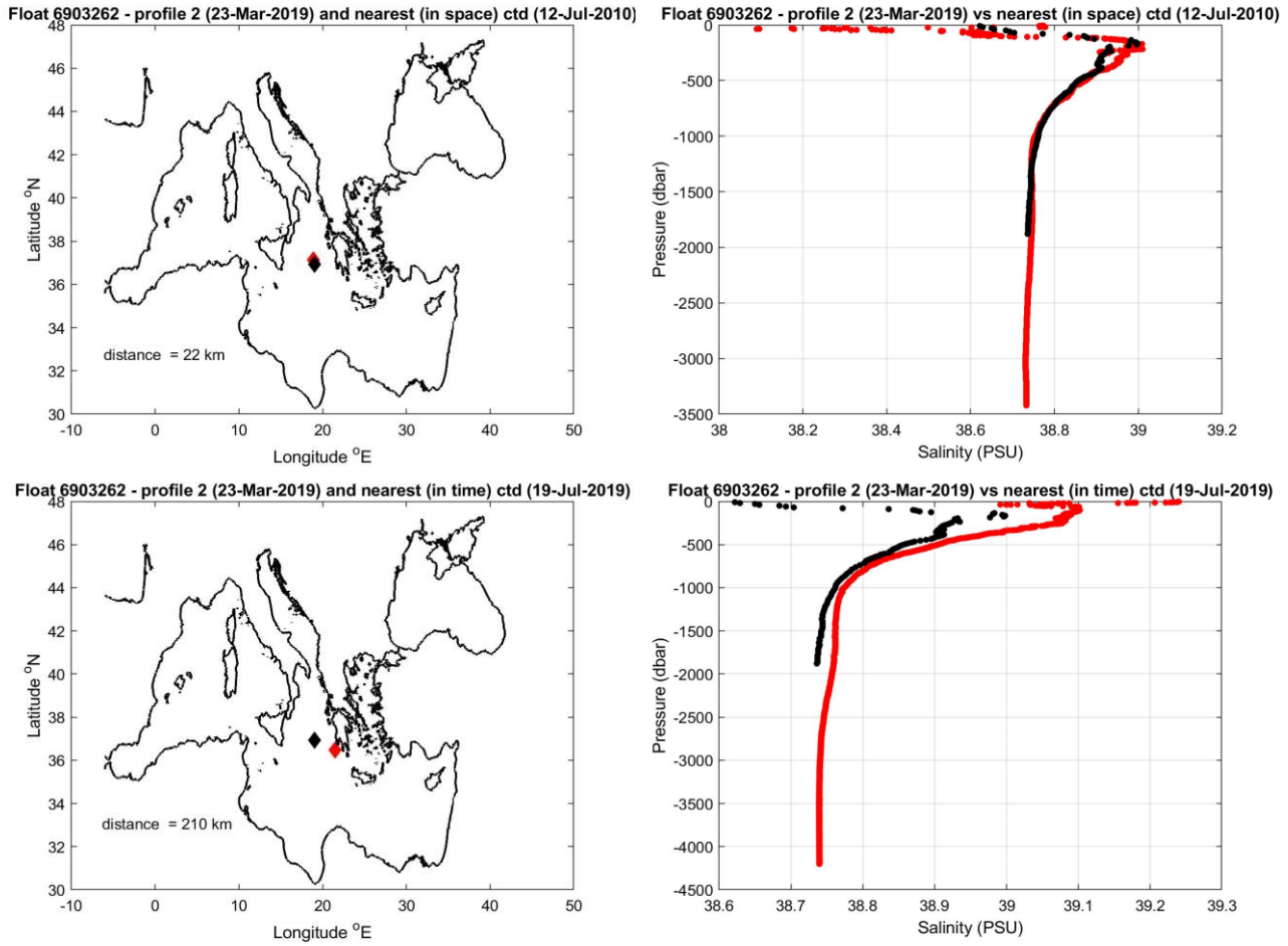
Figure 8: Float 6903262. The salinity float profile number 2 (black dots) are compared to the nearest in space (top) and in time (bottom) reference profile (red dots). The locations of the two profiles and their distance is given in the left panel.
