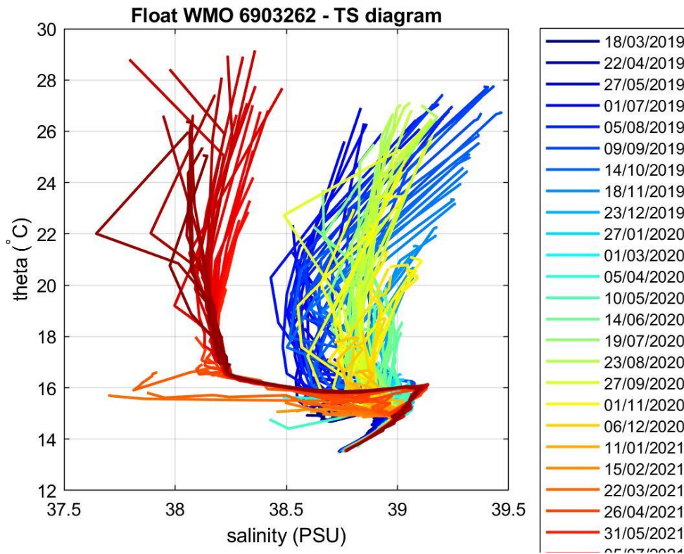
Figure 3: Float 6903262. \theta -S diagram color-coded per cycle number.
