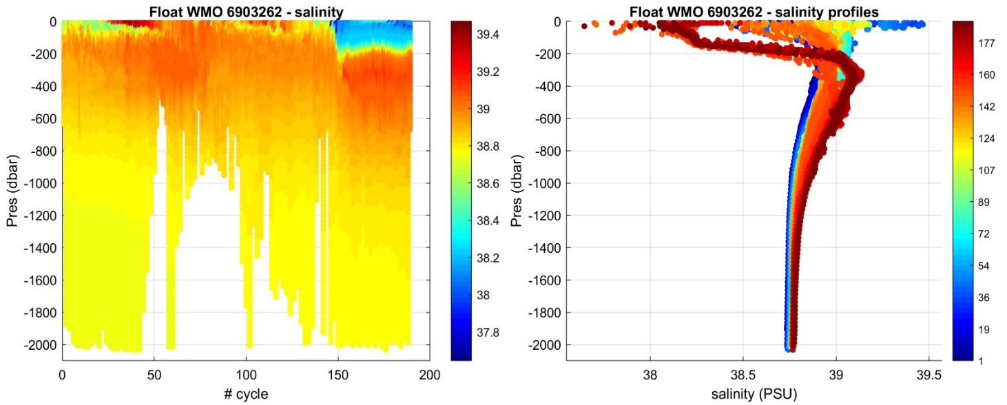
Figure 2: Float 6903262. Time series of Argo float potential salinity (PSS-78) on the left, and salinity profiles color-coded per cycle number on the right.
