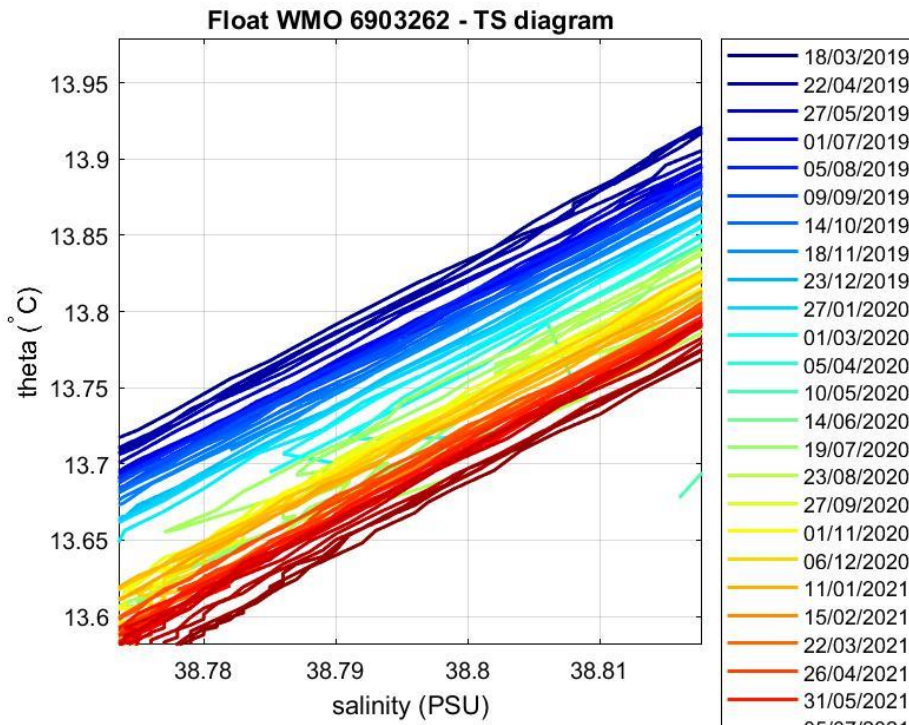
Figure 4: Float 6903262. Area of the \theta -S diagram (color-coded per cycle number) where the \theta -S relationship is more uniform.
