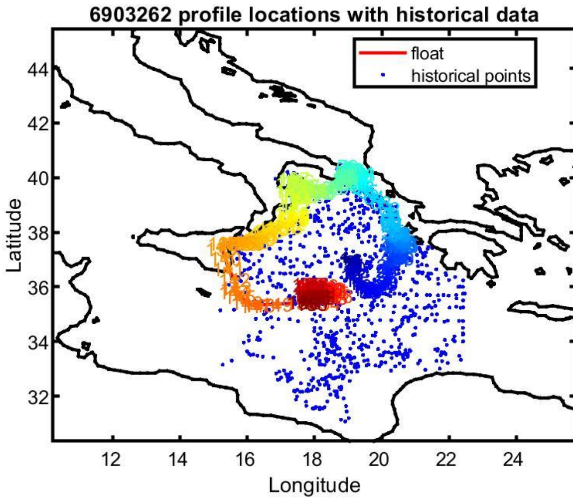
Figure 12: Float 6903262. Location of the float profiles (red line with colored numbers) and the reference data selected for mapping (blue dots).
