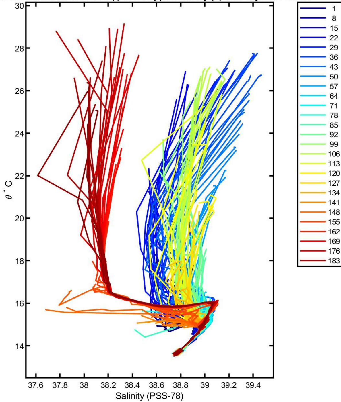
6903262 calibrated float data (-) and mapped salinity (o) with objective errors
