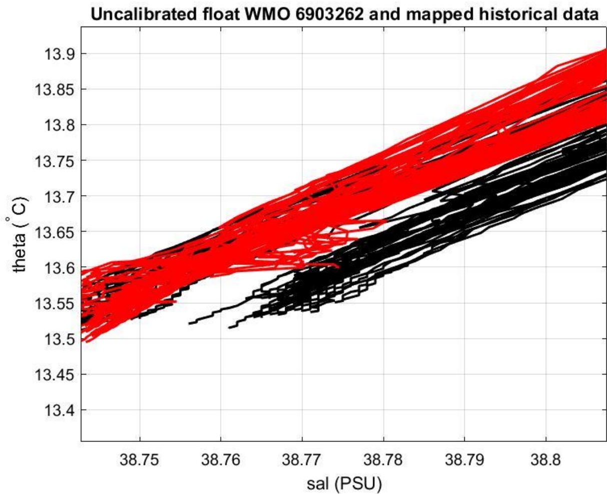
Figure 20: Float 6903262. Uncalibrated float salinity profile (black lines) and mapped historical data (red lines) in the most uniform part of the \theta -S curve.
