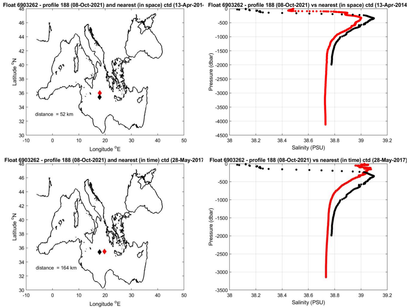
Figure 10: Float 6903262. The salinity float profile number 188 (black dots) are compared to the nearest in space (top) and in time (bottom) reference profile (red dots). The locations of the two profiles and their distance is given in the left panel.
