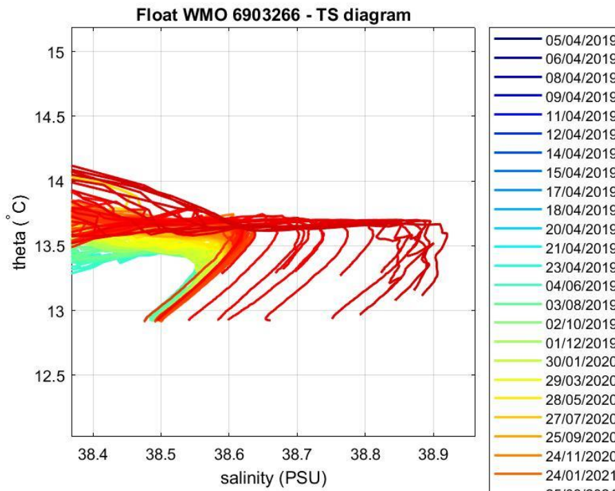
Figure 4: Float 6903266. Area of the \theta -S diagram (color-coded per cycle number) where the \theta -S relationship is more uniform.
