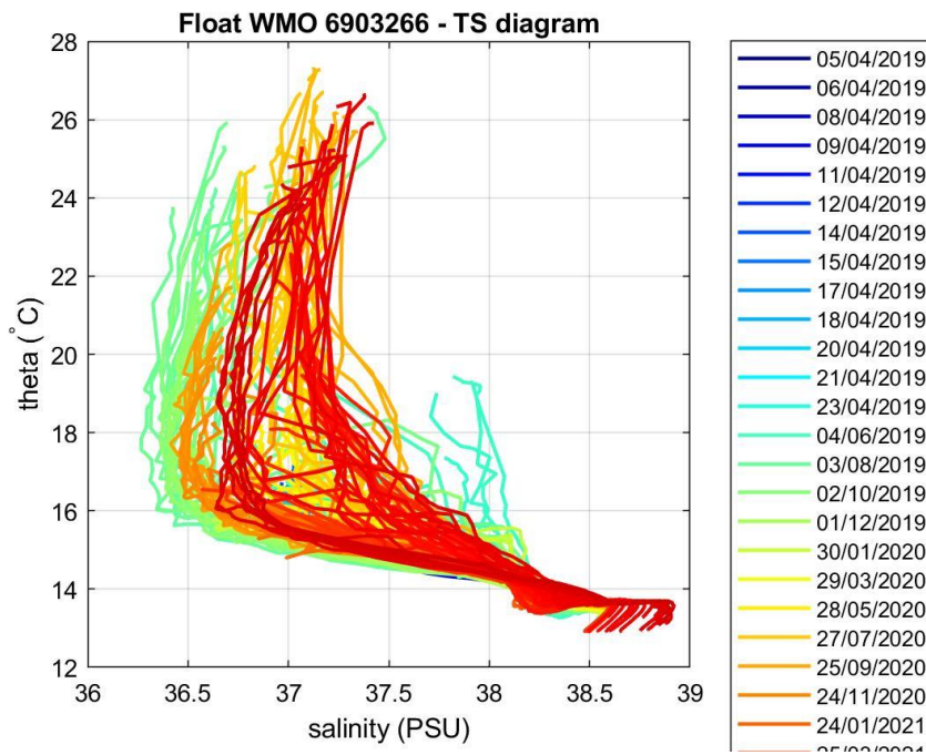
Figure 3: Float 6903266. \theta -S diagram color-coded per cycle number.
