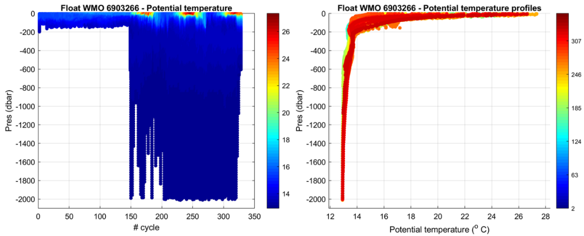
Figure 1: Float 6903266. Time series of Argo float potential temperature ( ^{\circ}\text{C} ) on the left, and potential temperature profiles color-coded per cycle number on the right.
