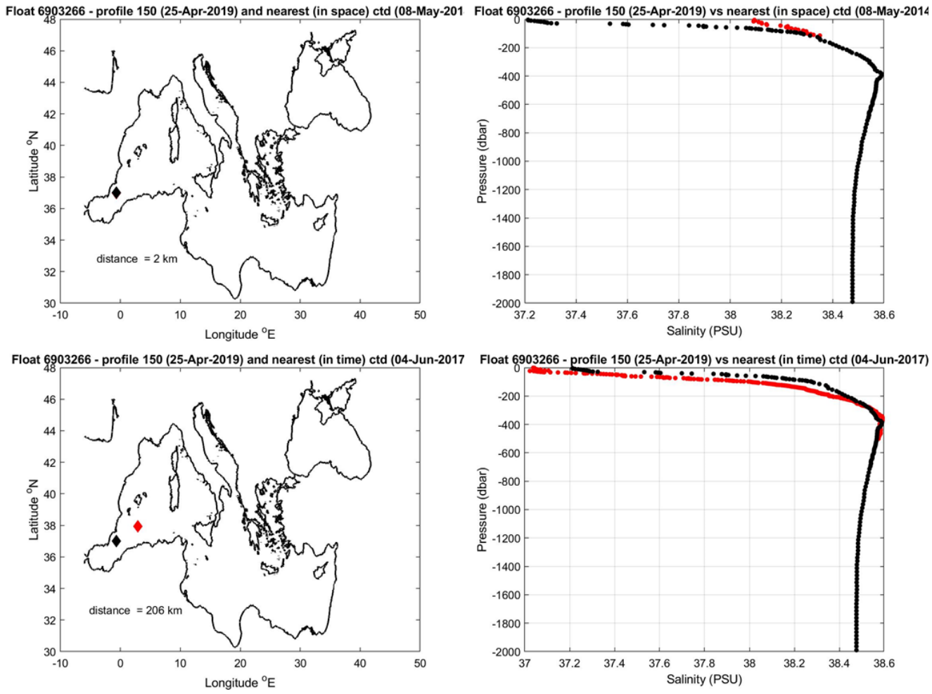
Figure 9: Float 6903266. The salinity float profile number 150 (black dots) are compared to the nearest in space (top) and in time (bottom) reference profile (red dots). The locations of the two profiles and their distance is given in the left panel.
