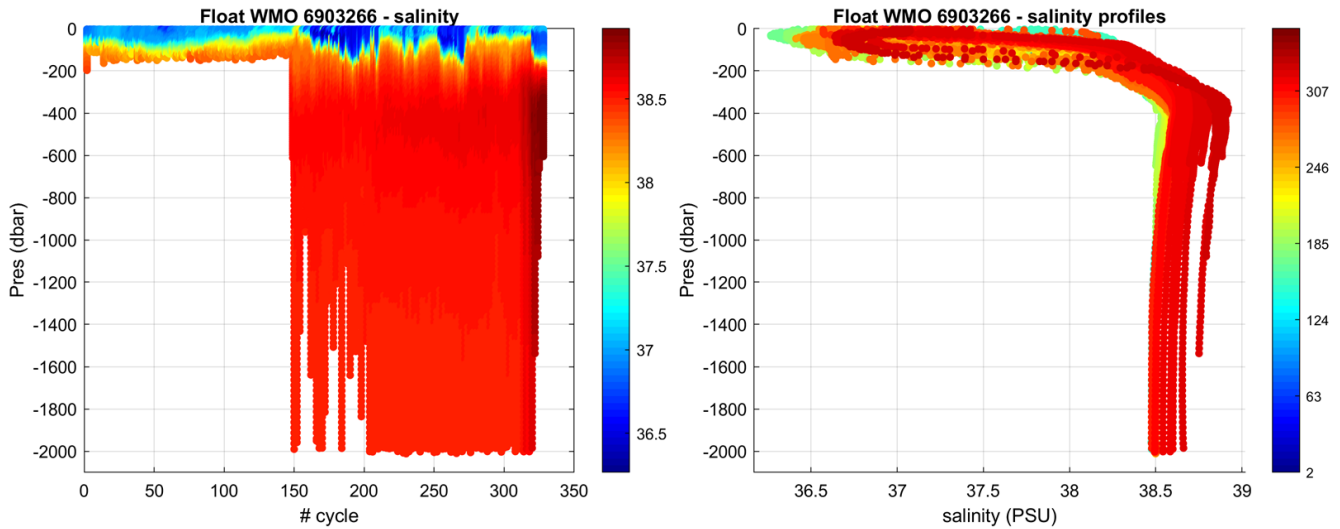
Figure 2: Float 6903266. Time series of Argo float potential salinity (PSS-78) on the left, and salinity profiles color-coded per cycle number on the right.
