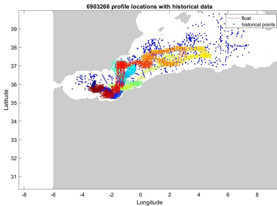
Figure 13: Float 6903266. Location of the float profiles (red line with colored numbers) and the reference data selected for mapping (blue dots).
