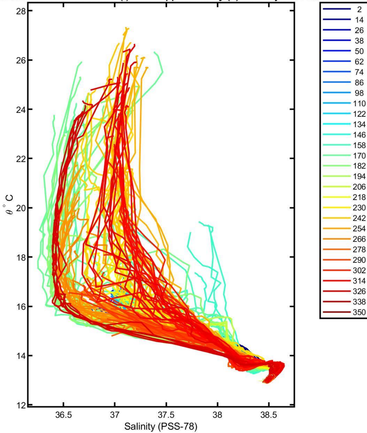
6903266 calibrated float data (-) and mapped salinity (o) with objective errors
