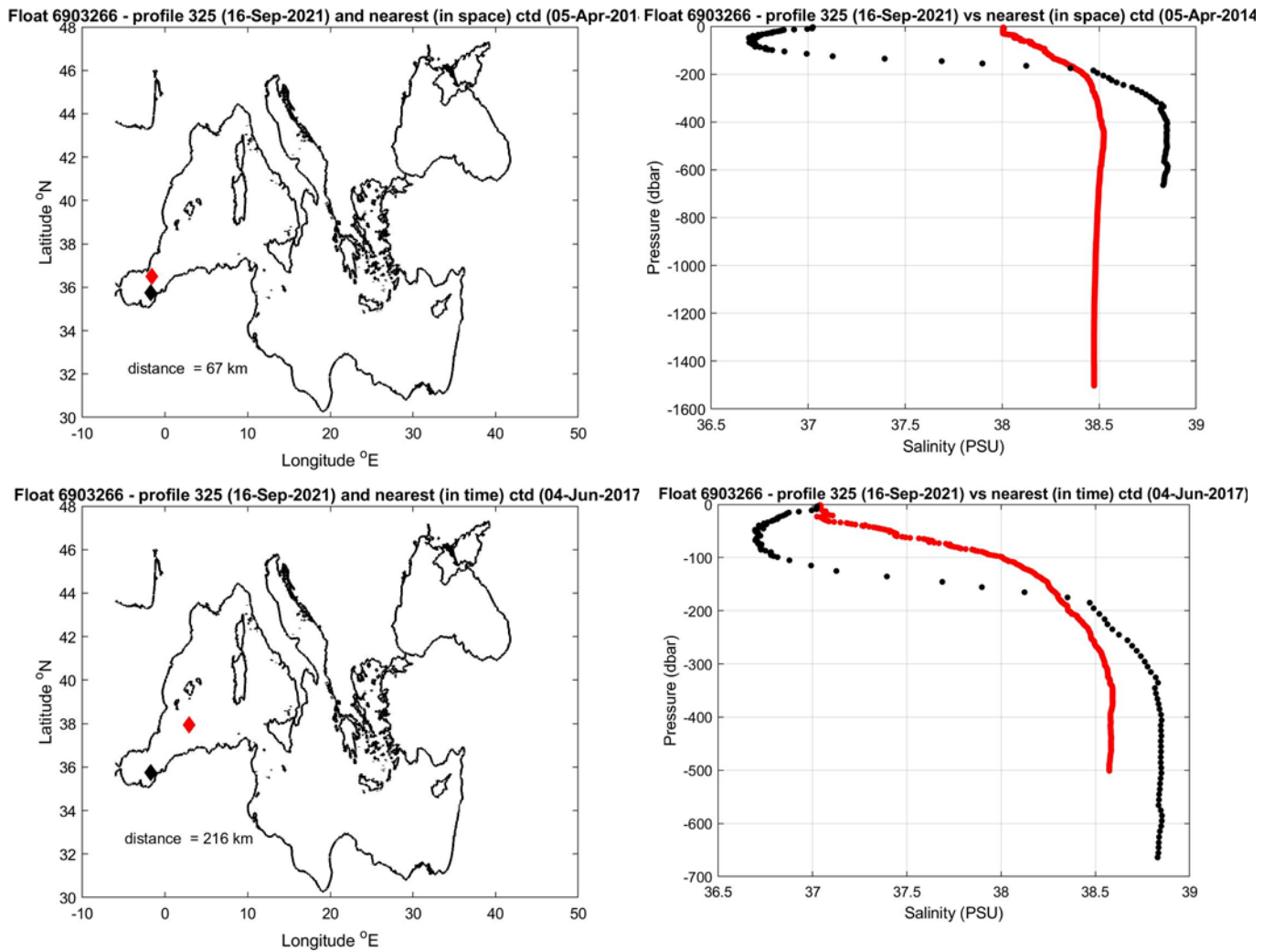
Figure 10: Float 6903266. The salinity float profile number 325 (black dots) are compared to the nearest in space (top) and in time (bottom) reference profile (red dots). The locations of the two profiles and their distance is given in the left panel.
