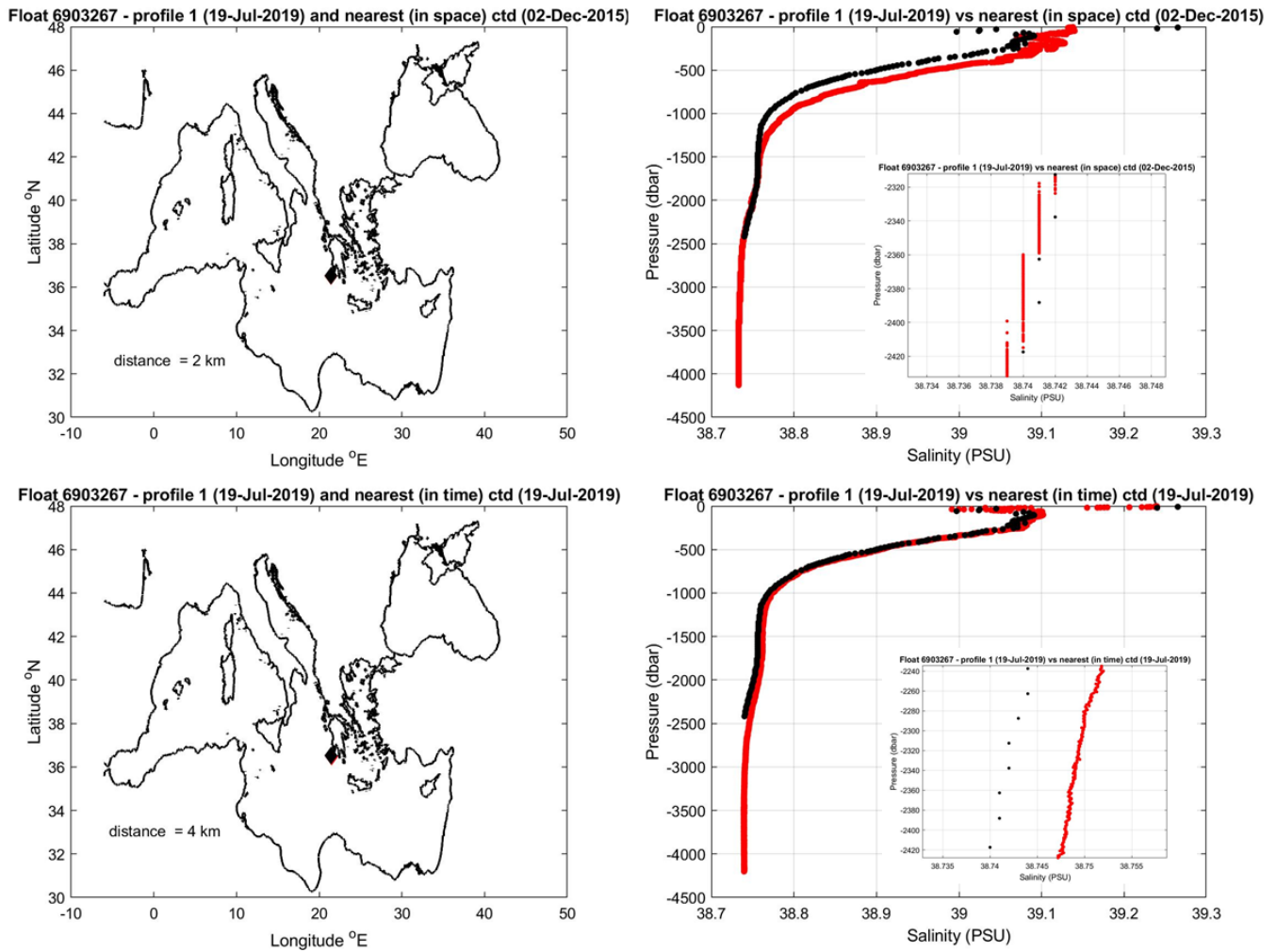
Figure 2: Float 6903267. The salinity float profile number 1 (black dots) are compared to the nearest in space (top) and in time (bottom) reference profile (red dots). The small plots show the comparison in the deeper layers. The locations of the two profiles and their distance is given in the left panel.
