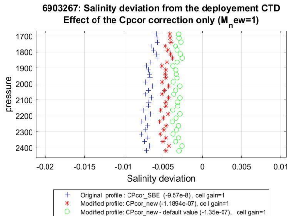
Figure 3: Float 6903267. Effect of the Cpcor correction: salinity deviation using the nominal CPcor (blue), the default value (green), the optimized value (red).
