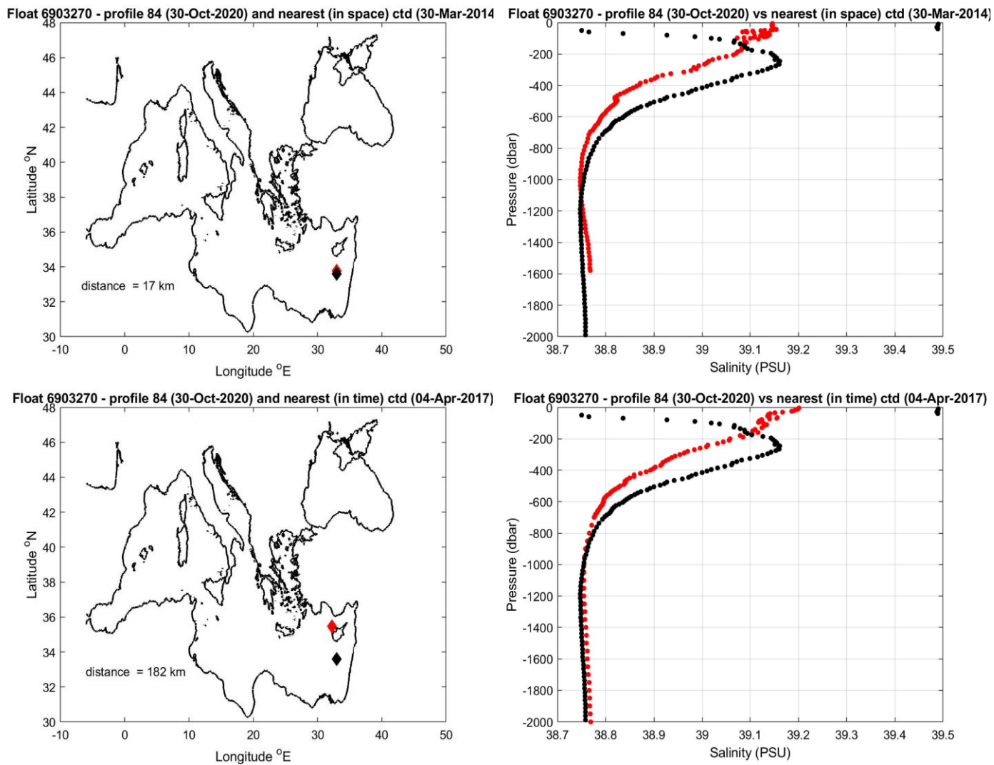
Figure 9: Float 6903270. The salinity float profile number 84 (black dots) are compared to the nearest in space (top) and in time (bottom) reference profile (red dots). The locations of the two profiles and their distance is given in the left panel.
