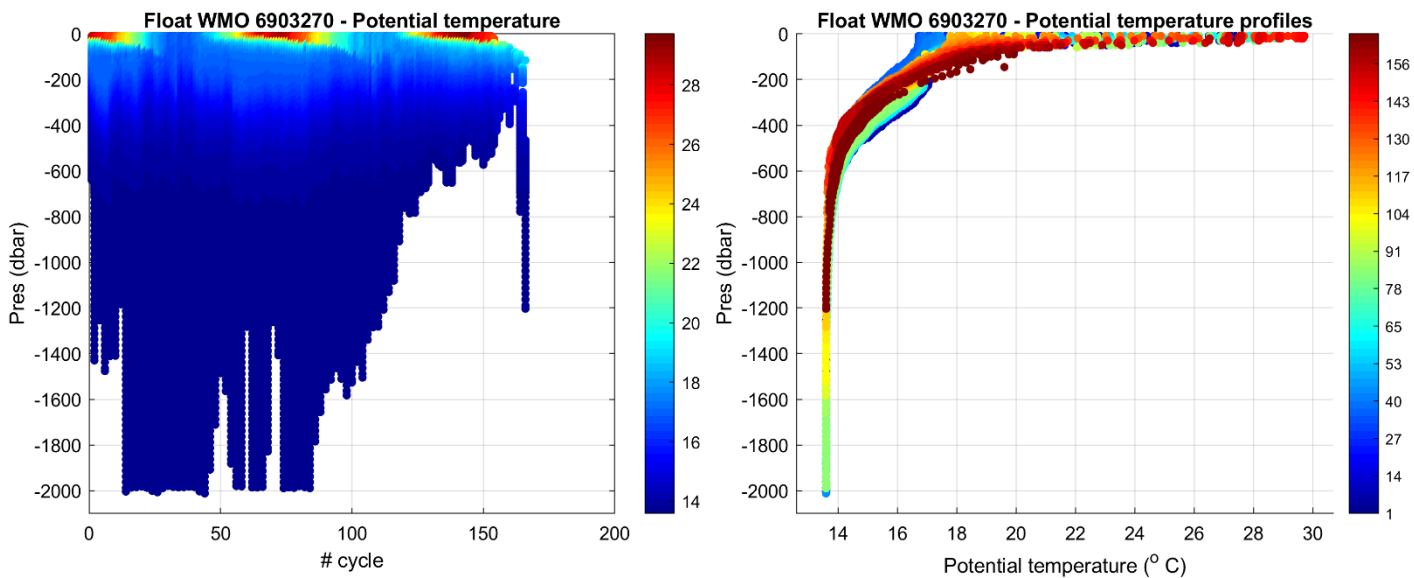
Figure 1: Float 6903270. Time series of Argo float potential temperature ( ^{\circ}\text{C} ) on the left, and potential temperature profiles color-coded per cycle number on the right.
