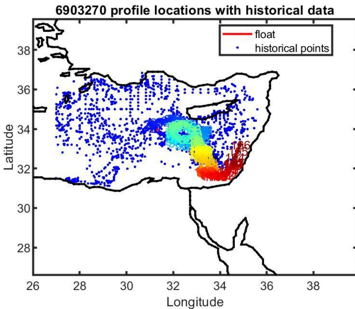
Figure 13: Float 6903270. Location of the float profiles (red line with colored numbers) and the reference data selected for mapping (blue dots).
