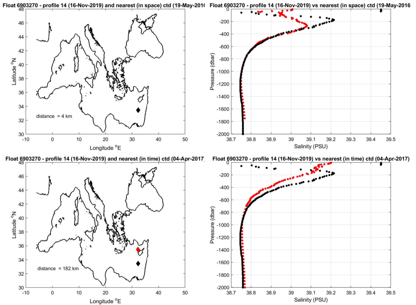
Figure 8: Float 6903270. The salinity float profile number 14 (black dots) are compared to the nearest in space (top) and in time (bottom) reference profile (red dots). The locations of the two profiles and their distance is given in the left panel.
