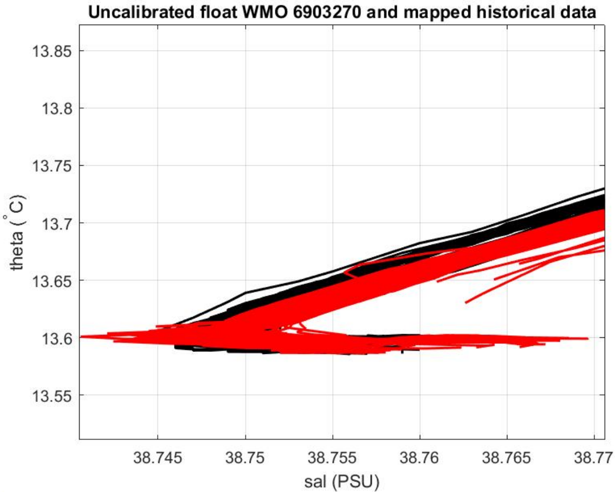
Figure 19: Float 6903270. Uncalibrated float salinity profile (black lines) and mapped historical data (red lines) in the most uniform part of the \theta -S curve.
