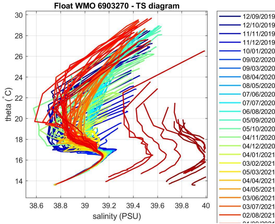
Figure 3: Float 6903270. \theta -S diagram color-coded per cycle number.
