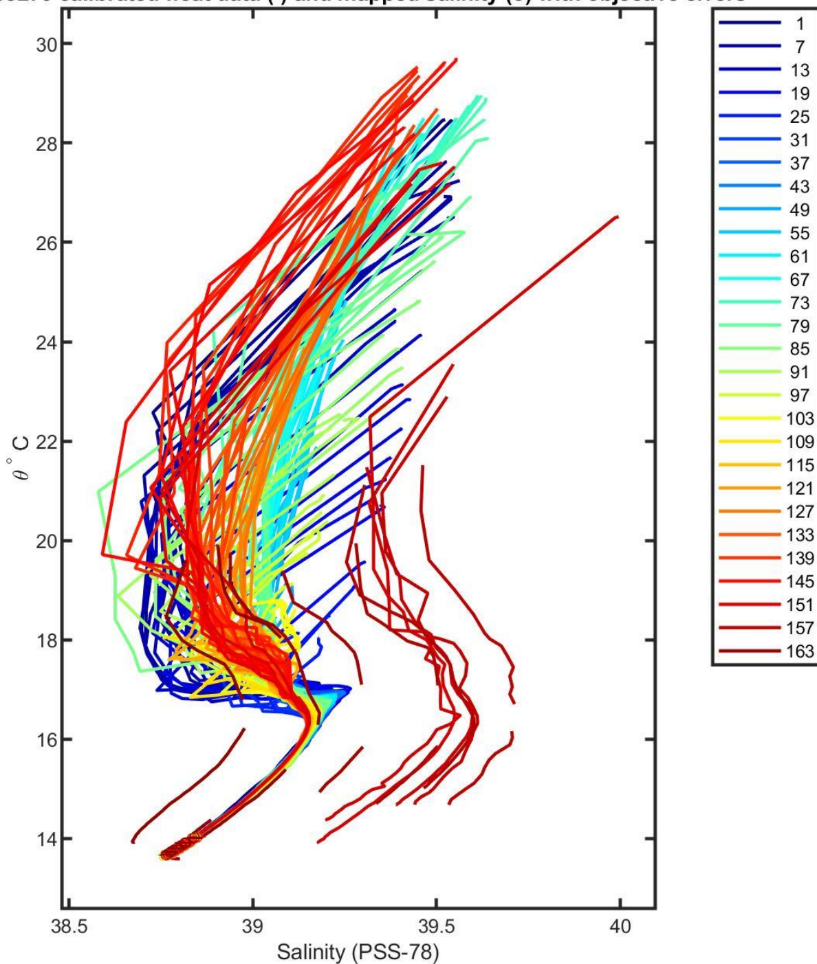
6903270 calibrated float data (-) and mapped salinity (o) with objective errors
