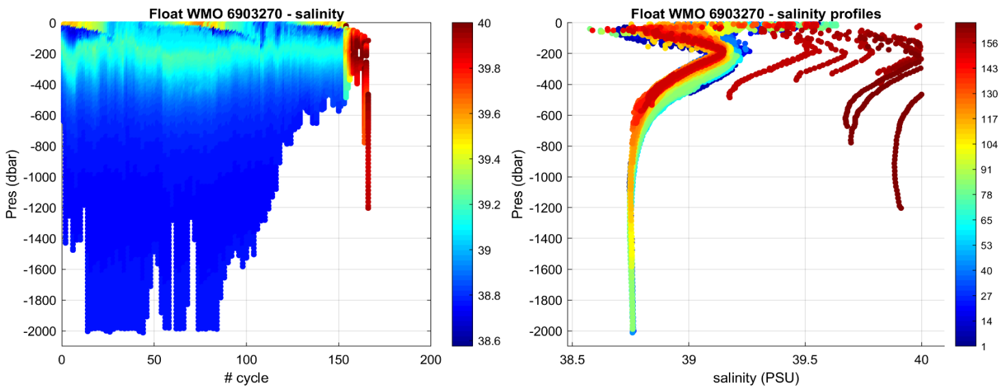
Figure 2: Float 6903270. Time series of Argo float potential salinity (PSS-78) on the left, and salinity profiles color-coded per cycle number on the right.
