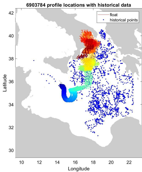
Figure 1: Location of the float profiles (red line with colored numbers) and the reference data selected for mapping (blue dots).
