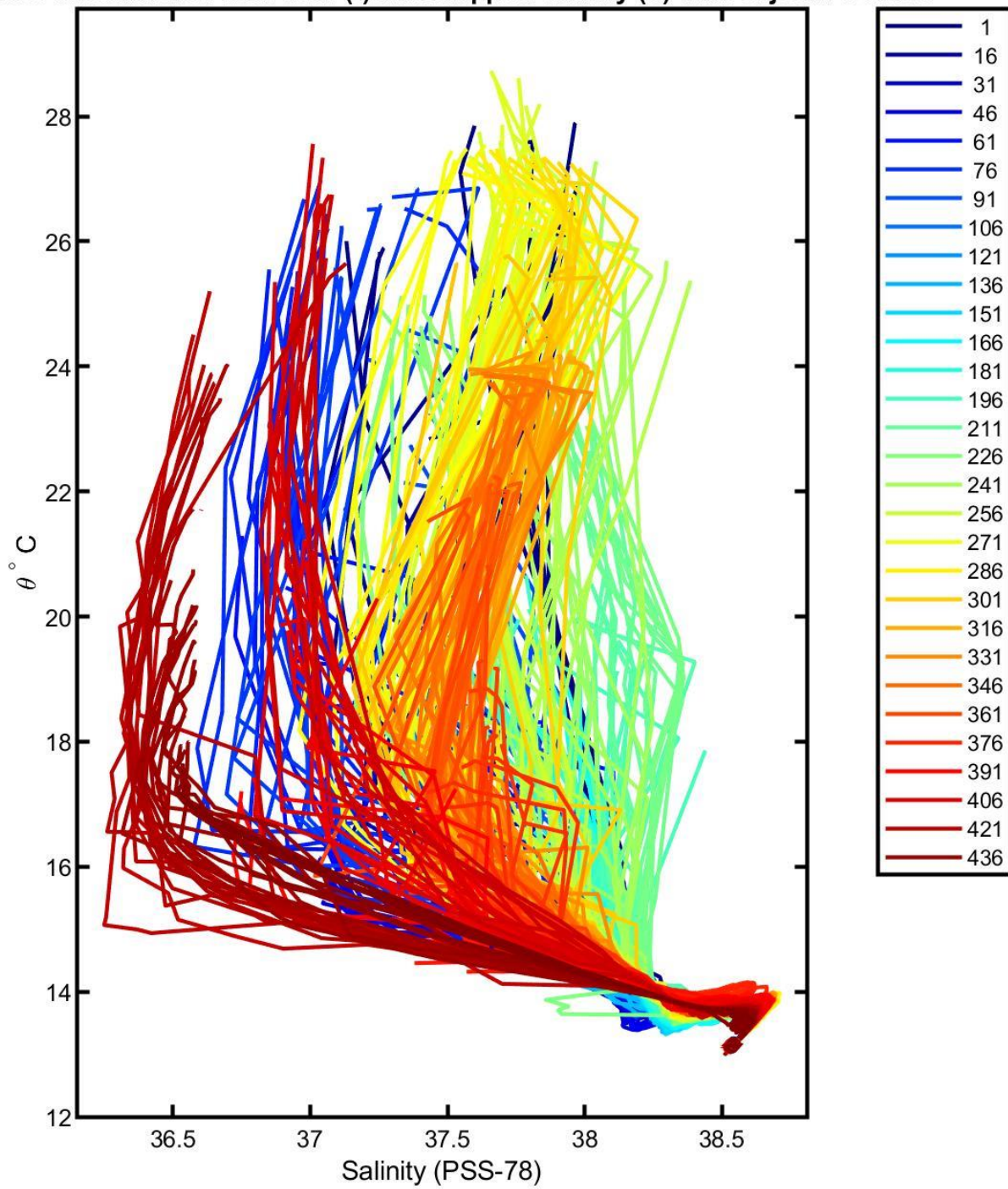
3904065 uncalibrated float data (-) and mapped salinity (o) with objective errors
