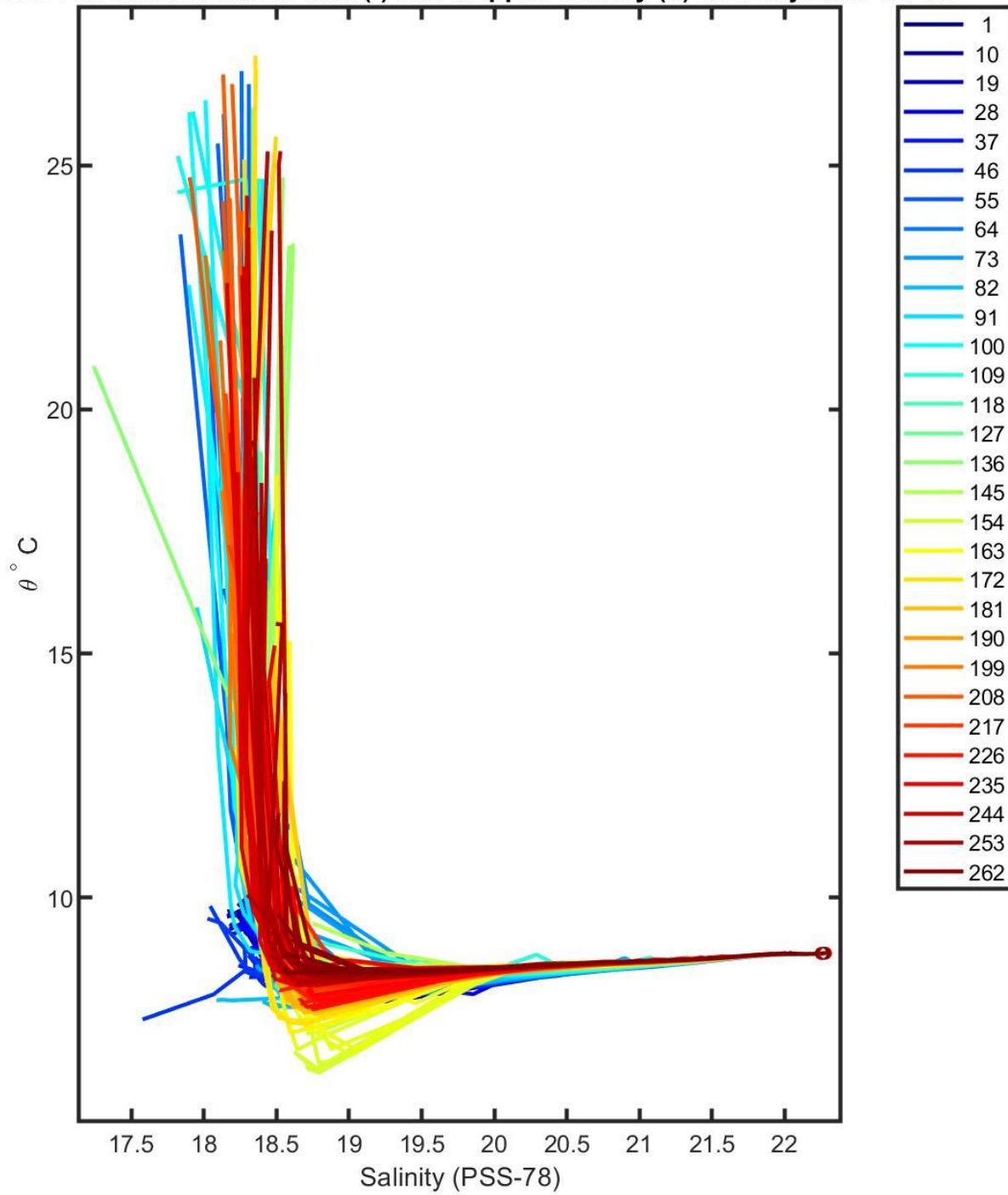
7900591 uncalibrated float data (-) and mapped salinity (o) with objective errors
