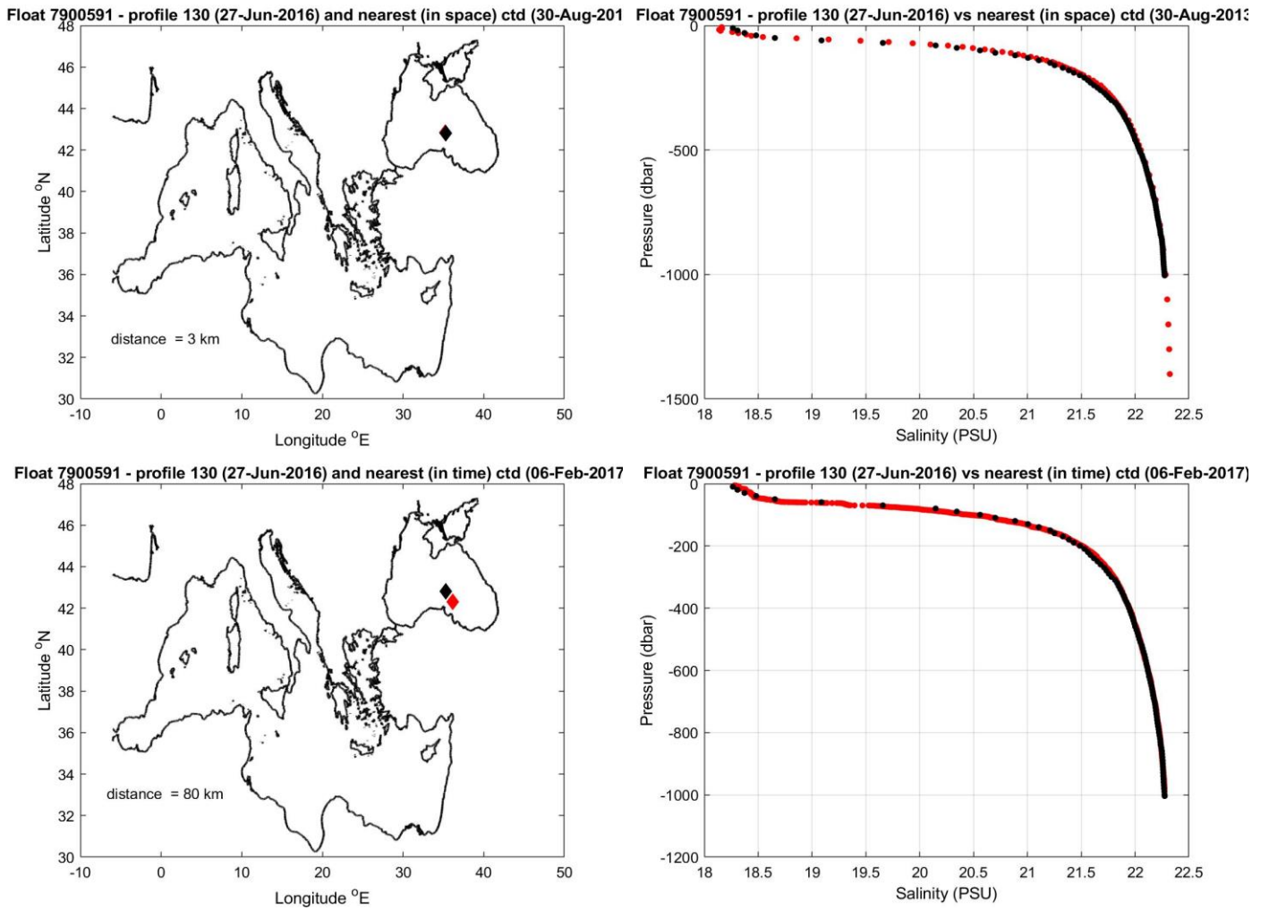
Figure 10: Float 7900591. The salinity float profile number 130 (black dots) are compared to the nearest in space (top) and in time (bottom) reference profile (red dots). The locations of the two profiles and their distance is given in the left panel.
