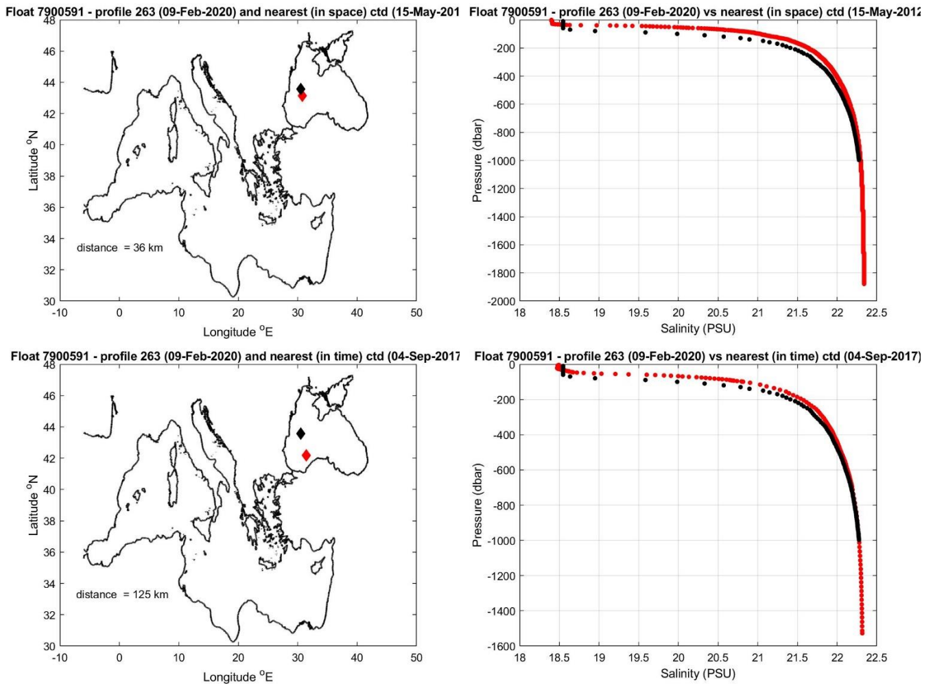
Figure 11: Float 7900591. The salinity float profile number 263 (black dots) are compared to the nearest in space (top) and in time (bottom) reference profile (red dots). The locations of the two profiles and their distance is given in the left panel.
