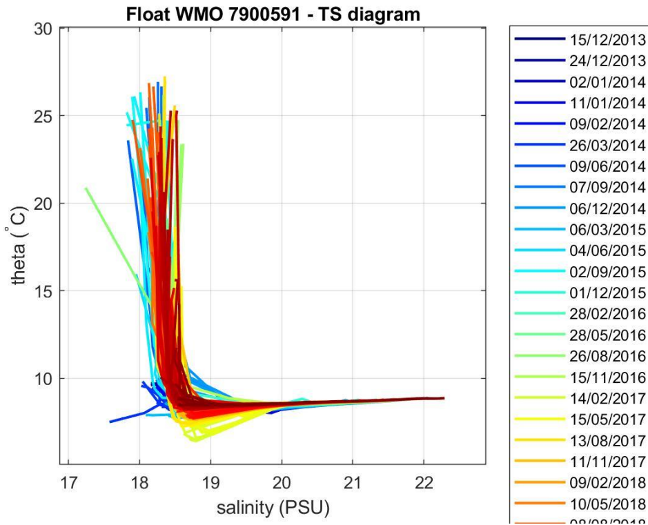
Figure 4: Float 7900591. \theta -S diagram color-coded per cycle number.
