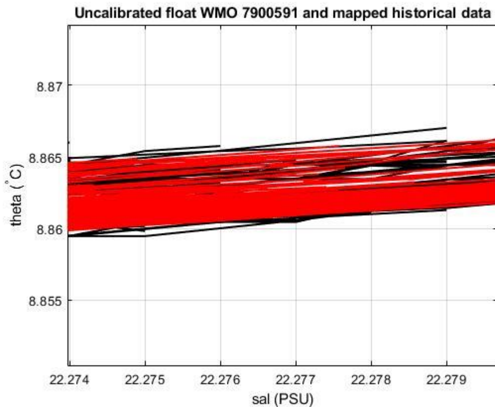
Figure 19: Float 7900591. Uncalibrated float salinity profile (black lines) and mapped historical data (red lines) in the most uniform part of the \theta -S curve.
