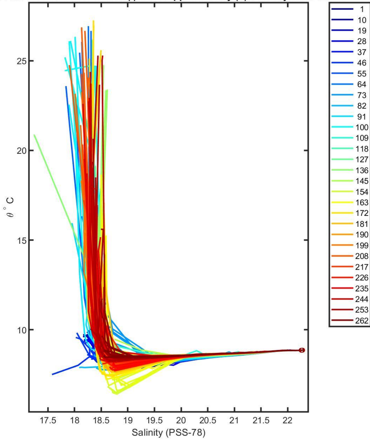
7900591 calibrated float data (-) and mapped salinity (o) with objective errors
