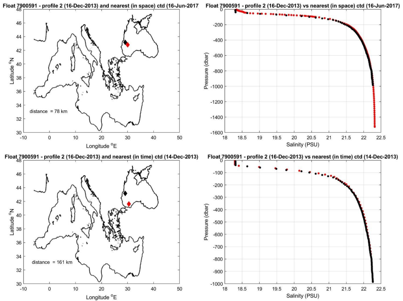
Figure 9: Float 7900591. The salinity float profile number 2 (black dots) are compared to the nearest in space (top) and in time (bottom) reference profile (red dots). The locations of the two profiles and their distance is given in the left panel.
