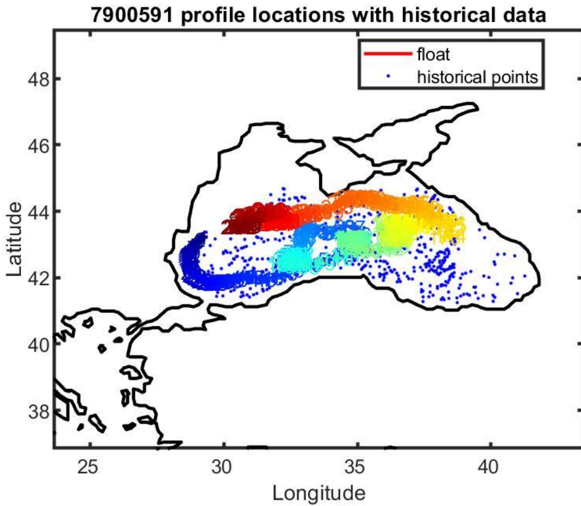
Figure 13: Float 7900591. Location of the float profiles (red line with colored numbers) and the reference data selected for mapping (blue dots).
