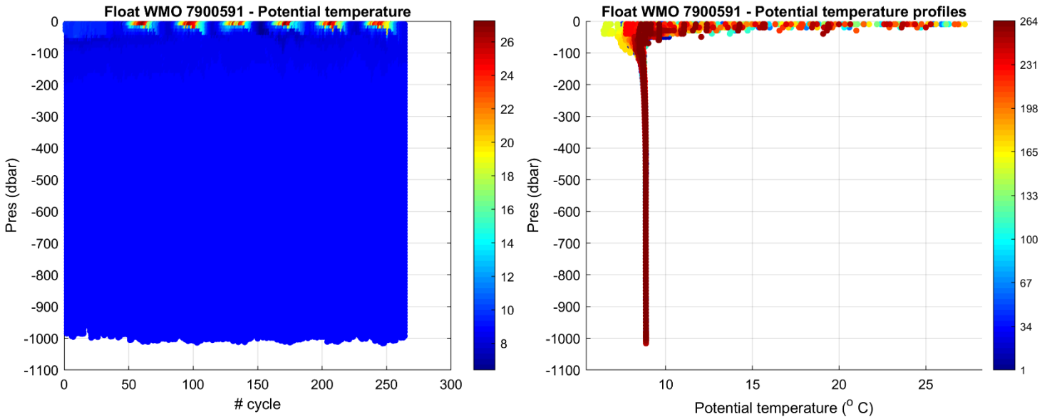
Figure 2: Float 7900591. Time series of Argo float potential temperature ( ^{\circ}\text{C} ) on the left, and potential temperature profiles color-coded per cycle number on the right.
