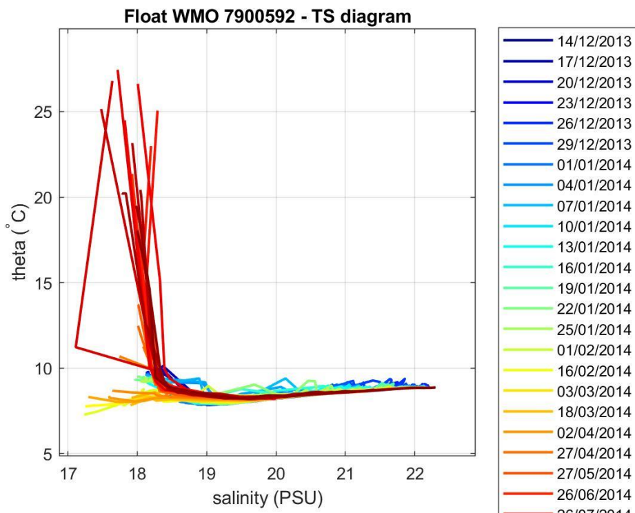
Figure 4: Float 7900592. \theta -S diagram color-coded per cycle number.
