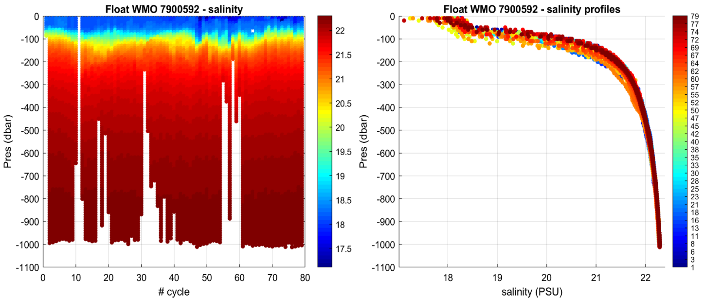
Figure 3: Float 7900592. Time series of Argo float potential salinity (PSS-78) on the left, and salinity profiles color-coded per cycle number on the right.
