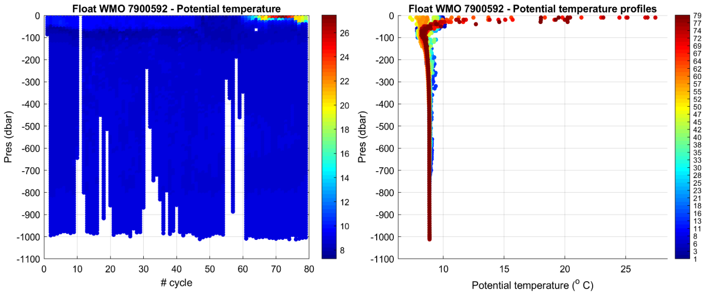
Figure 2: Float 7900592. Time series of Argo float potential temperature ( ^{\circ}\text{C} ) on the left, and potential temperature profiles color-coded per cycle number on the right.
